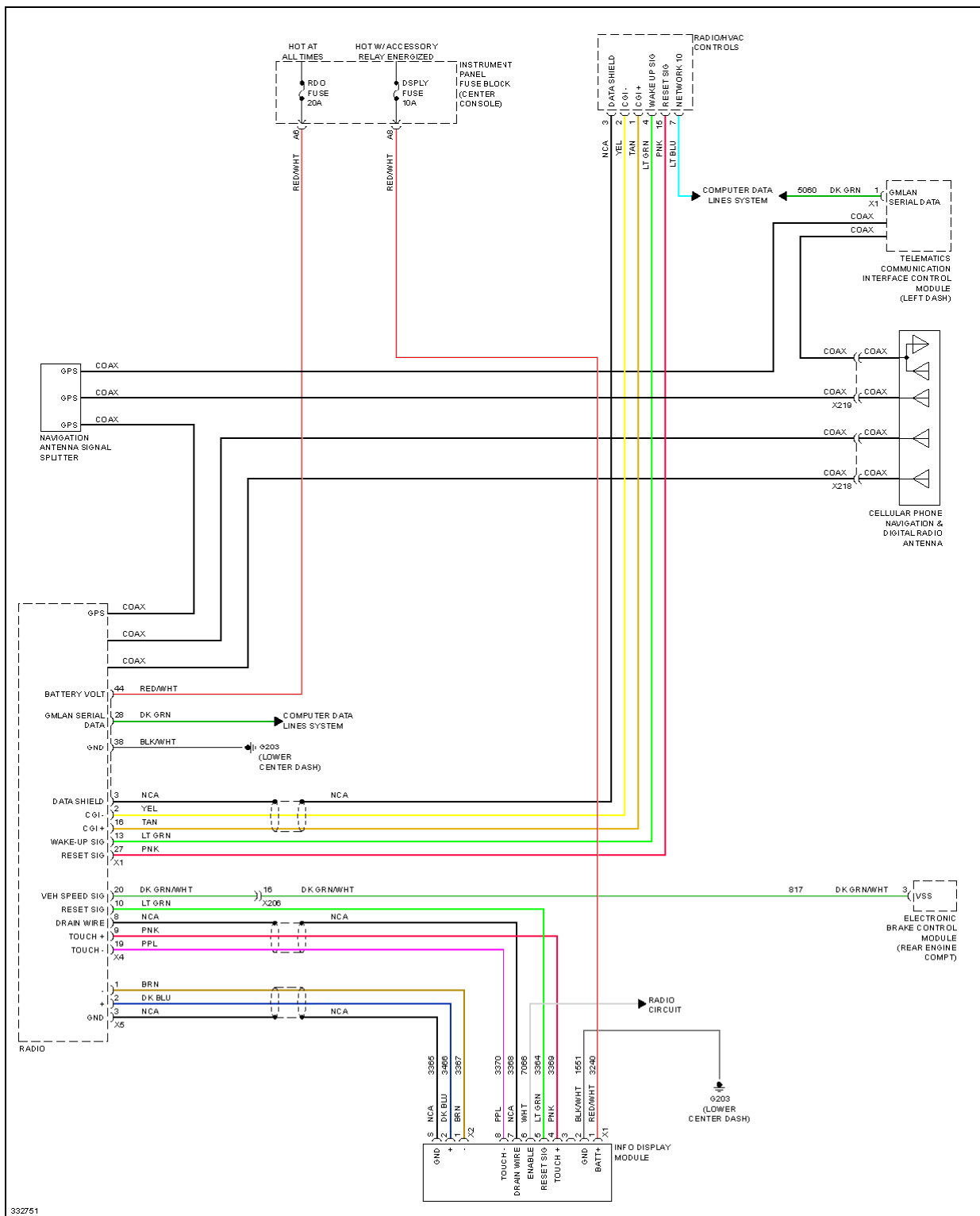
Fig. 46: Navigation Circuit
