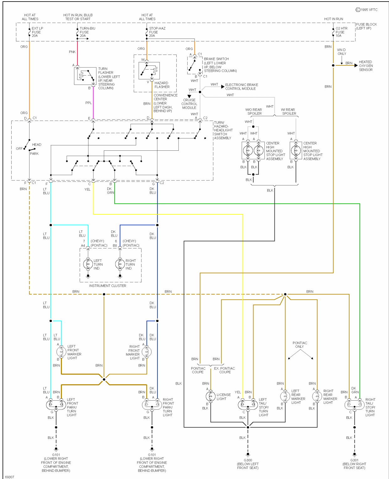
Fig. 18: Park, Stop, Tail & Turn Lamps Circuit
