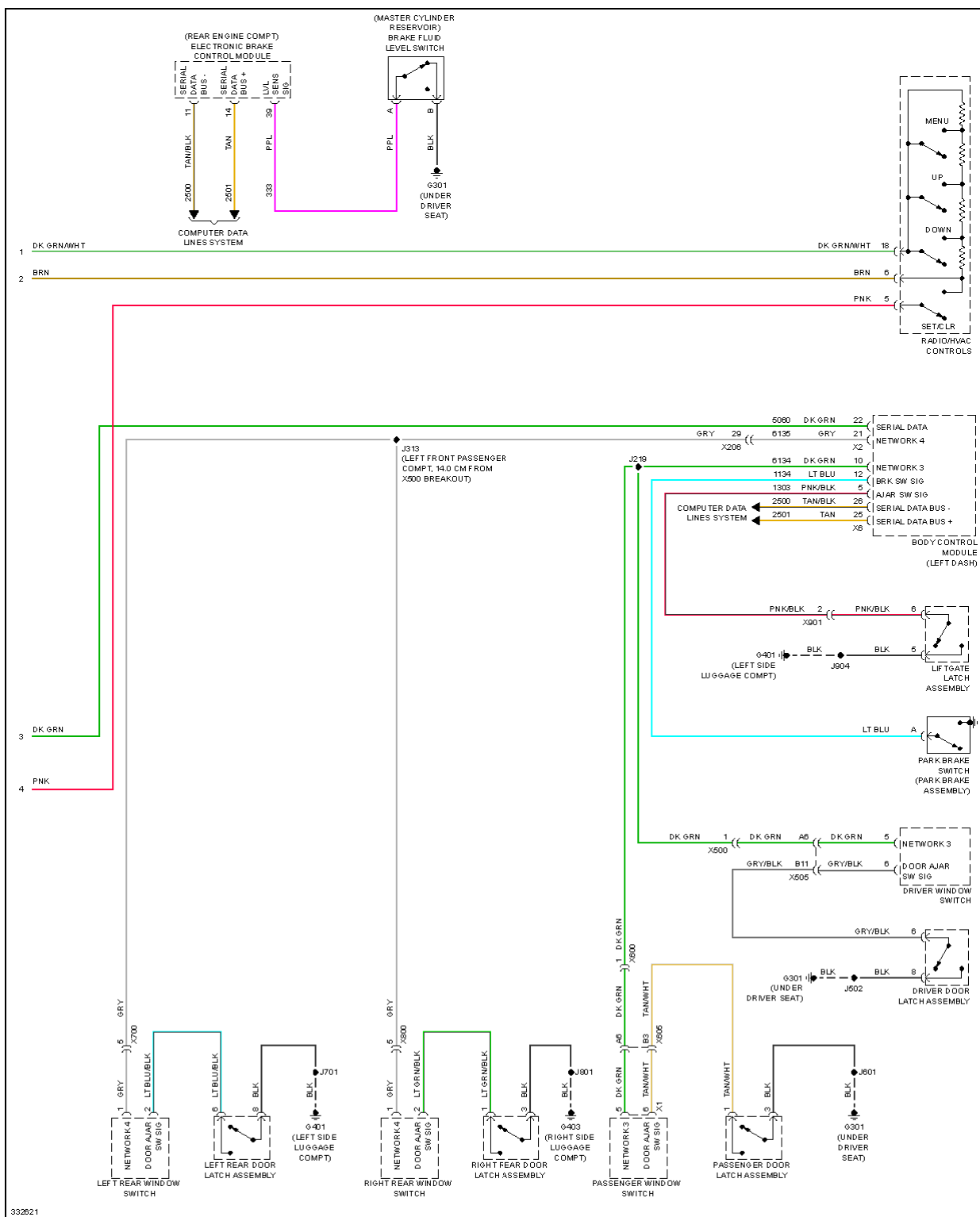
Fig. 39: Instrument Cluster Circuit (2 of 2)
