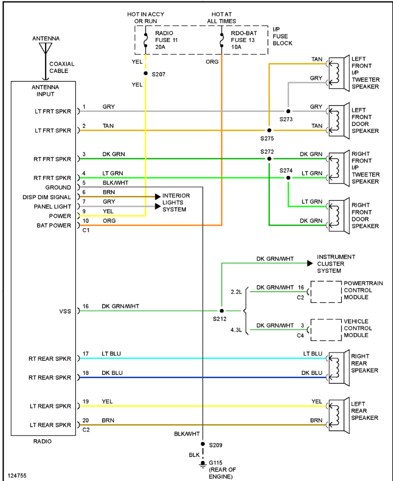
Fig. 31: 6-Speaker System Circuit
