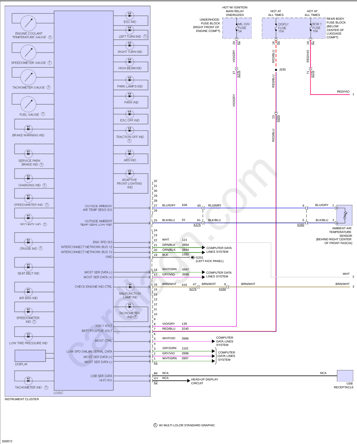
Fig 2: Instrument Cluster Circuit (1 of 3)
