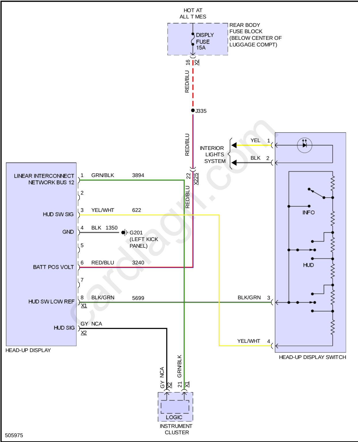
Fig 1: Head-Up Display Circuit
