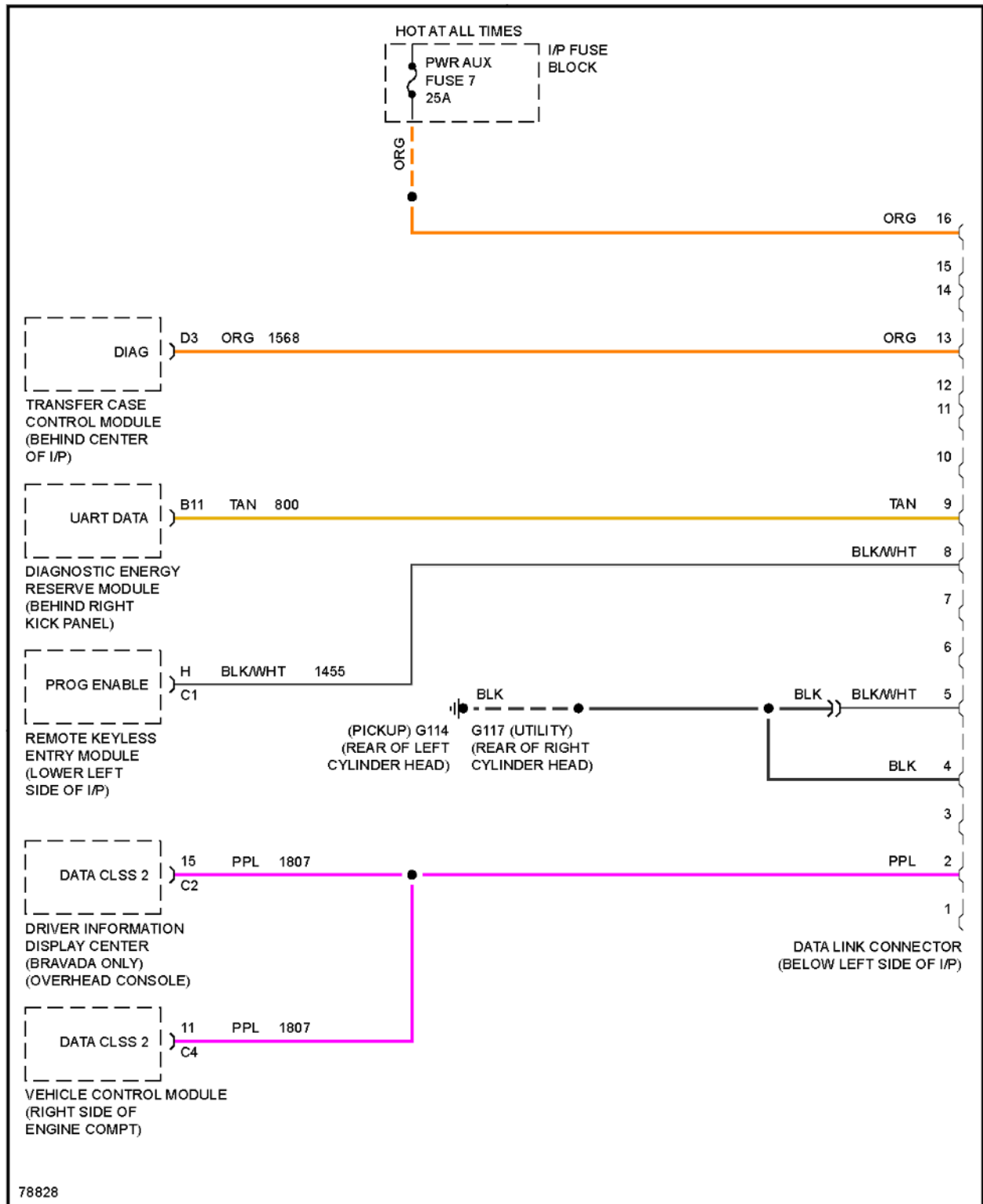
Fig. 3: 4.3L (VIN W), Computer Data Lines
