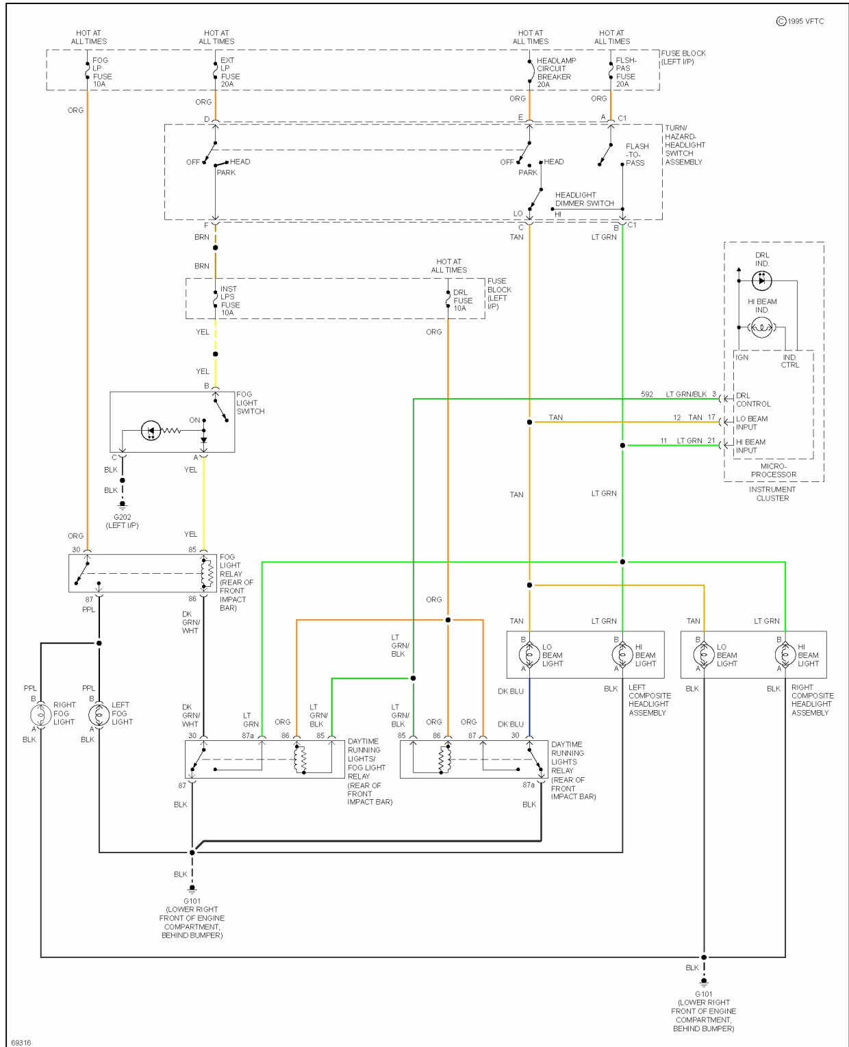
Fig. 22: Fog Lamps Circuit, W/ DRL
