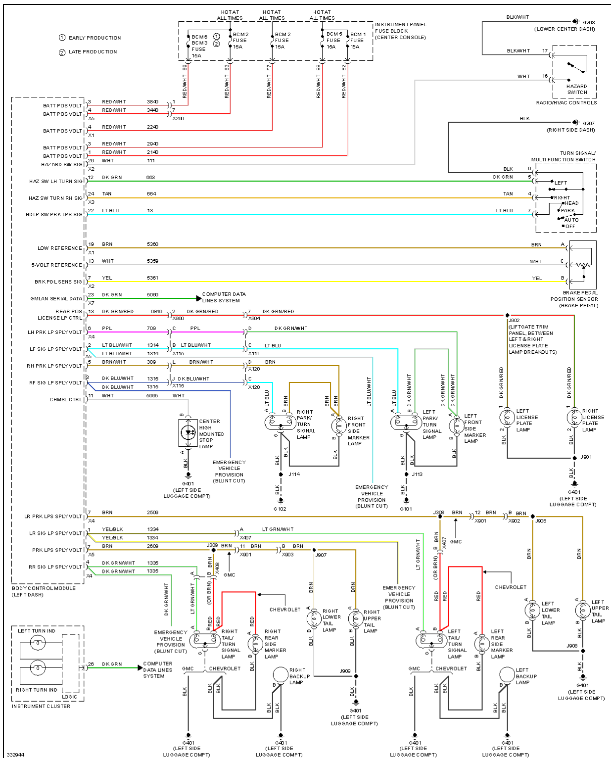
Fig. 30: Exterior Lamps Circuit
