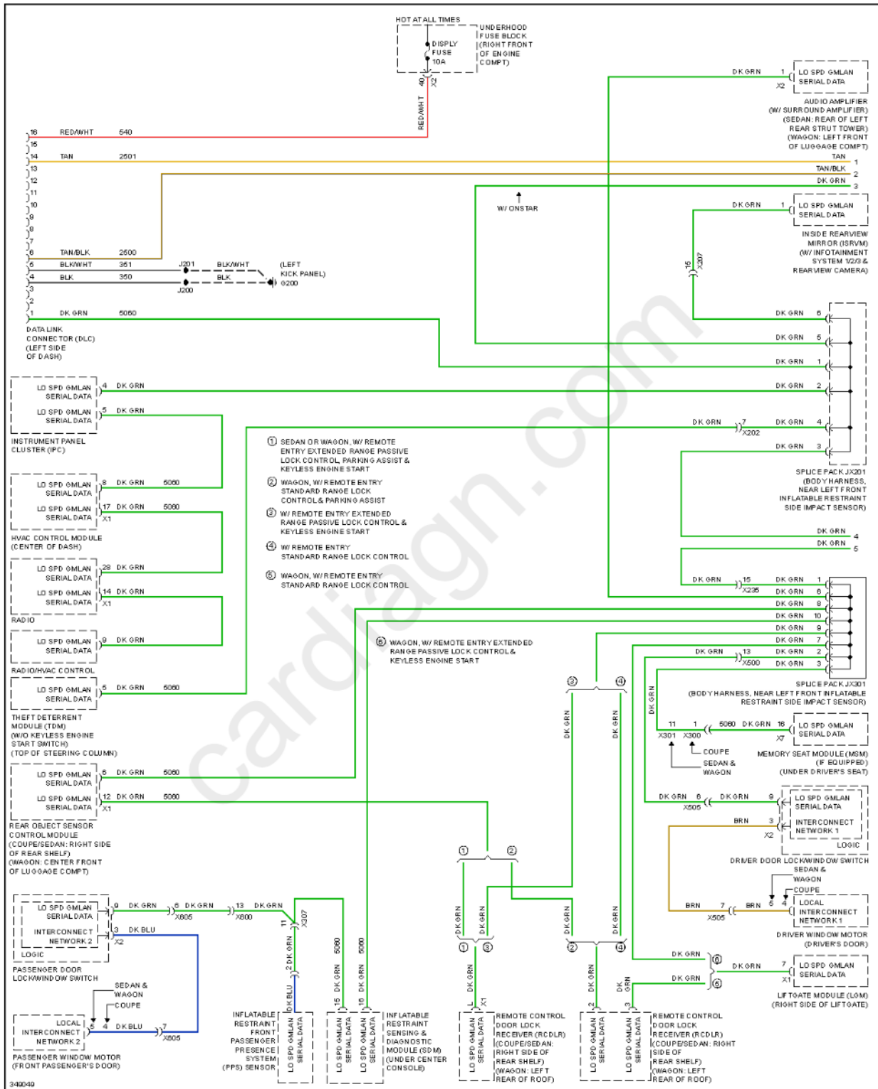
Fig. 12: 3.0L VIN Y, Computer Data Lines Circuit (1 of 3)
