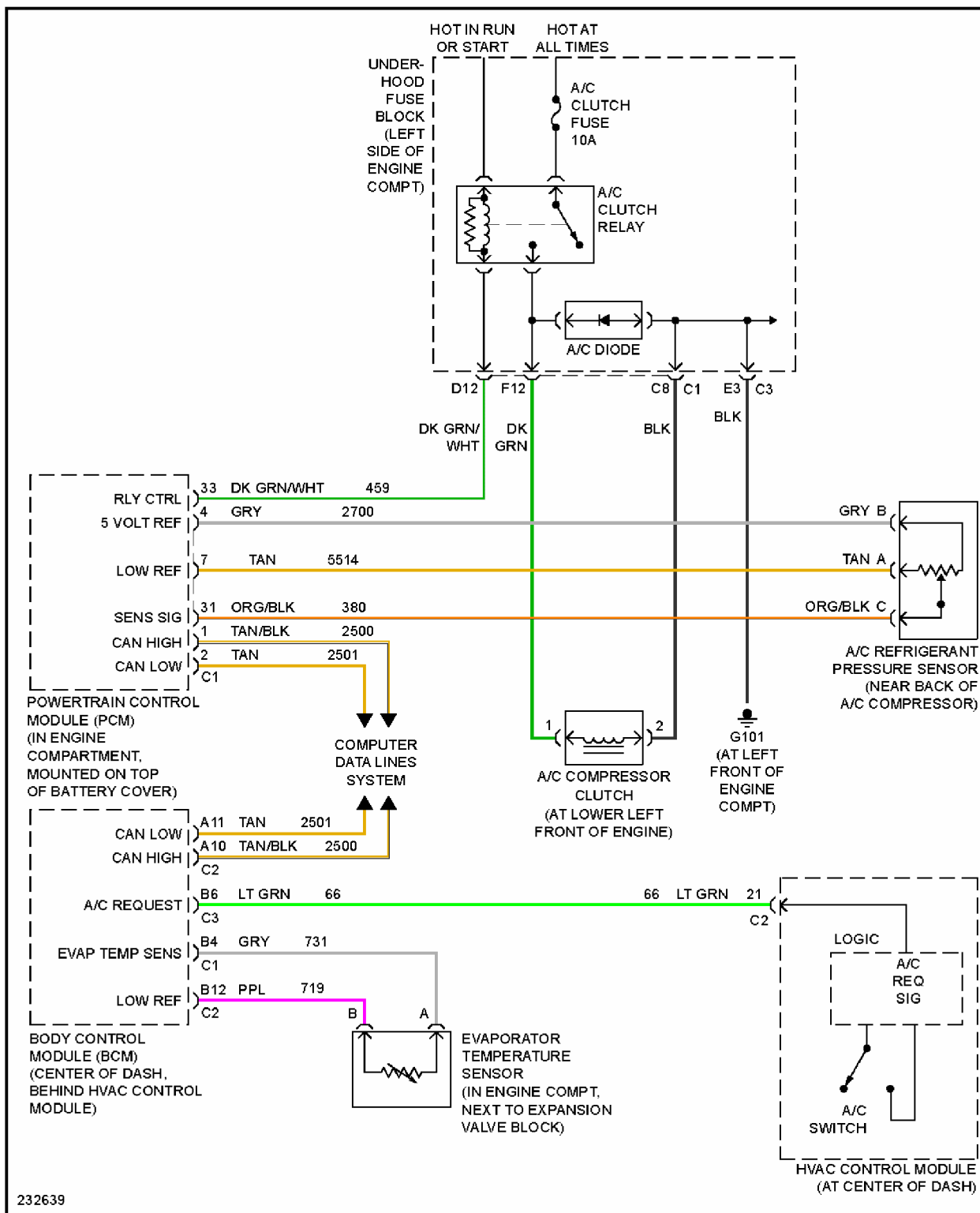
Fig. 1: Compressor Circuit
