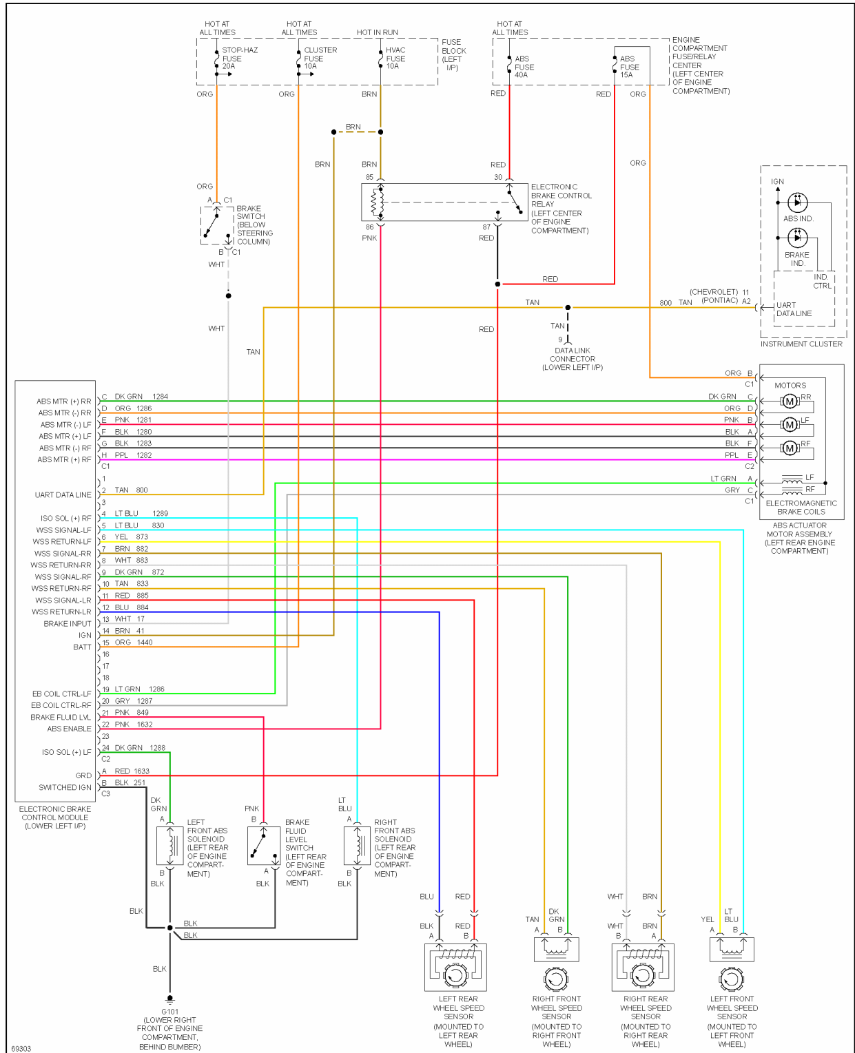
Fig. 3: Anti-lock Brake Circuits, W/ Traction Control
