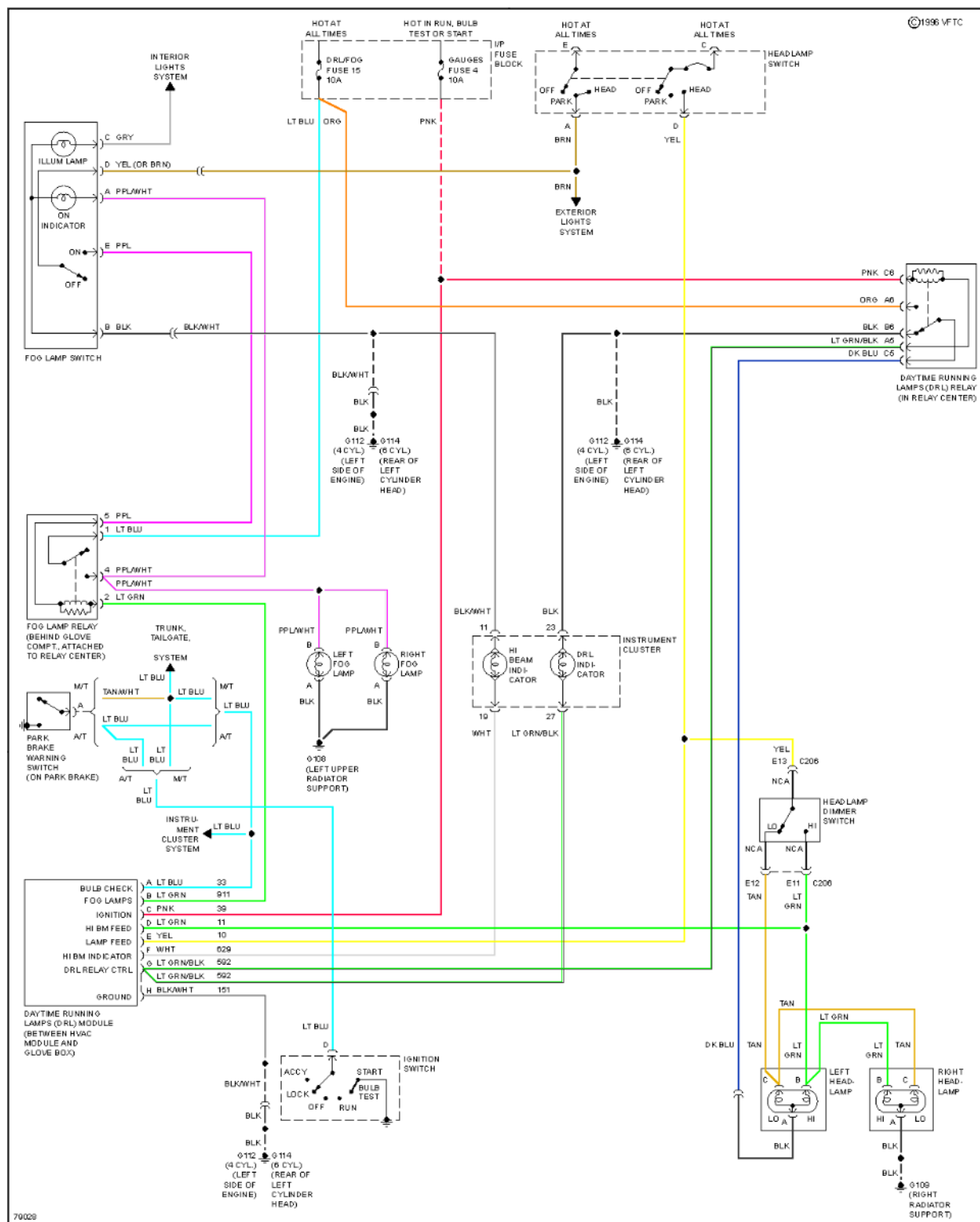
Fig. 15: Headlight Circuit, W/ Sealed Beam Lamps
