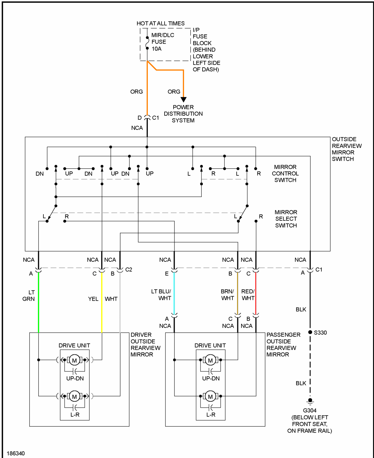
Fig. 26: Power Mirrors Circuit
