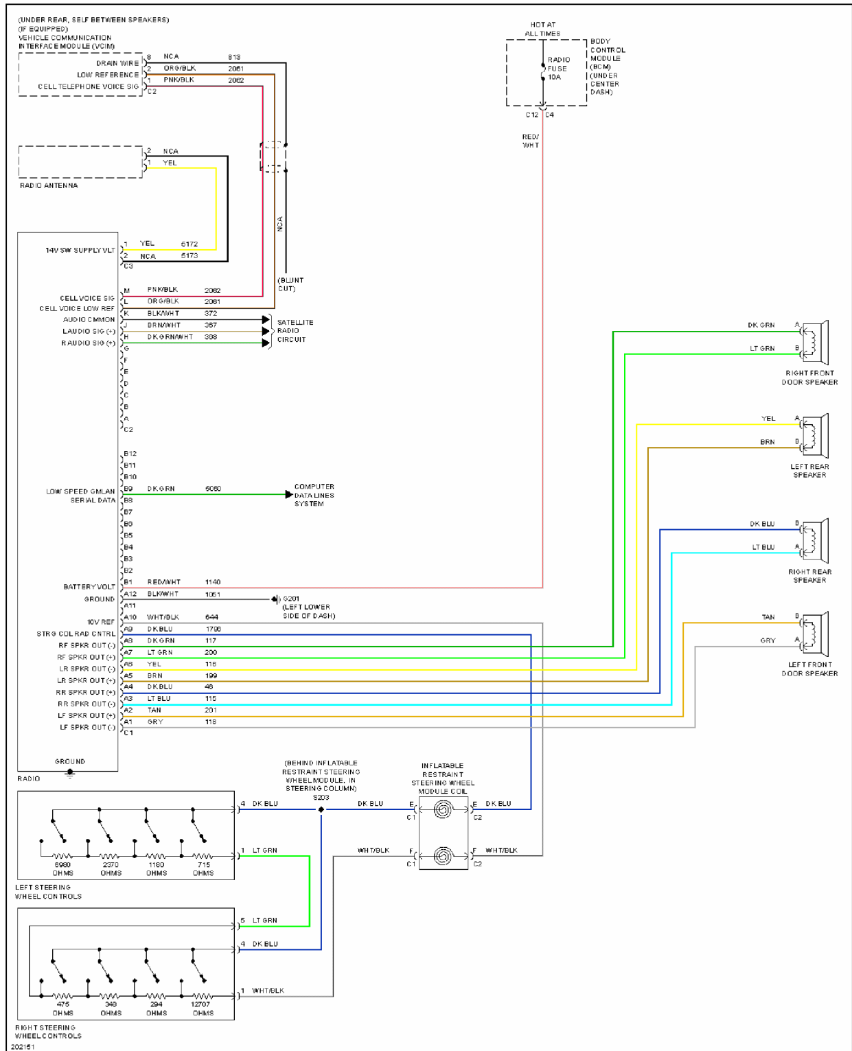
Fig. 51: Radio Circuit, W/O Amplifier
