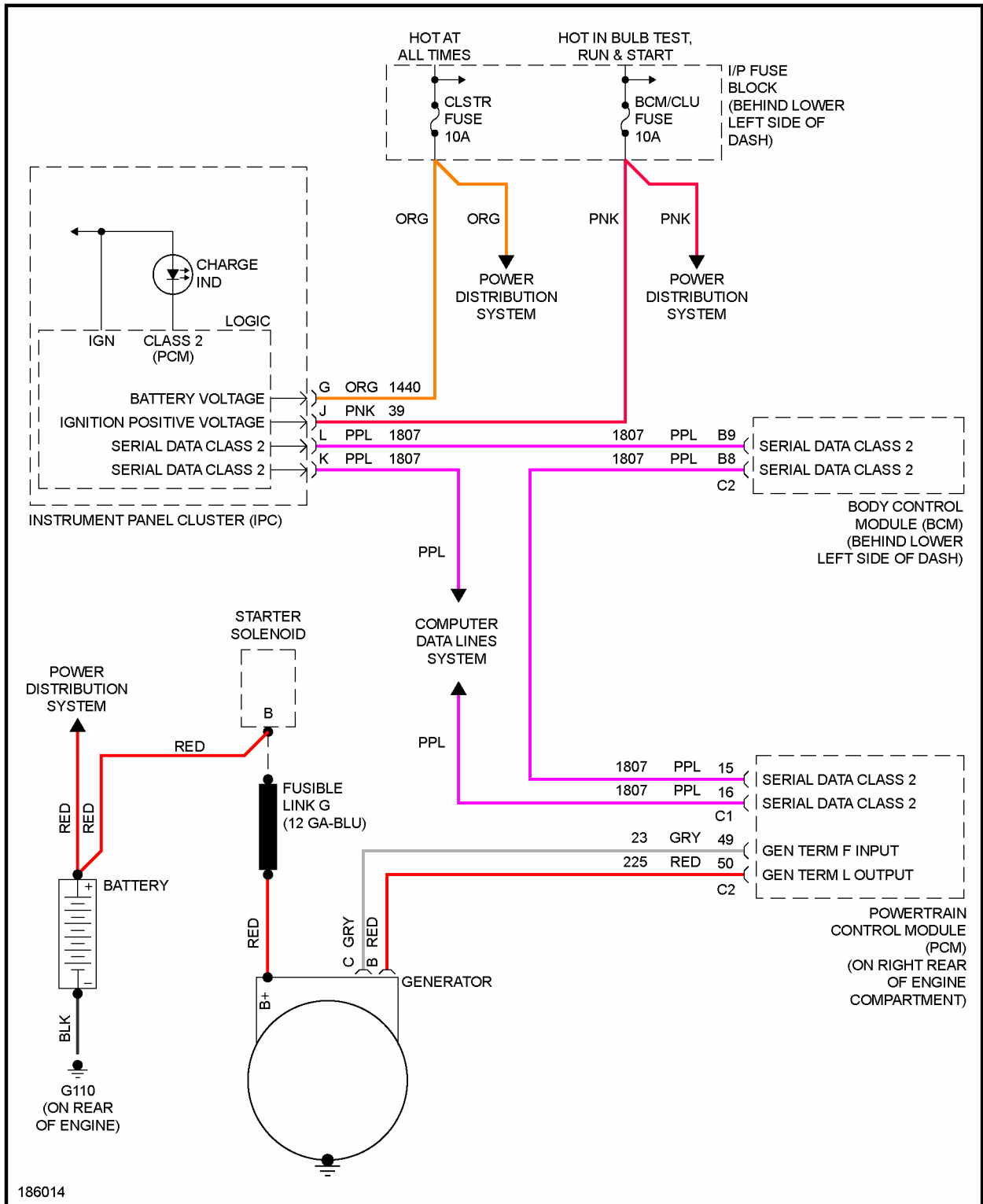
Fig. 36: Charging Circuit
