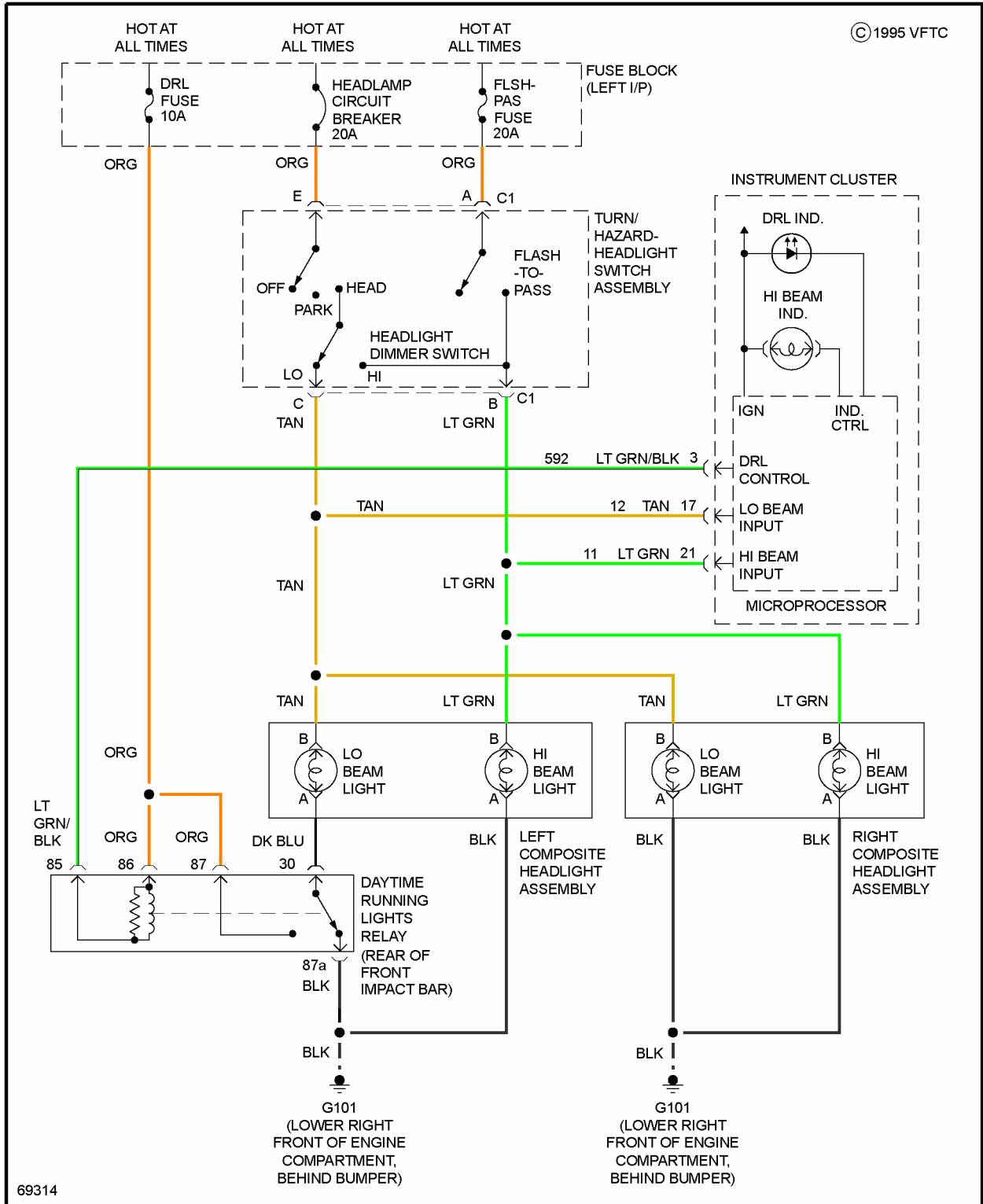
Fig. 24: Headlamps Circuit, W/ DRL
