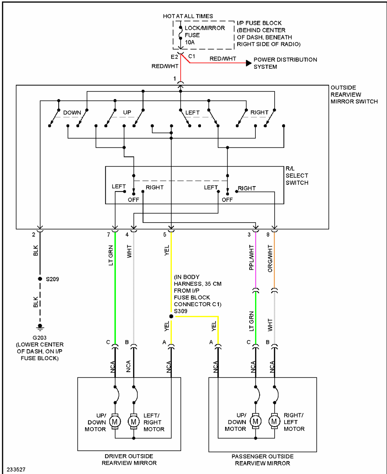
Fig. 33: Power Mirrors Circuit
