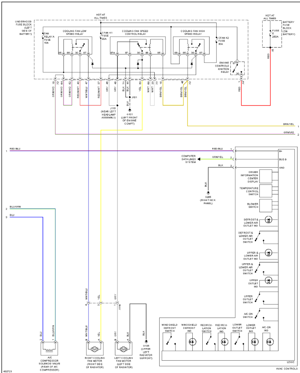
Fig. 6: Manual A/C Circuit (2 of 4)
