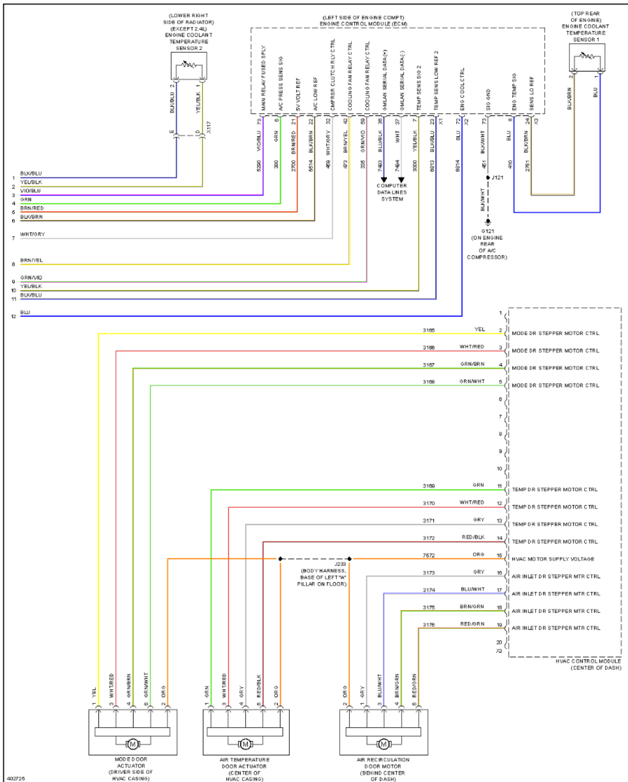
Fig. 8: Manual A/C Circuit (4 of 4)
