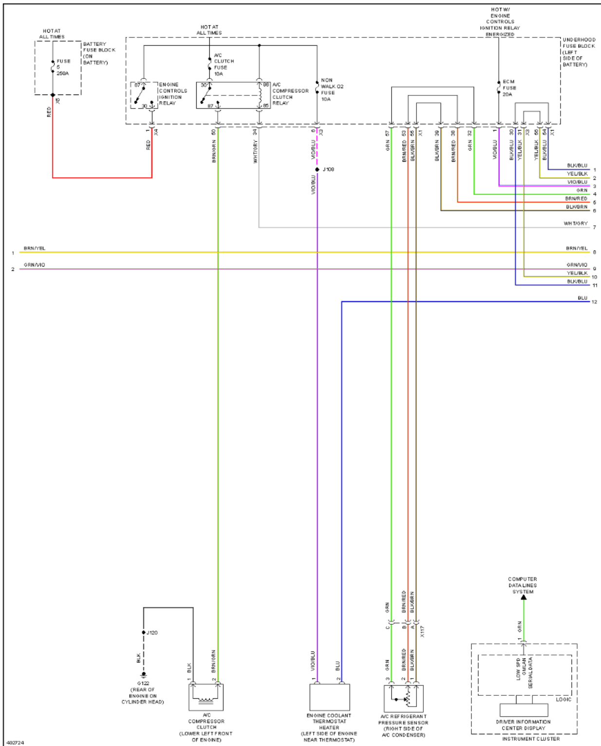
Fig. 7: Manual A/C Circuit (3 of 4)
