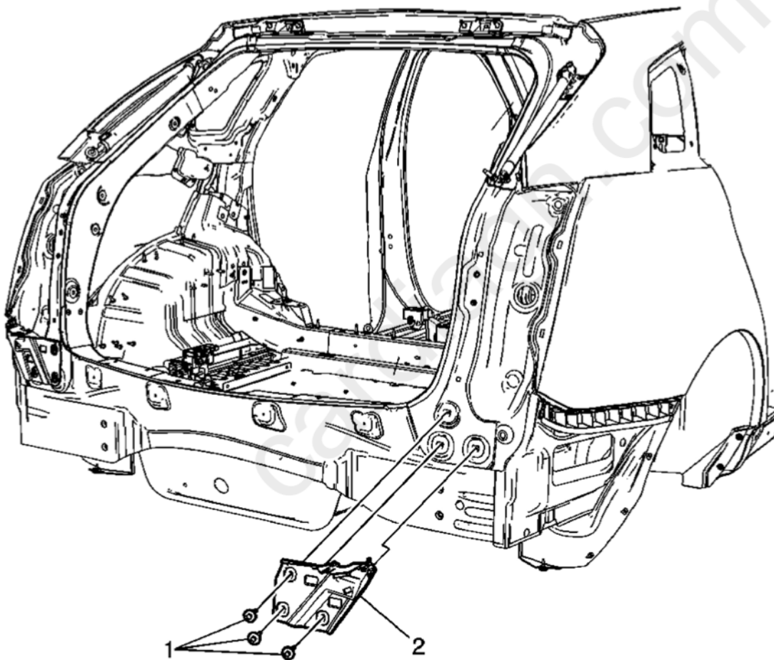
Fig. 12: Identifying Rear Bumper Fascia Bracket & Fasteners Outer Courtesy of GENERAL MOTORS CORP.
