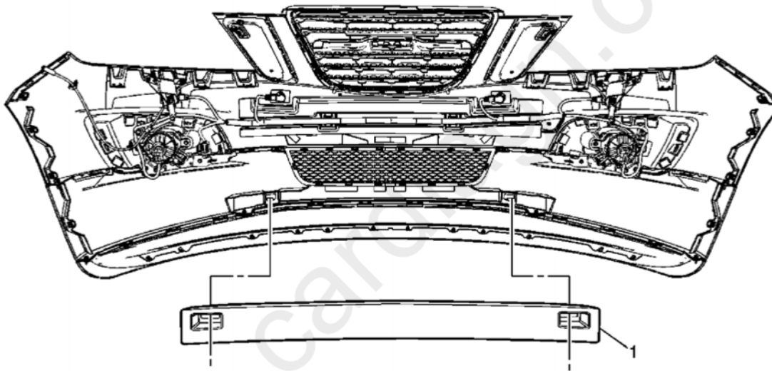
Fig. 2: View Of Front Bumper Fascia Energy Lower Absorber Courtesy of GENERAL MOTORS CORP.
