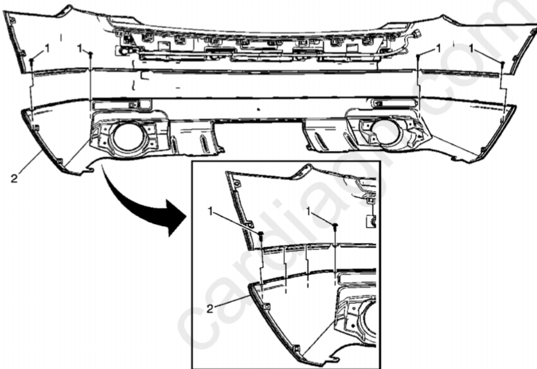
Fig. 1 : Identifying Rear Bumper Lower Fascia Courtesy of GENERAL MOTORS CORP.
