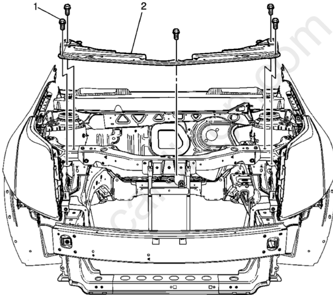
Fig. 8: Identifying Front Bumper Fascia Upper Support & Fasteners Courtesy of GENERAL MOTORS CORP.
