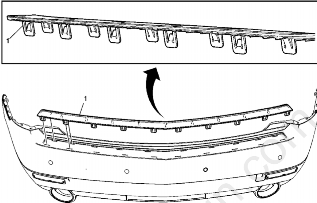
Fig. 19: Identifying Rear Bumper Fascia Step Pad Courtesy of GENERAL MOTORS CORP.
