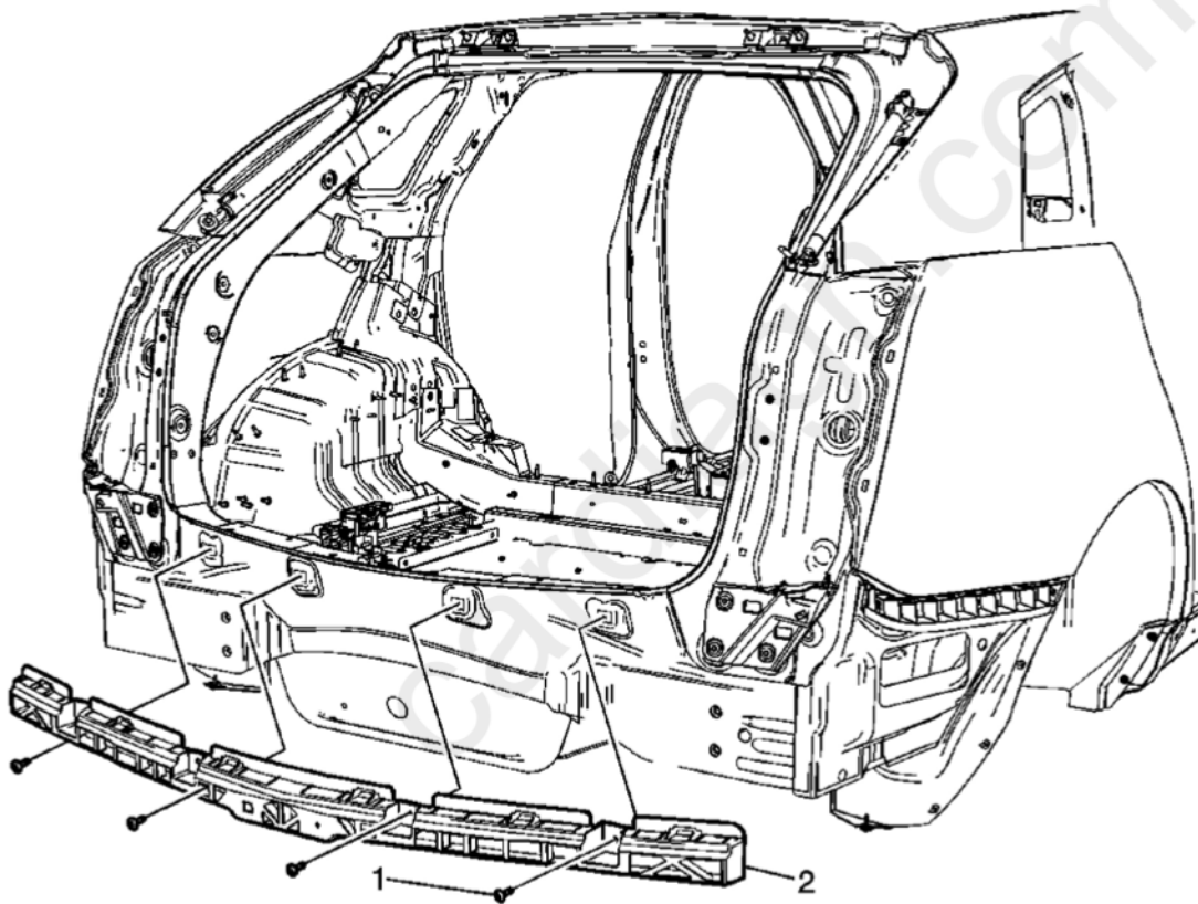
Fig. 1 : View Of Rear Bumper Fascia Center Bracket Courtesy of GENERAL MOTORS CORP.
