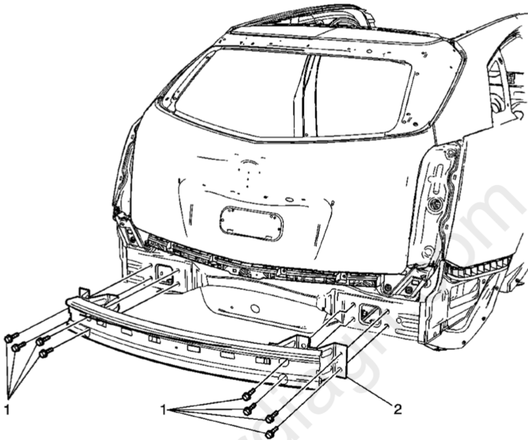
Fig. 18: View Of Rear Bumper Impact Bar & Bolts (South Korea) Courtesy of GENERAL MOTORS CORP.
