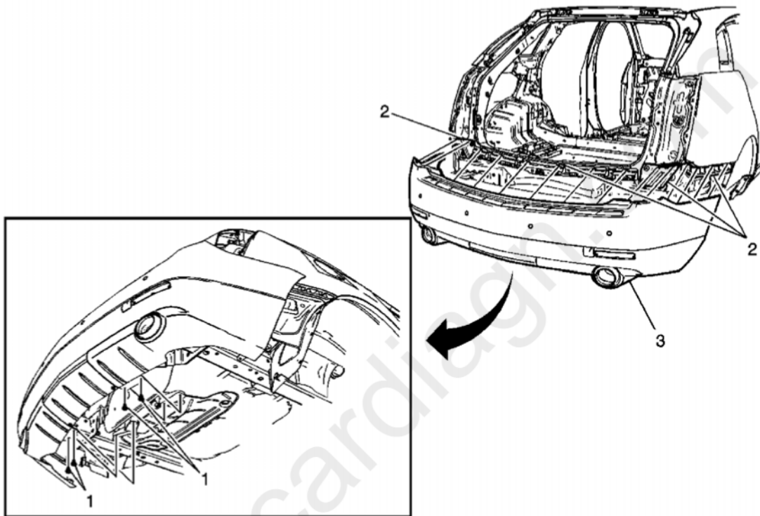
Fig. 10: View Of Rear Bumper Fascia Courtesy of GENERAL MOTORS CORP.
