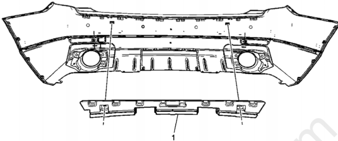
Fig. 16: View Of Rear Bumper Energy Absorber Courtesy of GENERAL MOTORS CORP.
