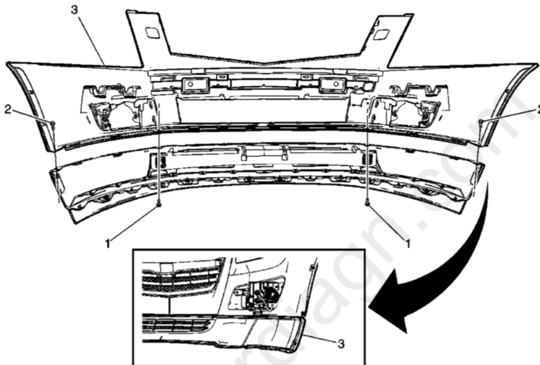
Fig. 7: Identifying Front Bumper Upper Fascia Courtesy of GENERAL MOTORS CORP.
