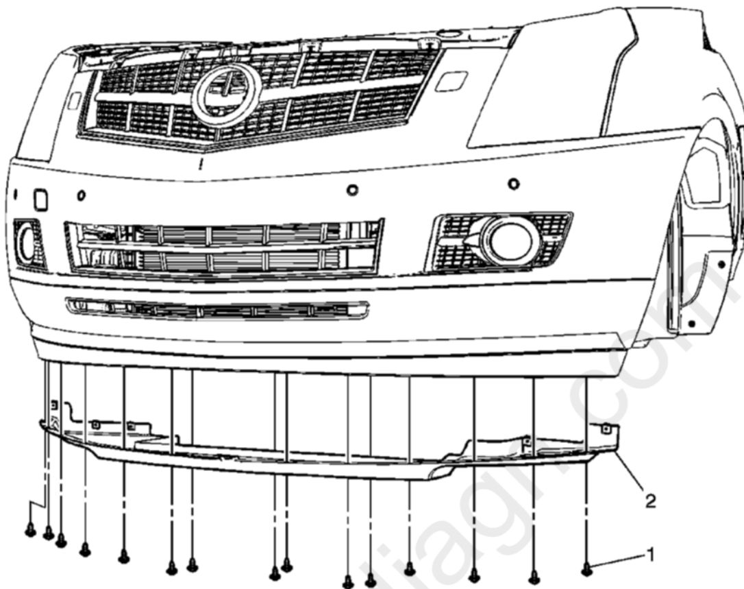
Fig. 21: View Of Radiator Air Lower Deflector & Retainers Courtesy of GENERAL MOTORS CORP.
