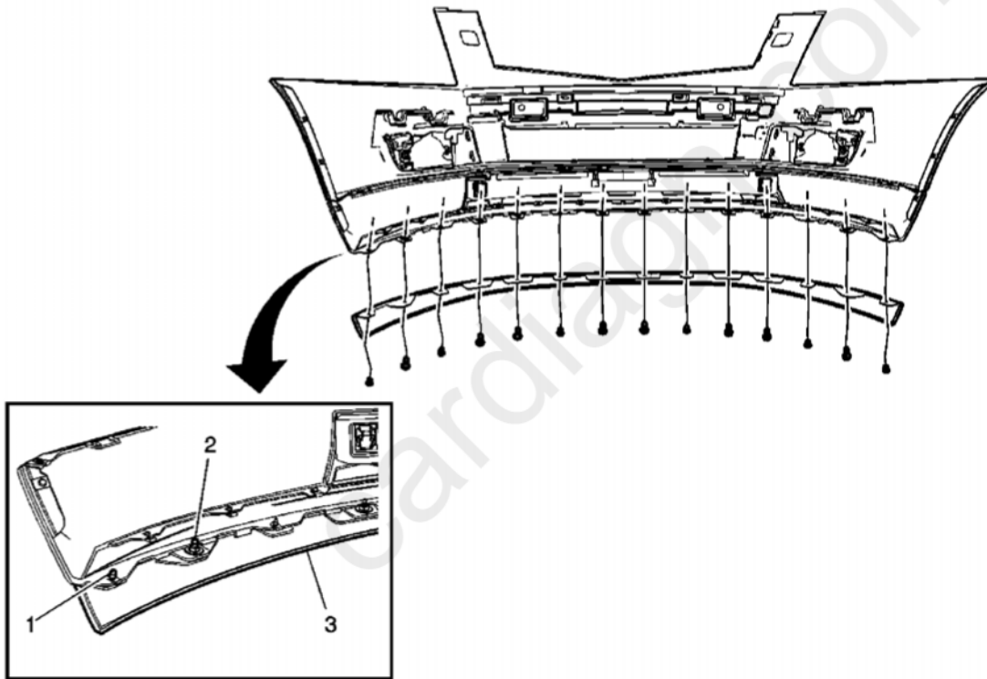
Fig. 9: View Of Front Bumper Fascia Lower Deflector & Fasteners Courtesy of GENERAL MOTORS CORP.
