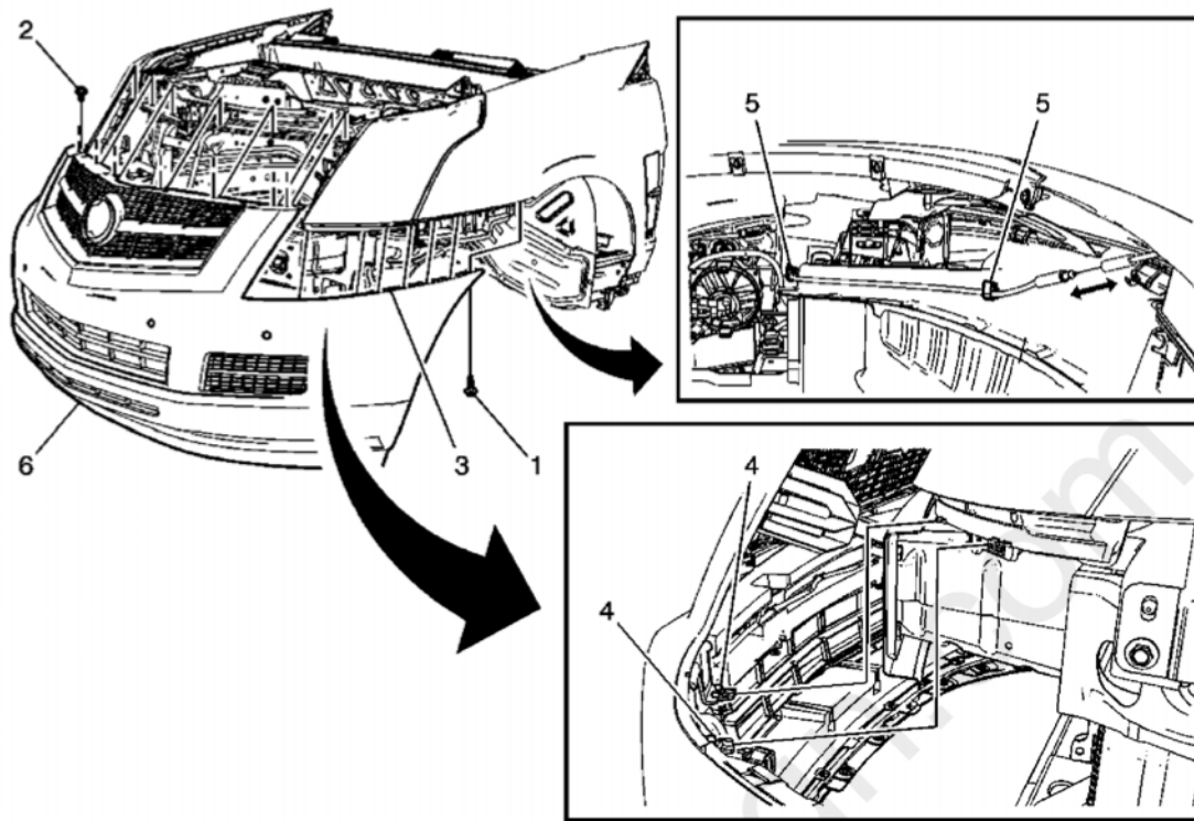
Fig. : Identifying Front Bumper Fascia Courtesy of GENERAL MOTORS CORP.
