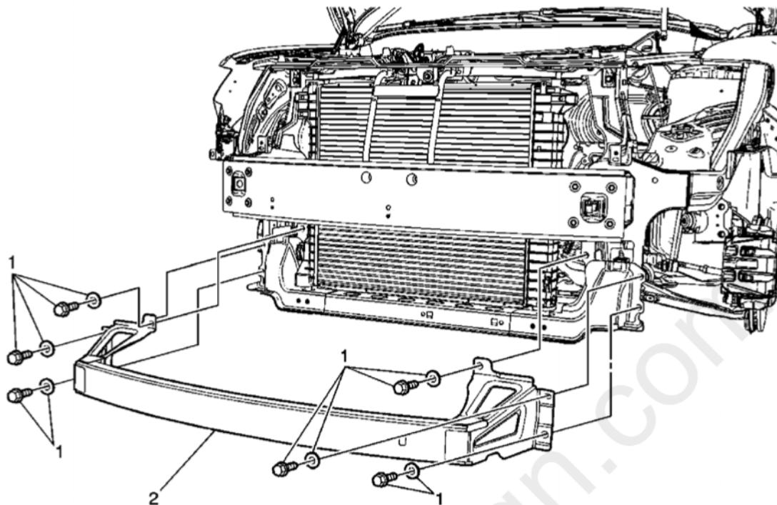
Fig. : View Of Front Bumper Lower Impact Bar Courtesy of GENERAL MOTORS CORP.
