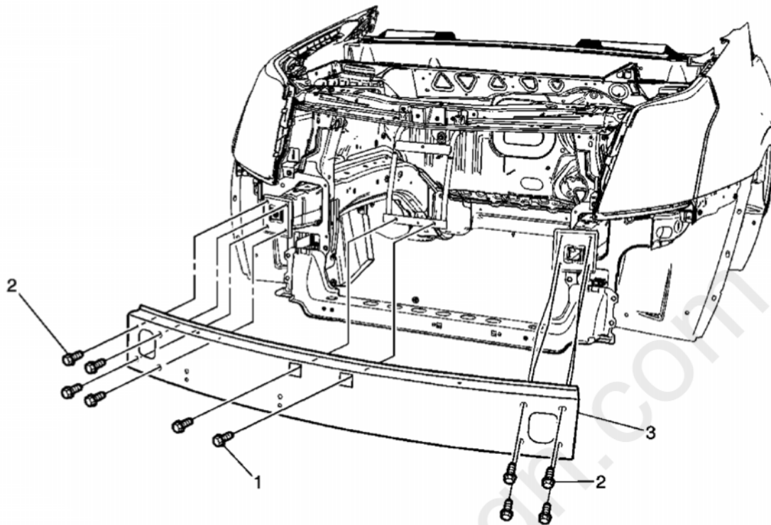
Fig. : Identifying Front Bumper Upper Impact Bar & Bolts Courtesy of GENERAL MOTORS CORP.
