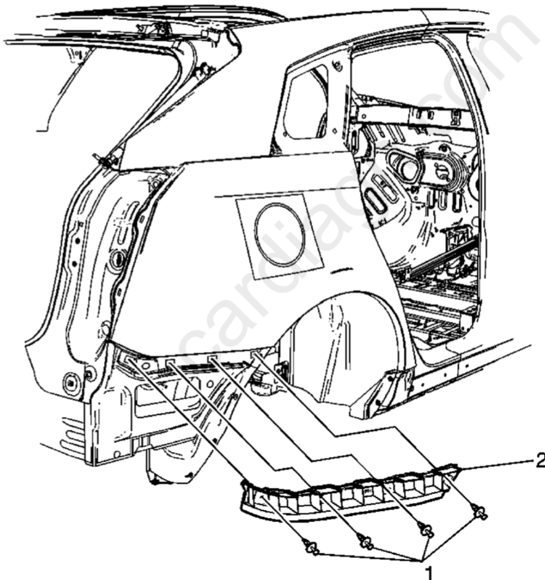
Fig. 11: Identifying Rear Bumper Fascia Bracket & Fasteners Side Courtesy of GENERAL MOTORS CORP.
