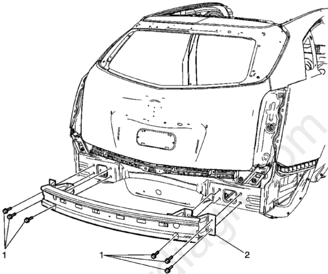
Fig. 17: View Of Rear Bumper Impact Bar & Bolts (North America) Courtesy of GENERAL MOTORS CORP.
