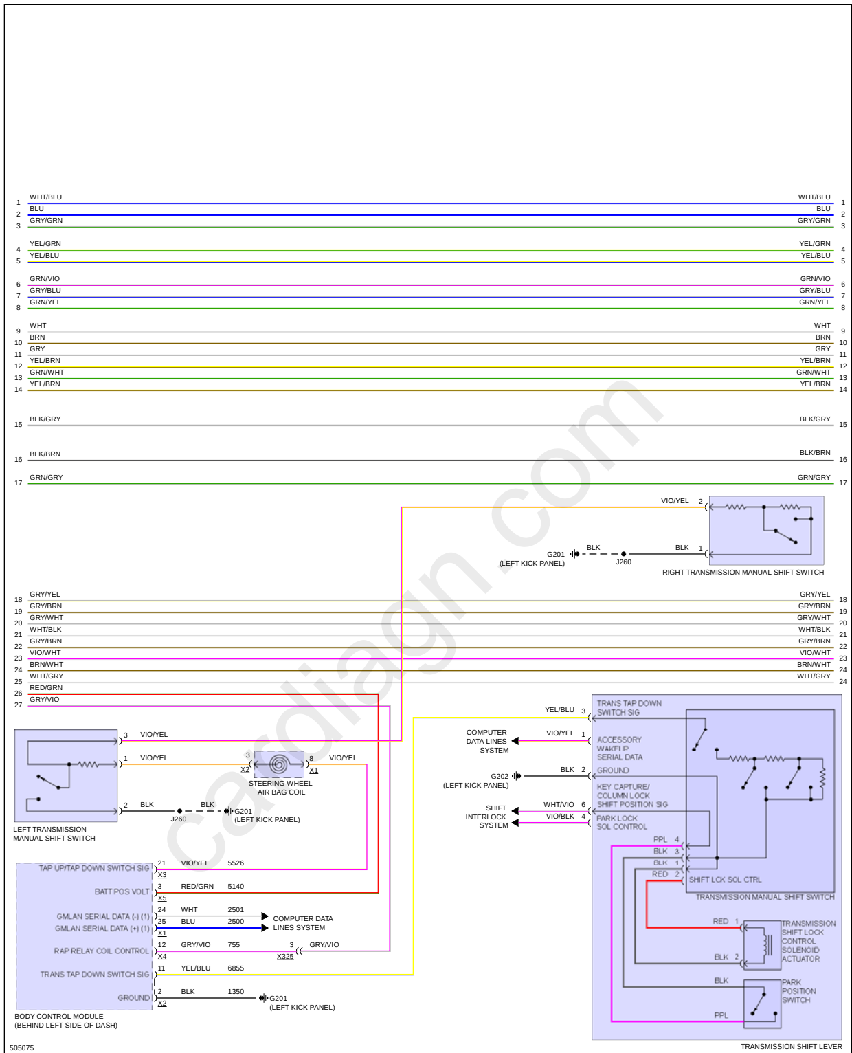
Fig 2: Transmission Circuit (2 of 3)
