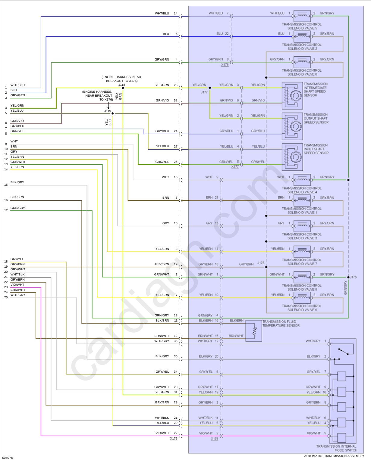
Fig 3: Transmission Circuit (3 of 3)
