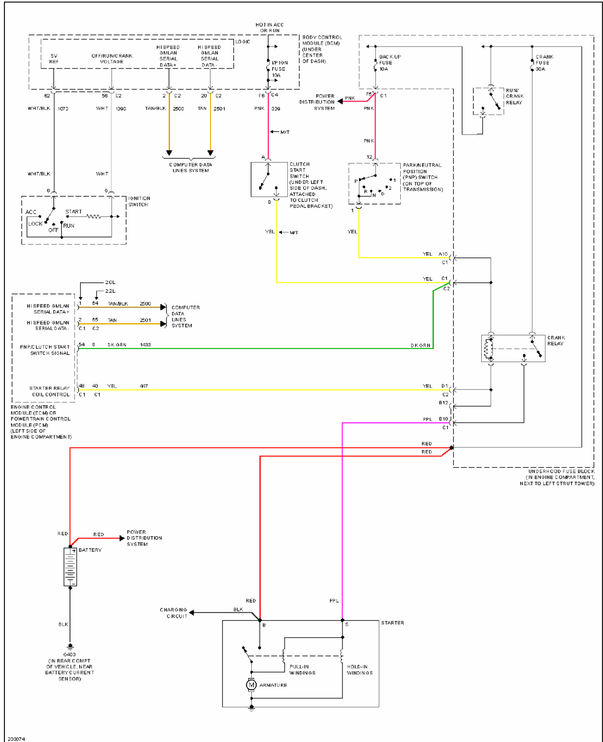
Fig. 55: Starting Circuit
