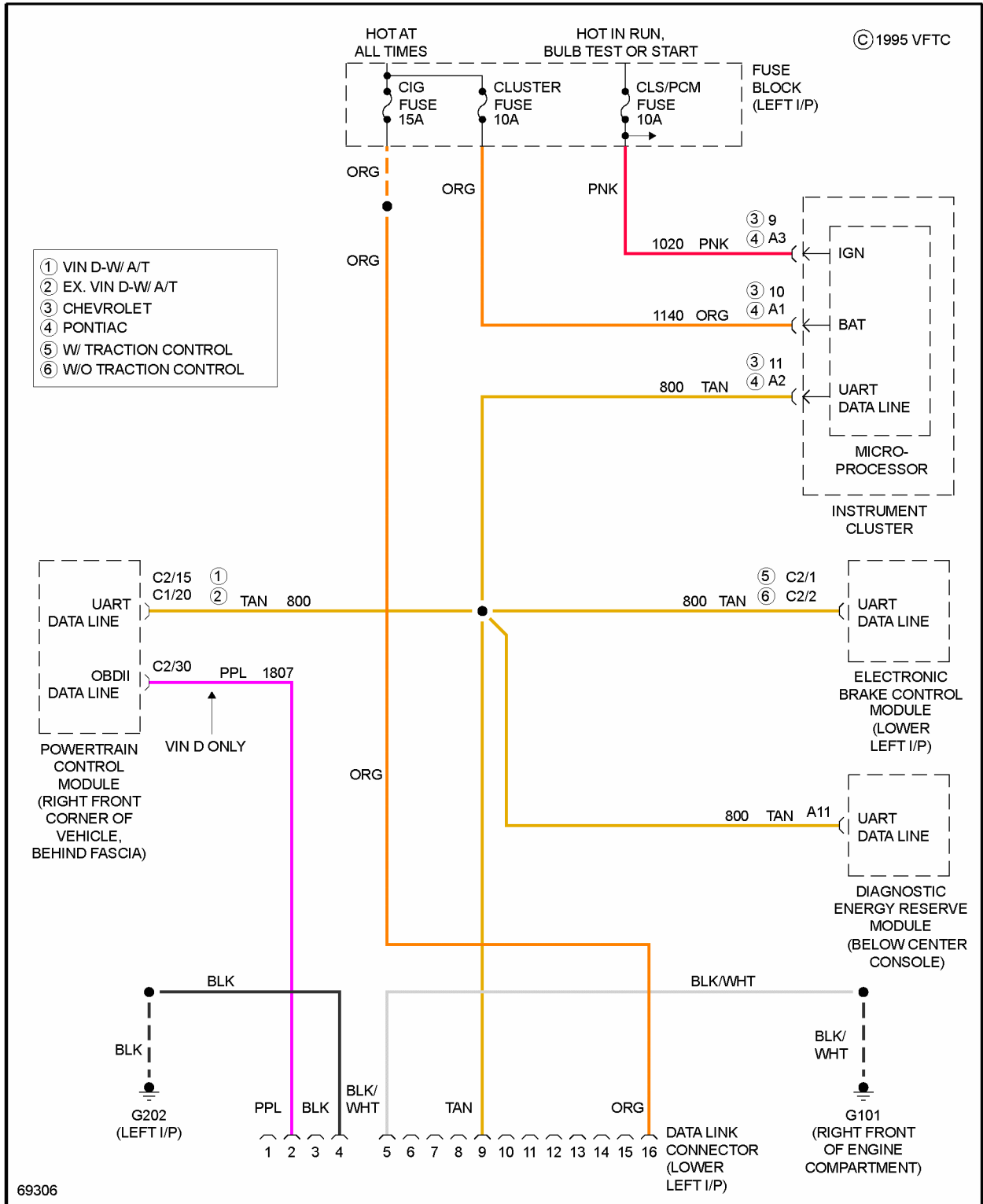
Fig. 6: Data Link Connector Circuit
