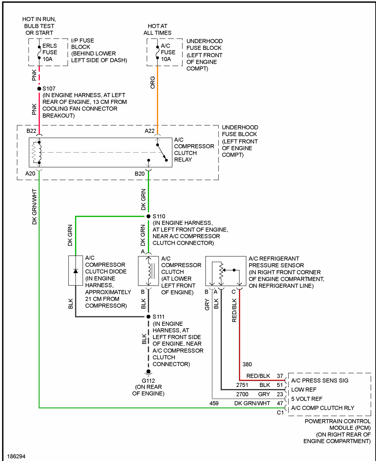
Fig. 1: Compressor Circuit
