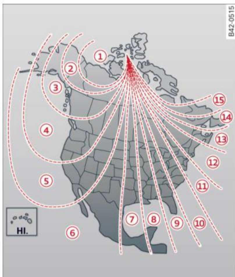
Fig. 75 Magnetic deflection zone boundaries
