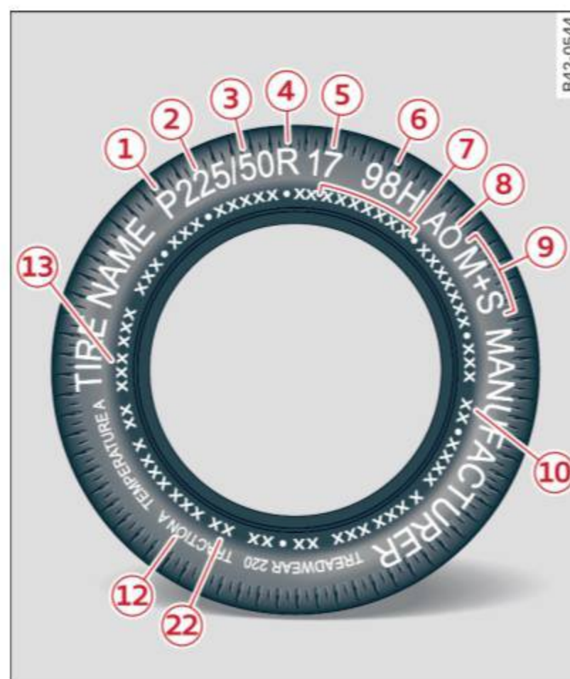
Fig. 153 Tire specification codes on the sidewall of a tire
