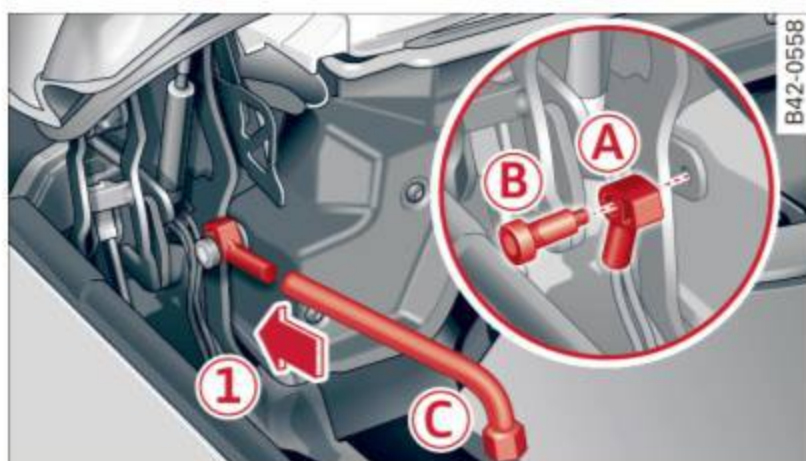
Fig. 56 Convertible top storage bay: installing the driver
