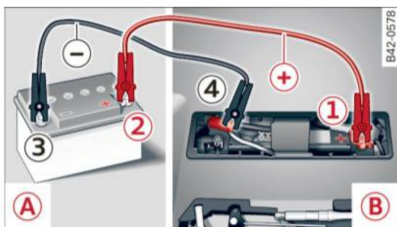
Fig. 163 Jump start using the battery in another vehicle: A - Female socket, B - Discharge
