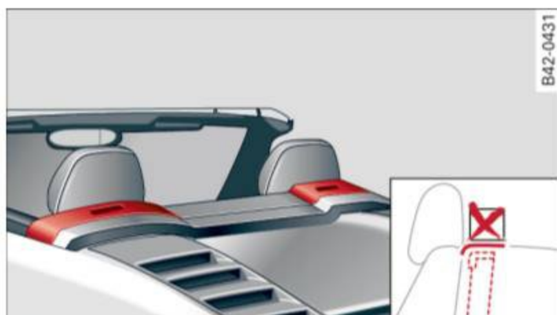
Fig. 108 Rollbar deployment range
