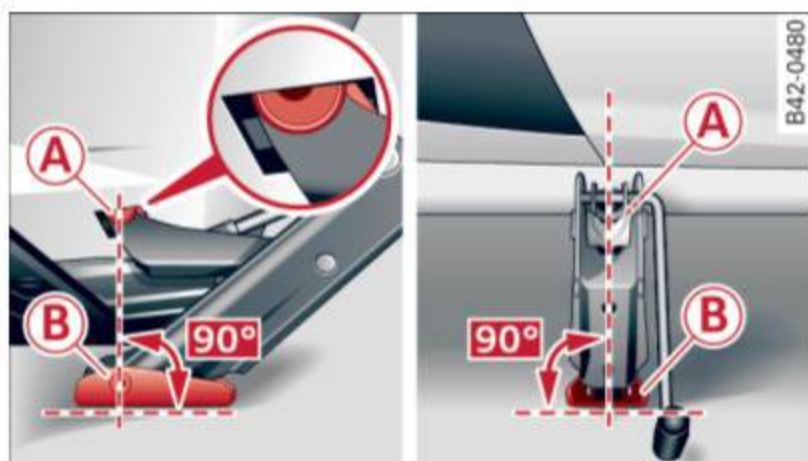
Fig. 160 Close-up: proper positioning of lifting jack
