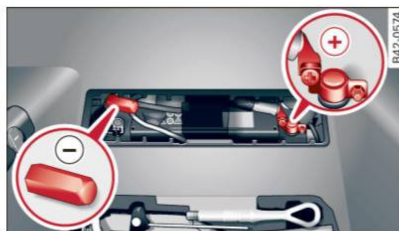
Fig. 148 Luggage compartment: connectors for a charger and jump start cables
