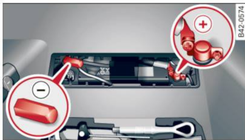
Fig. 162 Luggage compartment: connectors for a charger and jump start cables
