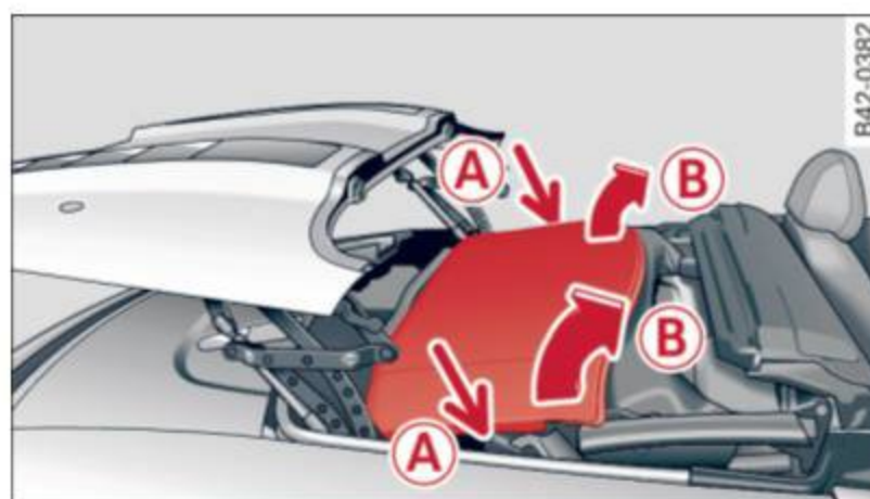
Fig. 54 Convertible top storage bay: lifting the convertible top out
