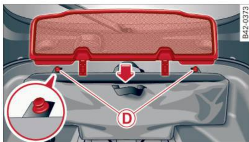
Fig. 45 Luggage compartment: storing the wind deflector
