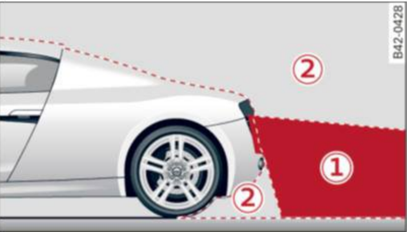
Fig. 95 Side view: Rearview camera coverage area
