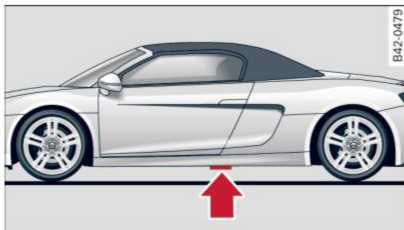
Fig. 159 Changing a wheel: mounting point for the jack
