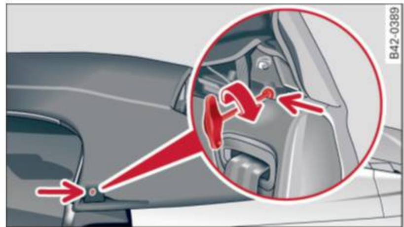
Fig. 61 Interior: tightening the bolt
