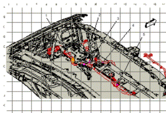
Fig. 2: Forward Lamp Harness Routing - Left Engine Compartment (HP5)
