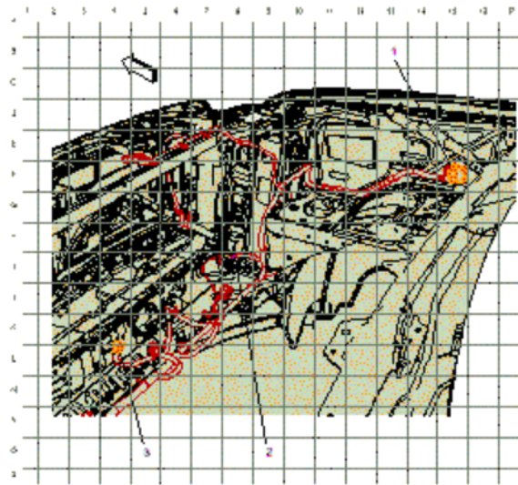
Fig. 5: Engine Compartment Right Harness Routing Courtesy of GENERAL MOTORS COMPANY
