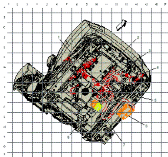
Fig. 12: Bottom of Driver Seat Harness Routing Courtesy of GENERAL MOTORS COMPANY
