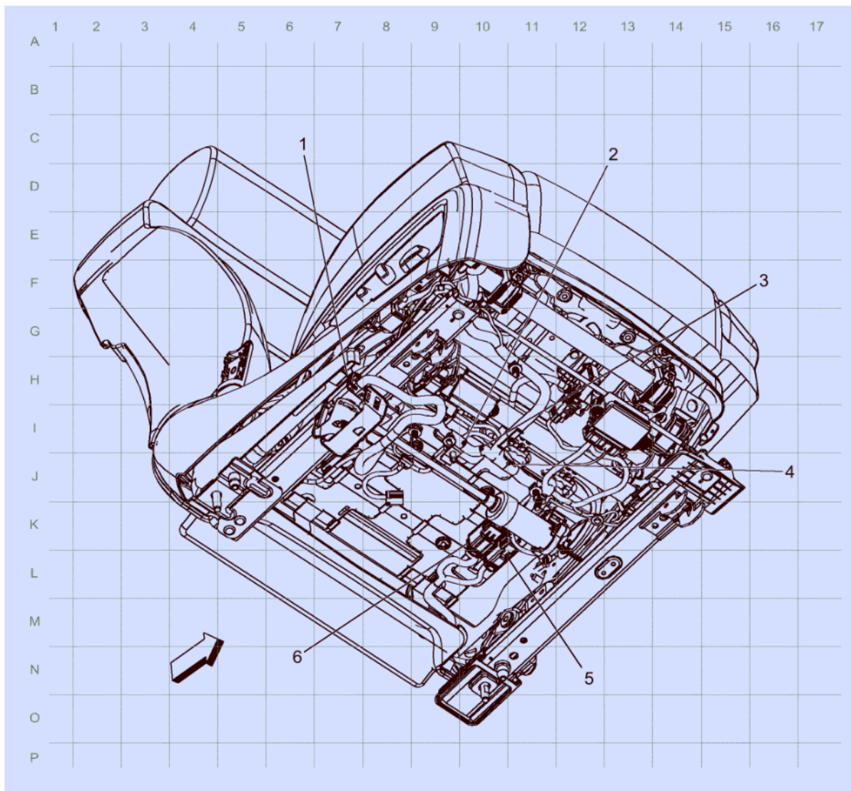
Fig. 16: Bottom of Passenger Seat Harness Routing
