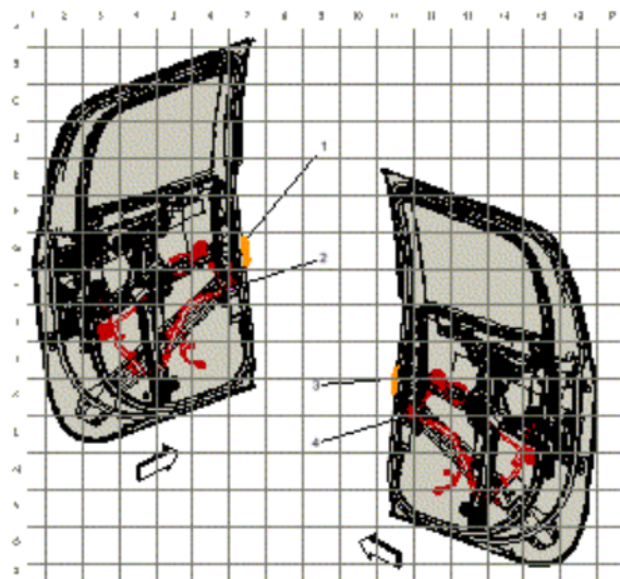
Fig. 21: Rear Doors Harness Routing Courtesy of GENERAL MOTORS COMPANY
