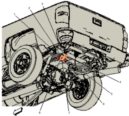
Fig. 26: Chassis Jumper Harness Routing (UY2)
