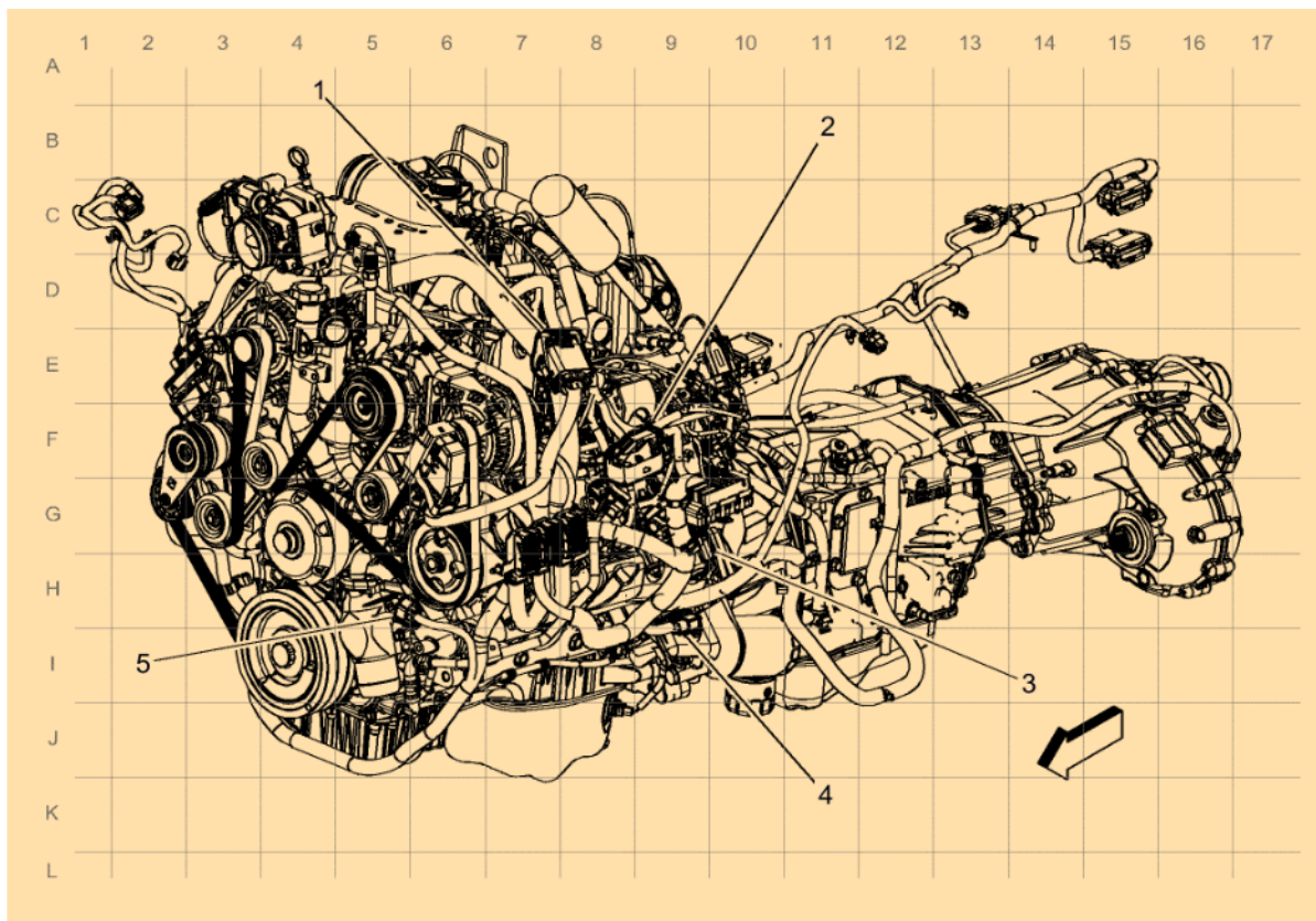
Fig. 9: Left Side of Engine Harness Routing (L5P)
