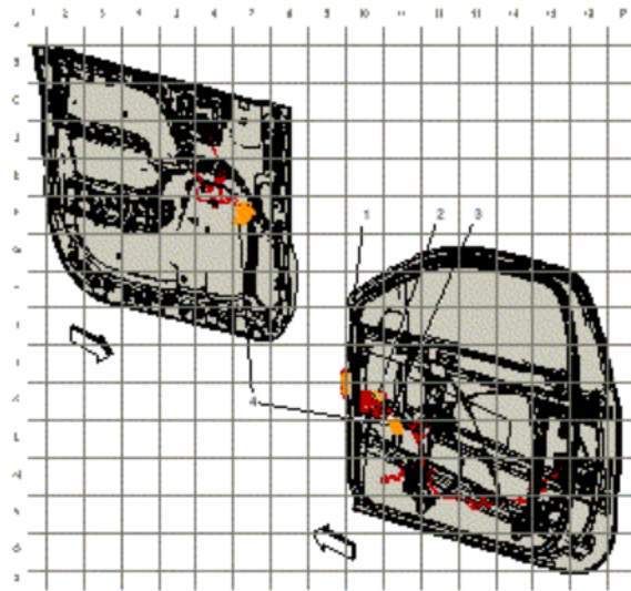
Fig. 20: Passenger Door Harness Routing Courtesy of GENERAL MOTORS COMPANY
