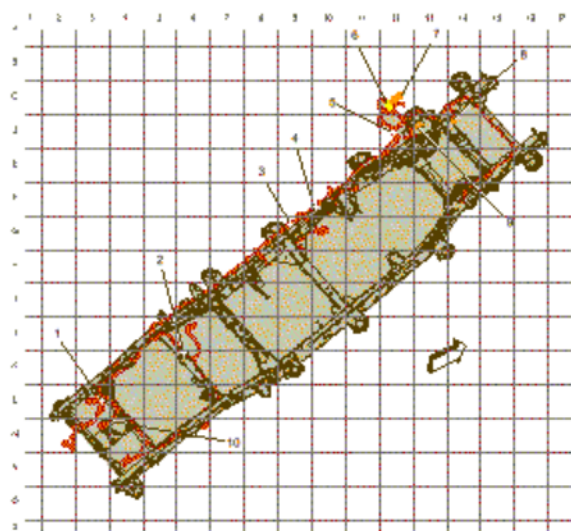
Fig. 25: Chassis Harness Routing Courtesy of GENERAL MOTORS COMPANY
