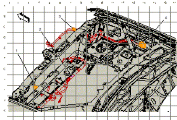
Fig. 3: Forward Lamp Harness Routing - Right Engine Compartment (HP5)
