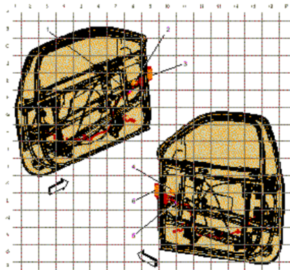
Fig. 18: Doors (Regular Cab with Manual Windows) Harness Routing Courtesy of GENERAL MOTORS COMPANY
