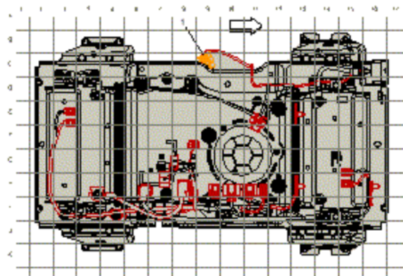
Fig. 15: High Voltage Battery Monitoring Harness Routing (HP5) Courtesy of GENERAL MOTORS COMPANY
