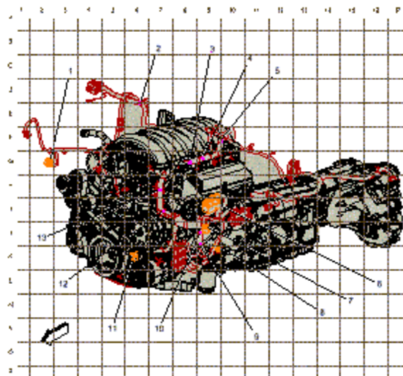
Fig. 6: Engine Harness Routing - Left Front (L8B) Courtesy of GENERAL MOTORS COMPANY
