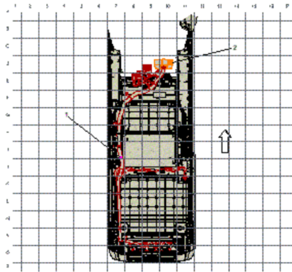
Fig. 14: Floor Console Harness Routing Courtesy of GENERAL MOTORS COMPANY
