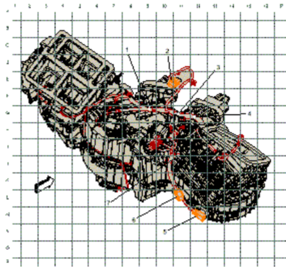
Fig. 11: HVAC Assembly Harness Routing Courtesy of GENERAL MOTORS COMPANY
