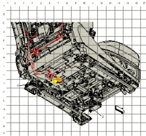
Fig. 17: Back of Passenger Seat Harness Routing Courtesy of GENERAL MOTORS COMPANY
