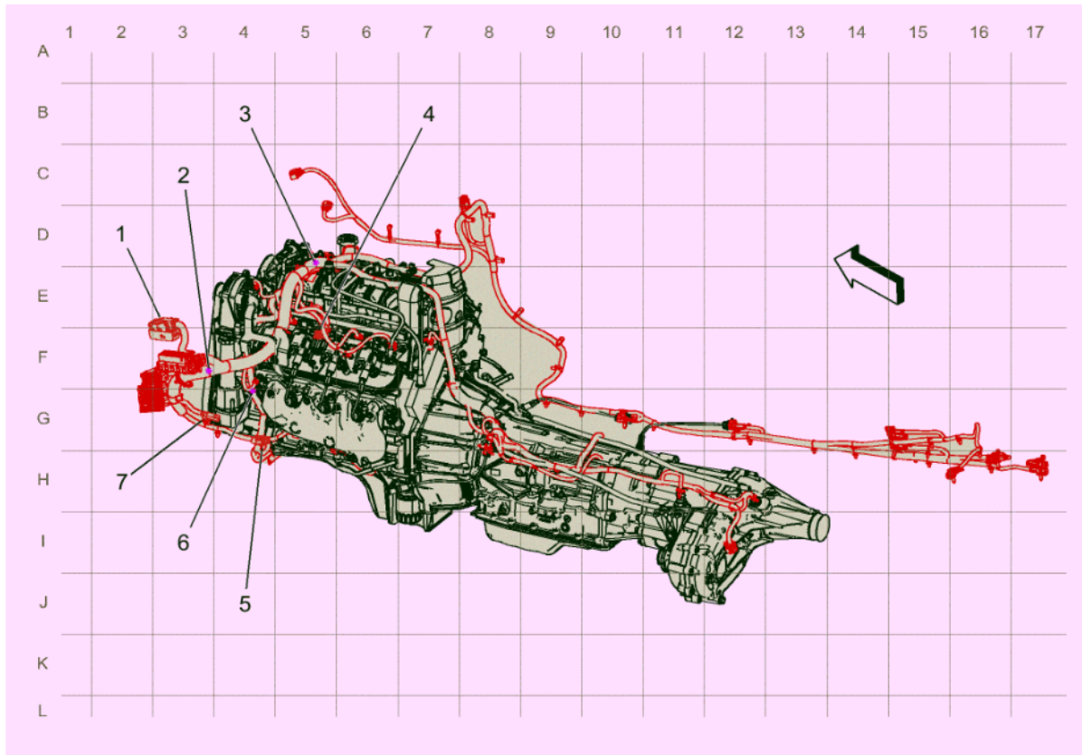
Fig. 8: Left Side of Engine Harness Routing (L96)
