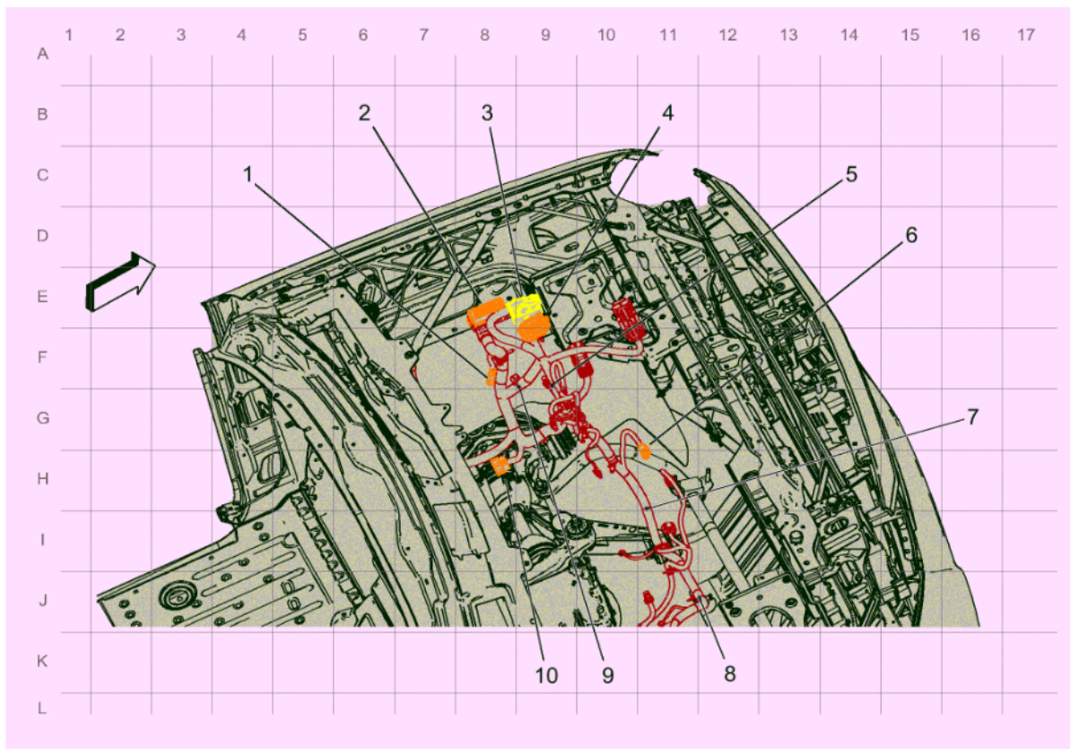
Fig. 4: Engine Compartment Left Harness Routing
