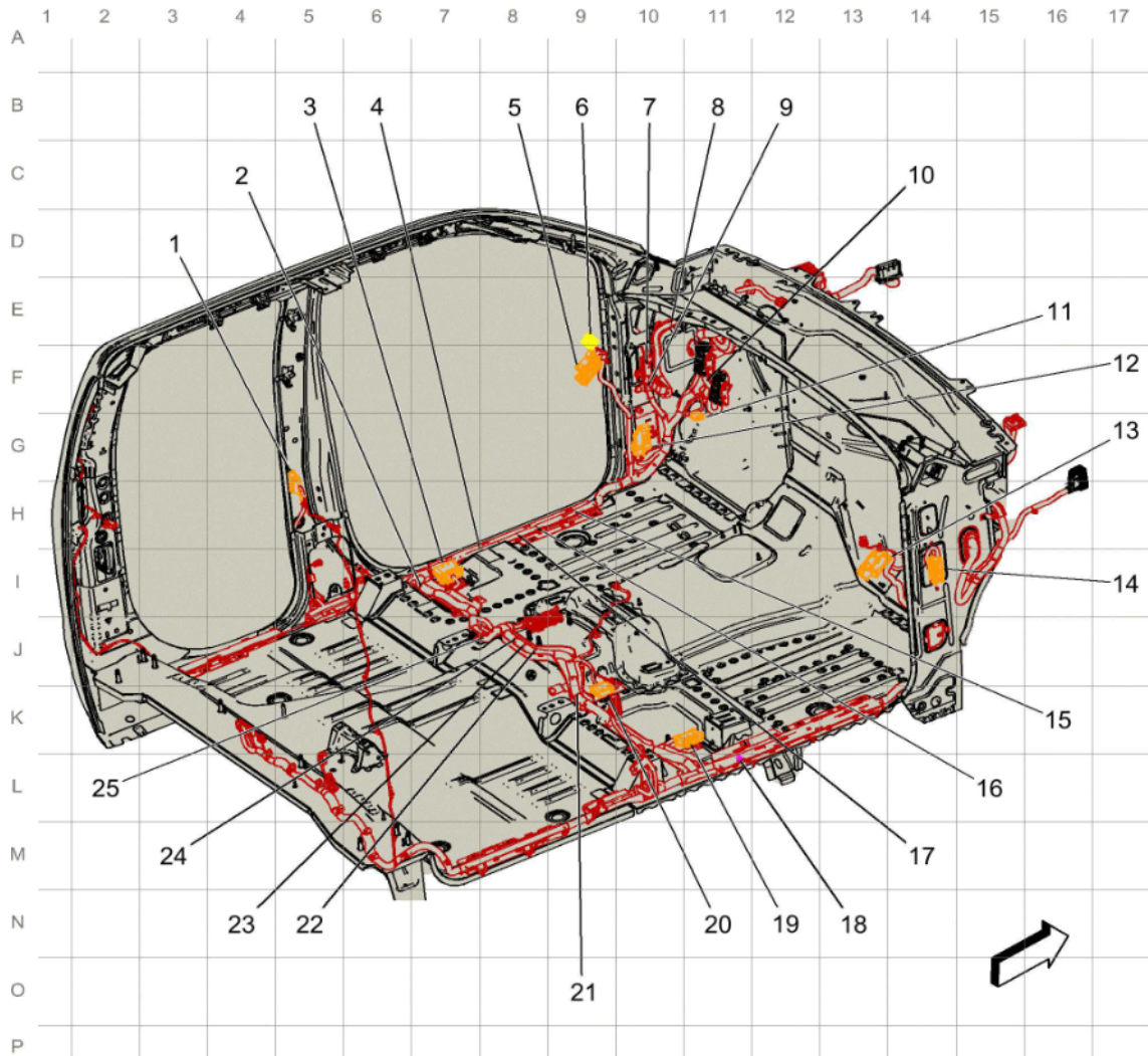
Fig. 22: Passenger Compartment Left Harness Routing
