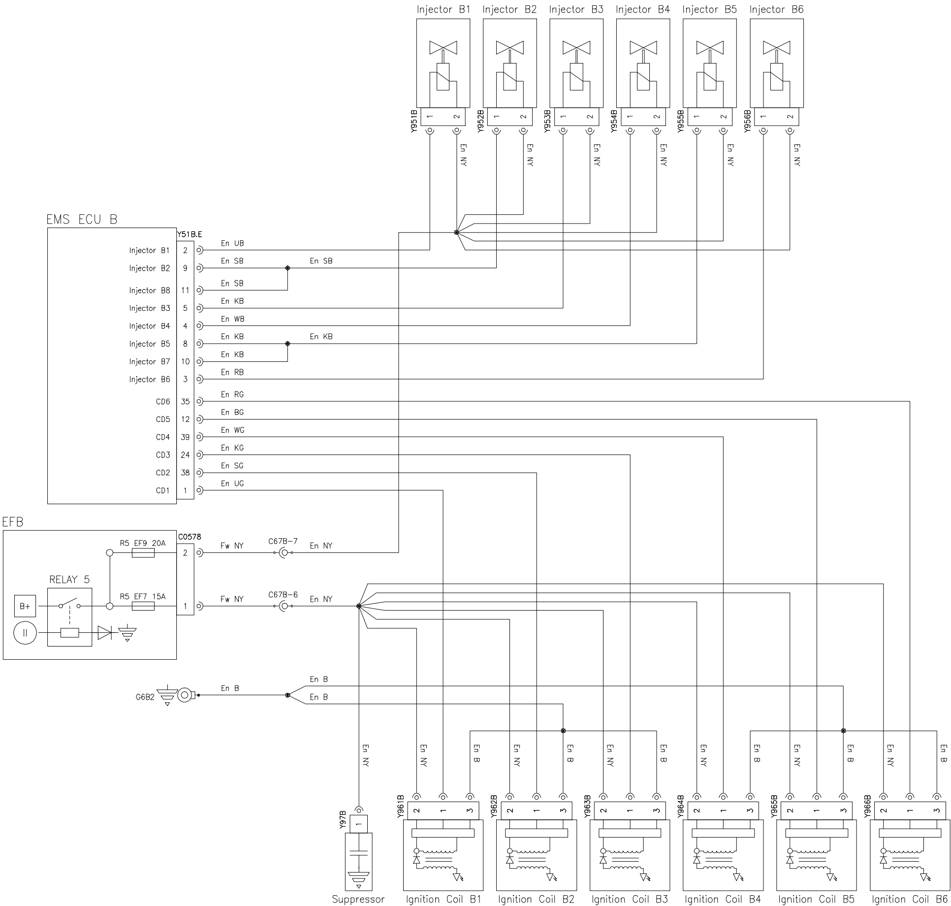
EFB - Enginebay Fusebox
