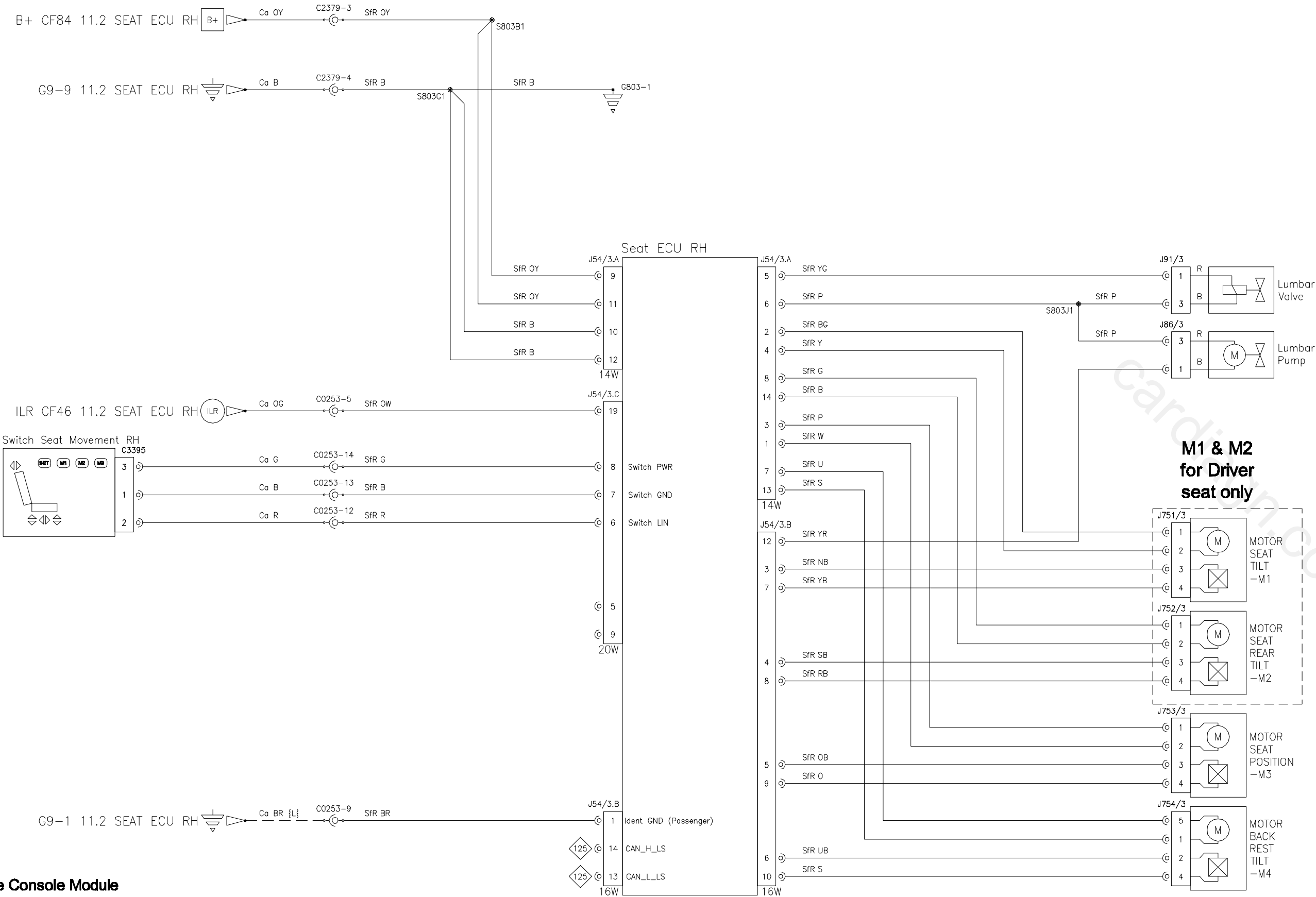
Seat Adjustment Front Right
