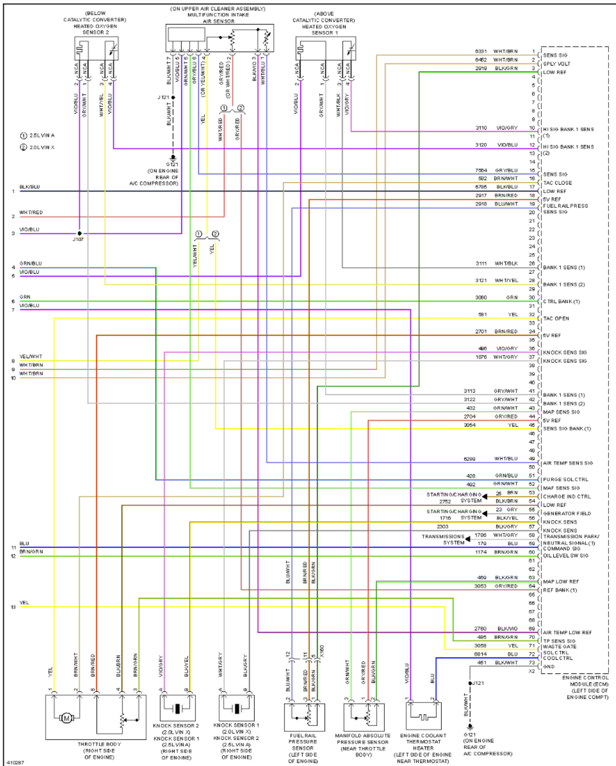
Fig. 34: 2.0L VIN X, Engine Performance Circuit (6 of 6)
