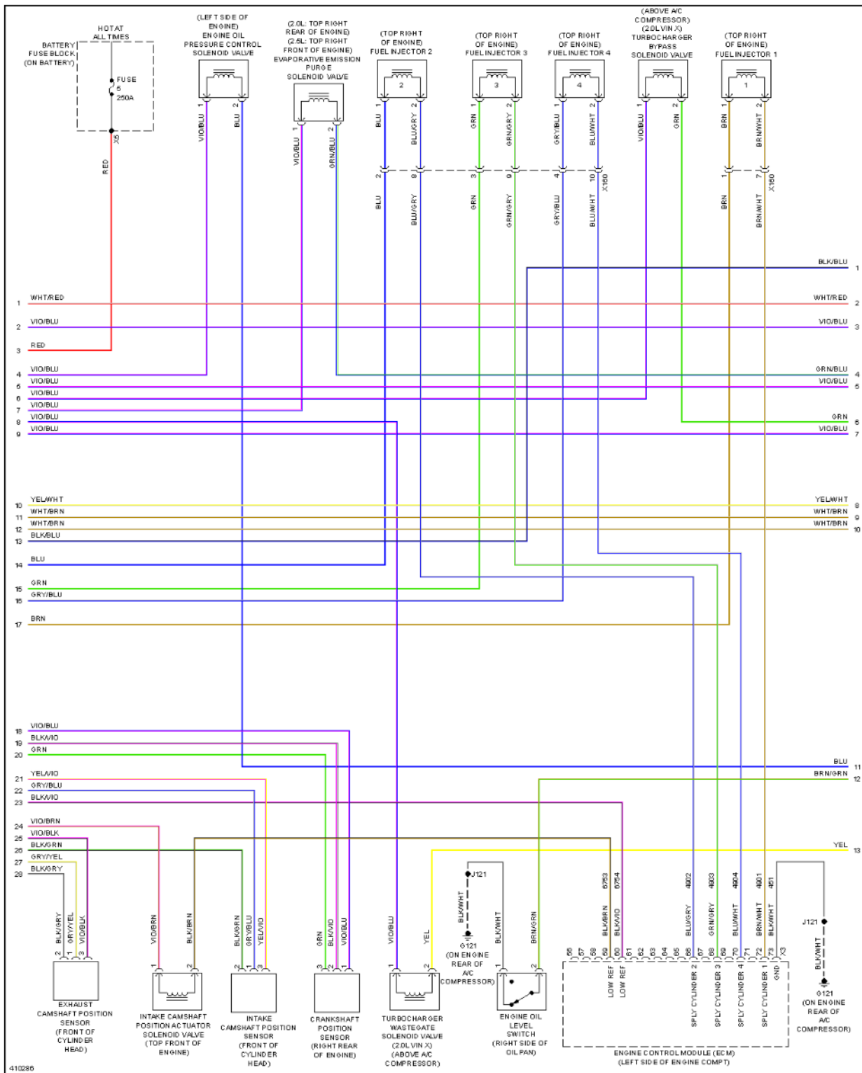
Fig. 33: 2.0L VIN X, Engine Performance Circuit (5 of 6)
