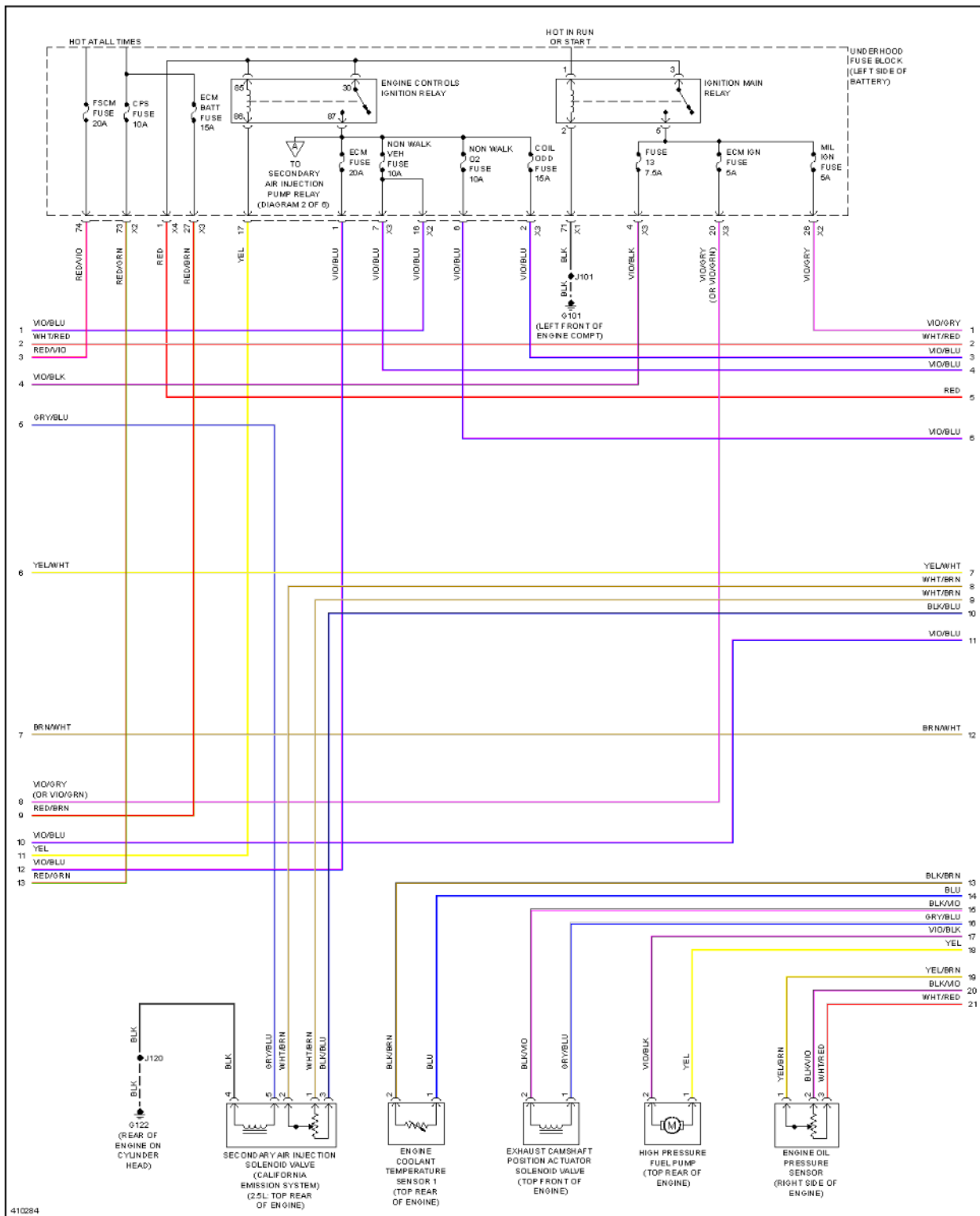
Fig. 31: 2.0L VIN X, Engine Performance Circuit (3 of 6)
