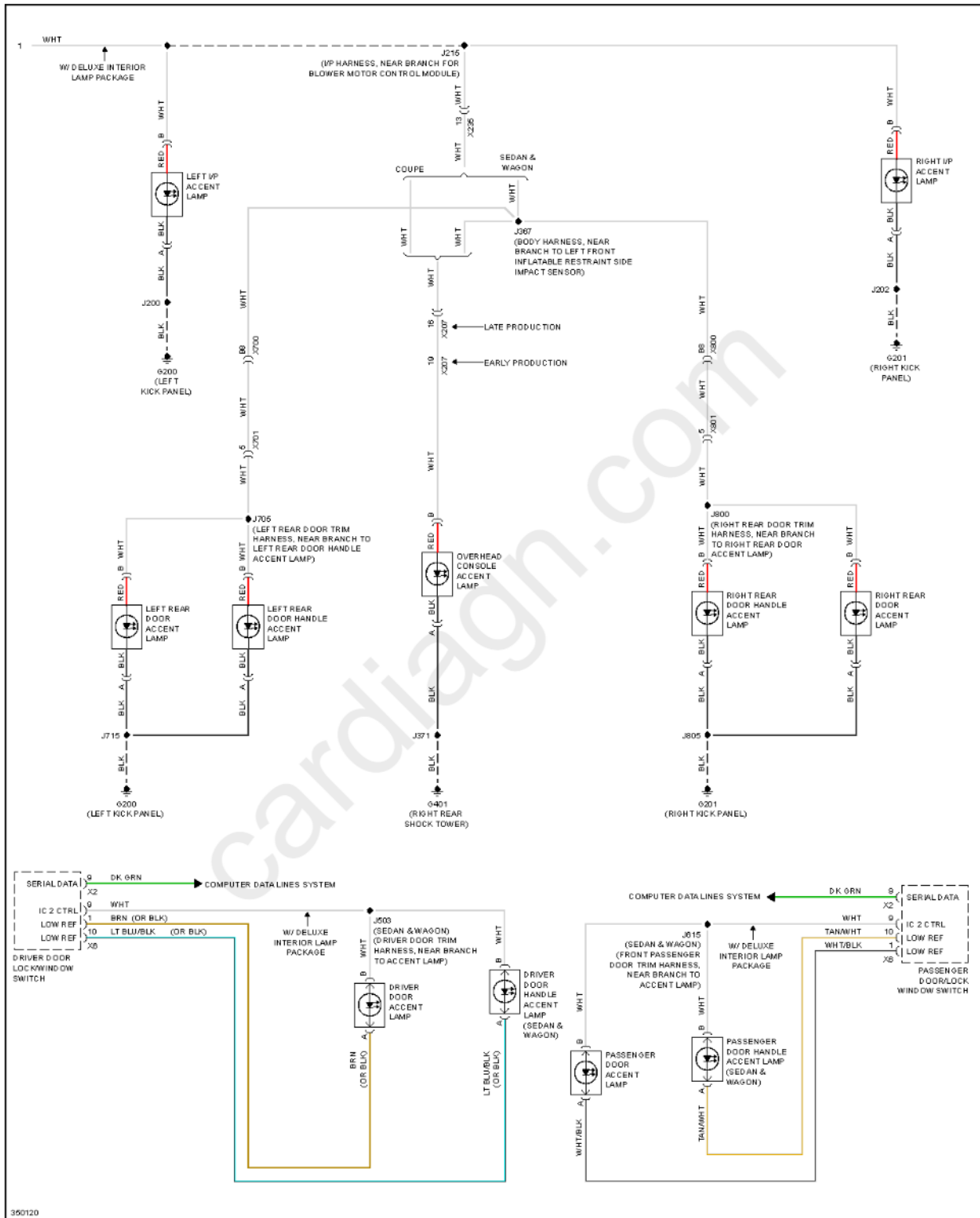
Fig. 57: Courtesy Lamps Circuit (2 of 2)
