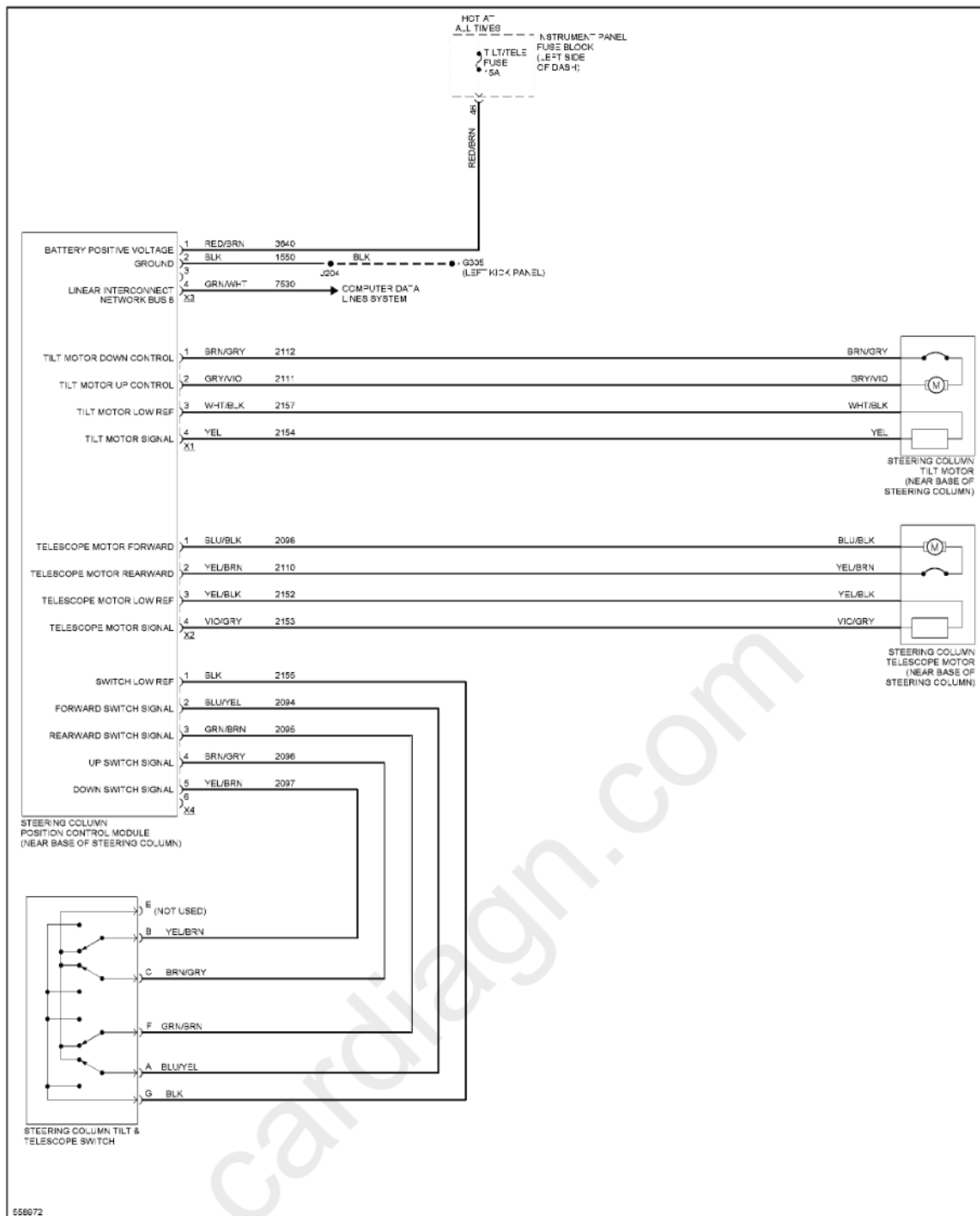
Fig. 34: Power Tilt Steering Column Circuit
