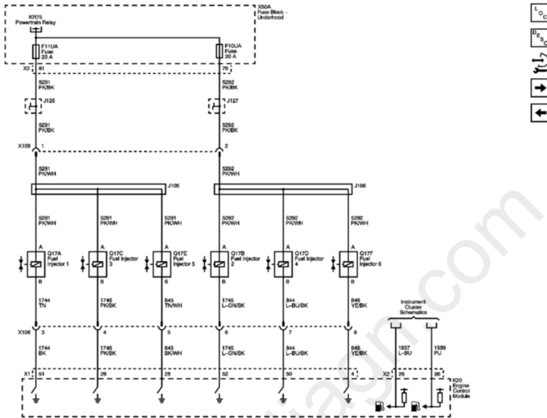
Fig. 11: Fuel Controls Circuit Schematic - Fuel Injectors Courtesy of GENERAL MOTORS CORP.
