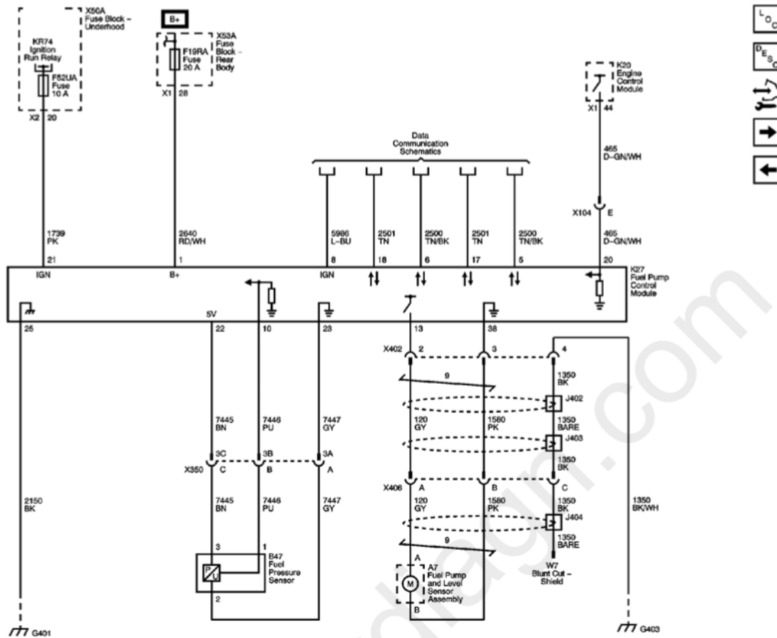
Fig. 24: Fuel Controls - Fuel Pump Flow Control Circuit Schematic Courtesy of GENERAL MOTORS CORP.
