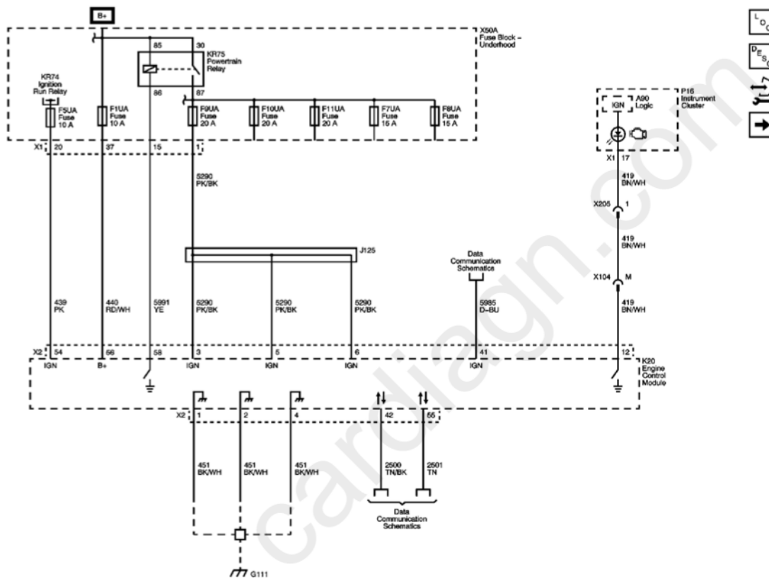
Fig. 1: Power, Ground, DLC & MIL Circuit Schematic Courtesy of GENERAL MOTORS CORP.
