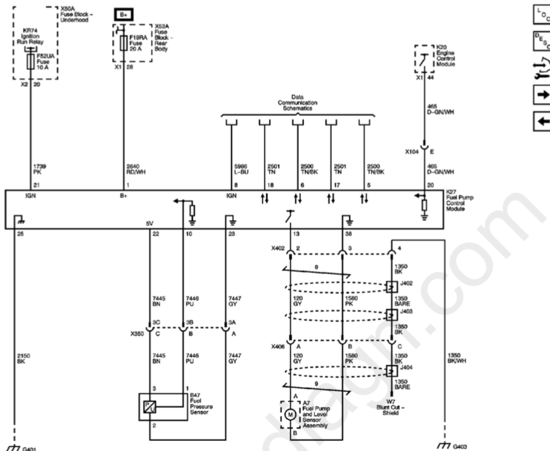
Fig. 12: Fuel Controls Circuit Schematic - Fuel Pump Flow Controls Courtesy of GENERAL MOTORS CORP.
