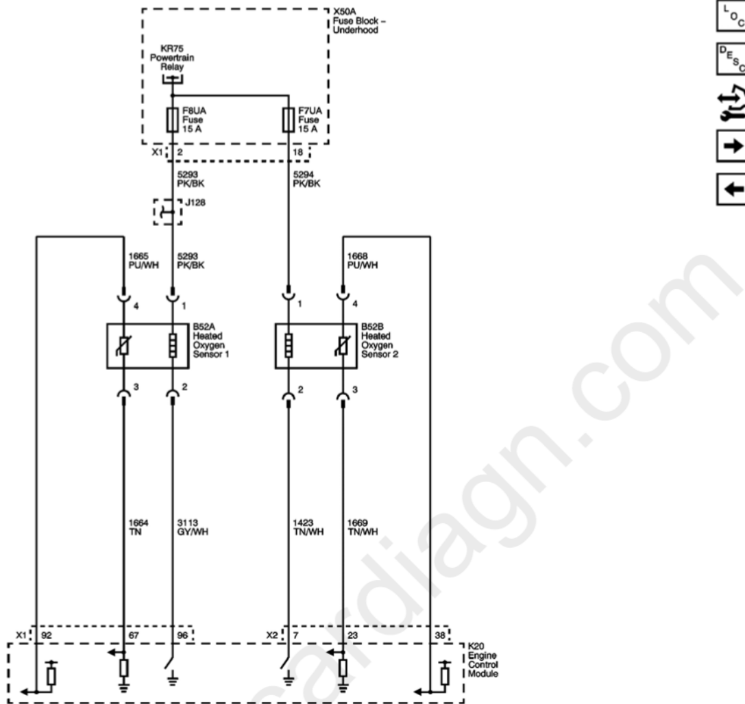
Fig. 6: Engine Data Sensors Circuit Schematic - HO2S Courtesy of GENERAL MOTORS CORP.
