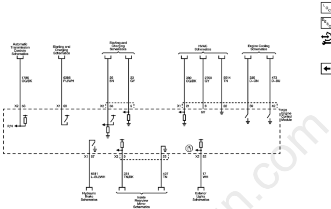
Fig. 26: Controlled/Monitored Subsystem References Circuit Schematic Courtesy of GENERAL MOTORS CORP.
