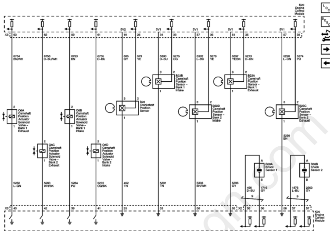
Fig. 22: Ignition Controls - CKP, CMP, KS Sensors & CMP Actuator Solenoids Circuit Schematic Courtesy of GENERAL MOTORS CORP.
