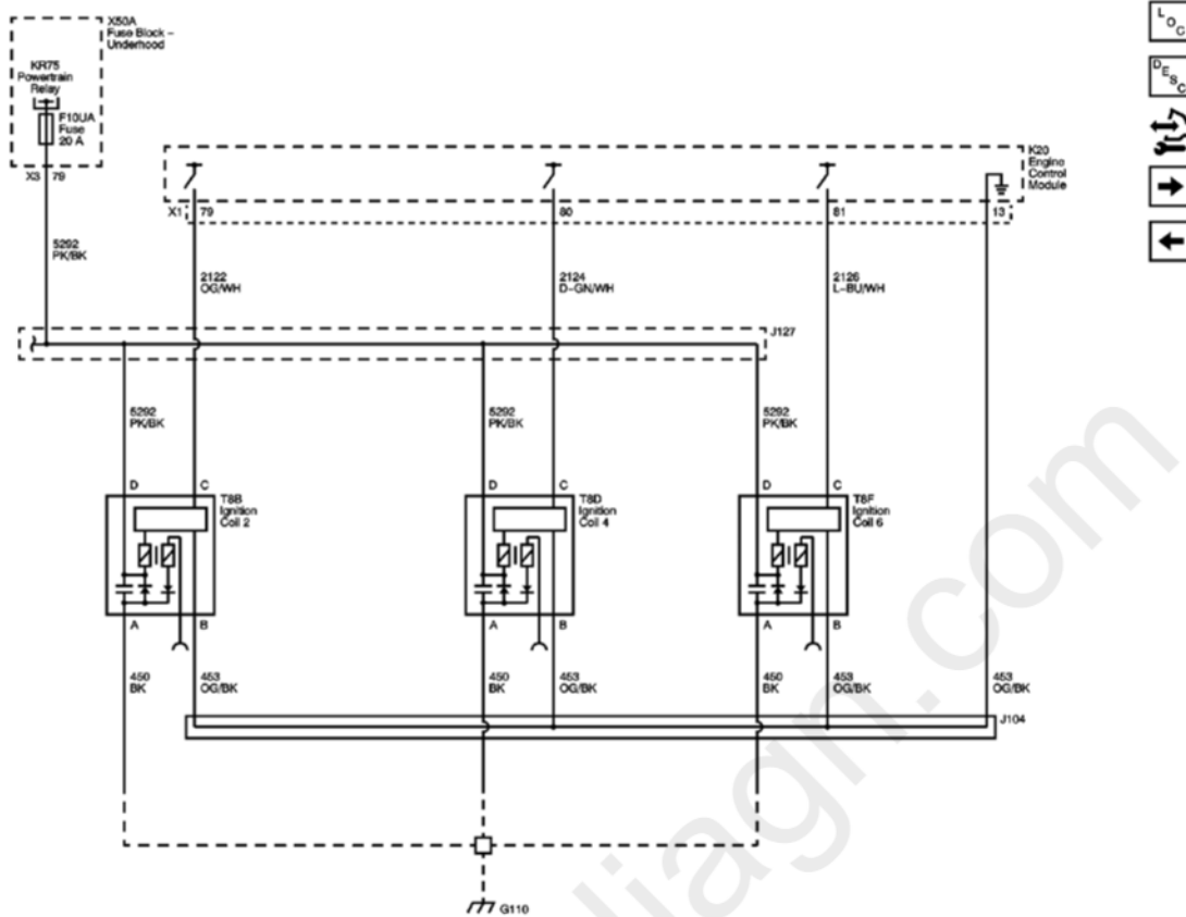
Fig. 8: Ignition Controls Circuit Schematic - Ignition Coils Bank 2 Courtesy of GENERAL MOTORS CORP.
