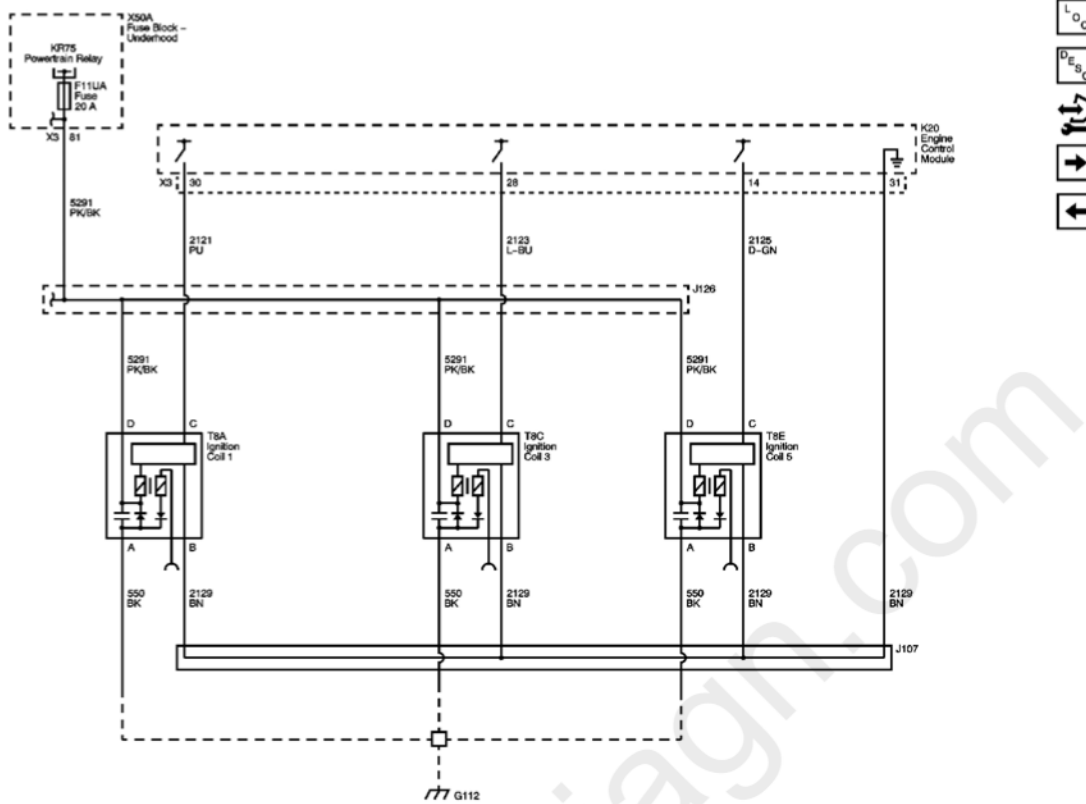
Fig. 20: Ignition Controls Circuit Schematic - Ignition Coils Bank 1 Courtesy of GENERAL MOTORS CORP.
