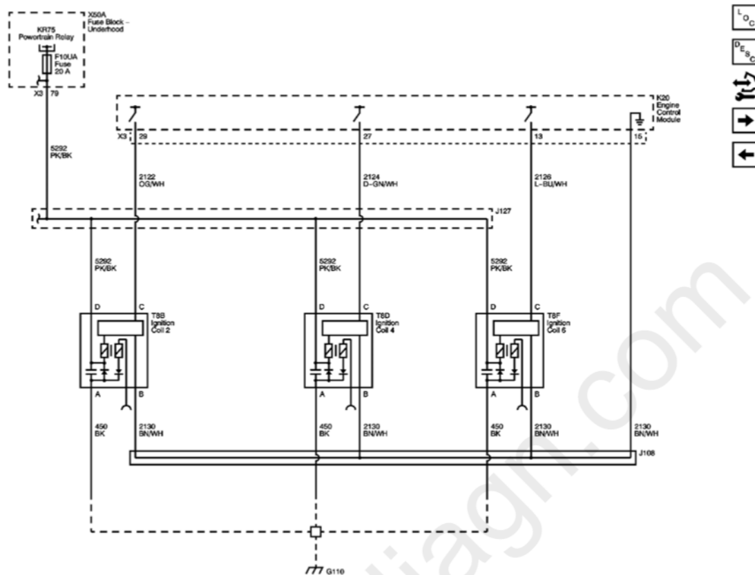
Fig. 21: Ignition Controls Circuit Schematic - Ignition Coils Bank 2 Courtesy of GENERAL MOTORS CORP.
