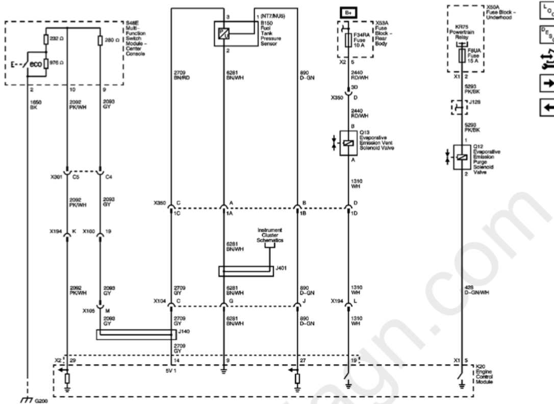
Fig. 13: Fuel Controls Circuit Schematic - EVAP and Fuel Economy Controls Courtesy of GENERAL MOTORS CORP.
