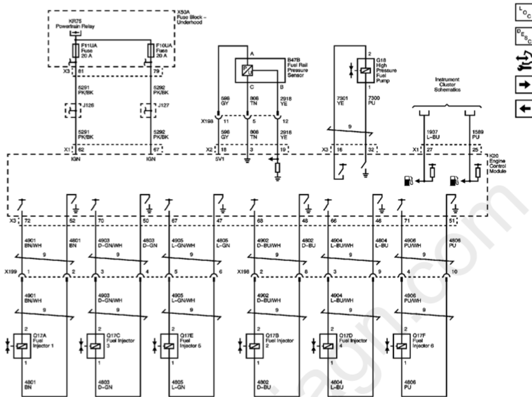
Fig. 23: Fuel Controls - Fuel Injectors Circuit Schematic Courtesy of GENERAL MOTORS CORP.
