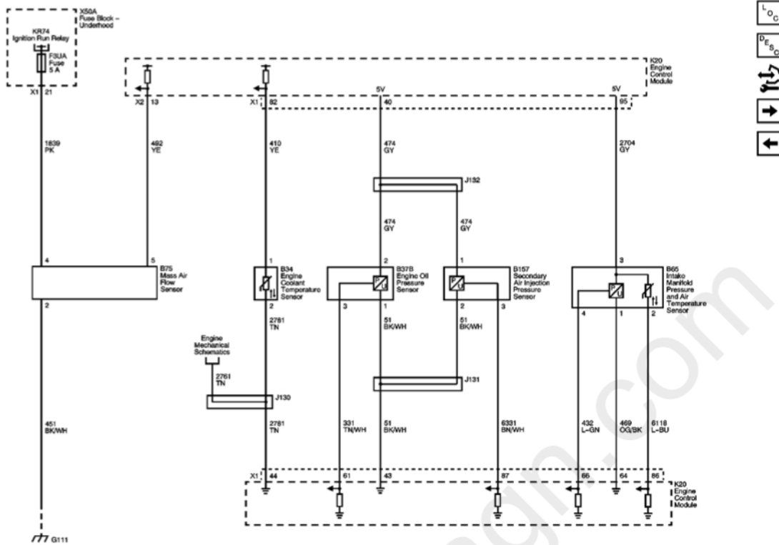
Fig. : Engine Data Sensors Circuit Schematic - Pressure & Temperature Courtesy of GENERAL MOTORS CORP.
