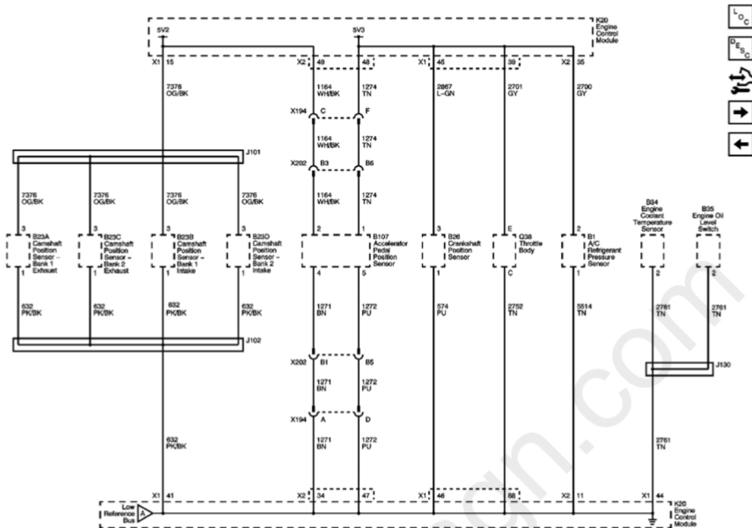
Fig. : 2, & Lo Reference Bus Circuit Schematic Courtesy of GENERAL MOTORS CORP.
