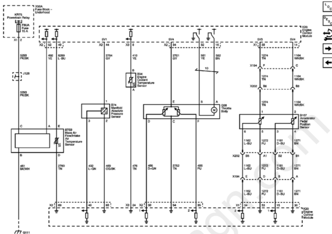
Fig. 18: Engine Data Sensors - Pressure, Temperature & Throttle Controls Circuit Schematic Courtesy of GENERAL MOTORS CORP.
