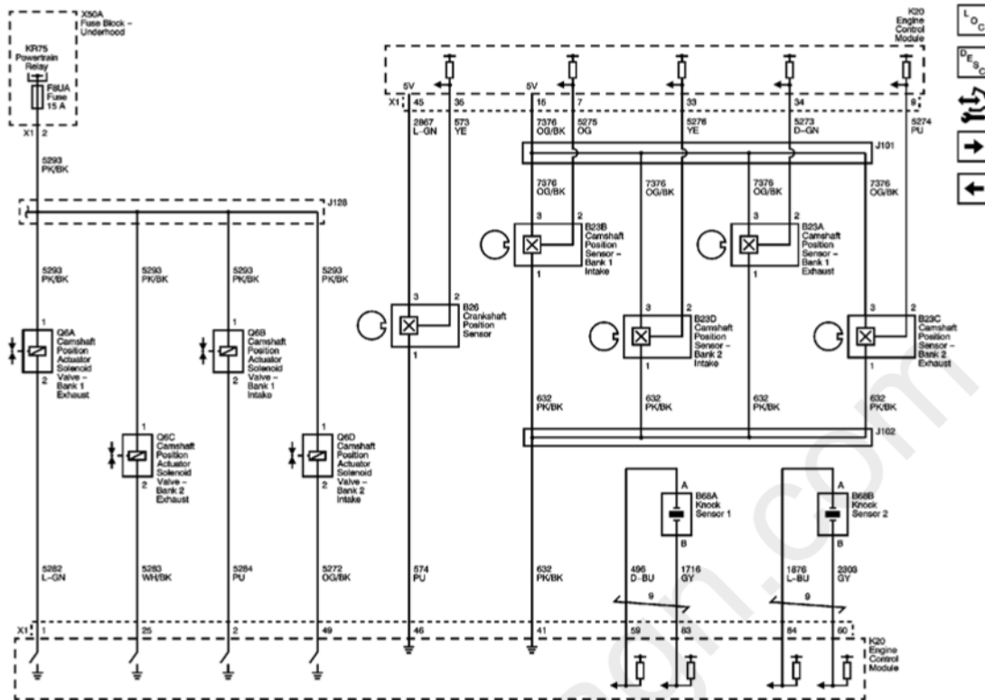
Fig. 9: Ignition Controls Circuit Schematic - CKP, CMP, KS Sensors & CMP Actuator Solenoids Courtesy of GENERAL MOTORS CORP.
