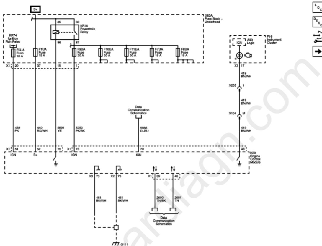
Fig. 15: Power, Ground , Serial Data & MIL Circuit Schematic Courtesy of GENERAL MOTORS CORP.
