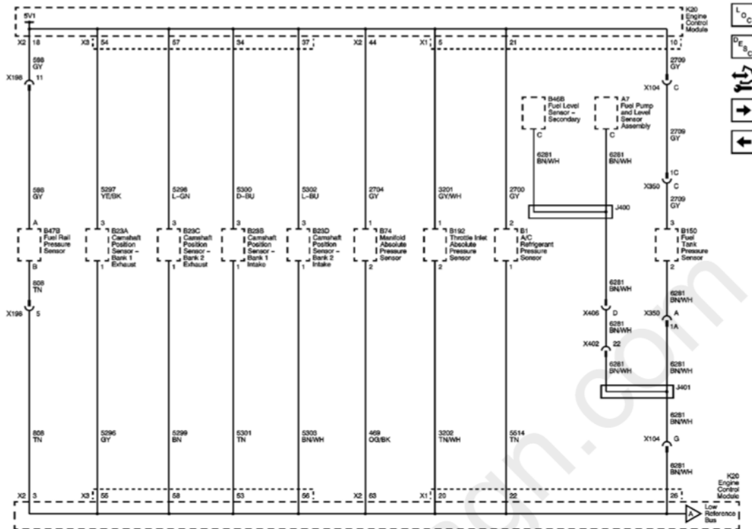
Fig. 1 : 5V1 & Low Reference Bus Circuit Schematic Courtesy of GENERAL MOTORS CORP.
