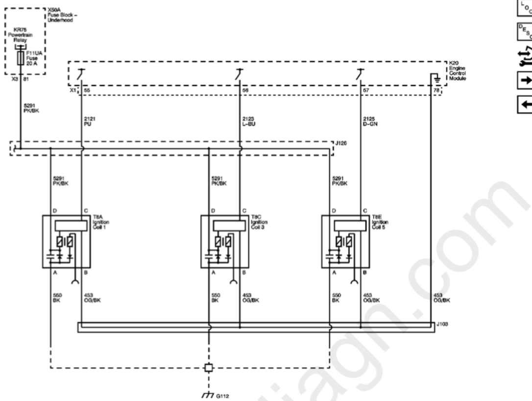
Fig. 7: Ignition Controls Circuit Schematic - Ignition Coils Bank 1 Courtesy of GENERAL MOTORS CORP.
