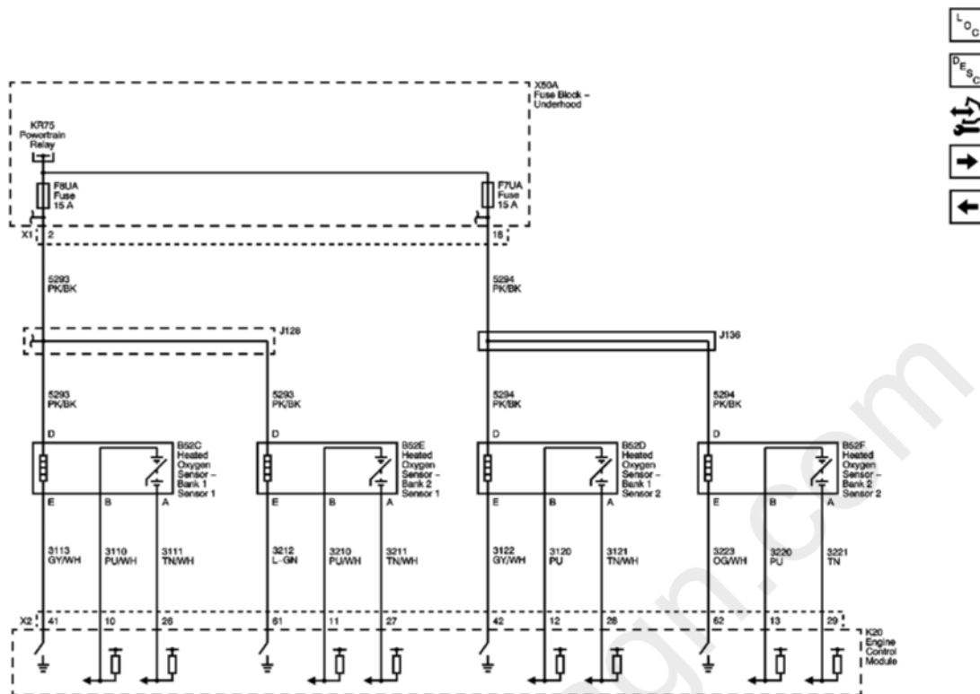
Fig. 19: Engine Data Sensors Circuit Schematic - HO2S Courtesy of GENERAL MOTORS CORP.
