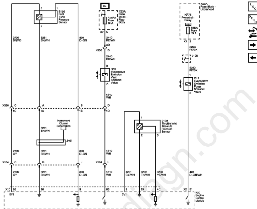
Fig. 25: Fuel Controls - EVAP Controls Circuit Schematic Courtesy of GENERAL MOTORS CORP.
