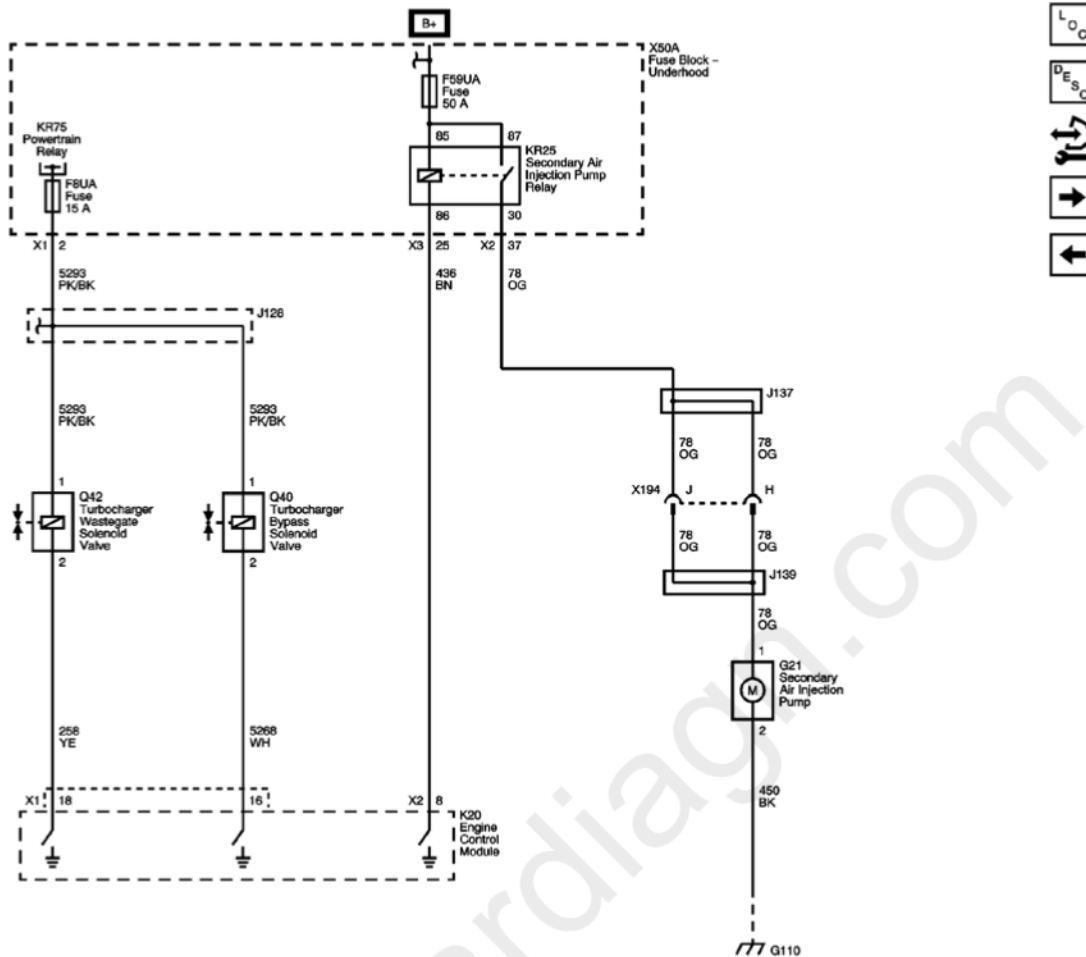
Fig. 10: Turbocharger Controls & Secondary Air Injection (AIR) Pump Circuit Schematic Courtesy of GENERAL MOTORS CORP.
