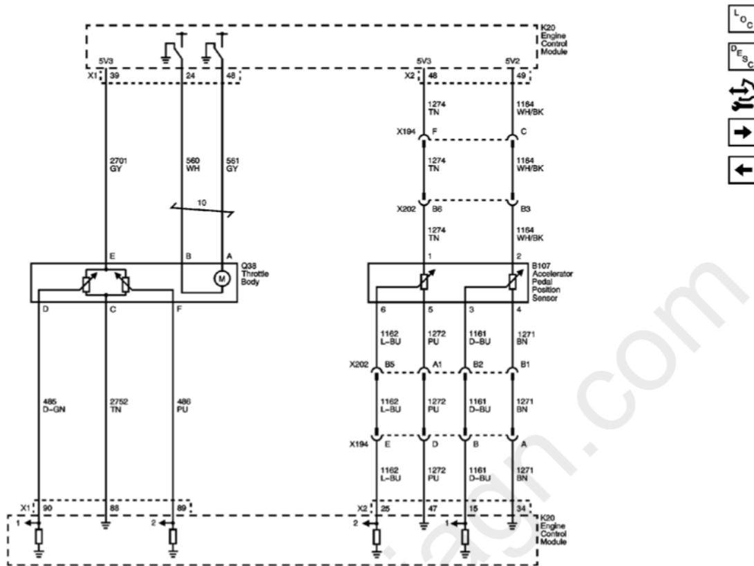
Fig. : Engine Data Sensors Circuit Schematic - Throttle Controls Courtesy of GENERAL MOTORS CORP.
