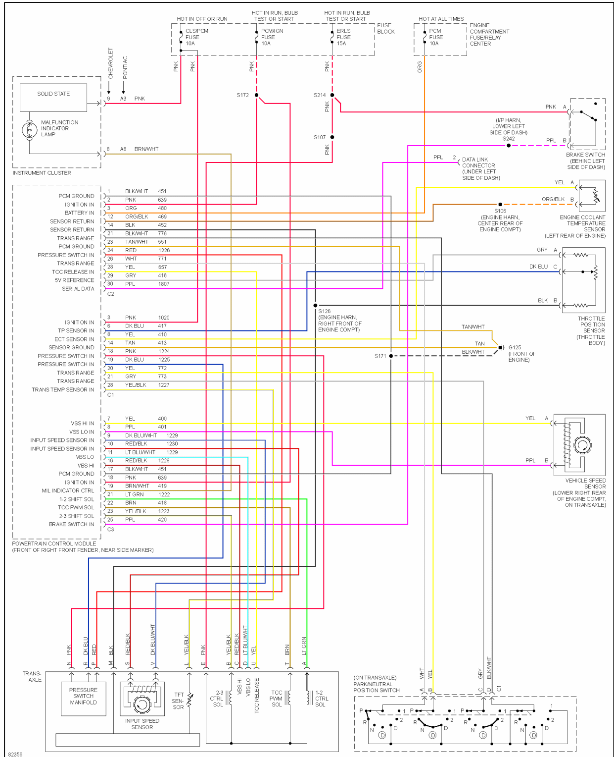
Fig. 44: 2.3L (VIN D), Transmission Circuit
