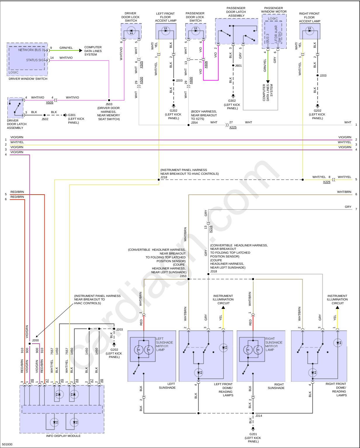
Fig 2: Courtesy Lamps Circuit (2 of 3)
