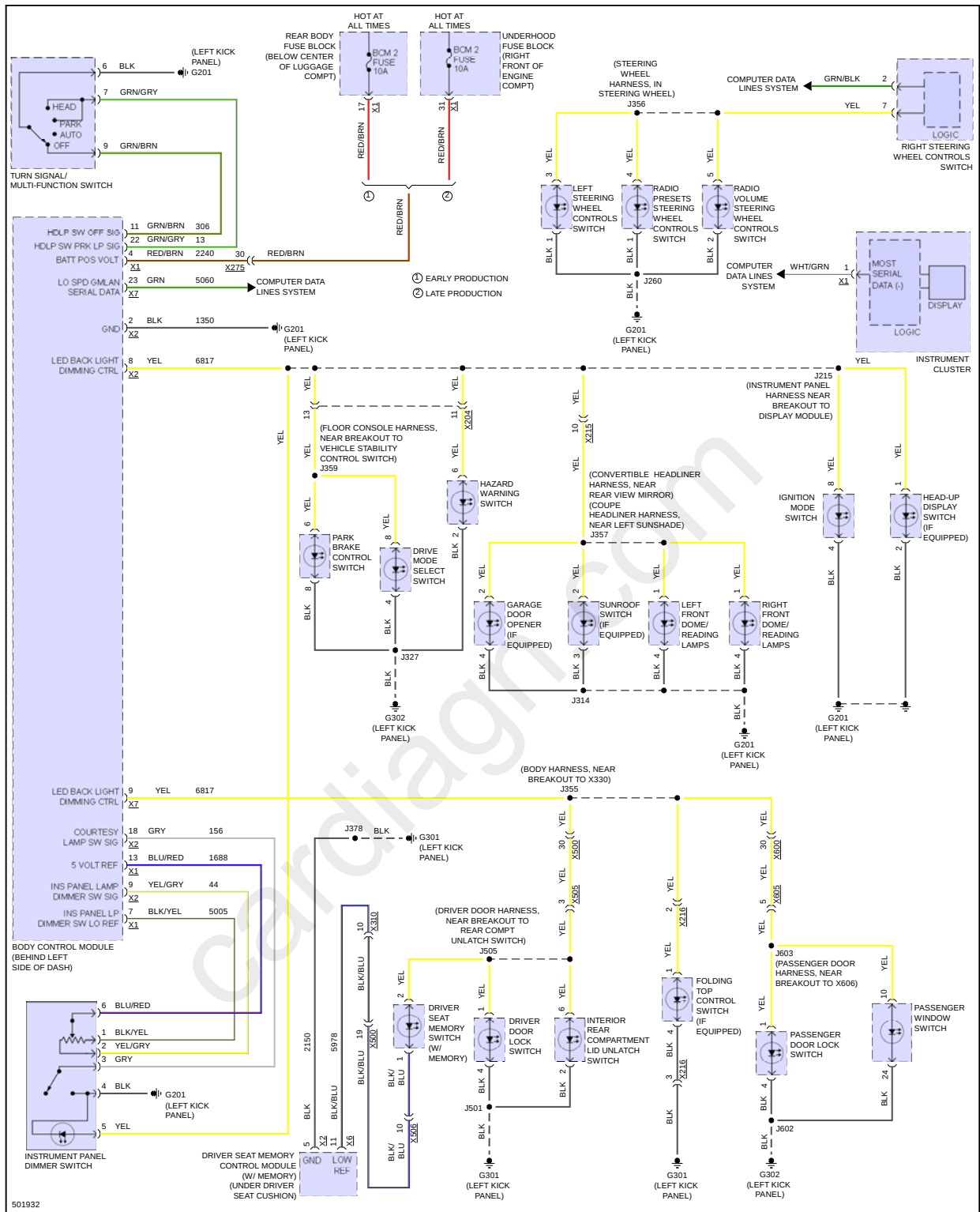
Fig 4: Instrument Illumination Circuit
