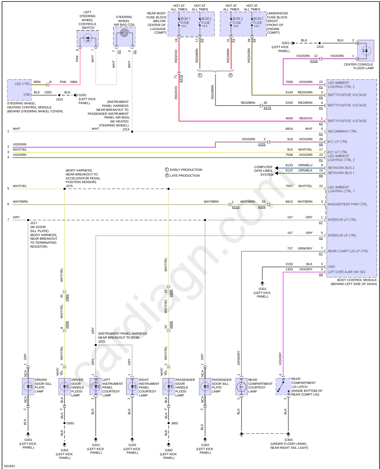
Fig 3: Courtesy Lamps Circuit (3 of 3)
