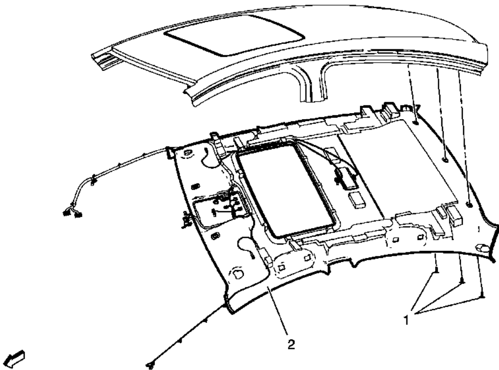
Fig. 10: Headlining Trim Panel (With Sunroof)
