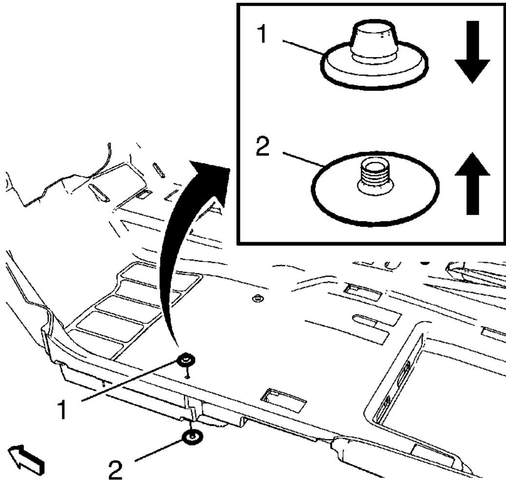
Fig. 4: Floor Carpet Retainer
