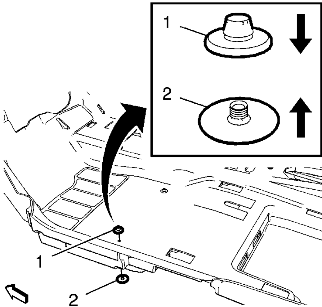
Fig. 5: Floor Carpet Retainer
