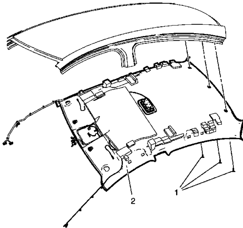
Fig. 9: Headlining Trim Panel (Without Sunroof)
