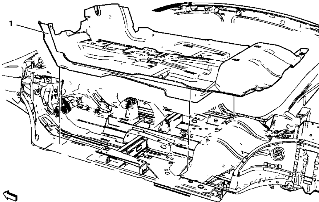
Fig. 1: View Of Front Floor Panel Carpet Assembly Courtesy of GENERAL MOTORS COMPANY
