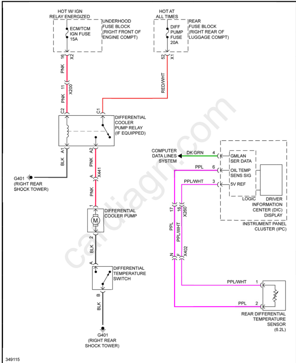
Fig. 117: Rear Differential Cooler Circuit
