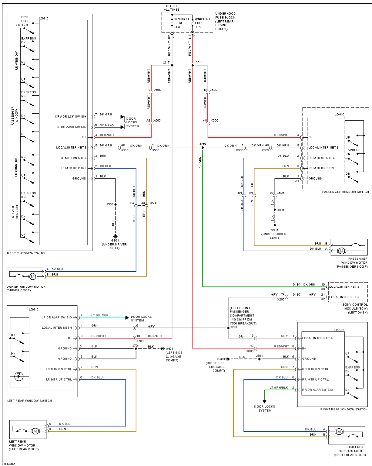
Fig. 64: Power Windows Circuit
