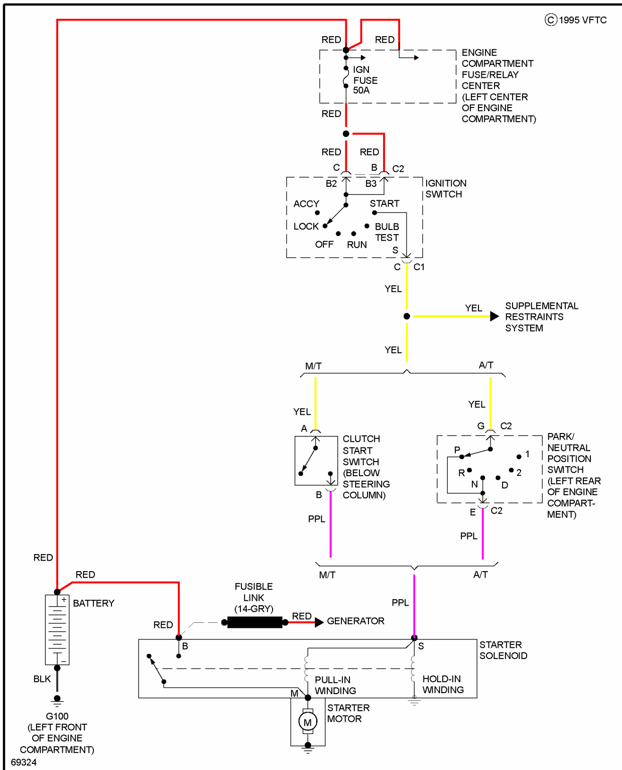
Fig. 41: Starting Circuit
