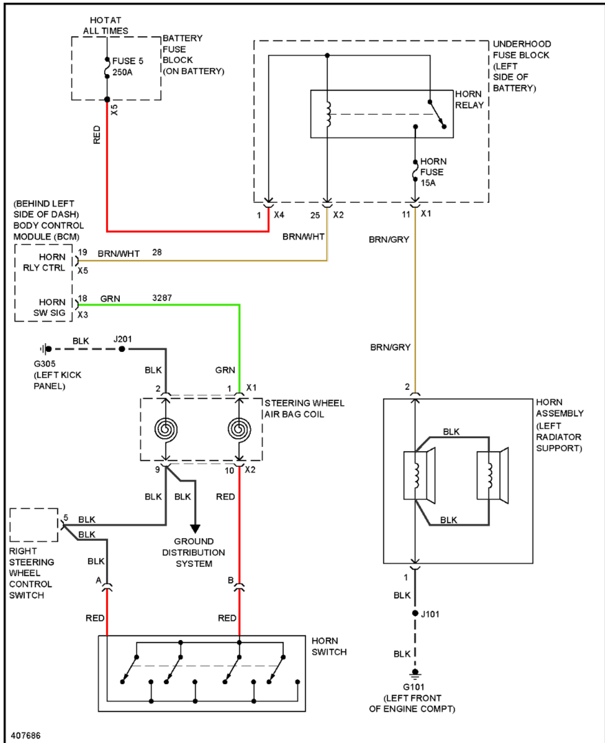
Fig. 65: Horn Circuit
