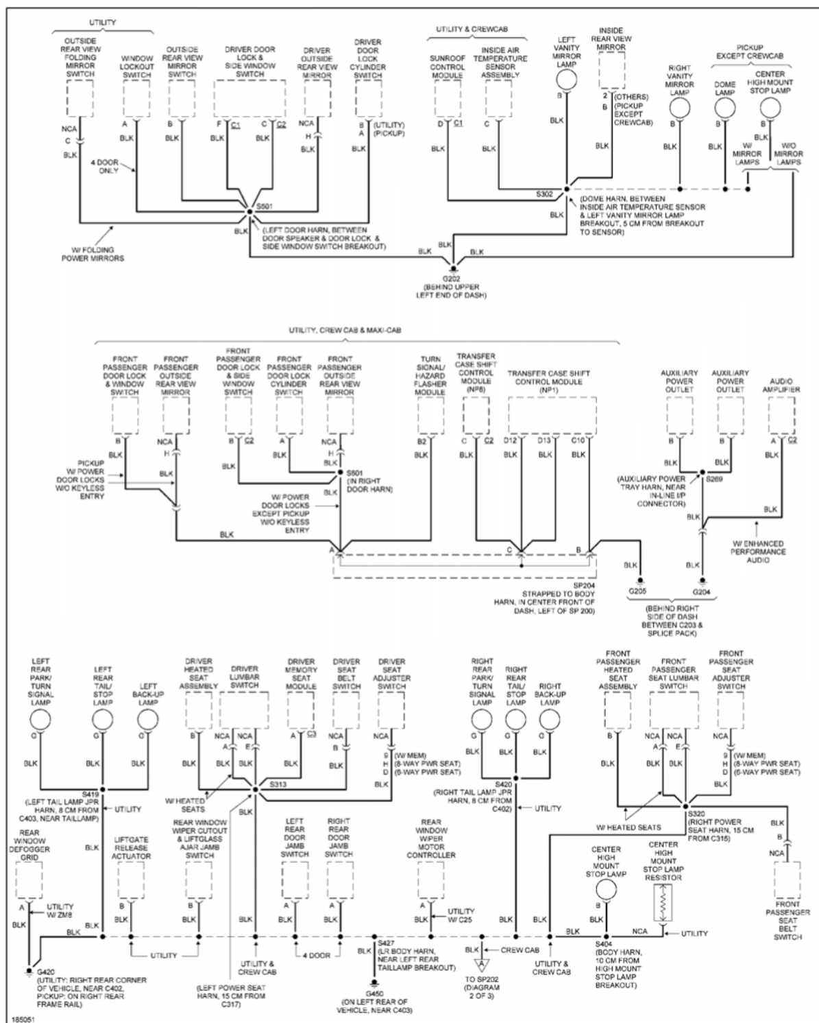
Fig. 18: Ground Distribution Circuit (3 of 3)
