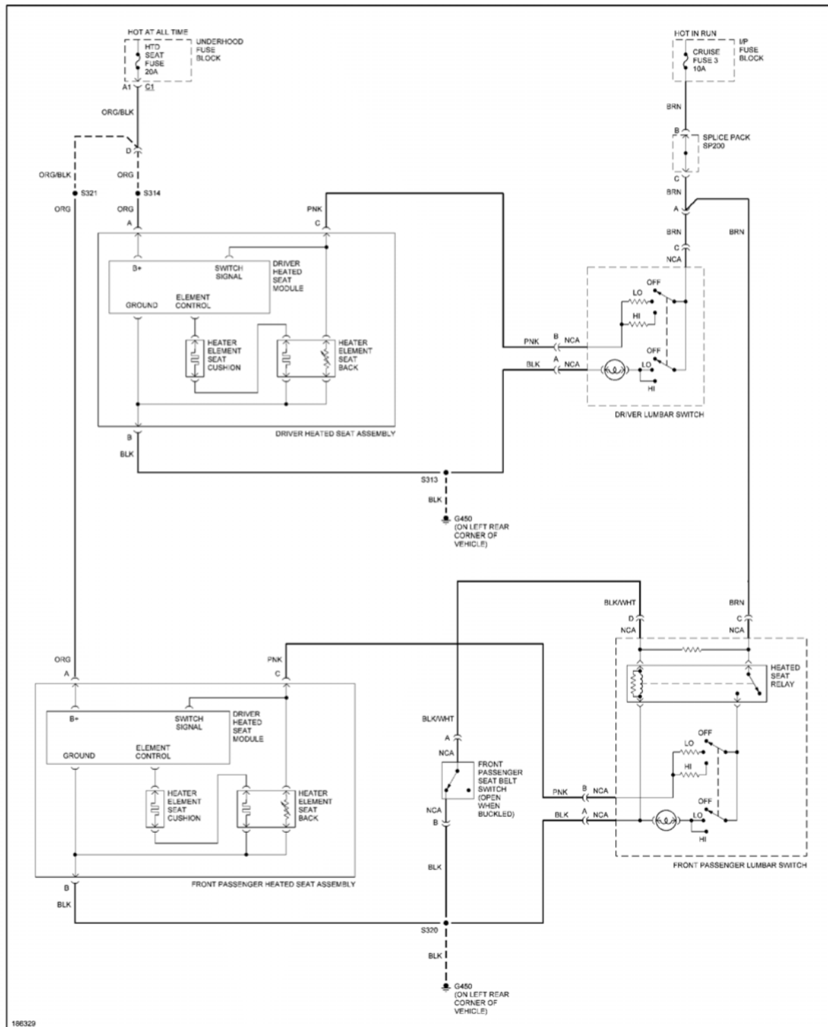
Fig. 38: Heated Seats Circuit
