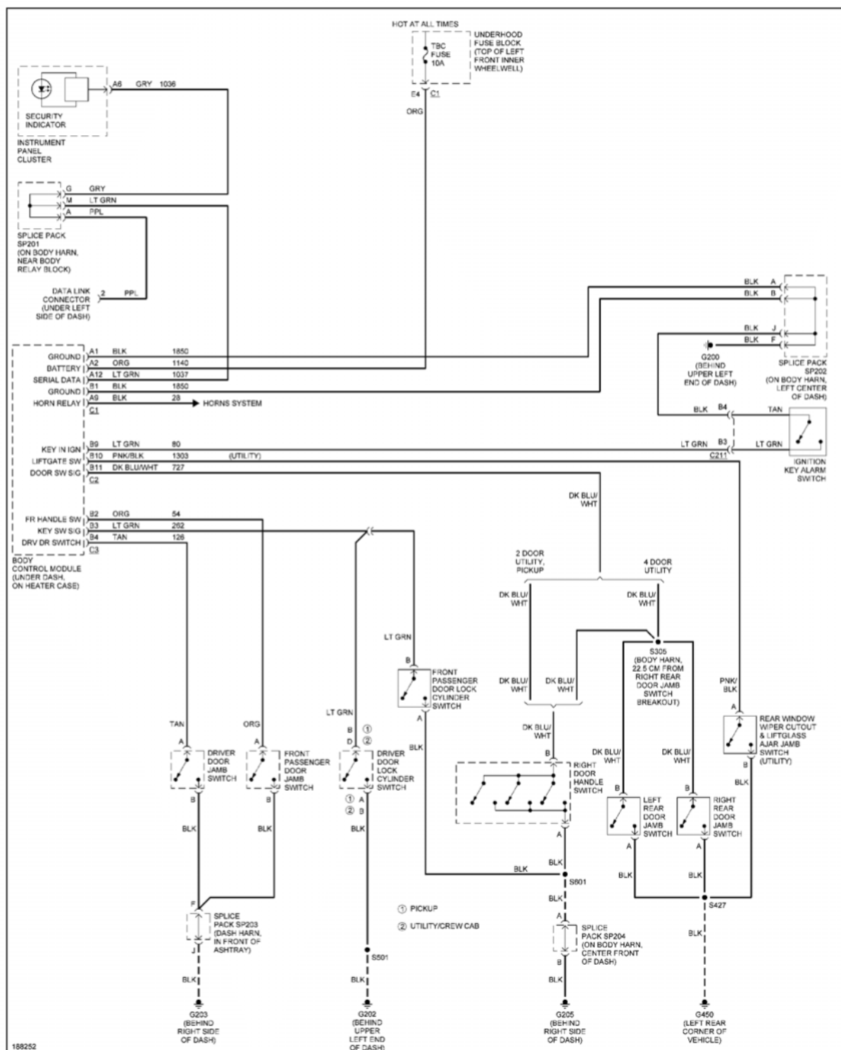
Fig. 4: Forced Entry Circuit
