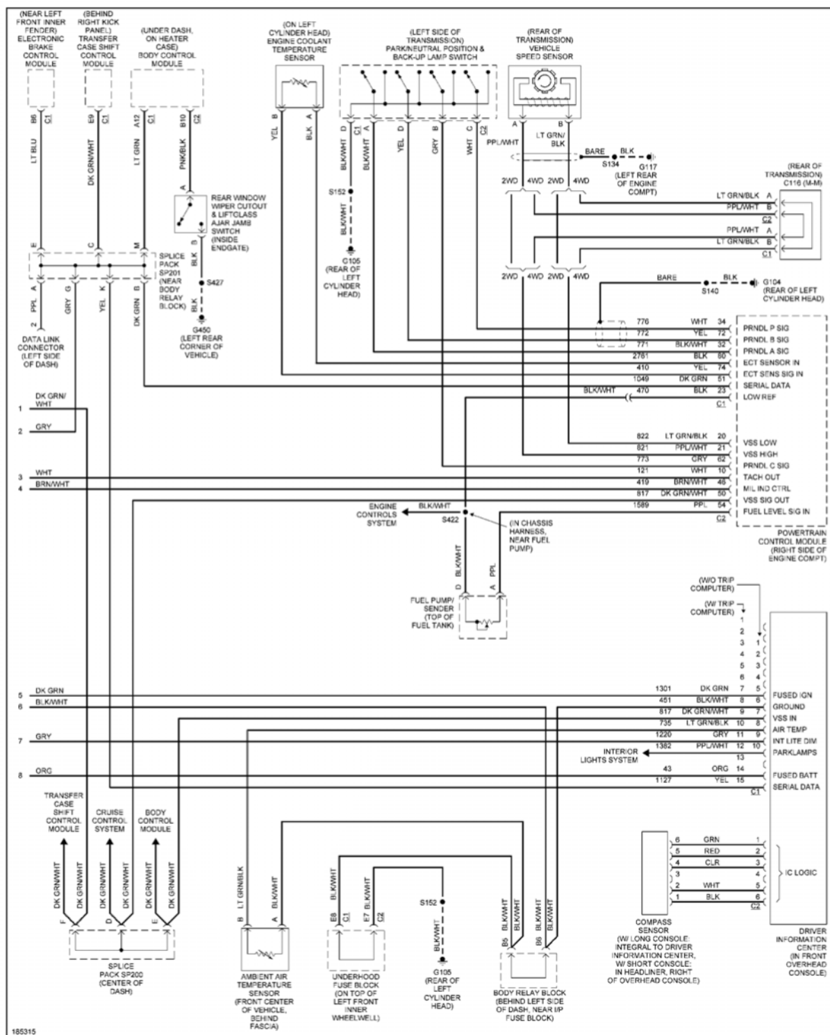
Fig. 23: Instrument Cluster Circuit (2 of 2)
