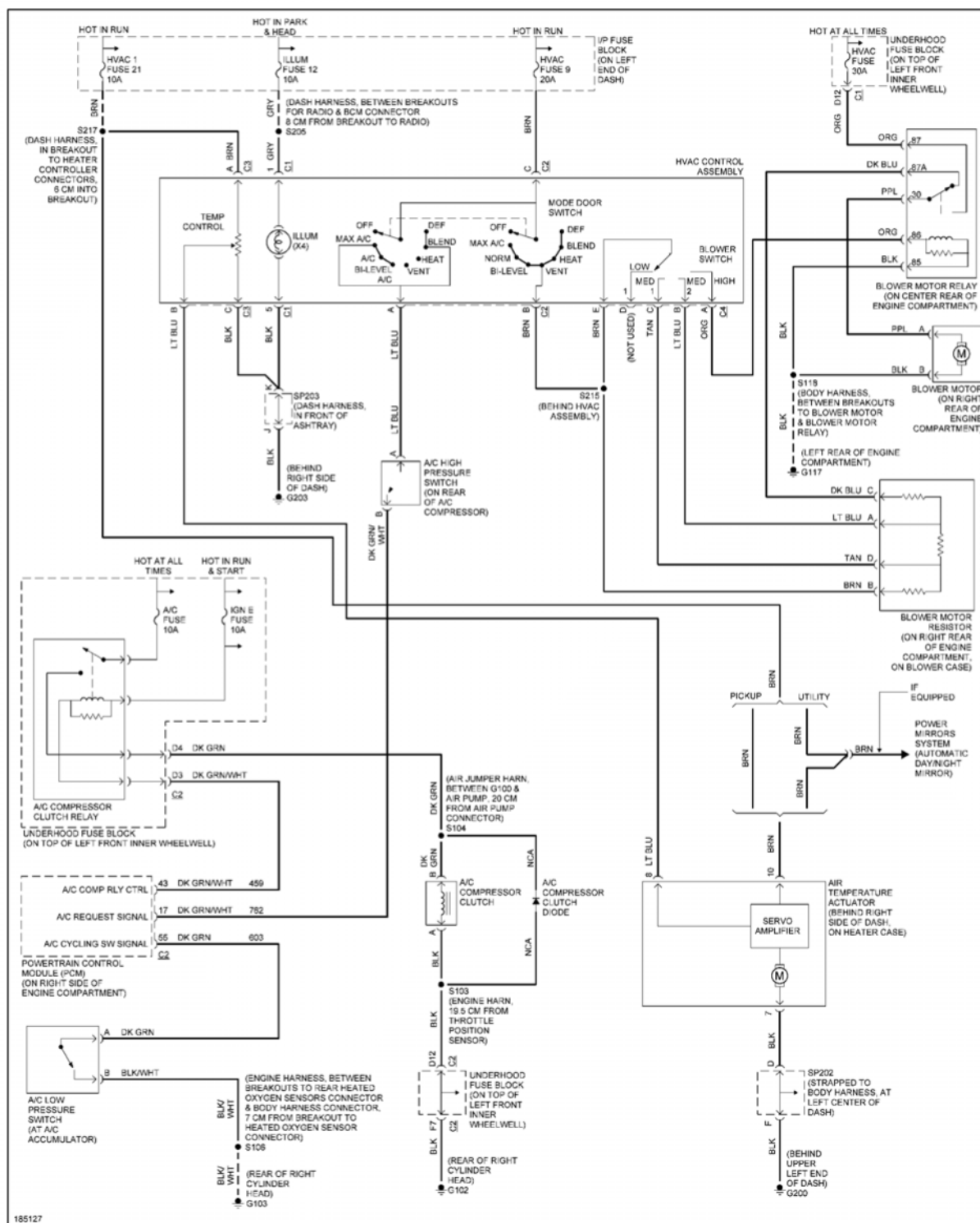
Fig. 2: Manual A/C Circuit
