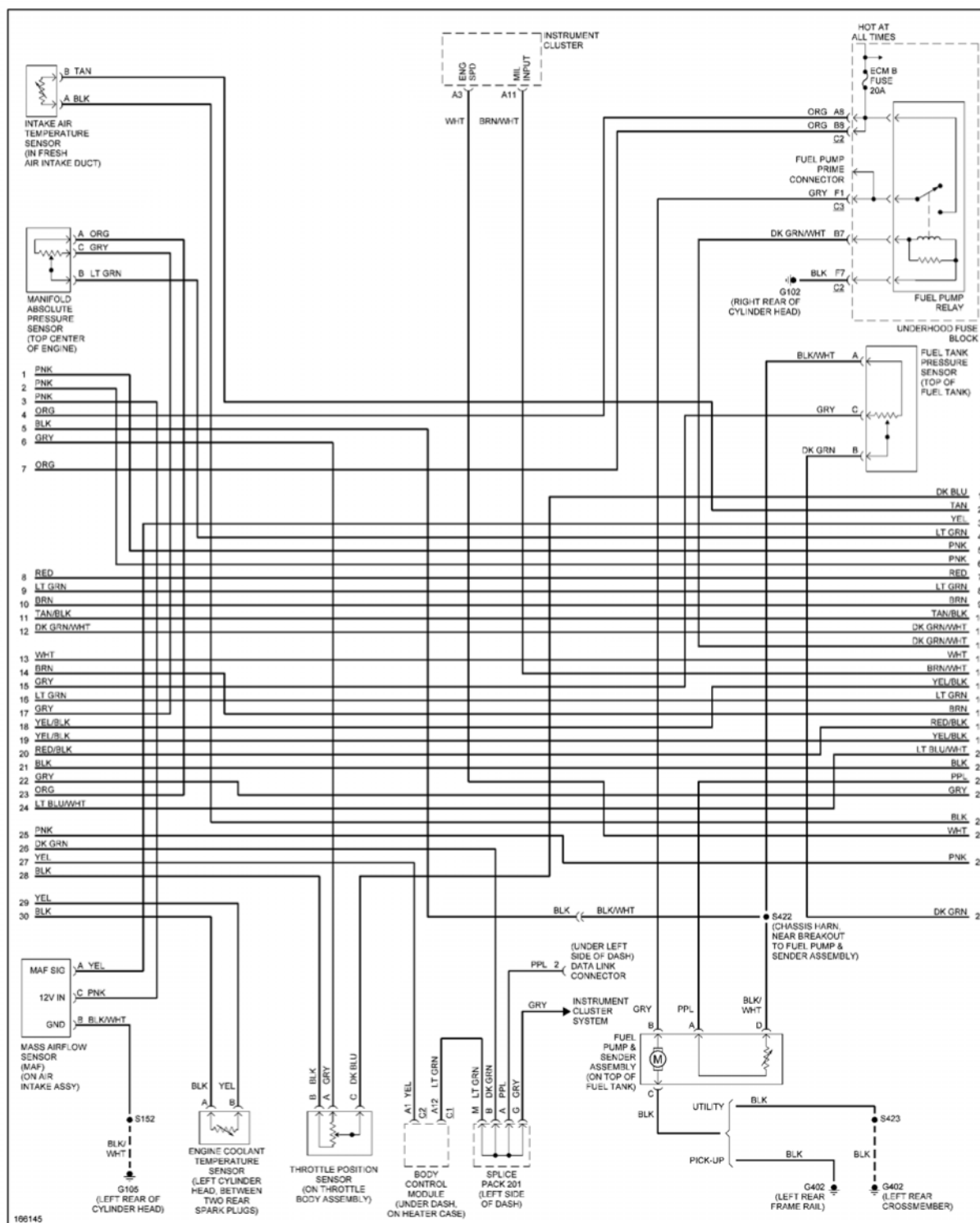
Fig. 12: 4.3L VIN X, Engine Performance Circuit (3 of 4)
