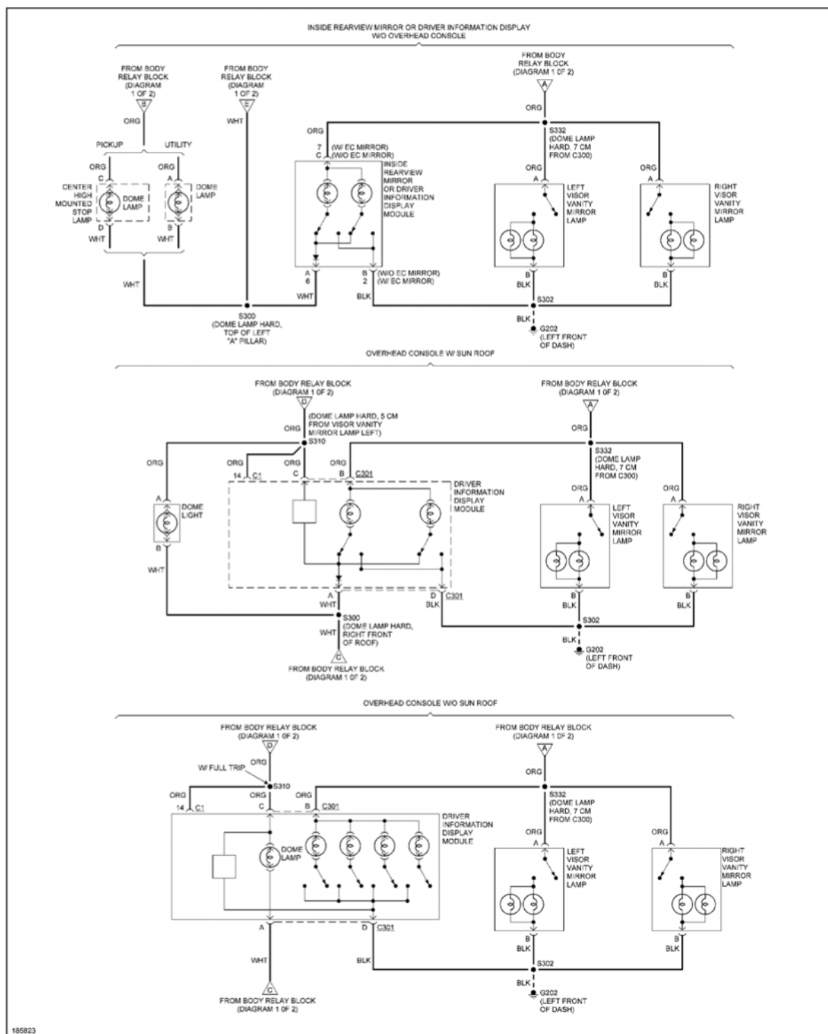
Fig. 25: Courtesy Lamps Circuit (2 of 2)
