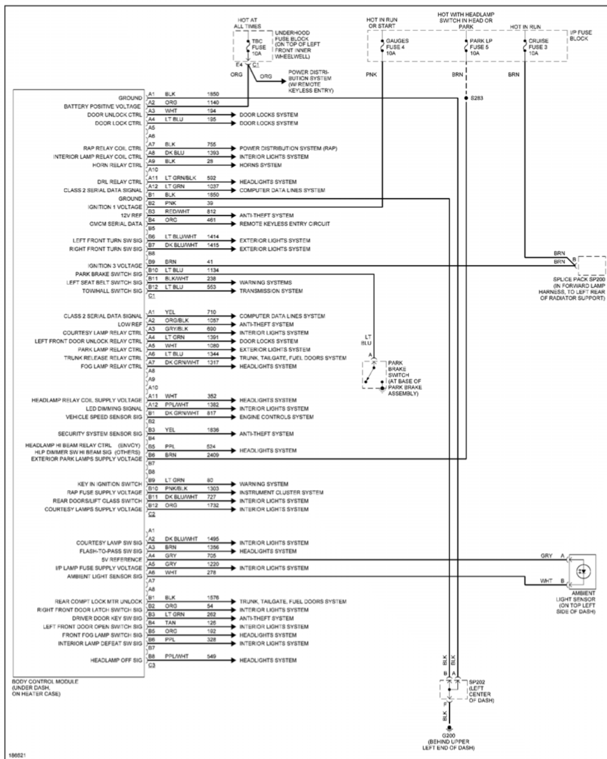
Fig. 6: Body Control Modules Circuit
