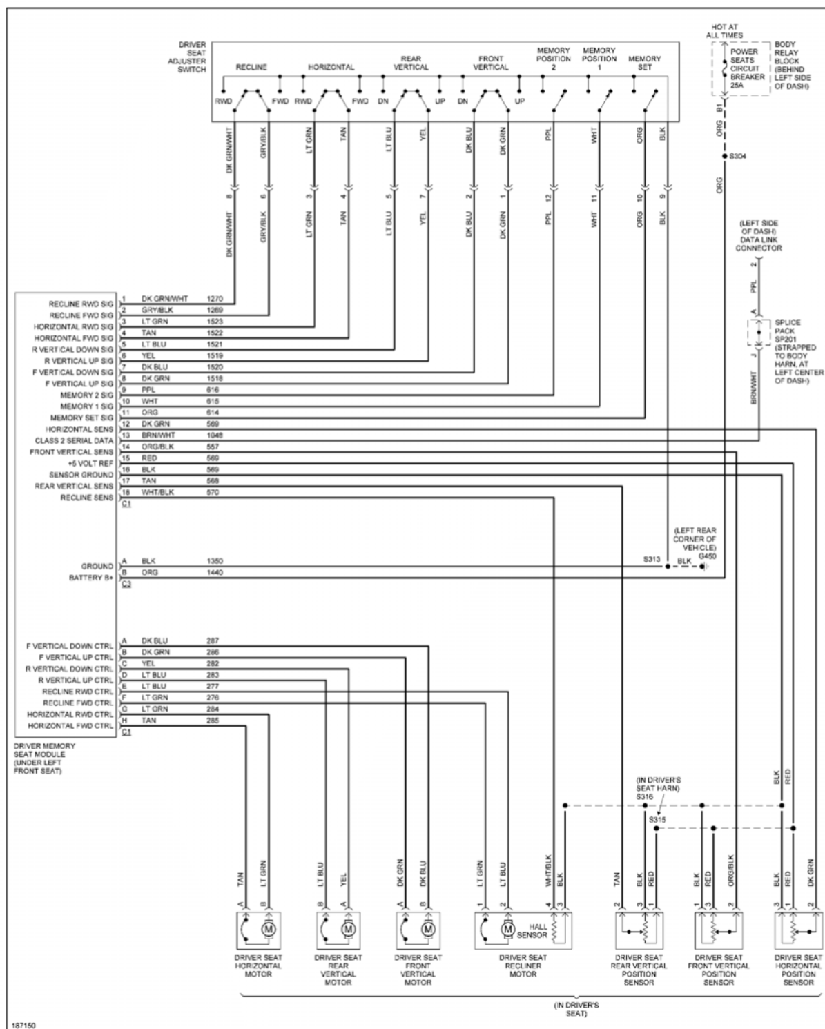
Fig. 27: Driver's Memory Seat Circuit
