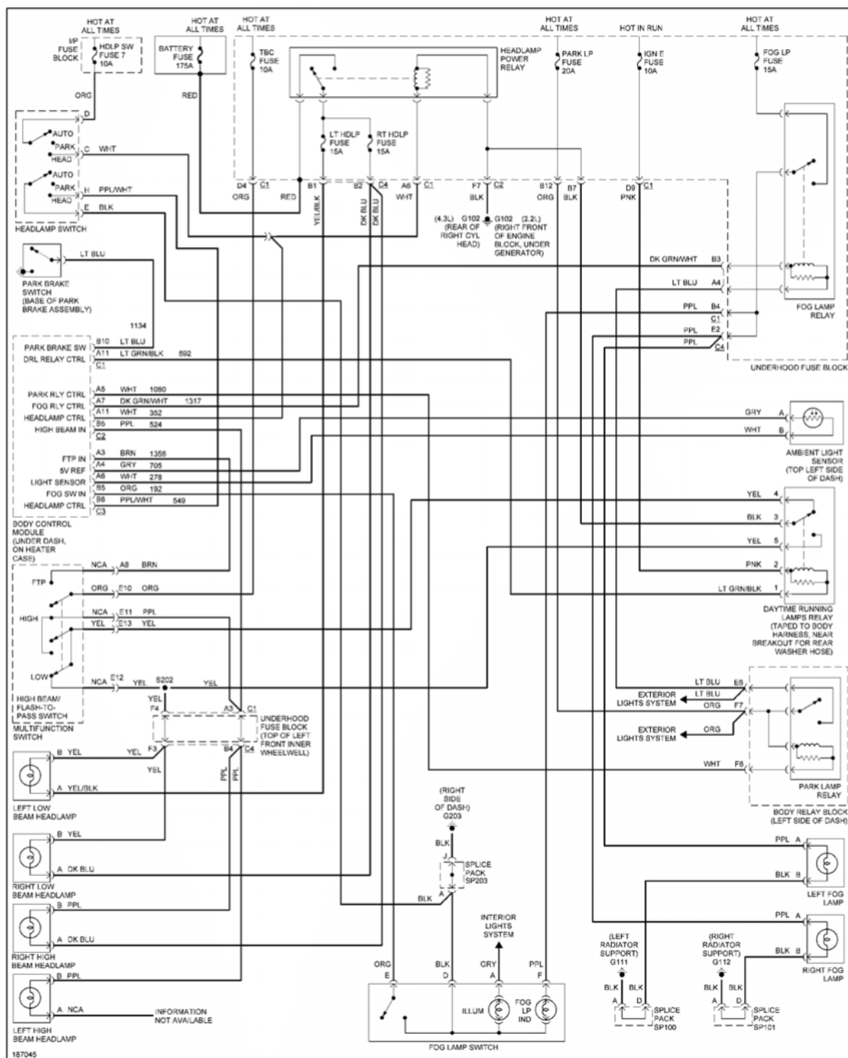
Fig. 19: Headlights Circuit, W/ ZR2
