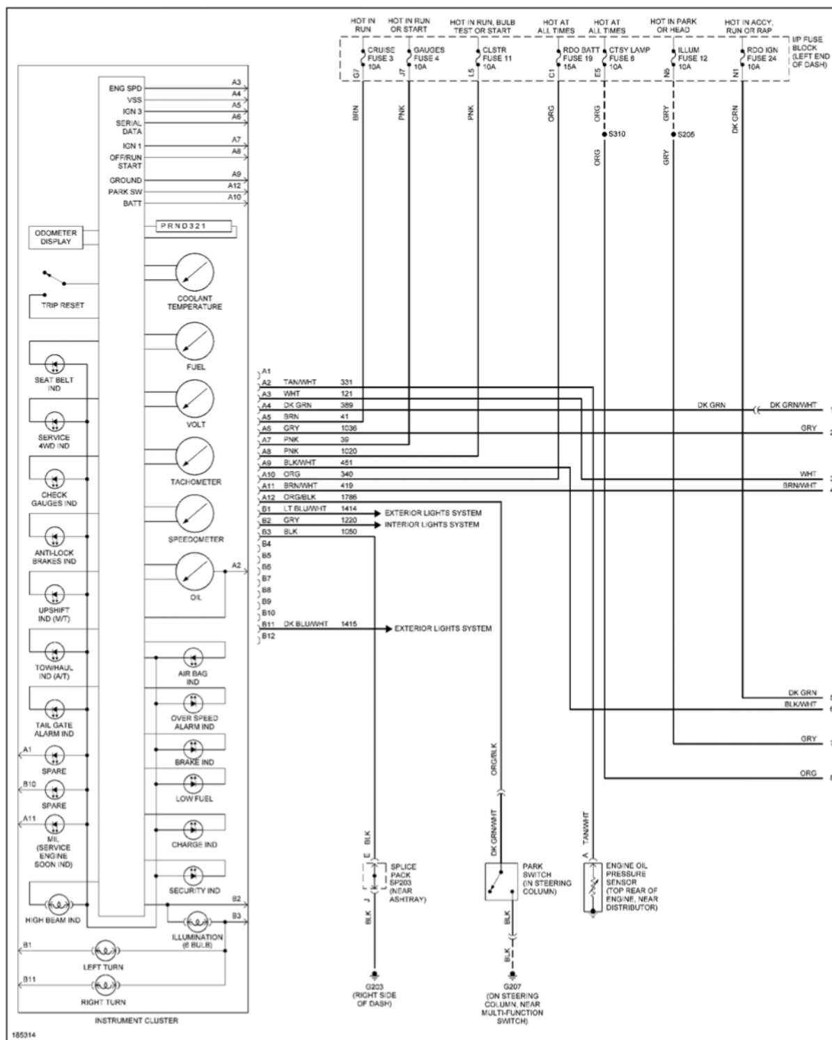
Fig. 22: Instrument Cluster Circuit (1 of 2)
