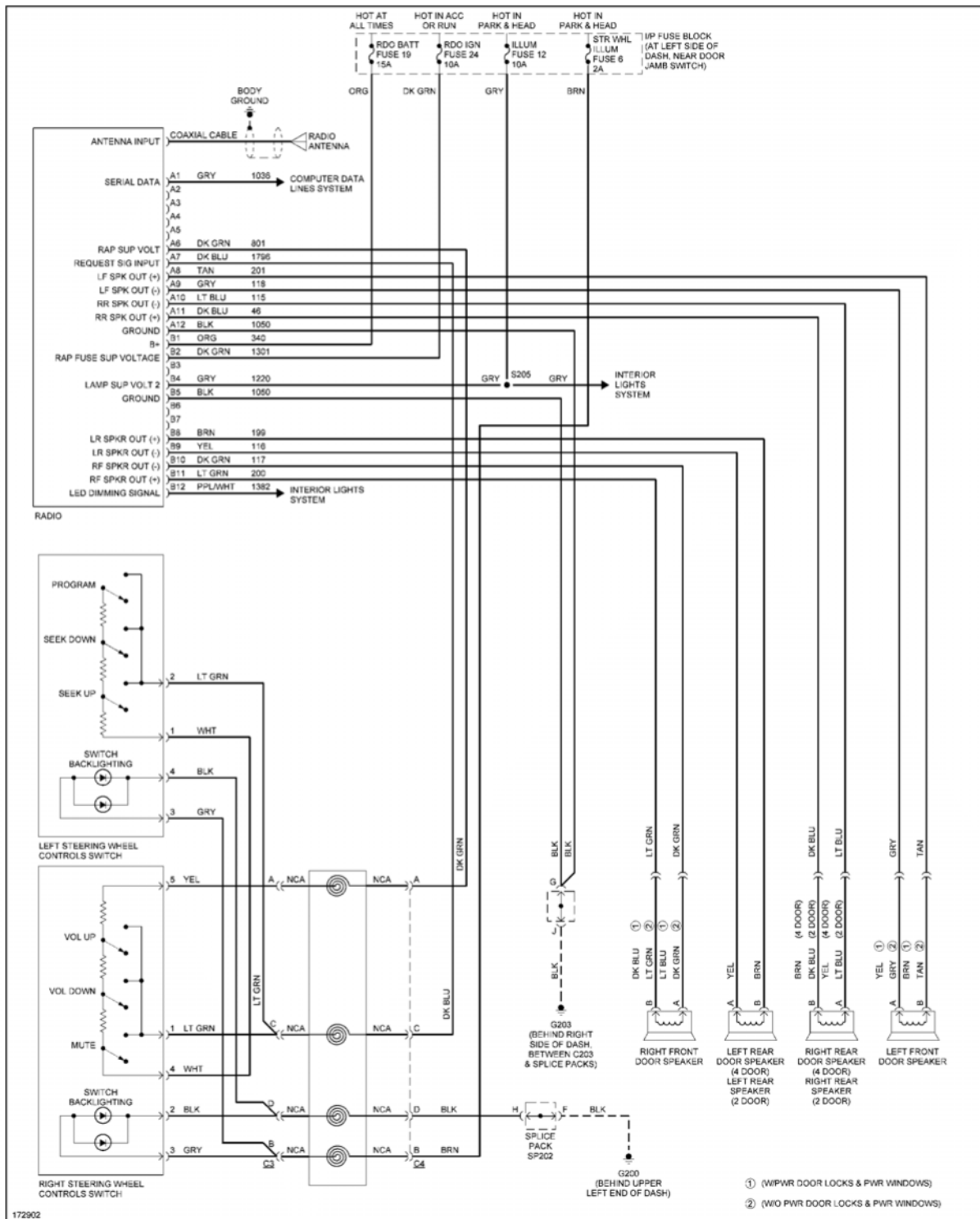
Fig. 44: Radio Circuit
