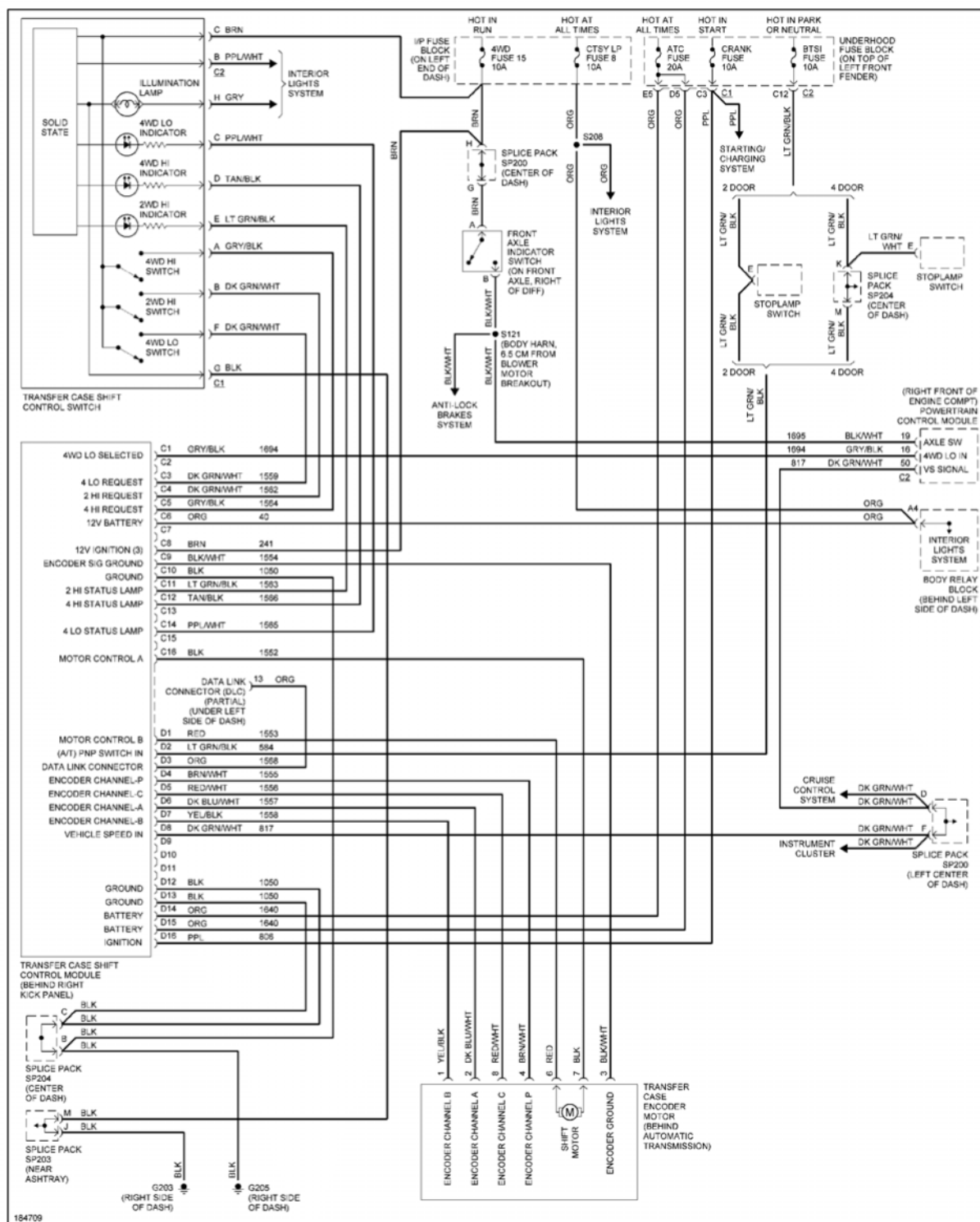
Fig. 53: Transfer Case Circuit, W/ 2-Speed Selectable Transfer Case
