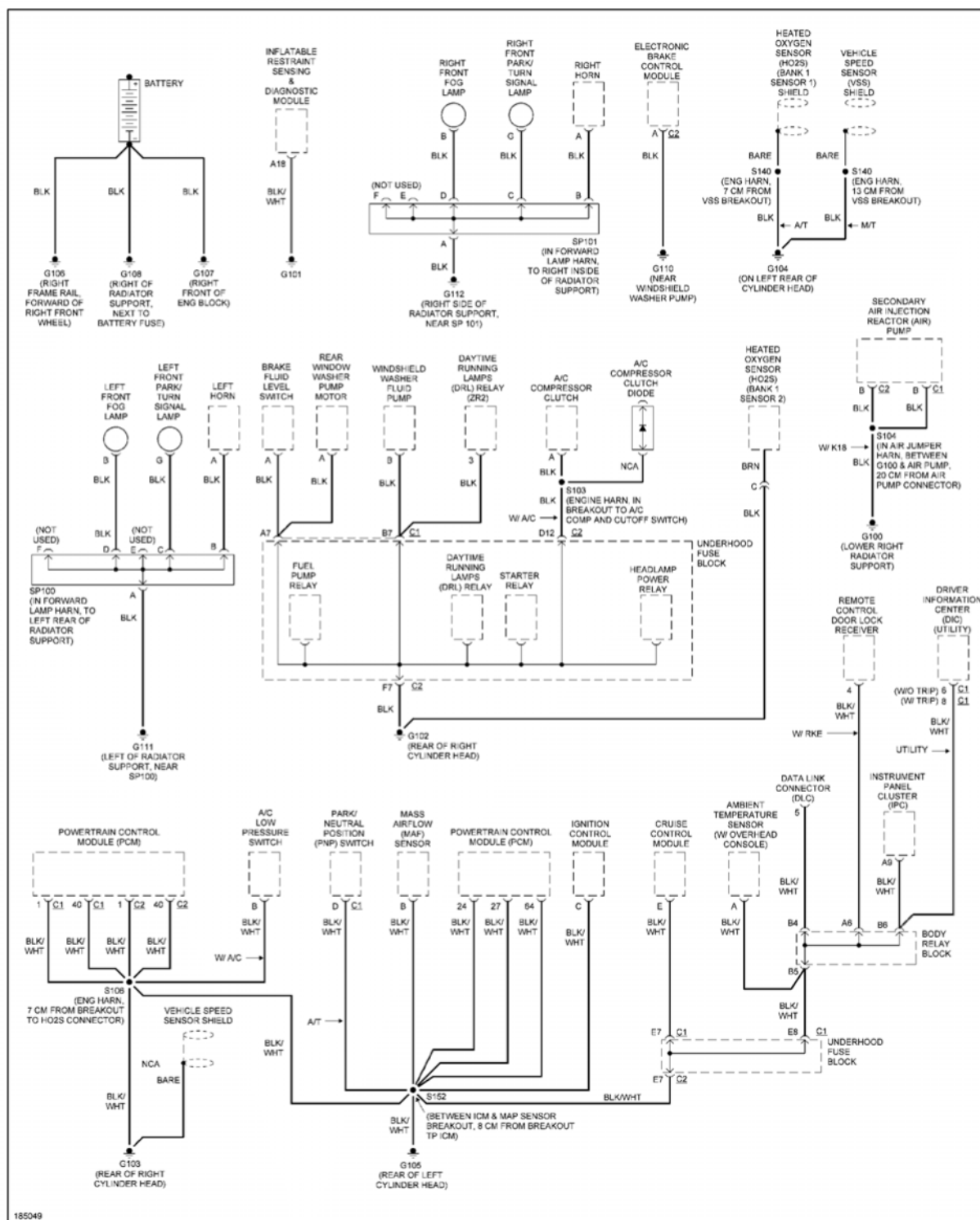
Fig. 16: Ground Distribution Circuit (1 of 3)
