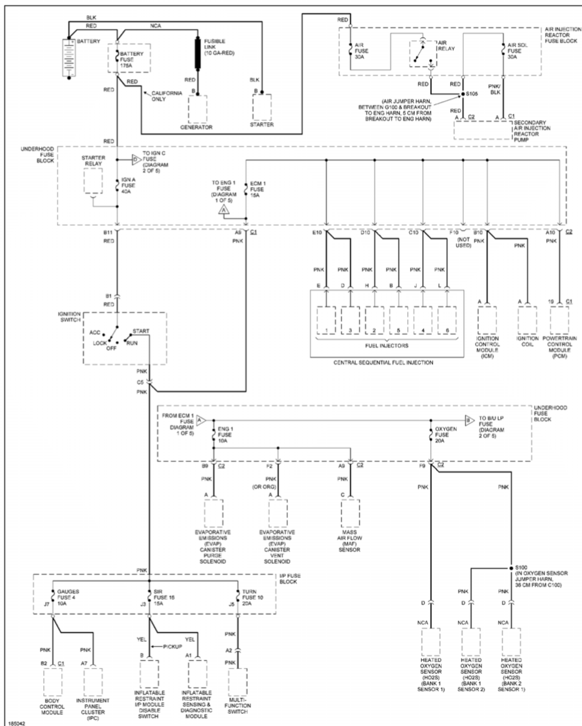
Fig. 28: Power Distribution Circuit (1 of 5)
