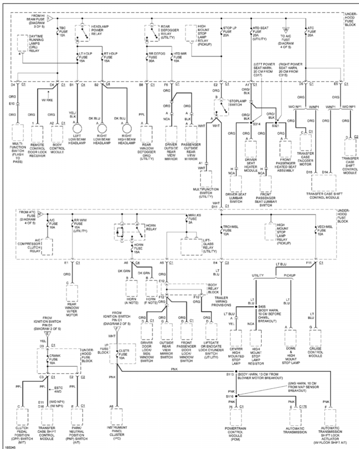
Fig. 31: Power Distribution Circuit (4 of 5)
