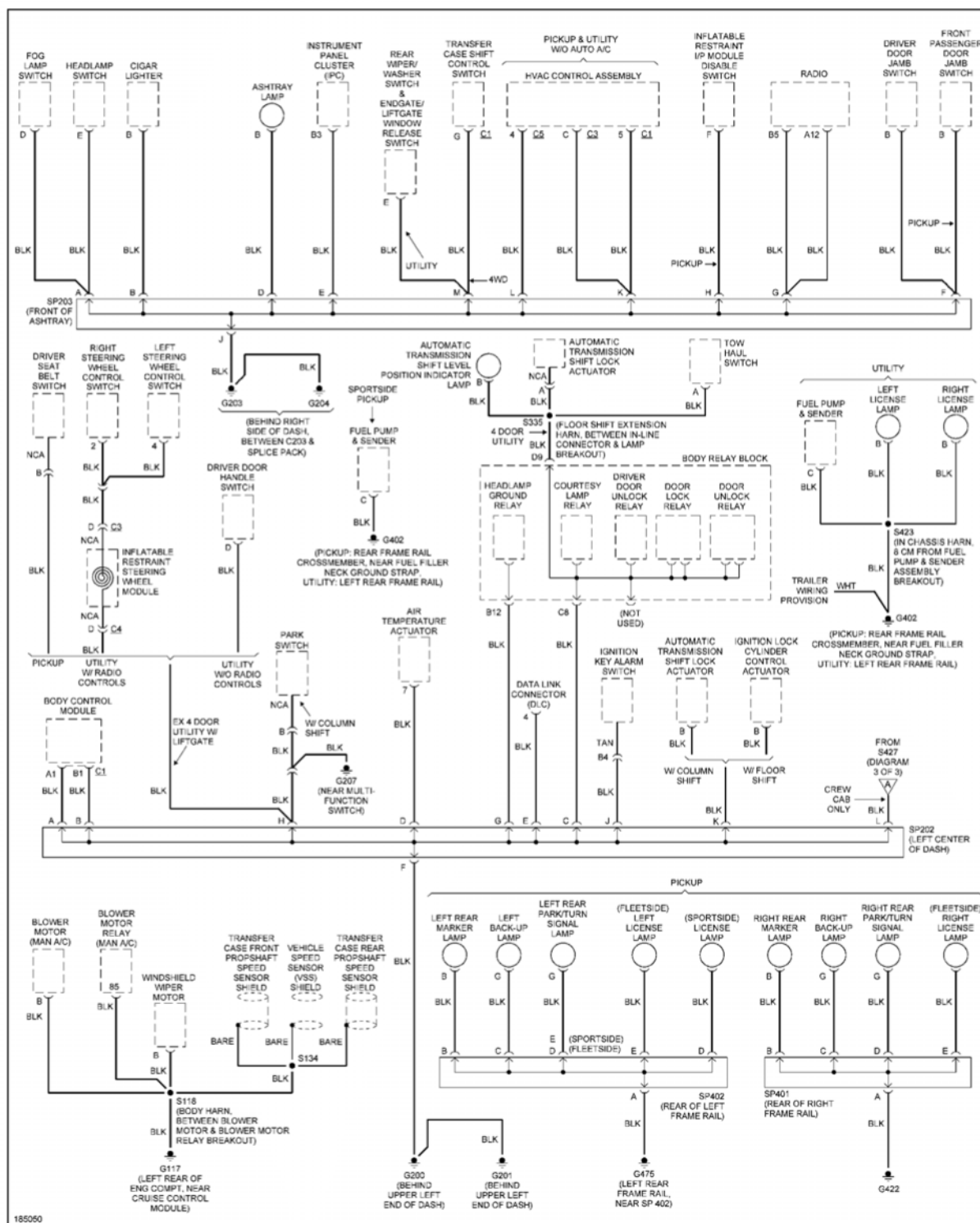
Fig. 17: Ground Distribution Circuit (2 of 3)
