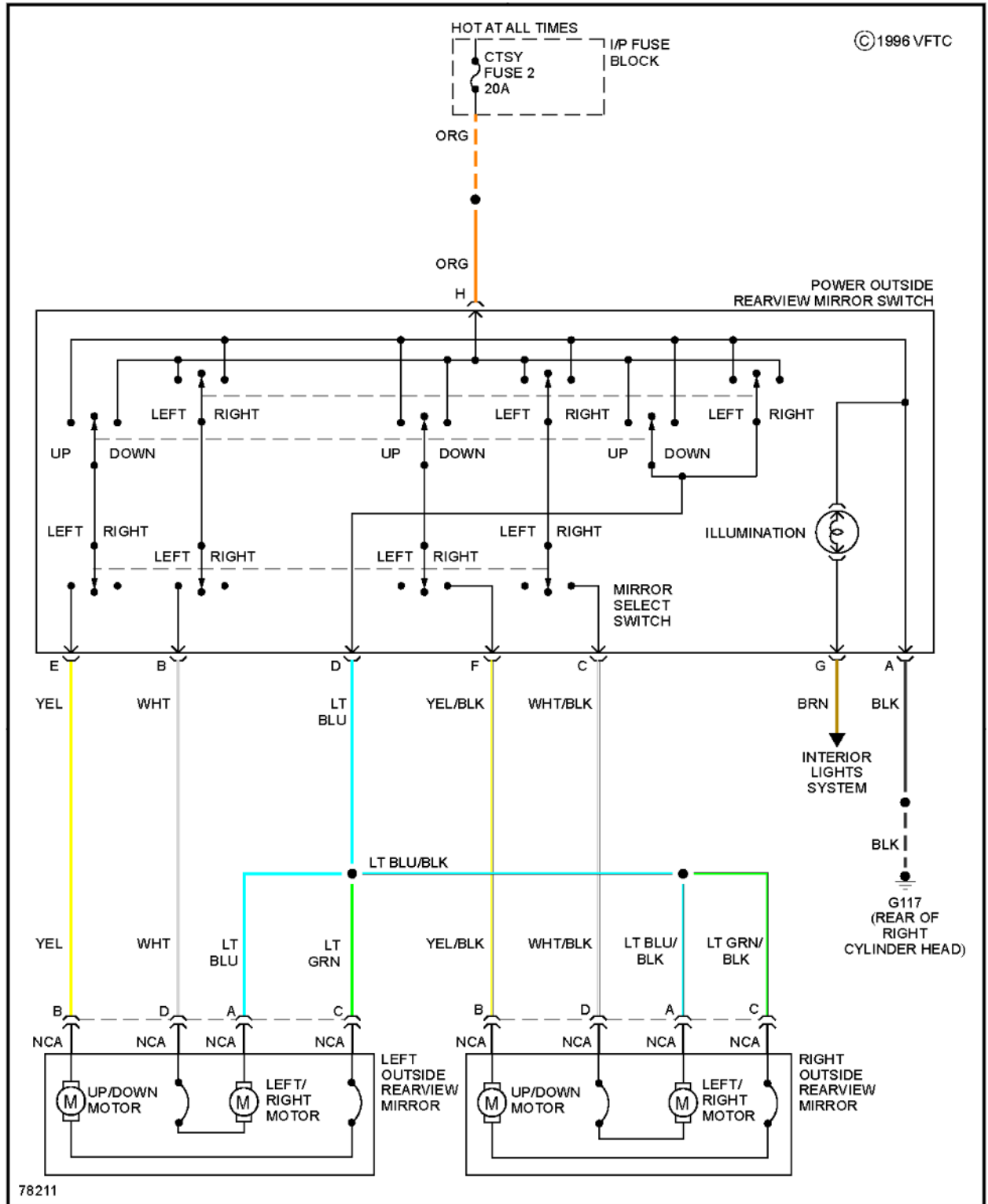
Fig. 25: Power Mirror Circuit
