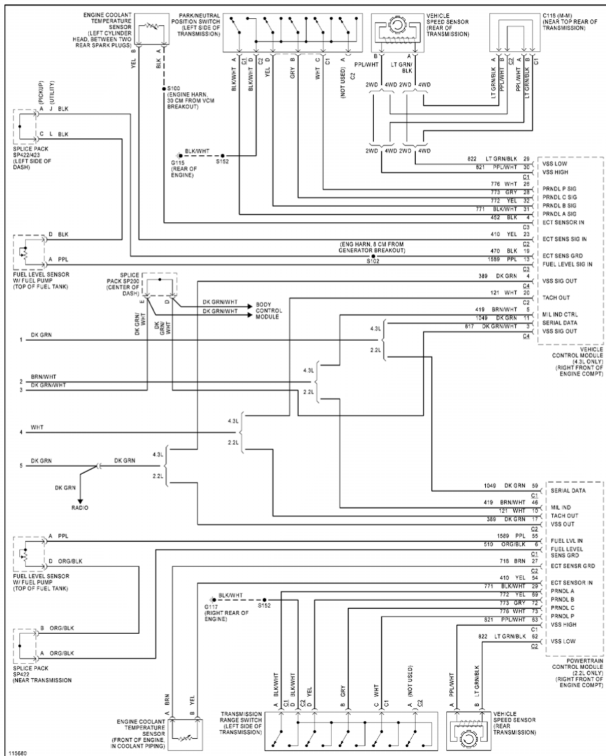
Fig. 25: Instrument Cluster Circuit (2 of 2)
