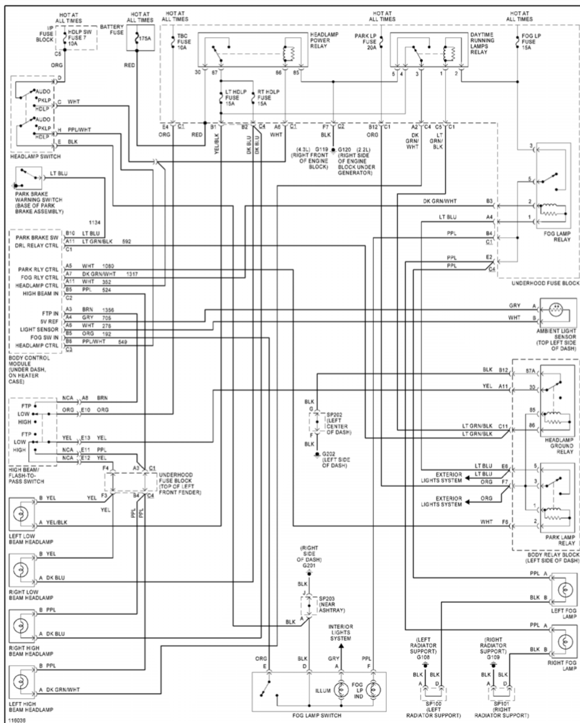
Fig. 22: Headlight Circuit
