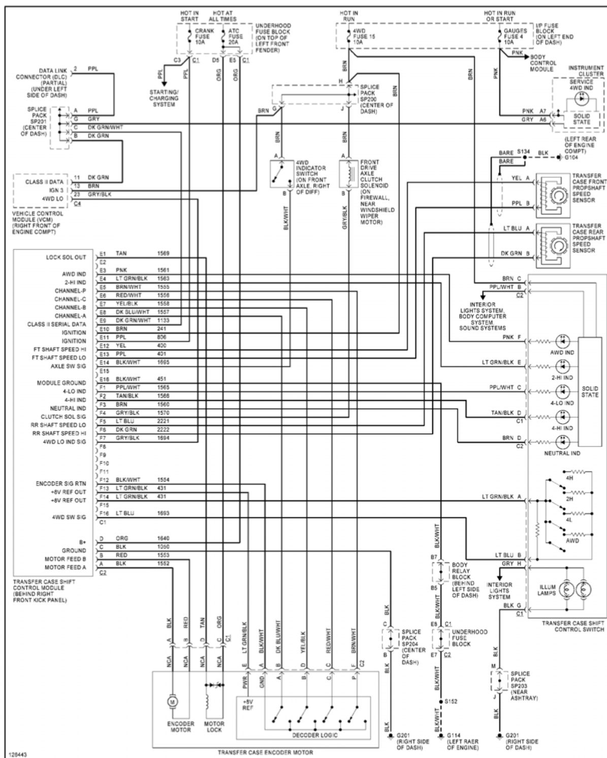
Fig. 52: 4WD Circuit, W/ 2-Speed Automatic Transfer Case
