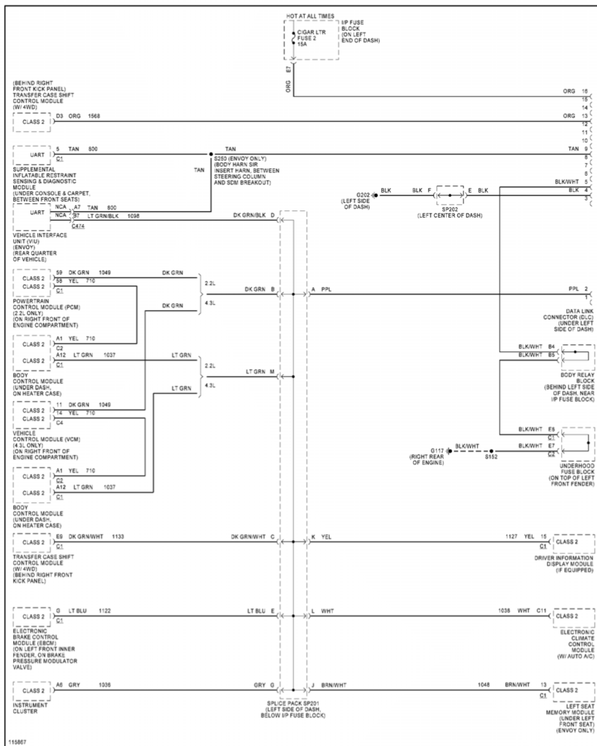
Fig. 9: Computer Data Lines
