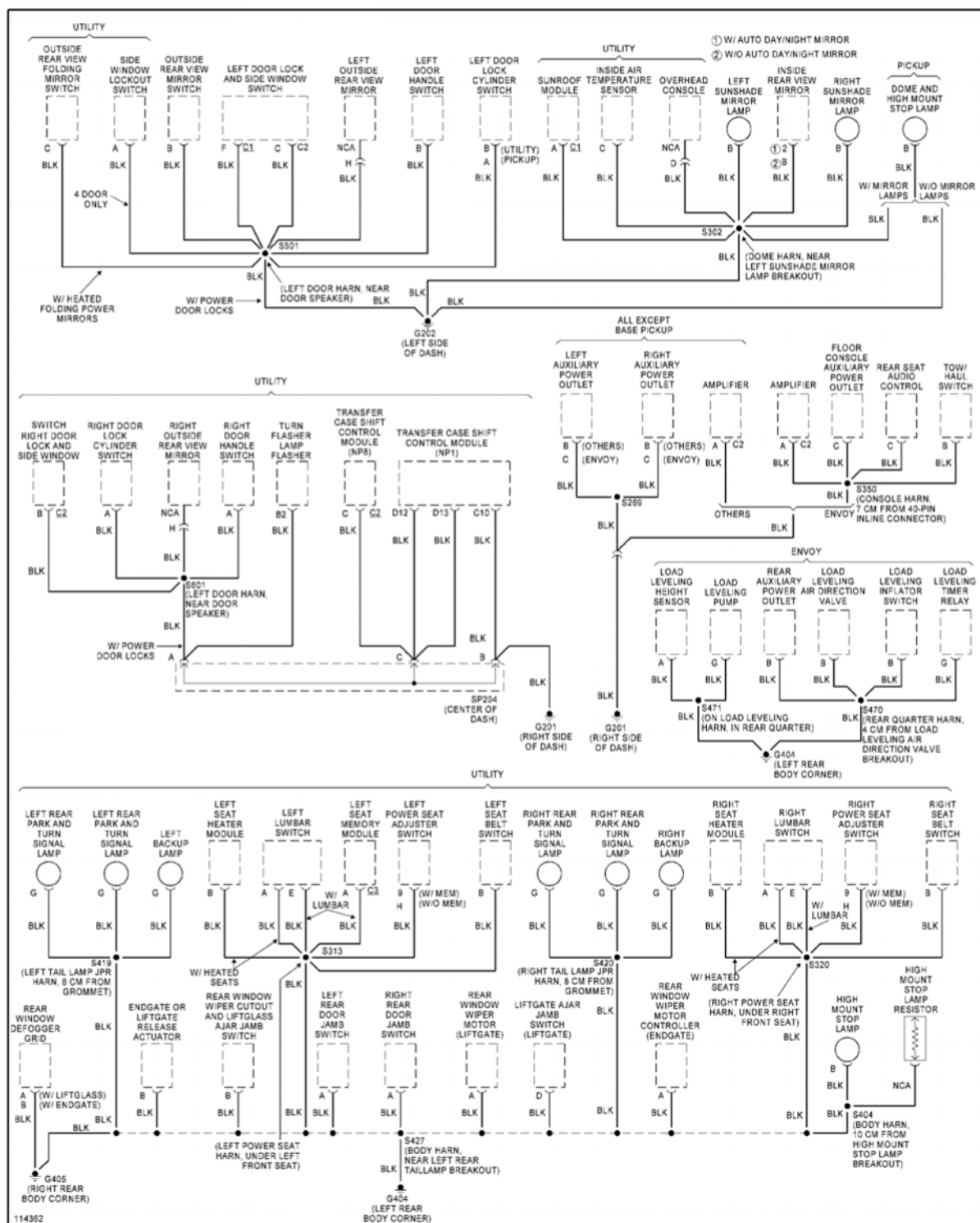
Fig. 21: Ground Distribution Circuit (3 of 3)
