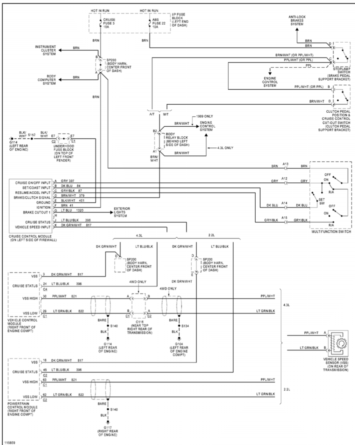
Fig. 10: Cruise Control Circuit
