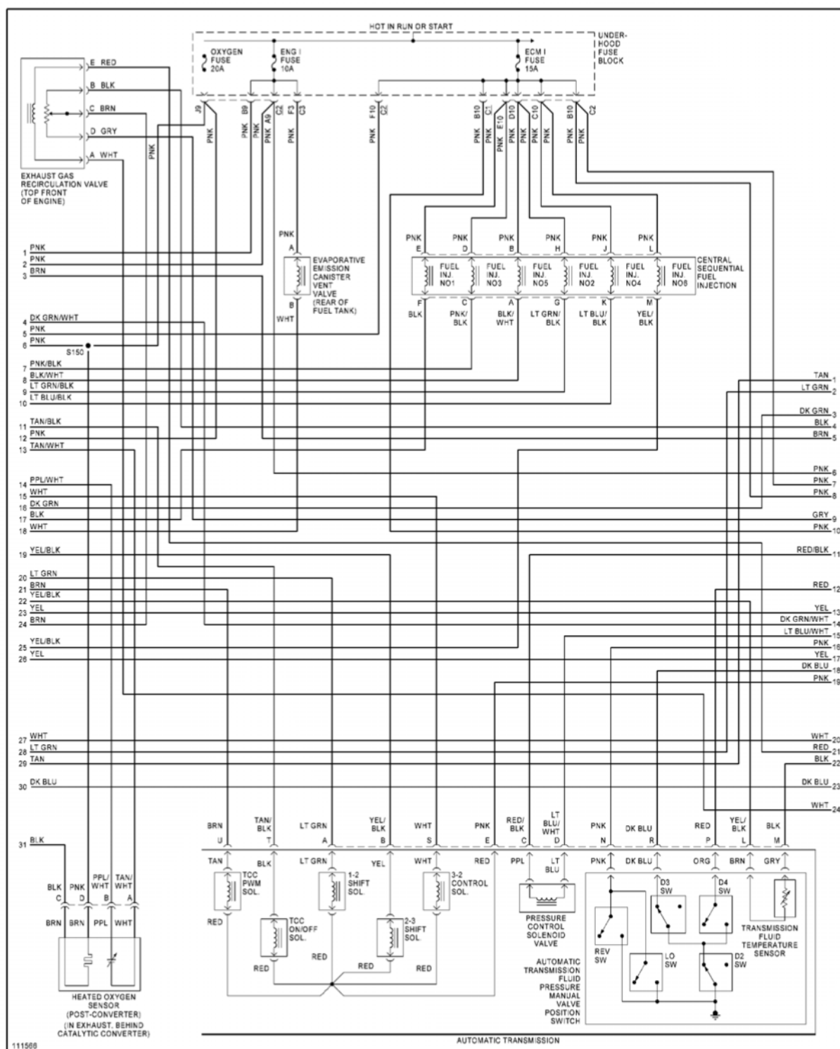
Fig. 14: 4.3L VIN W, Engine Performance Circuits (2 of 4)
