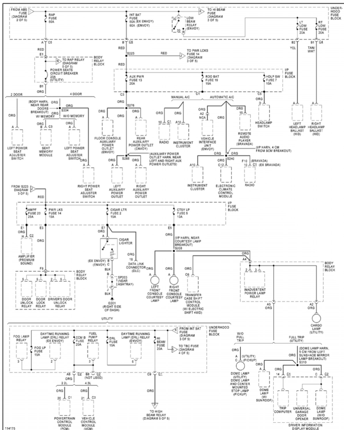
Fig. 32: Power Distribution Circuit (3 of 5)
