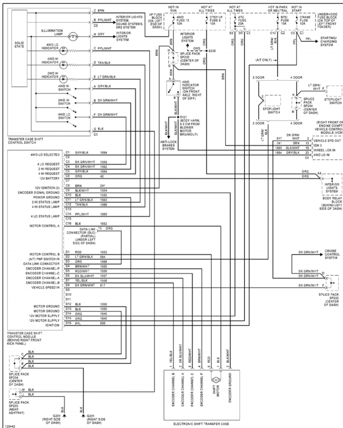
Fig. 53: 4WD Circuit, W/ 2-Speed Selectable Transfer Case
