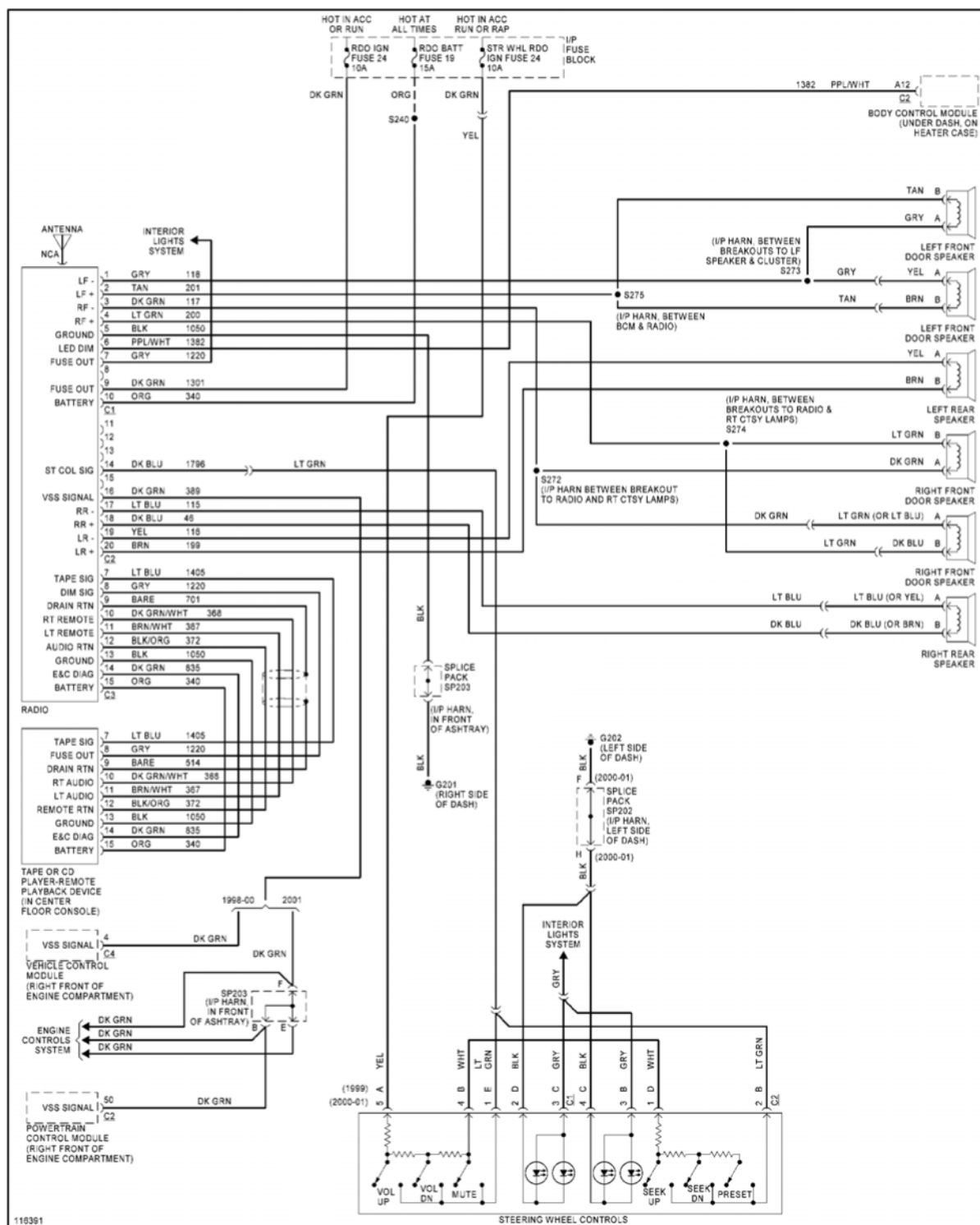
Fig. 45: Radio Circuits, W/O Amplifier
