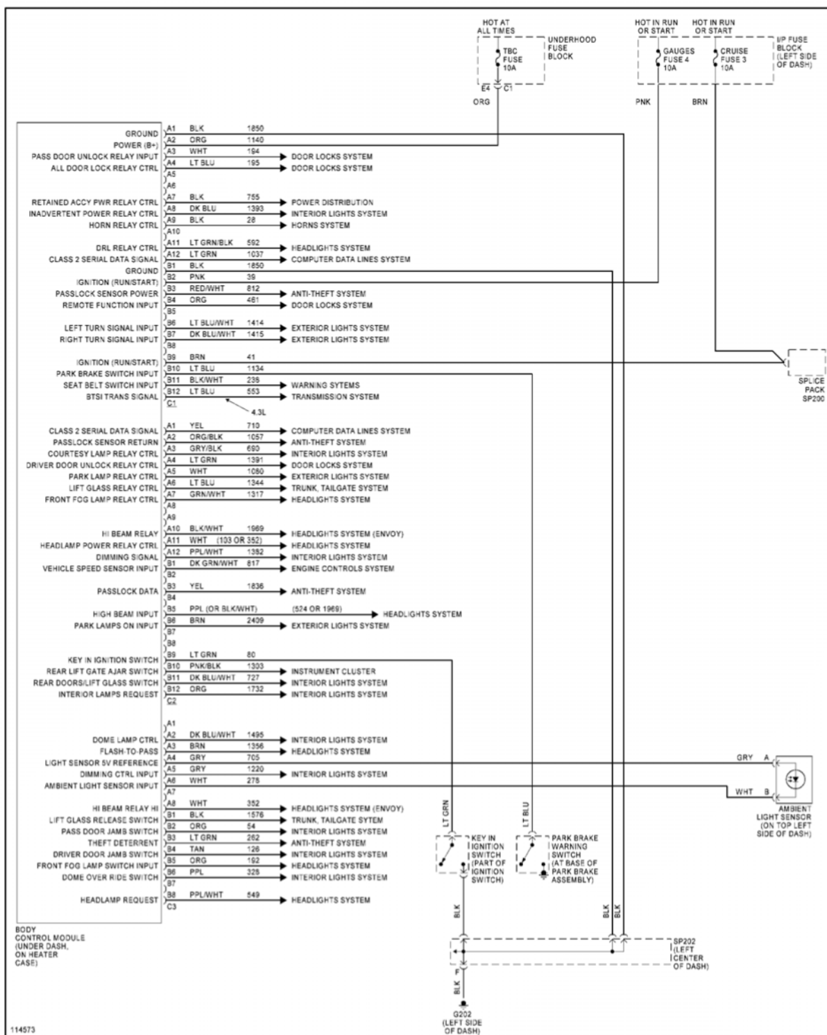
Fig. 8: Body Computer Circuits
