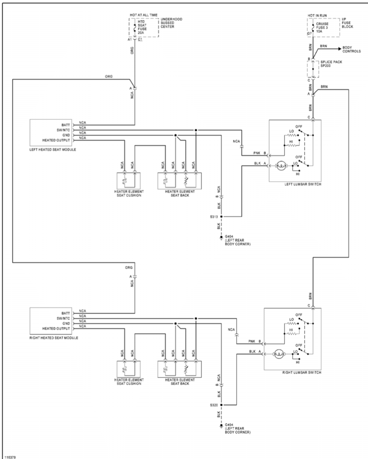
Fig. 39: Heated Seats Circuit
