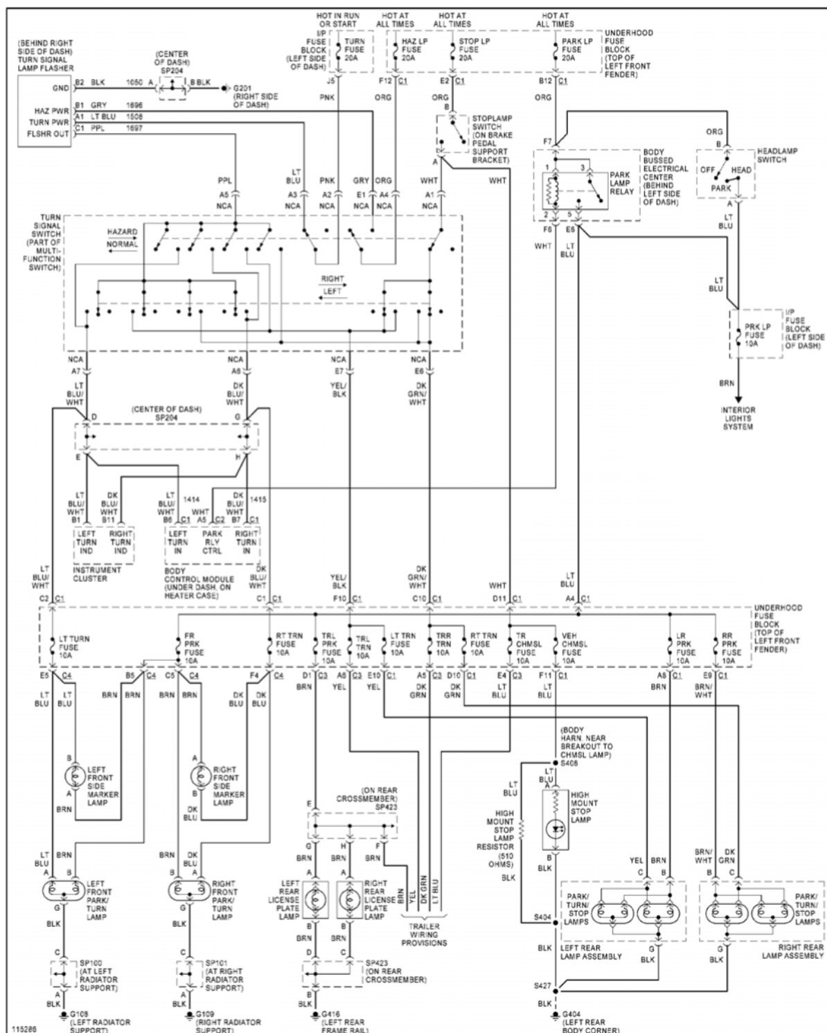
Fig. 18: Exterior Lamps Circuit
