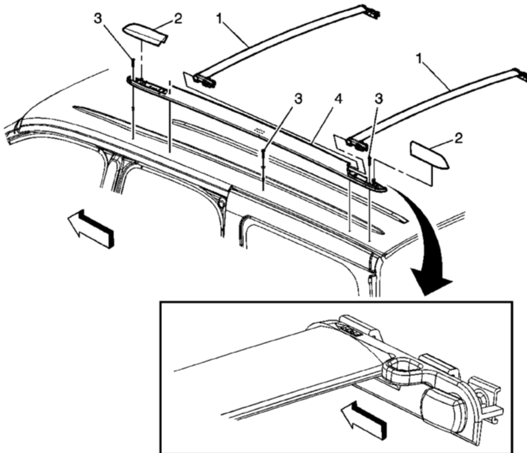
Fig. 2: View Of Luggage Rack & Components
