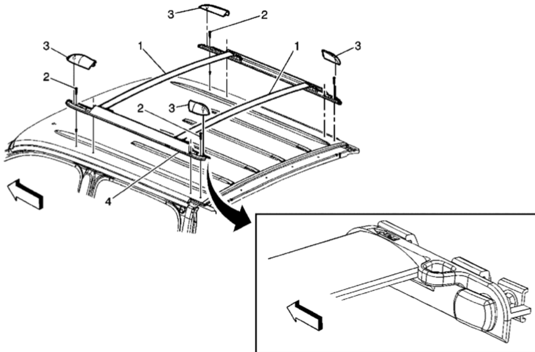
Fig. 1: View Of Luggage Rack & Components Courtesy of GENERAL MOTORS CORP.
