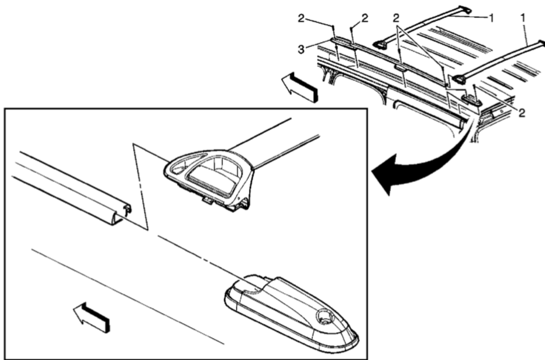
Fig. 3: View Of Luggage Rack & Components Courtesy of GENERAL MOTORS CORP.
