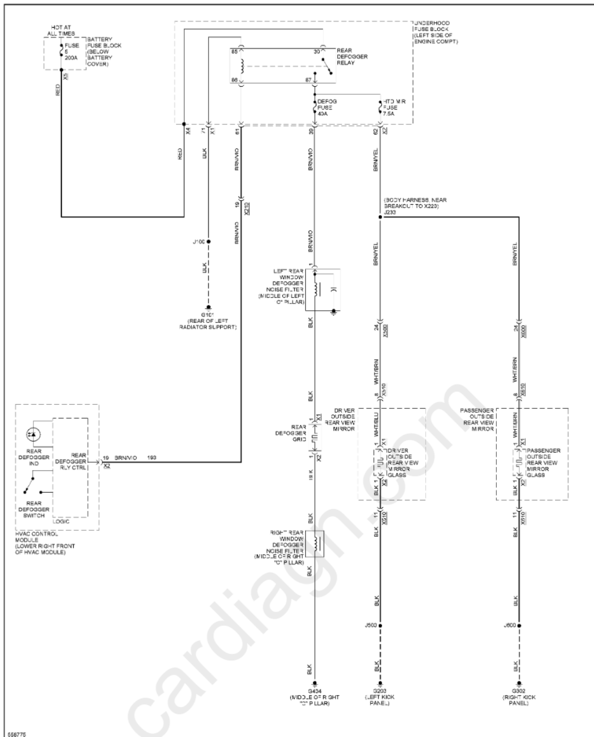
Fig. 31: Defoggers Circuit
