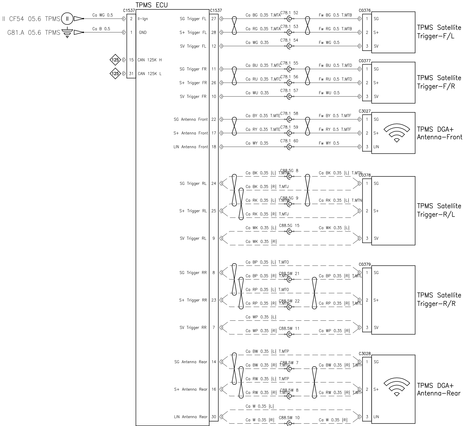
TPMS - Tyre Pressure Monitoring System
