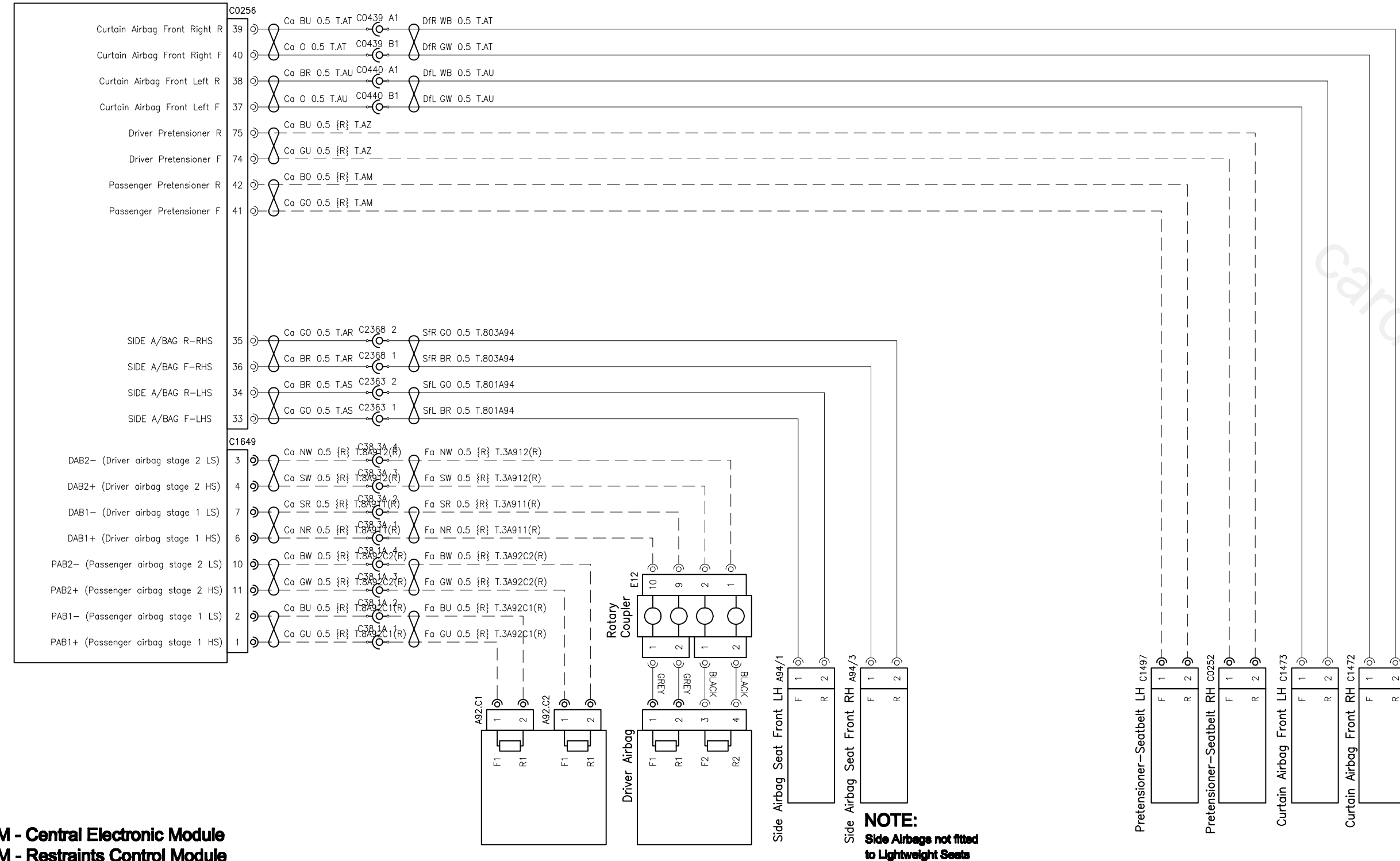
Supplementary Restraint System RHD Vehicles - Front Occupant Airbags and Actuators
