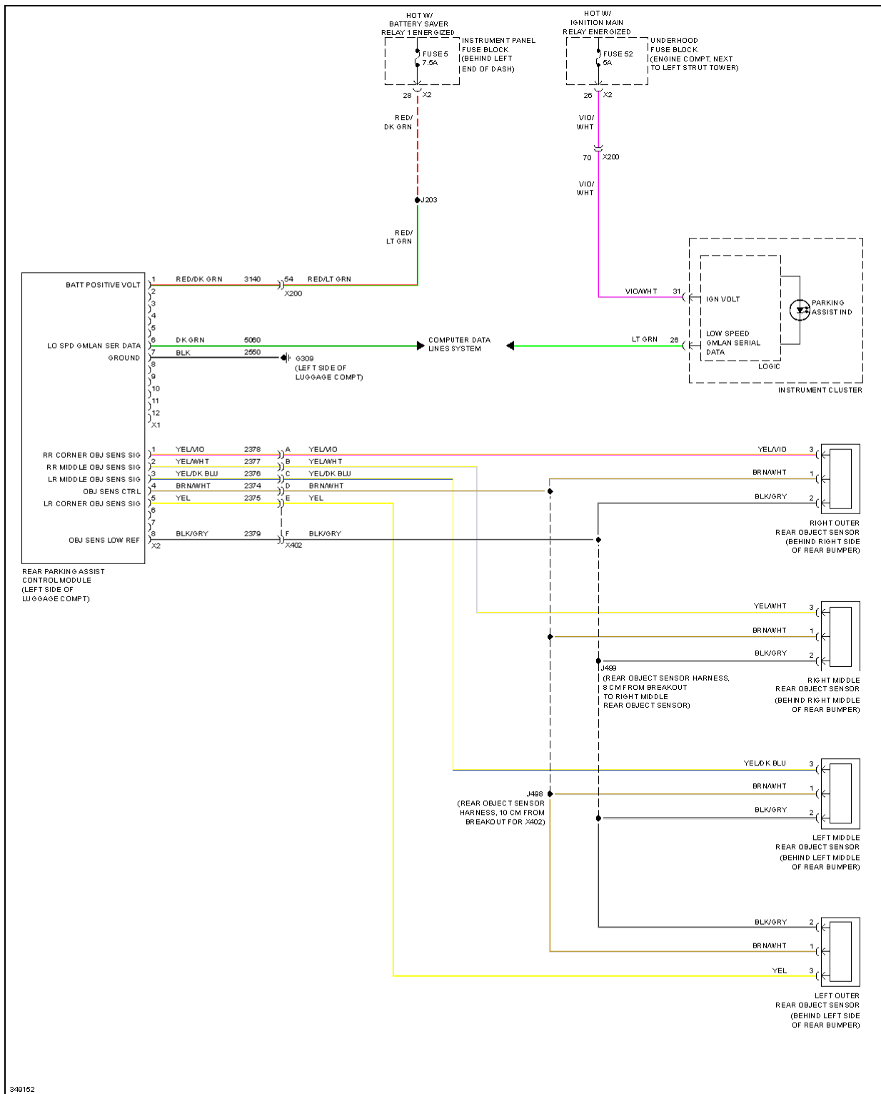
Fig. 46: Parking Assistant Circuit
