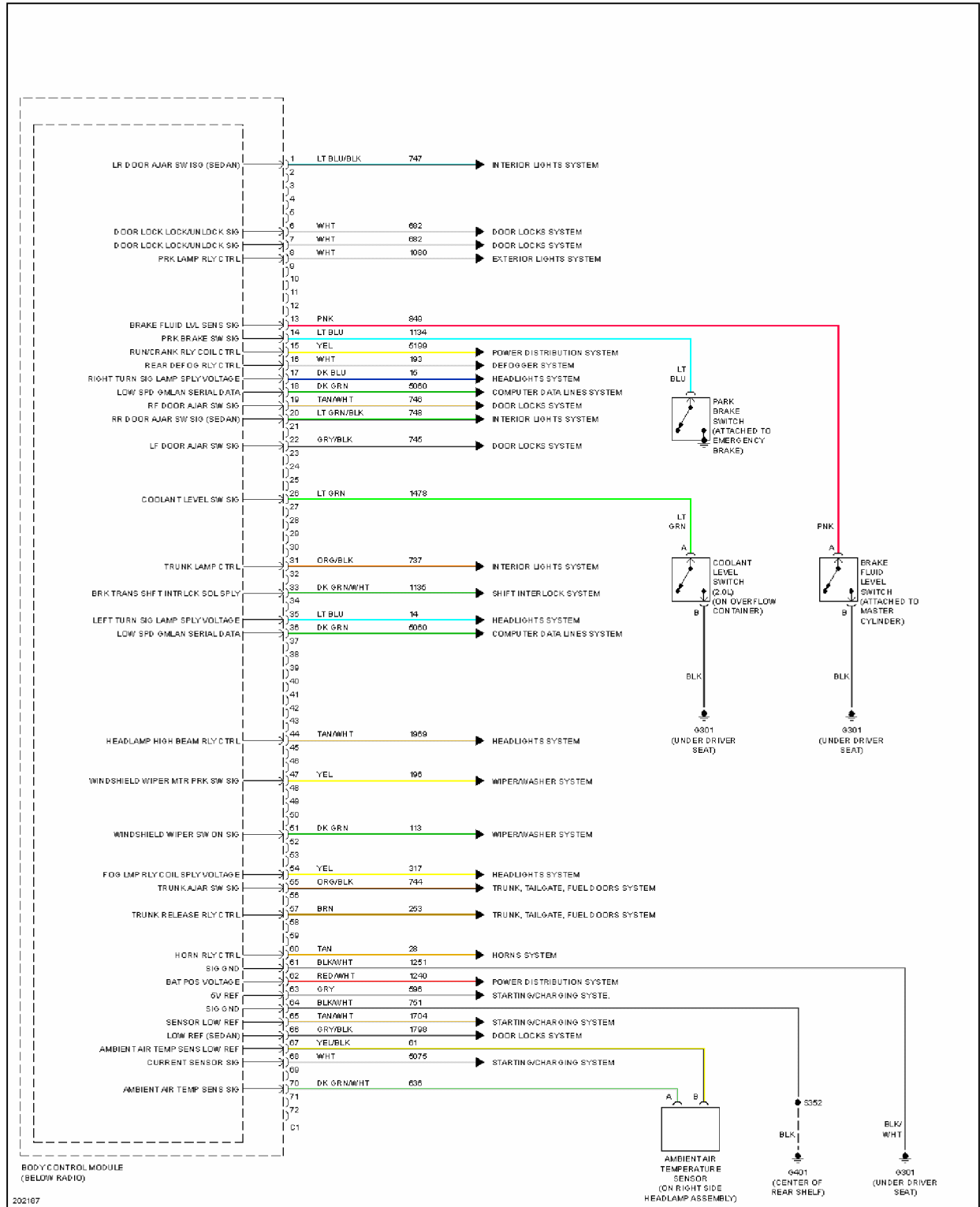
Fig. 10: Body Control Modules Circuit (1 of 4)
