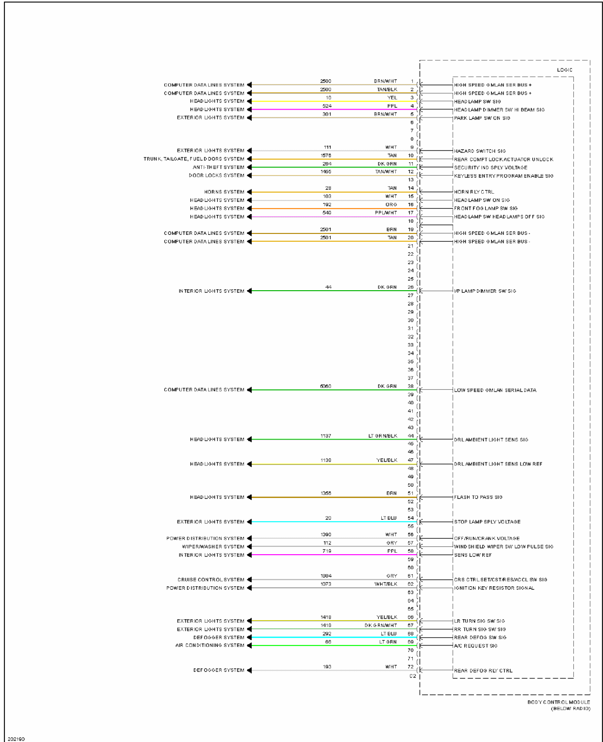
Fig. 13: Body Control Modules Circuit (4 of 4)
