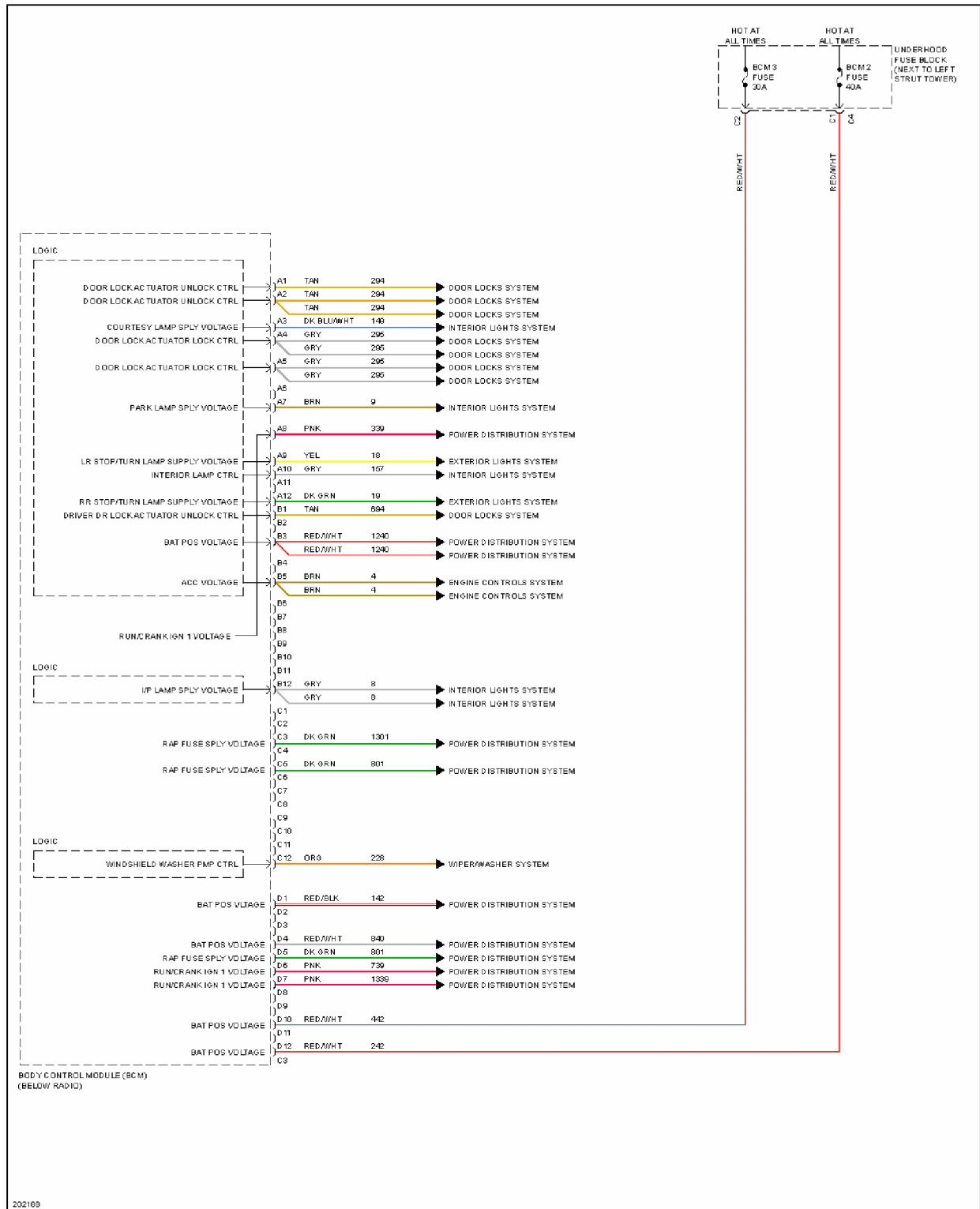
Fig. 11: Body Control Modules Circuit (2 of 4)
