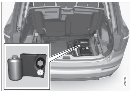
Location of the tire sealing system
