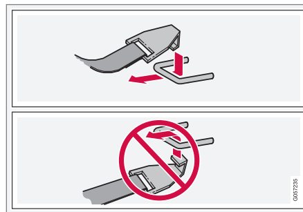
Fasten the attachment correctly to the ISOFIX/LATCH lower anchors
