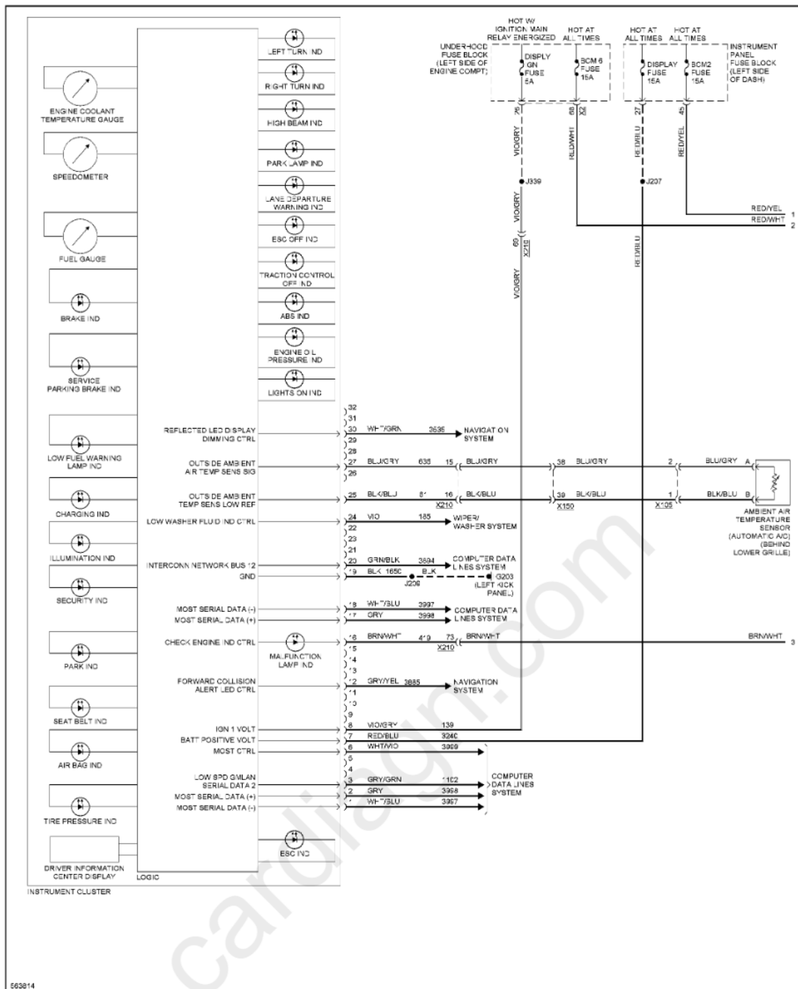
Fig. 63: Instrument Cluster Circuit (1 of 3)
