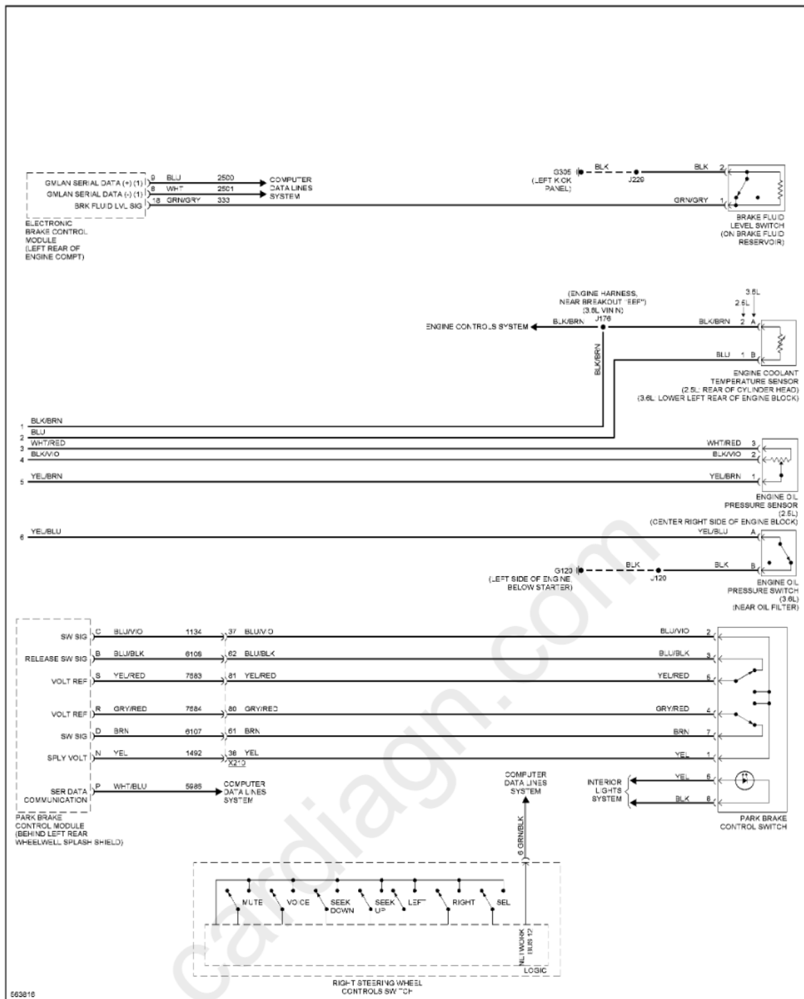
Fig. 65: Instrument Cluster Circuit (3 of 3)
