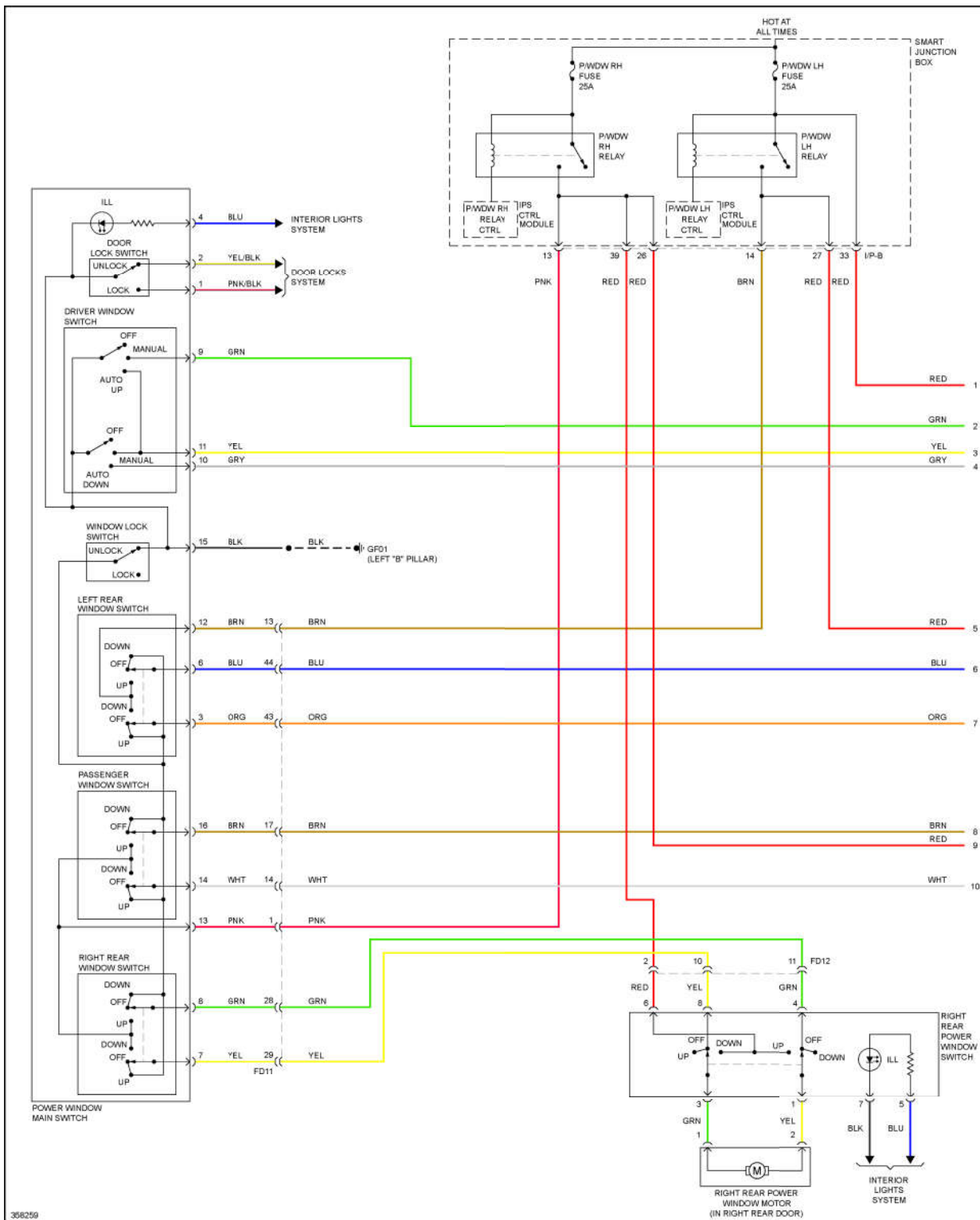
Fig. 63: Power Windows Circuit, W/ Safety Power Windows W/O Central Door Locks (1 of 2)
