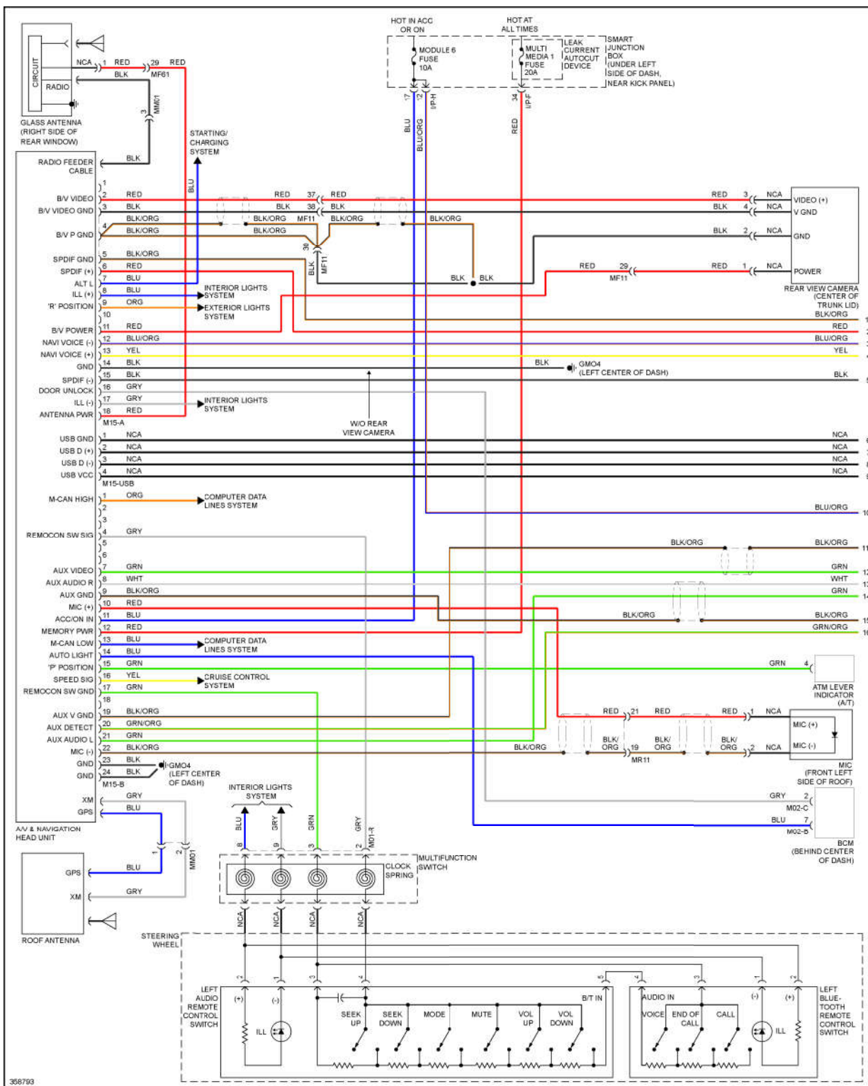
Fig. 71: Radio Circuit, W/ Navigation (1 of 2)
