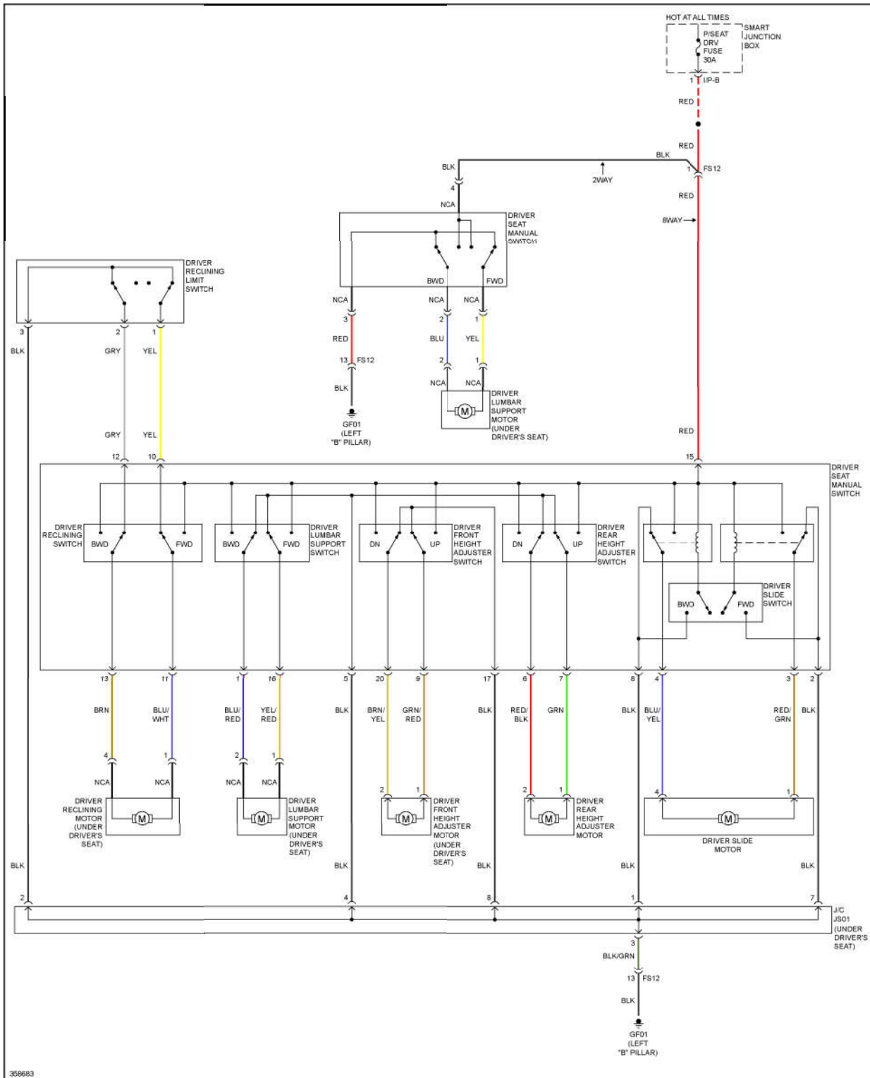
Fig. 59: Power Seats Circuit
