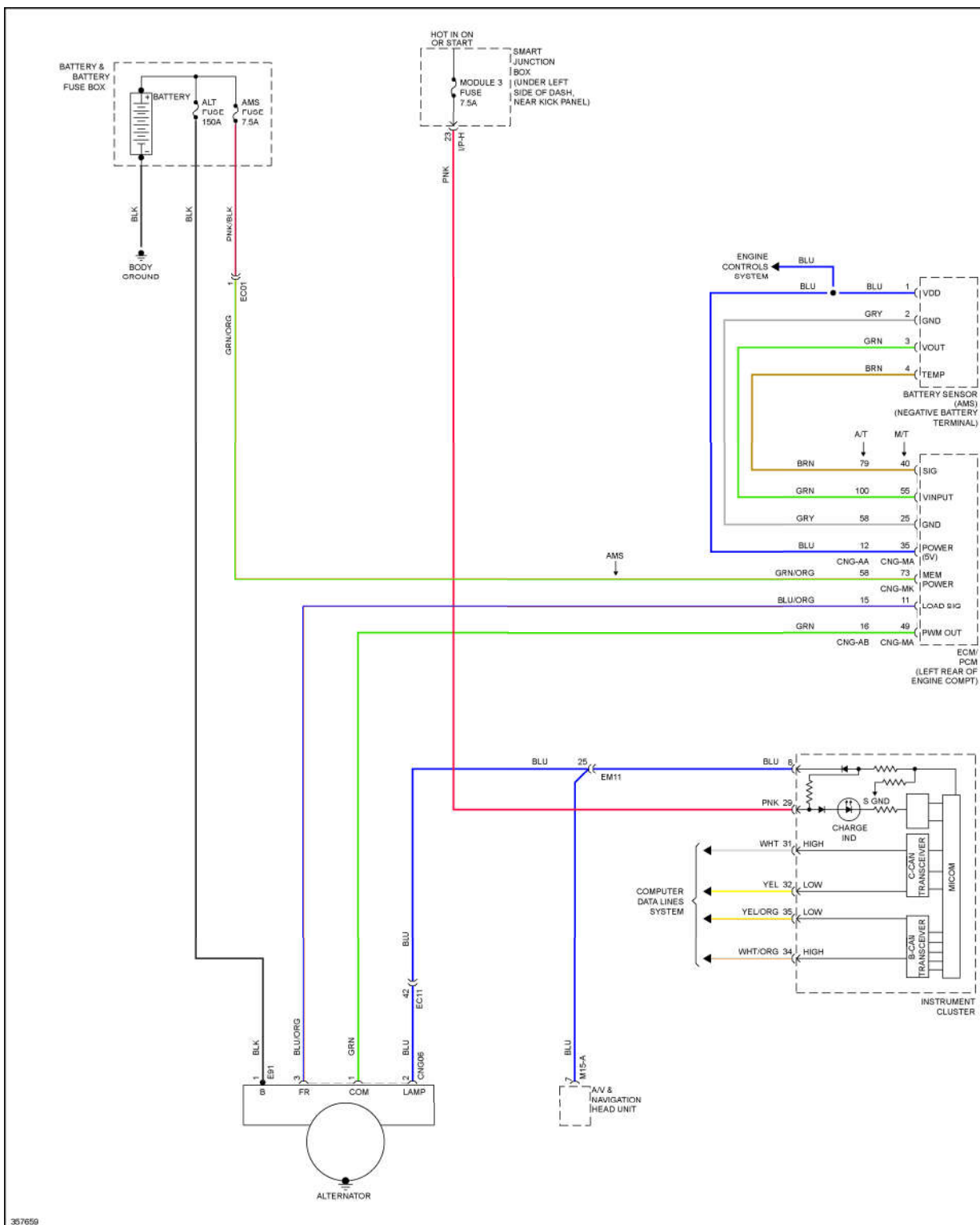
Fig. 76: Charging Circuit
