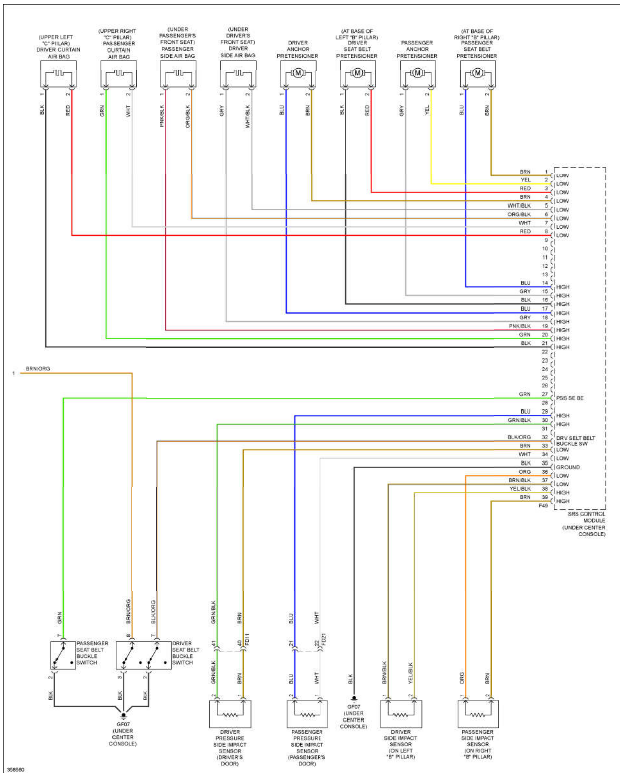
Fig. 80: Supplemental Restraints Circuit (2 of 2)
