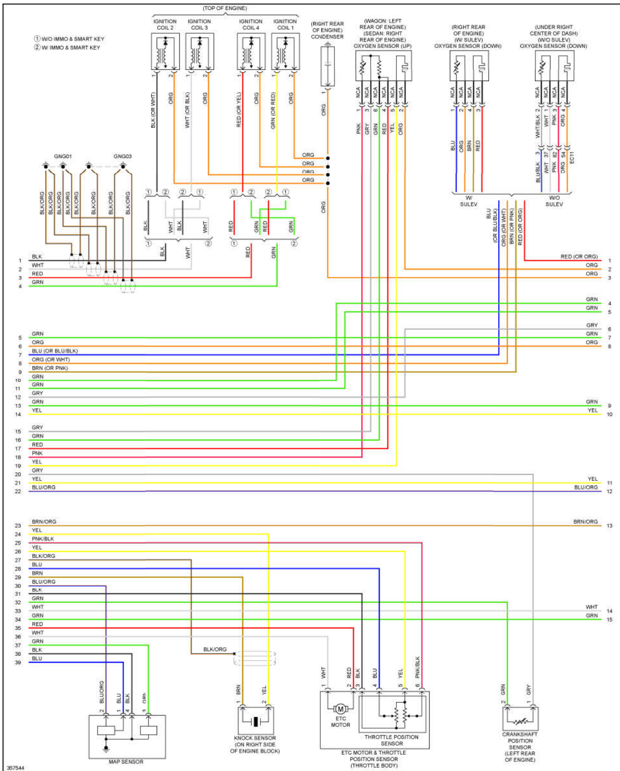
Fig. 26: 1.8L, Engine Performance Circuit, M/T (2 of 5)
