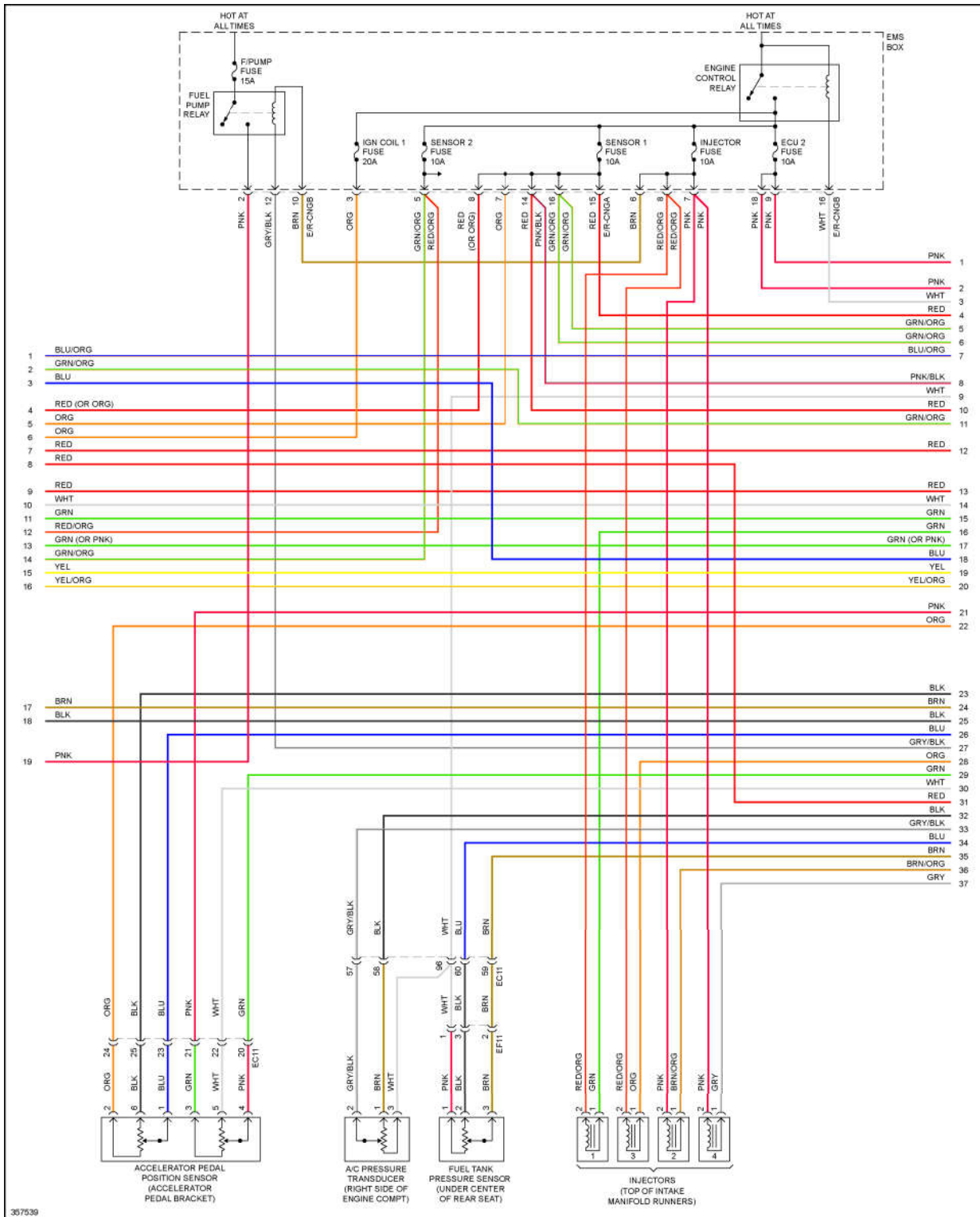
Fig. 23: 1.8L, Engine Performance Circuit, A/T (4 of 5)
