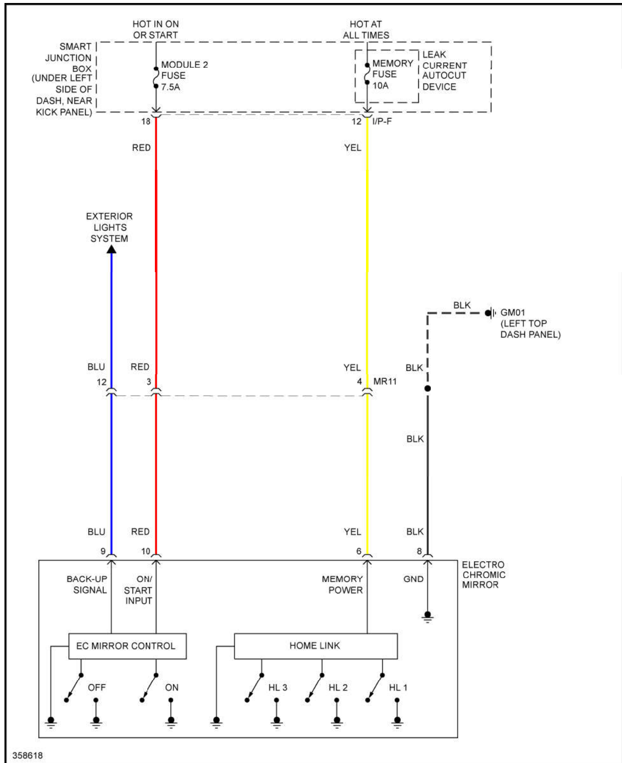
Fig. 54: Electrochromic Mirror Circuit, W/ Home Link
