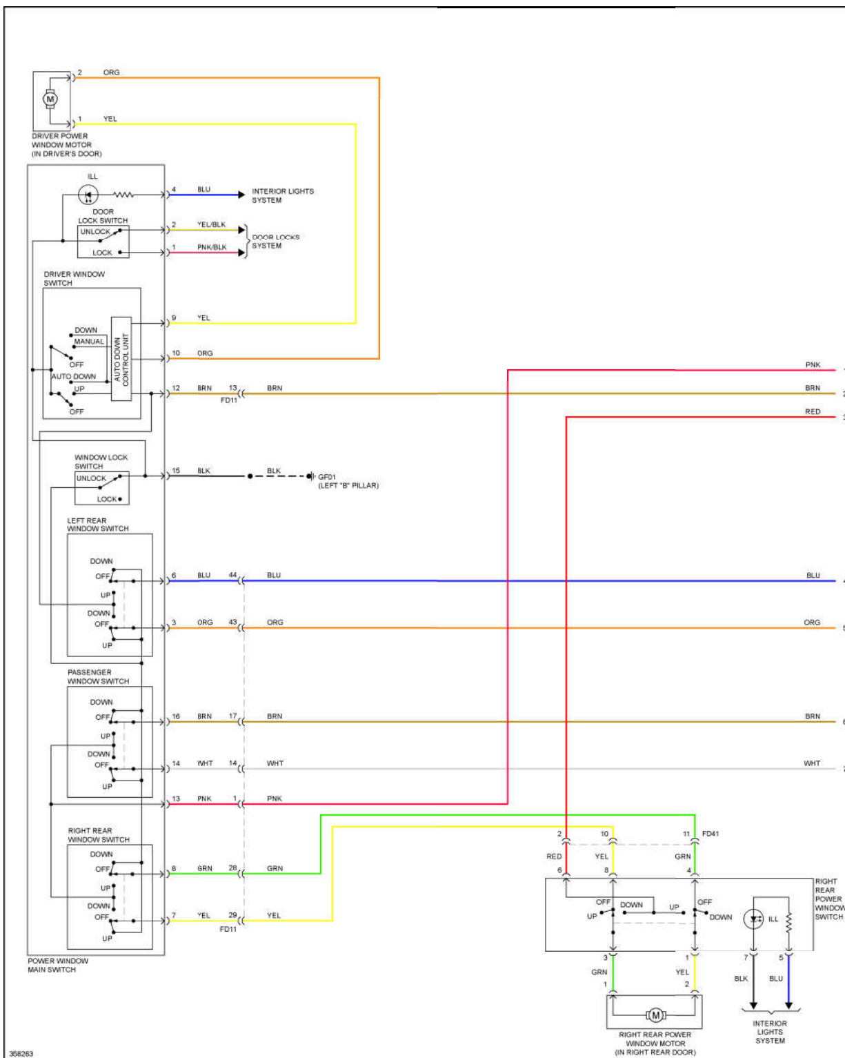
Fig. 67: Power Windows Circuit, W/O Safety Power Windows W/O Central Door Locks (1 of 2)
