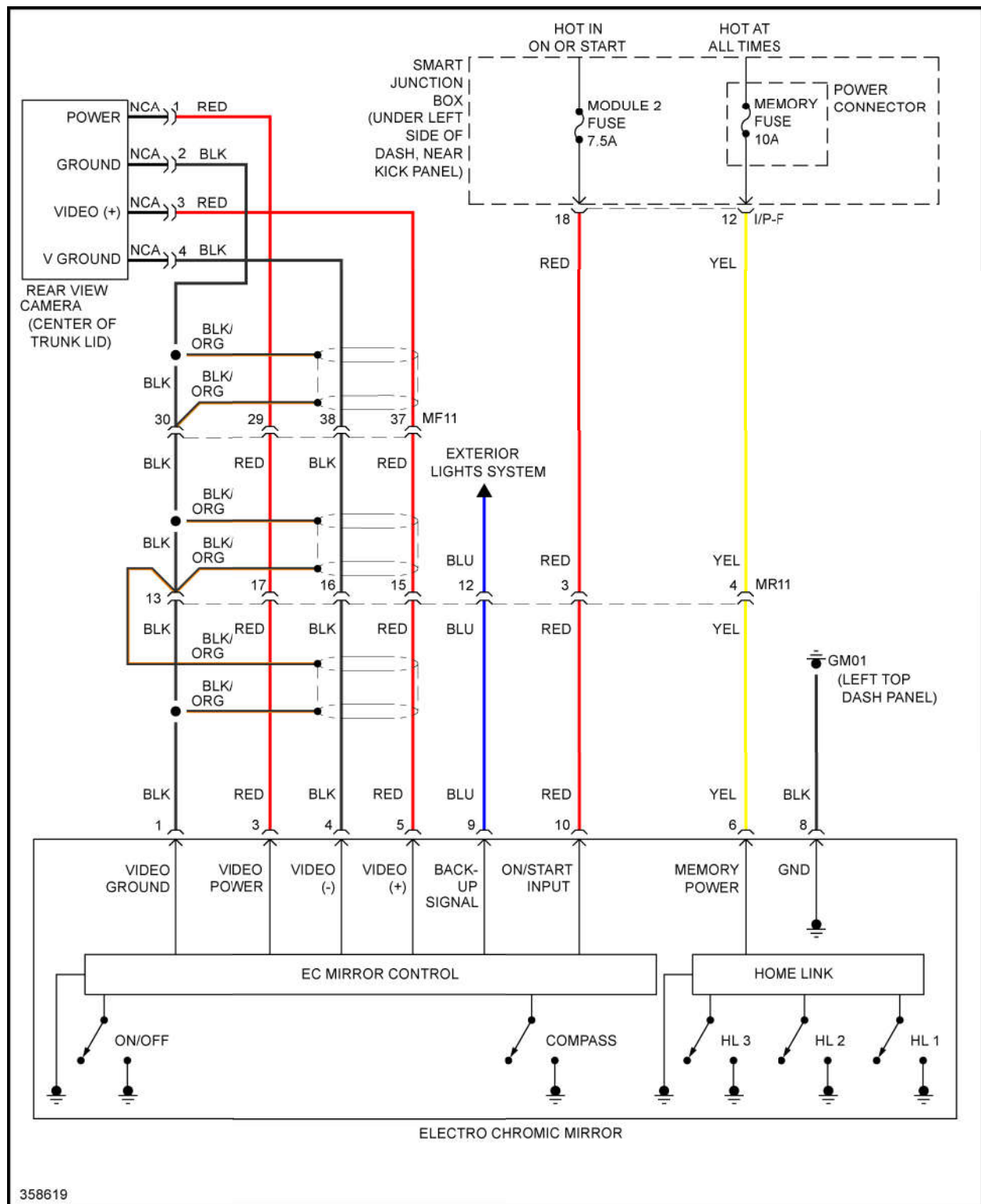
Fig. 53: Electrochromic Mirror Circuit, W/ Home Link & Rear Camera Display
