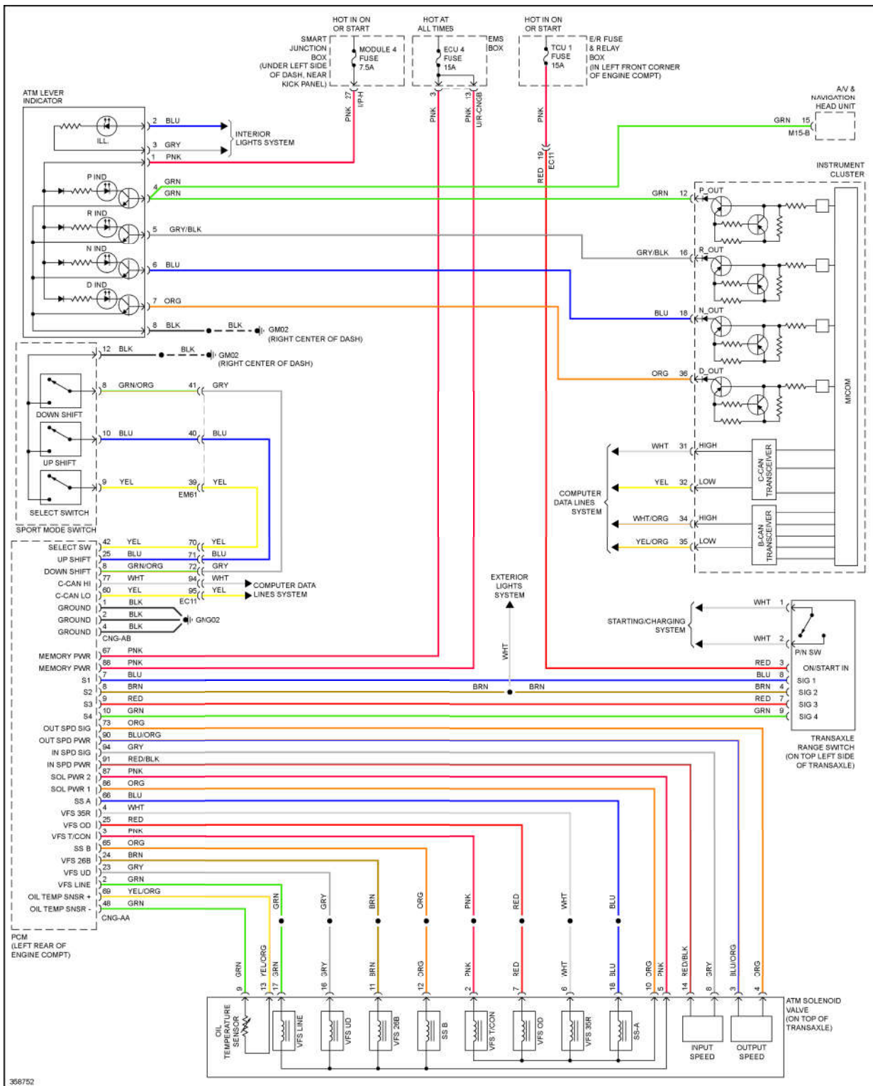
Fig. 81: Transmission Circuit
