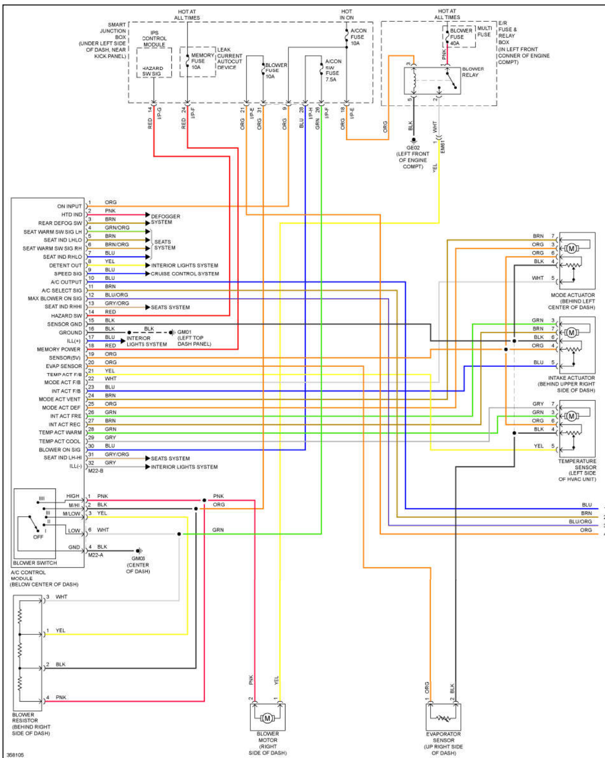
Fig. 4: Manual A/C Circuit (1 of 2)
