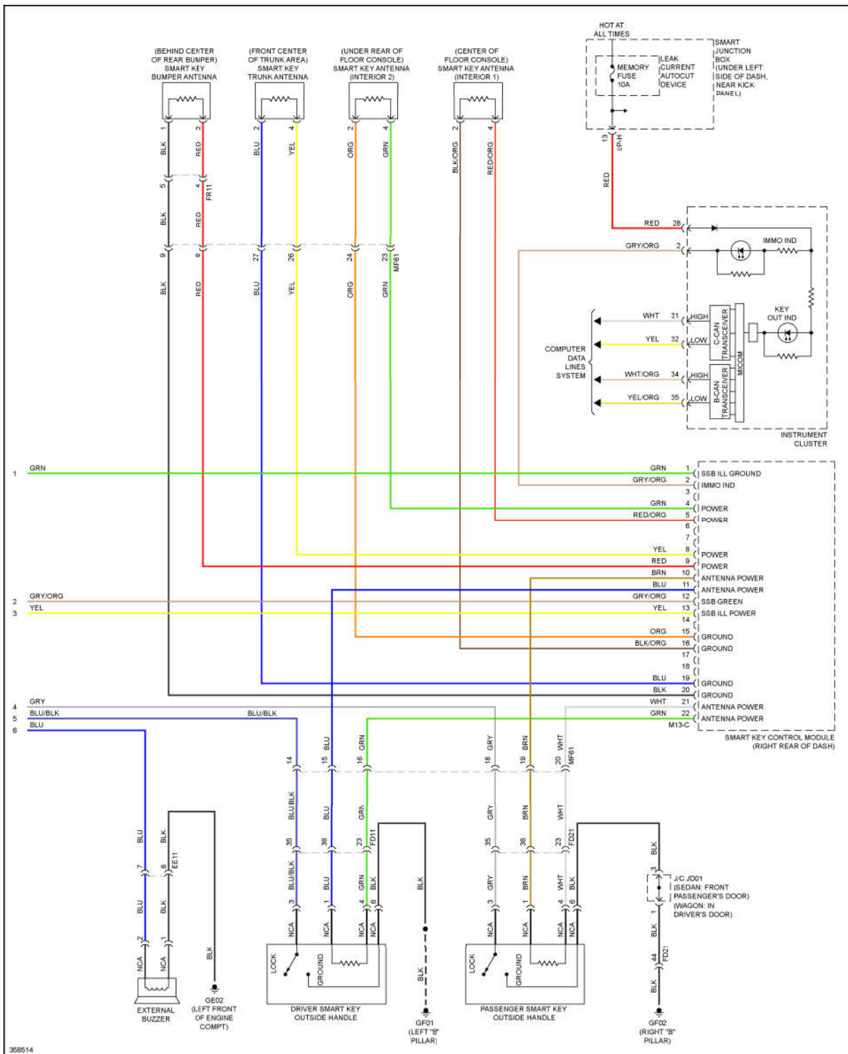
Fig. 10: Immobilizer Circuit, W/ Smart Key System (3 of 3)
