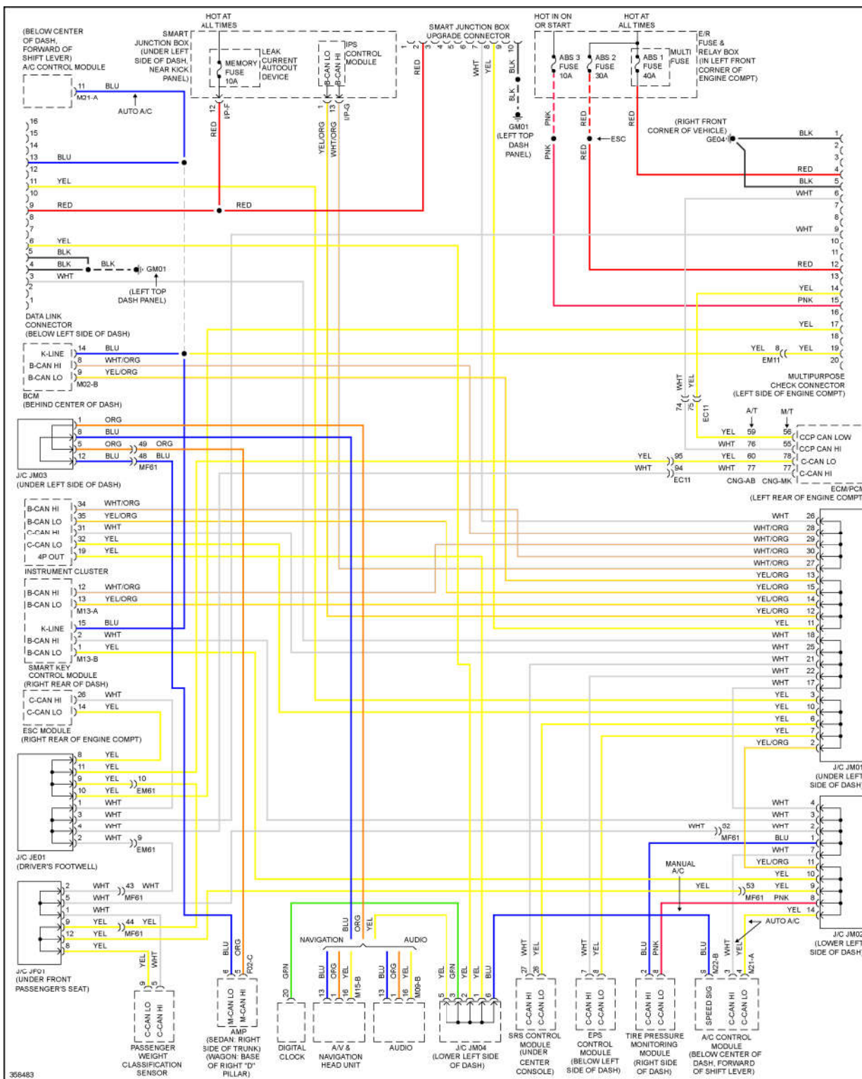
Fig. 13: Computer Data Lines Circuit
