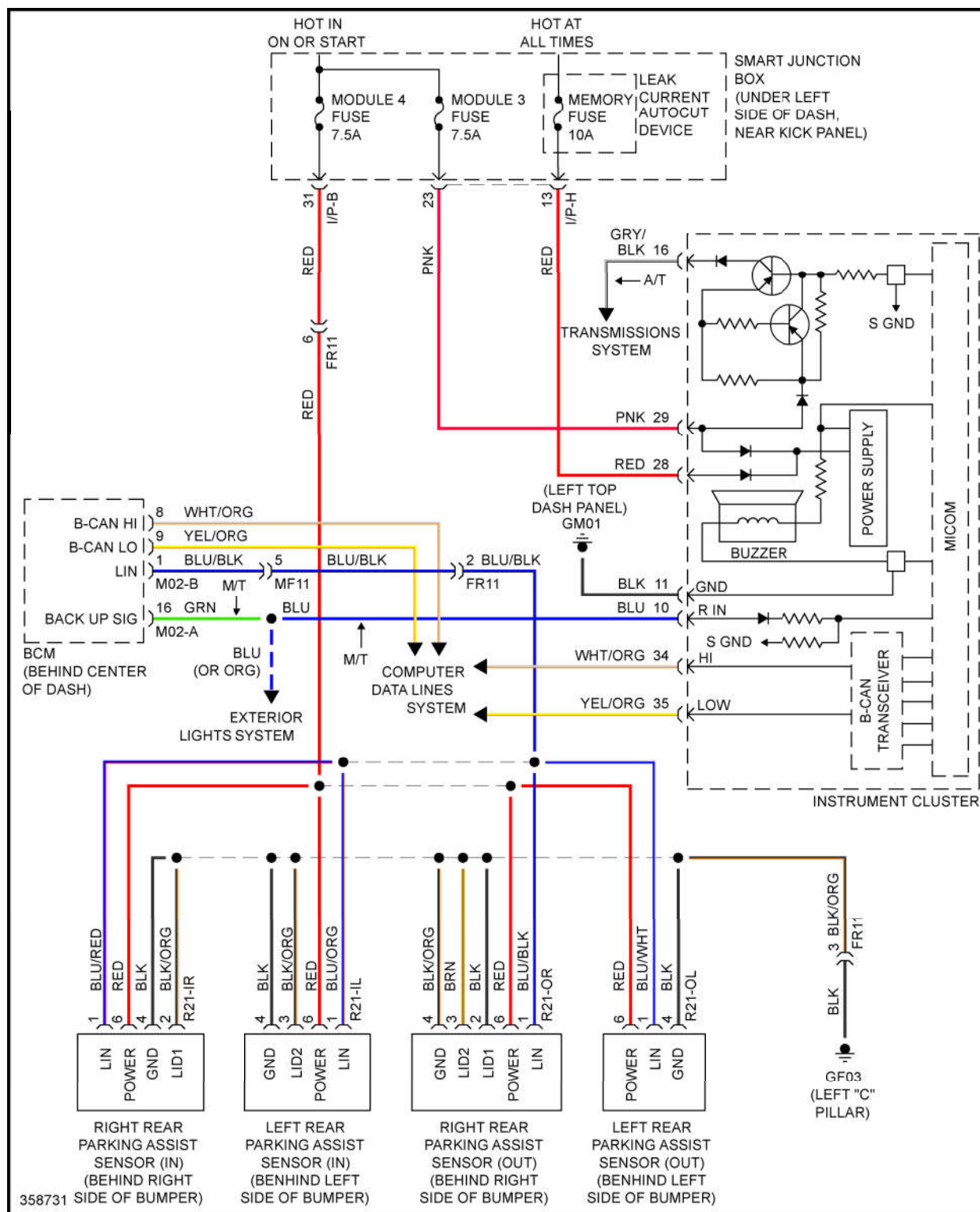
Fig. 45: Parking Assistant Circuit
