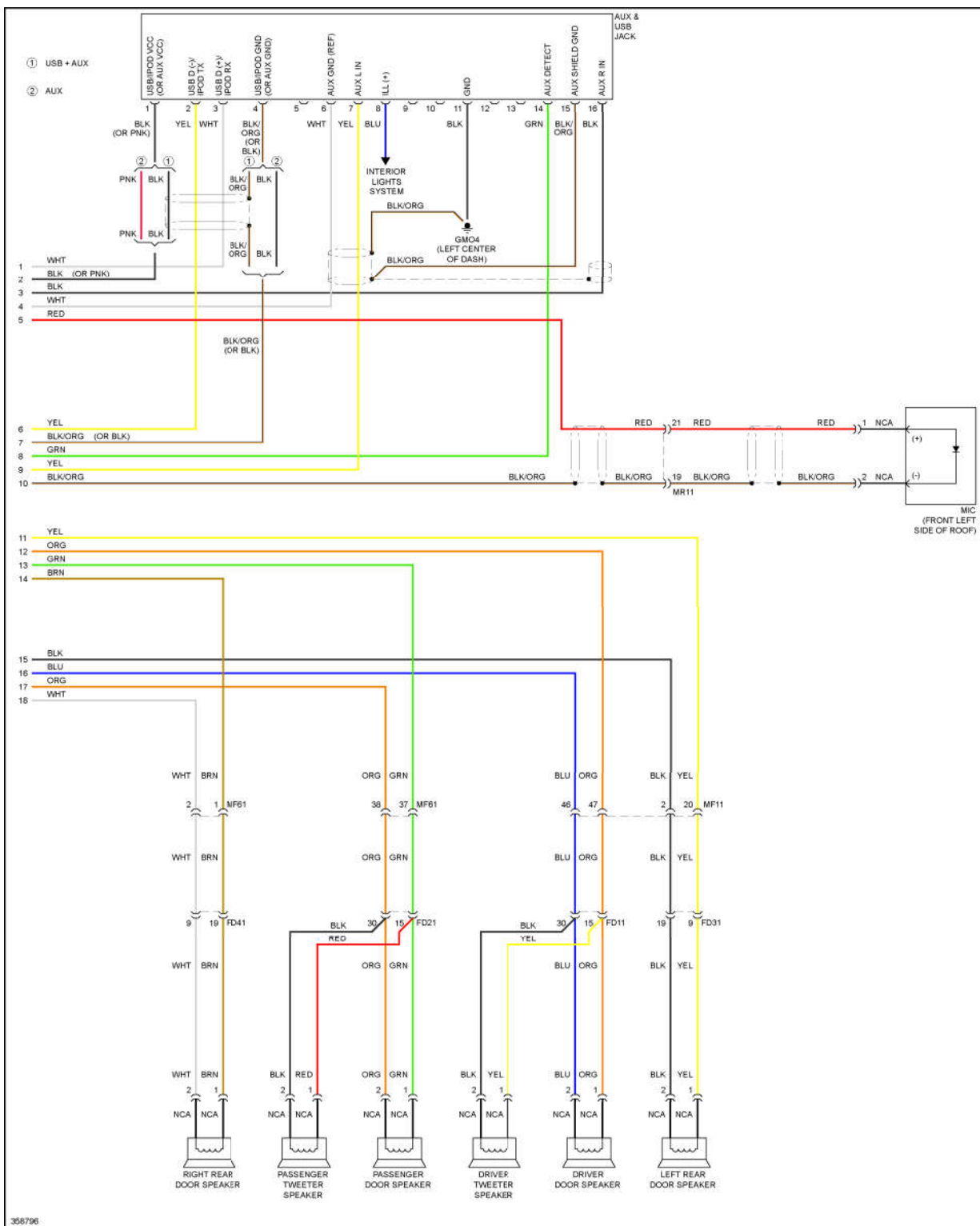
Fig. 74: Radio Circuit, W/O Amplifier (2 of 2)
