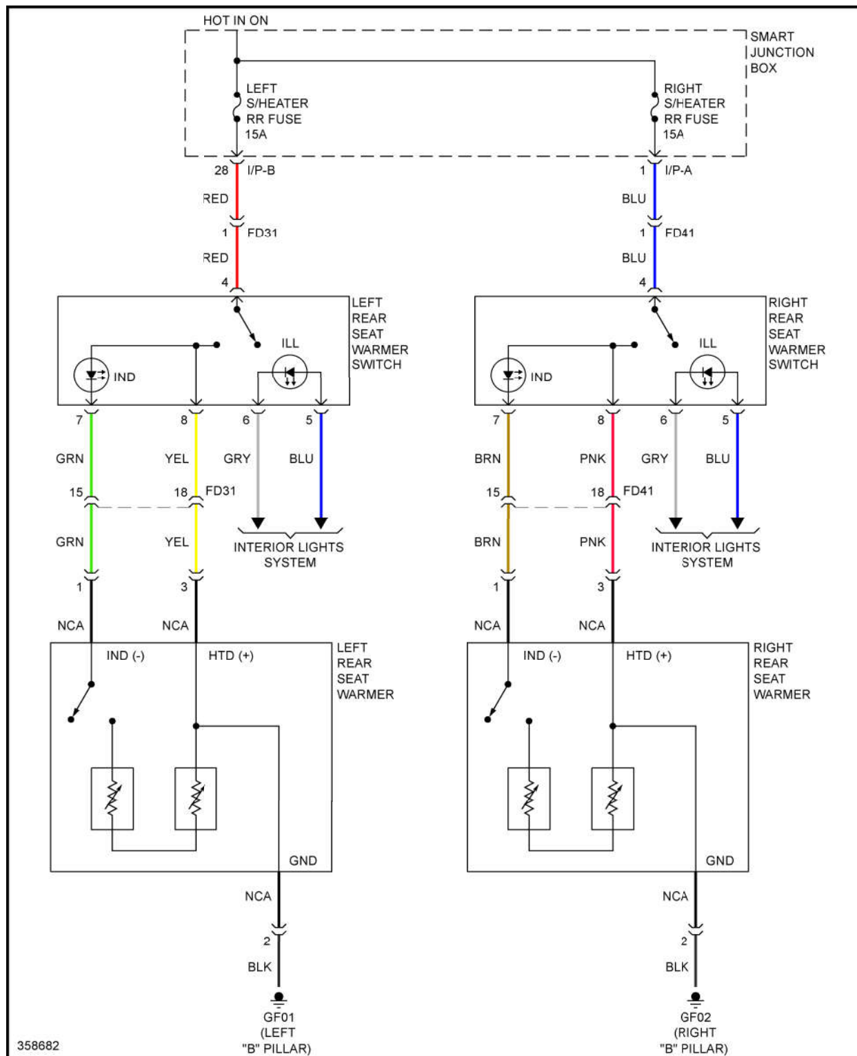
Fig. 56: Heated Seats Circuit, Rear Seat Warmer
