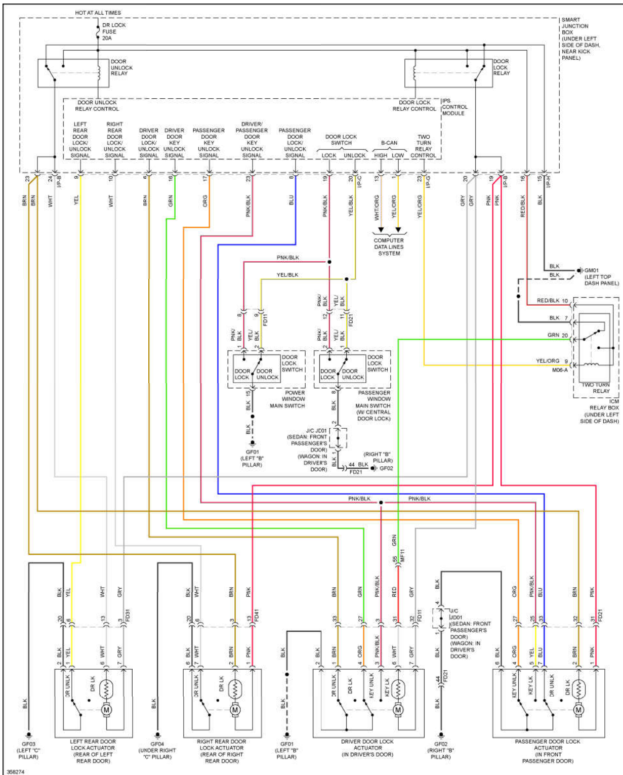
Fig. 52: Power Door Locks Circuit
