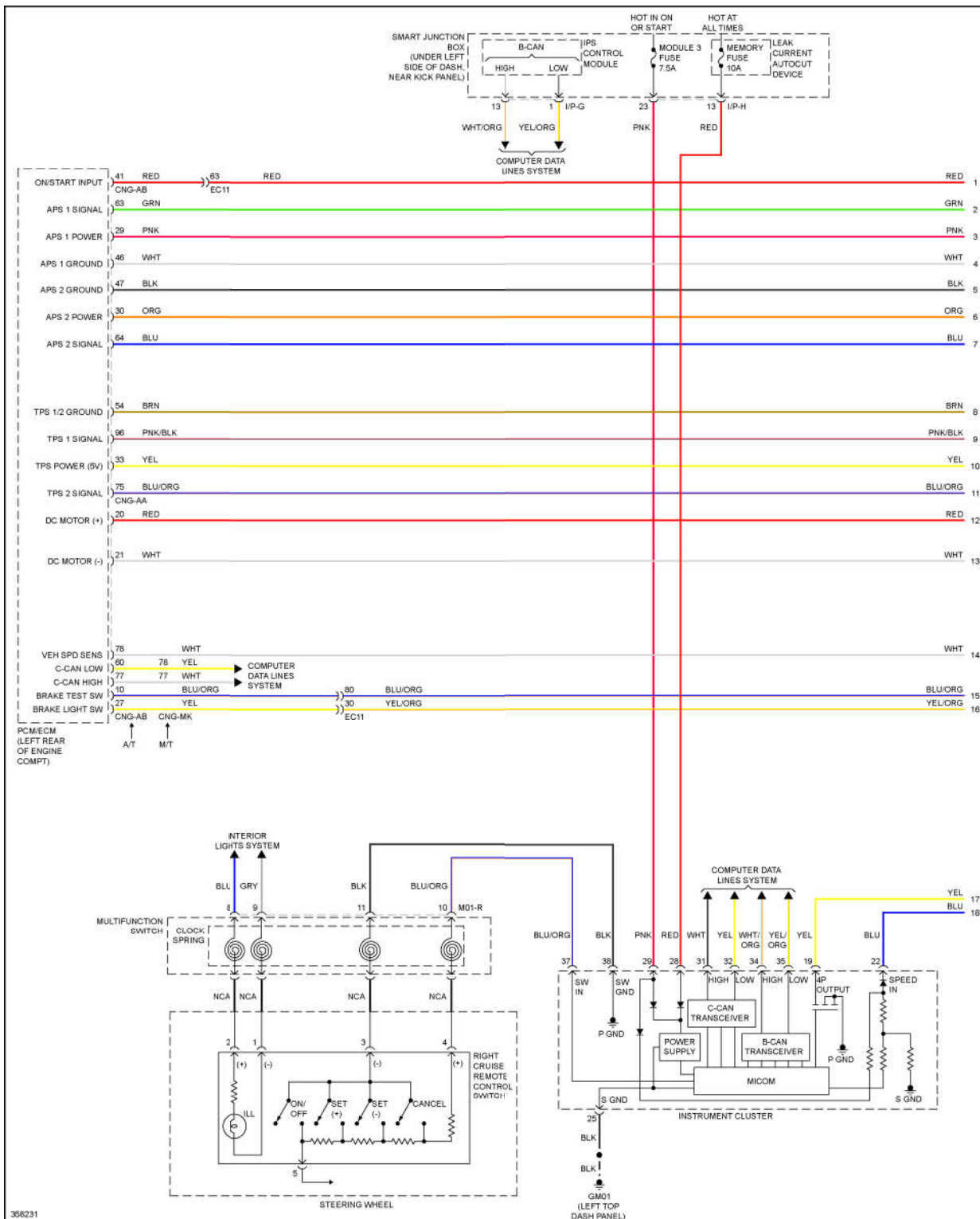
Fig. 15: Cruise Control Circuit (1 of 2)
