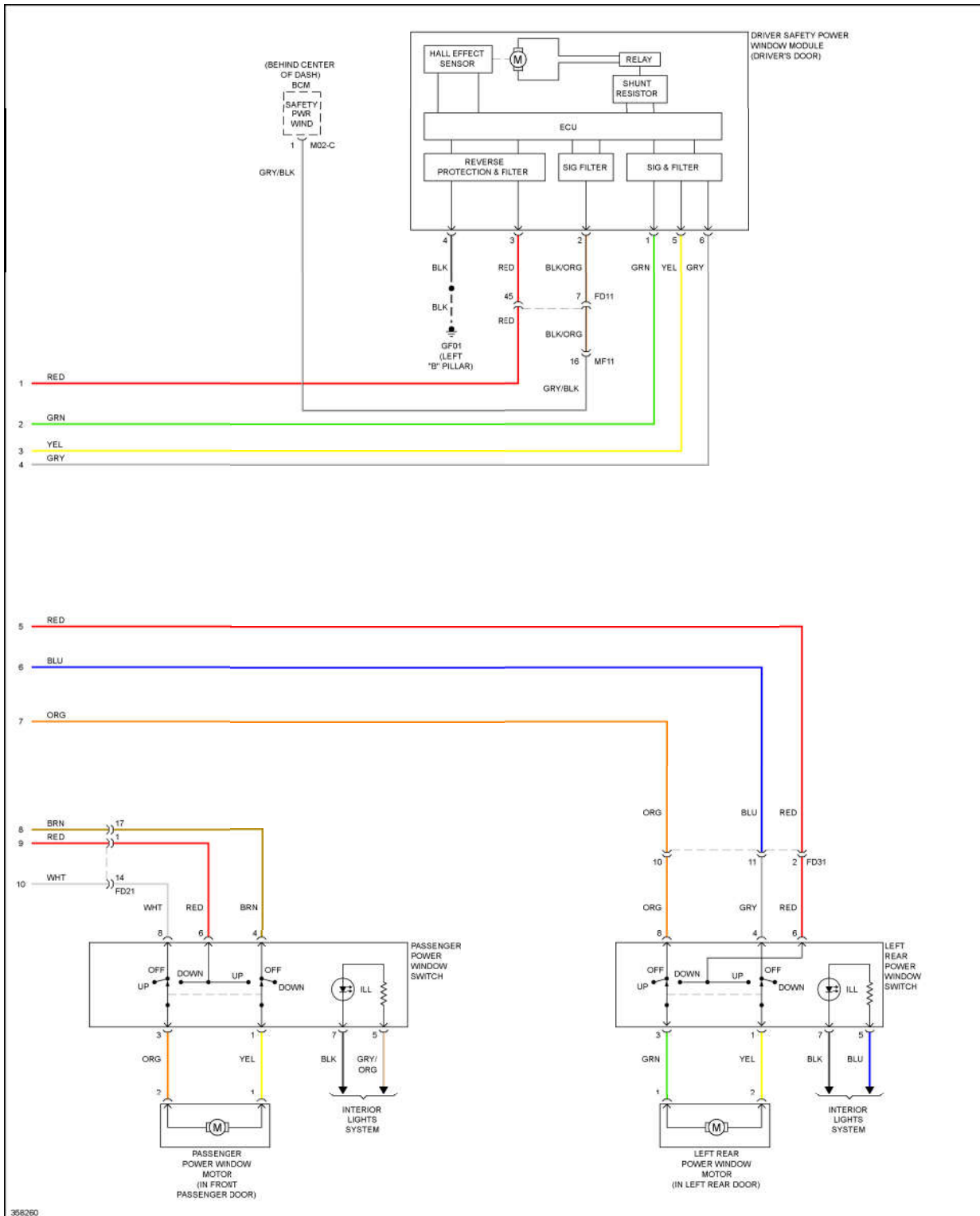
Fig. 64: Power Windows Circuit, W/ Safety Power Windows W/O Central Door Locks (2 of 2)
