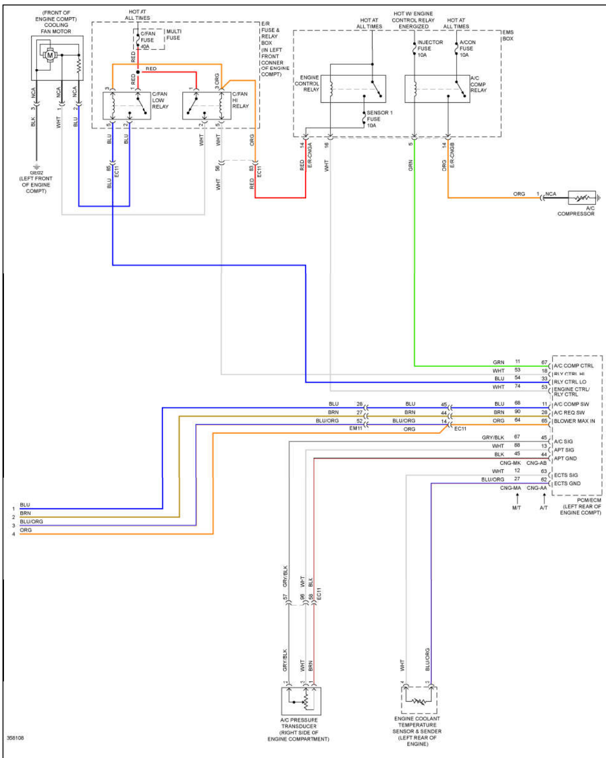
Fig. 5: Manual A/C Circuit (2 of 2)
