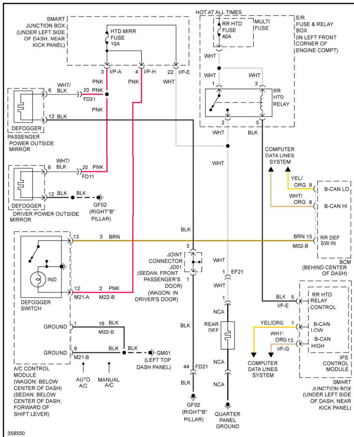
Fig. 18: Defoggers Circuit, W/O Auto Defogger
