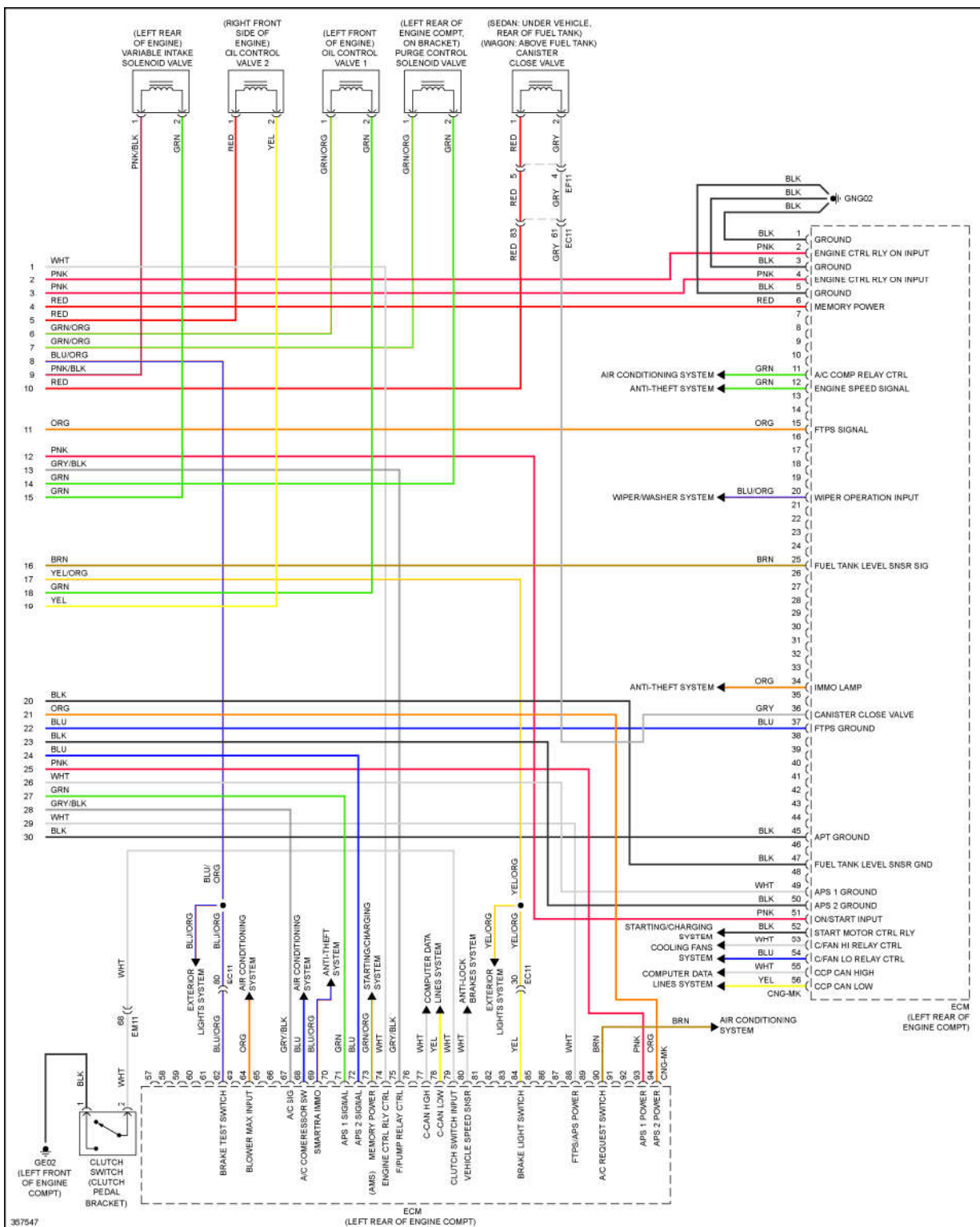
Fig. 29: 1.8L, Engine Performance Circuit, M/T (5 of 5)
