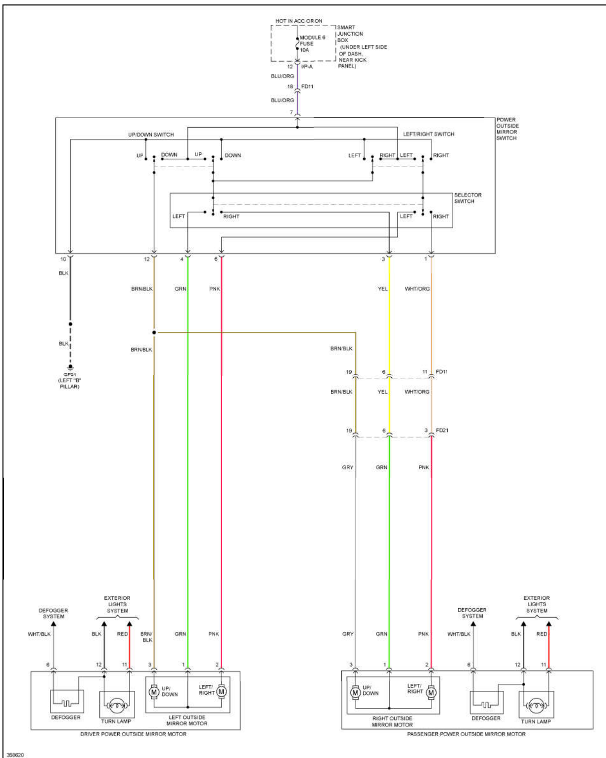
Fig. 55: Power Mirrors Circuit
