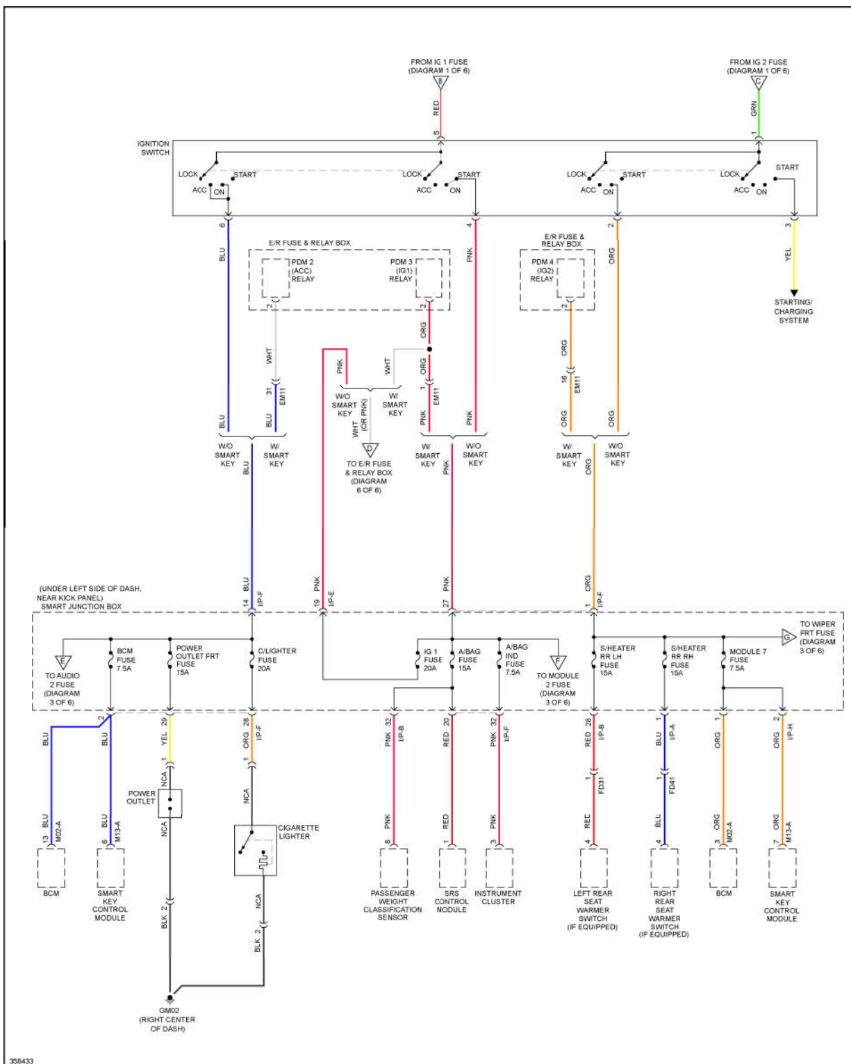
Fig. 47: Power Distribution Circuit (2 of 6)
