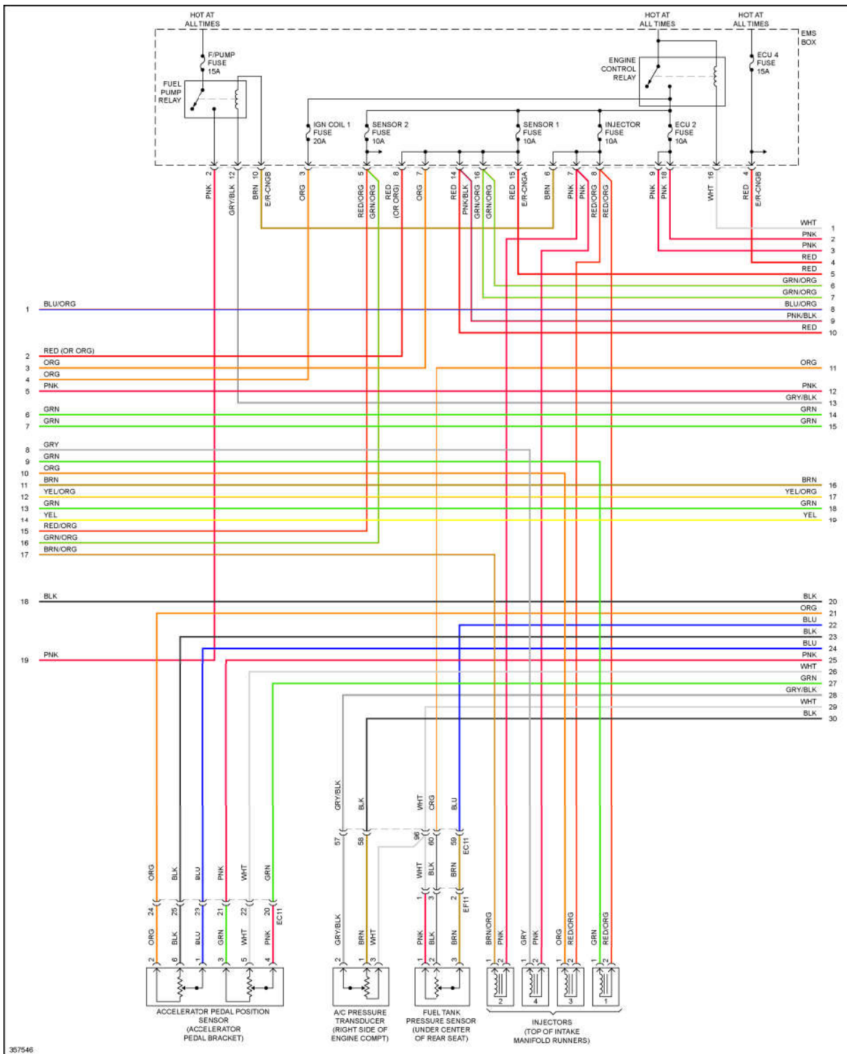
Fig. 28: 1.8L, Engine Performance Circuit, M/T (4 of 5)
