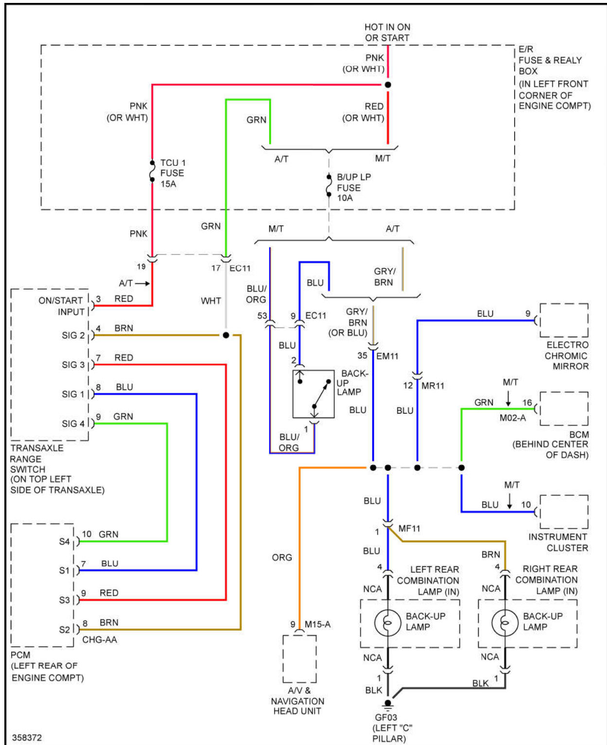
Fig. 30: Backup Lamps Circuit
