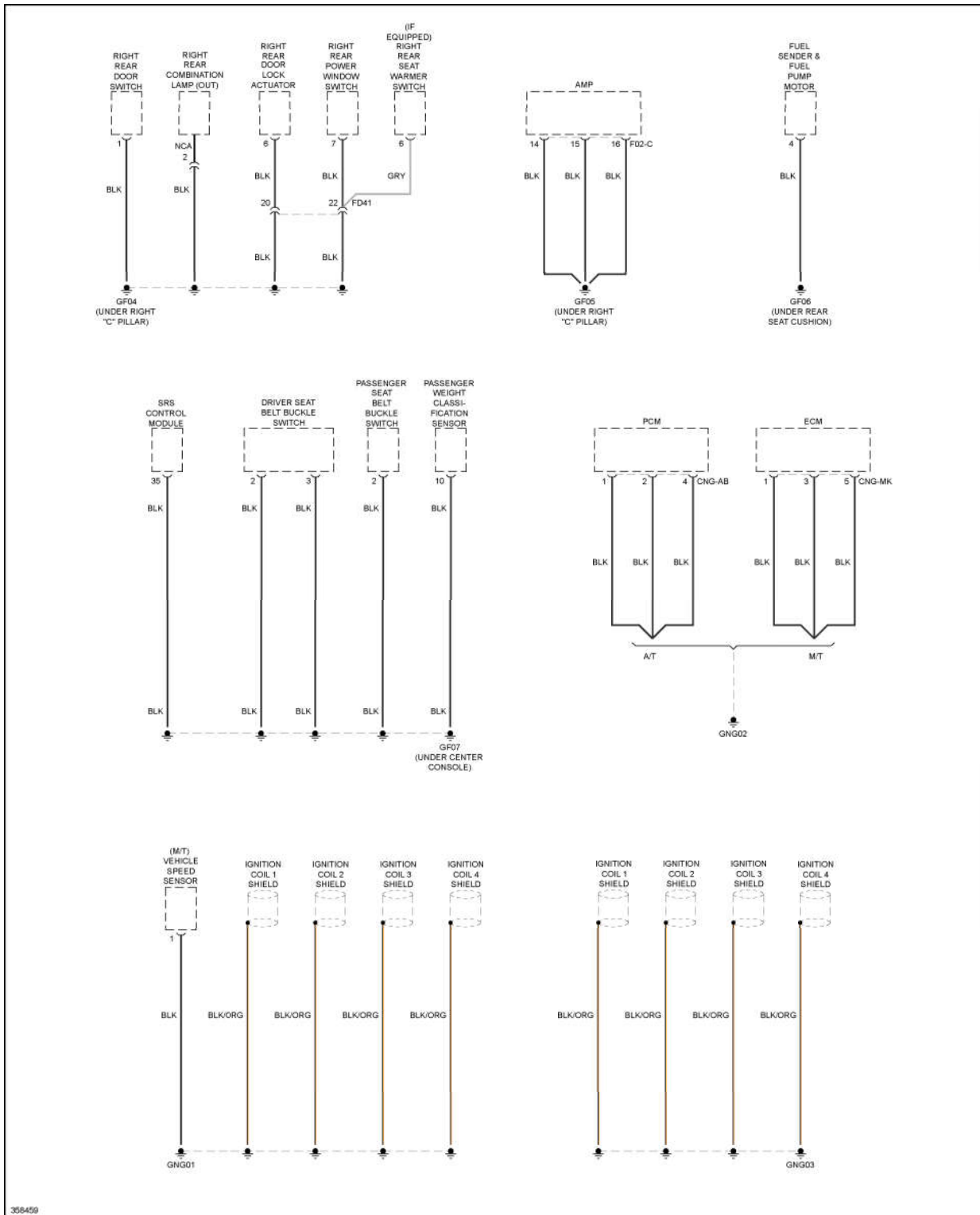
Fig. 35: Ground Distribution Circuit (3 of 3)
