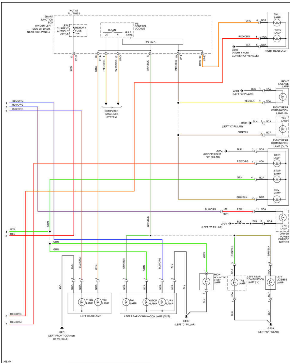
Fig. 32: Exterior Lamps Circuit (2 of 2)
