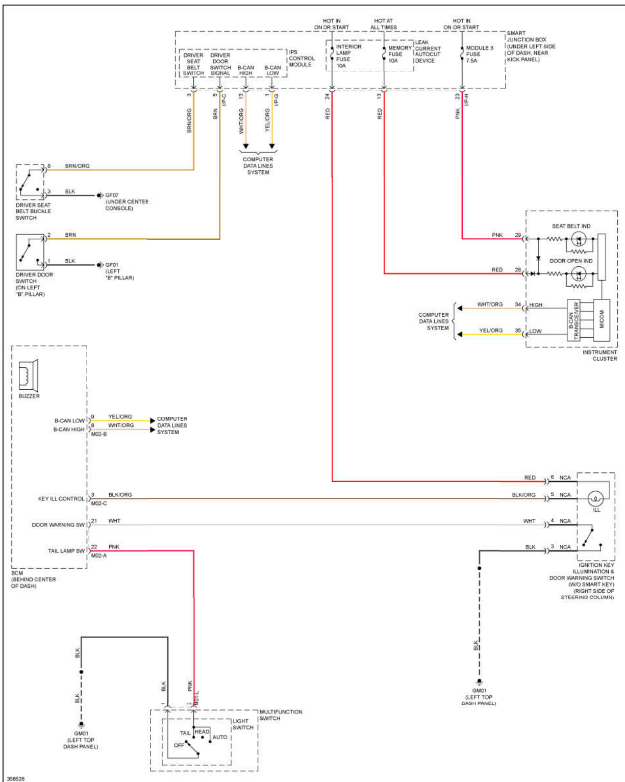
Fig. 83: Chime Circuit
