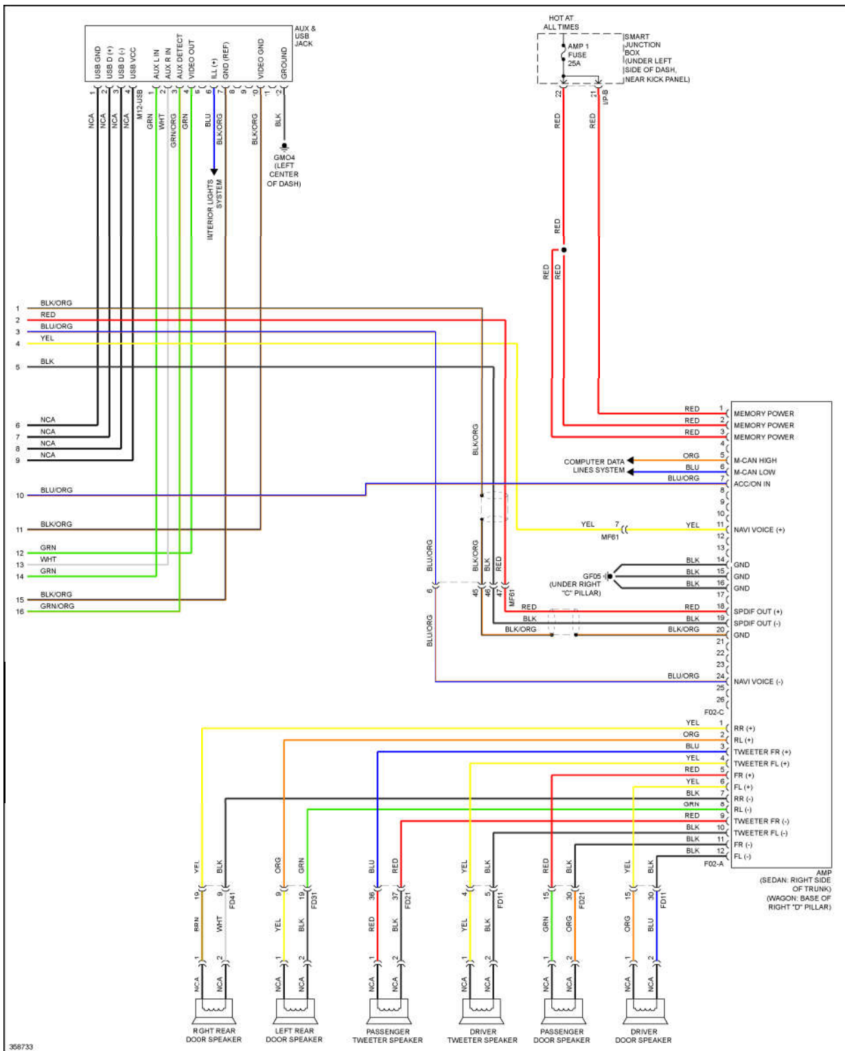
Fig. 44: Navigation Circuit (2 of 2)
