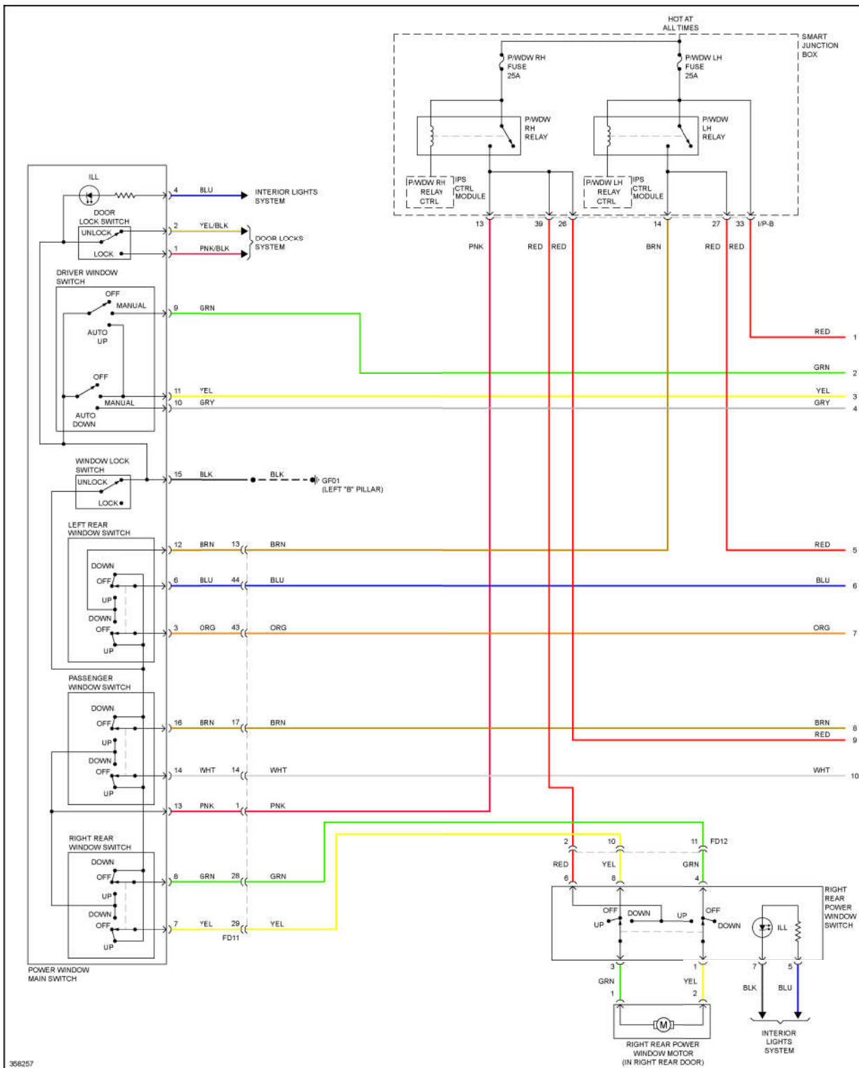
Fig. 61: Power Windows Circuit, W/ Safety Power Windows W/ Central Door Locks (1 of 2)
