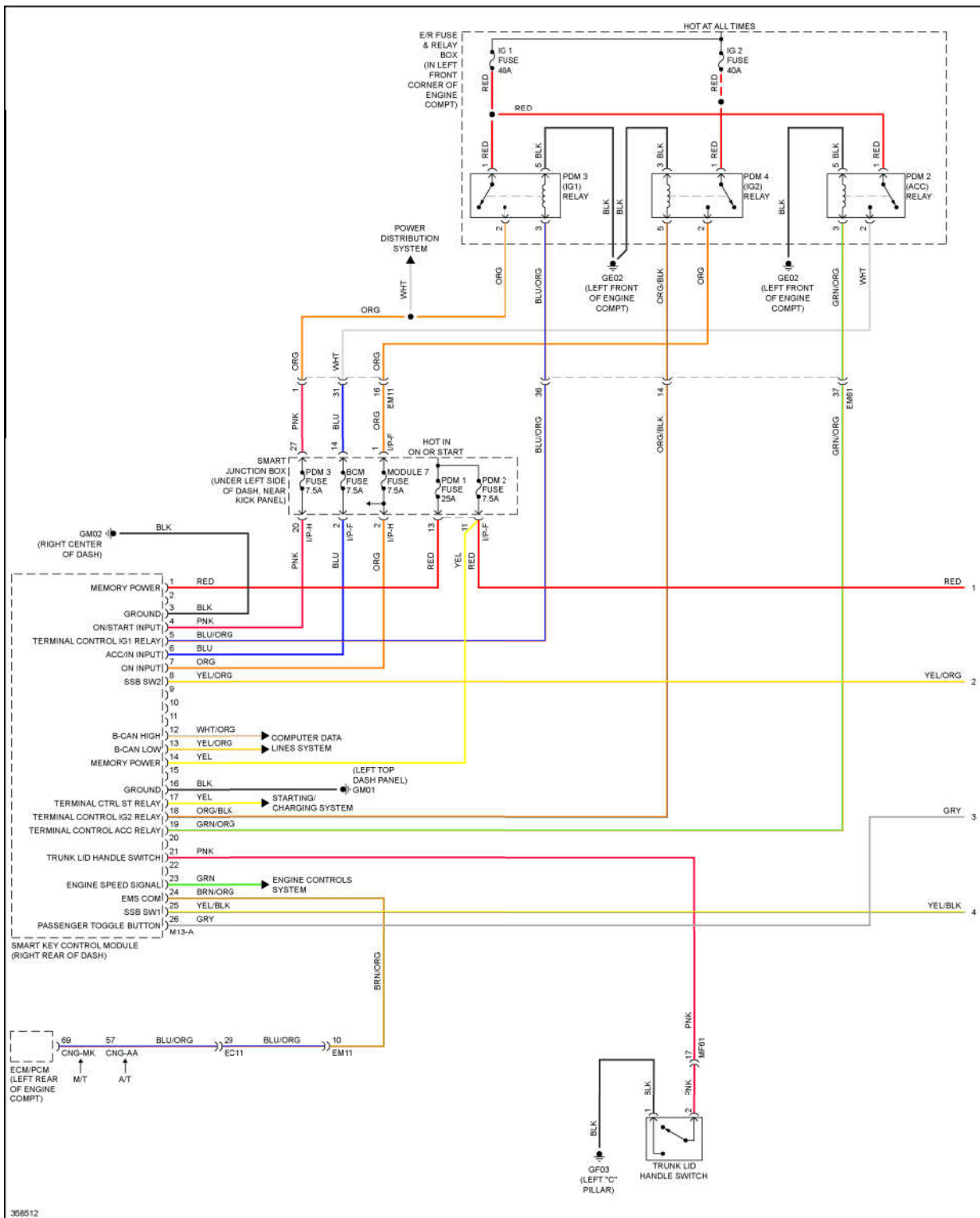
Fig. 8: Immobilizer Circuit, W/ Smart Key System (1 of 3)
