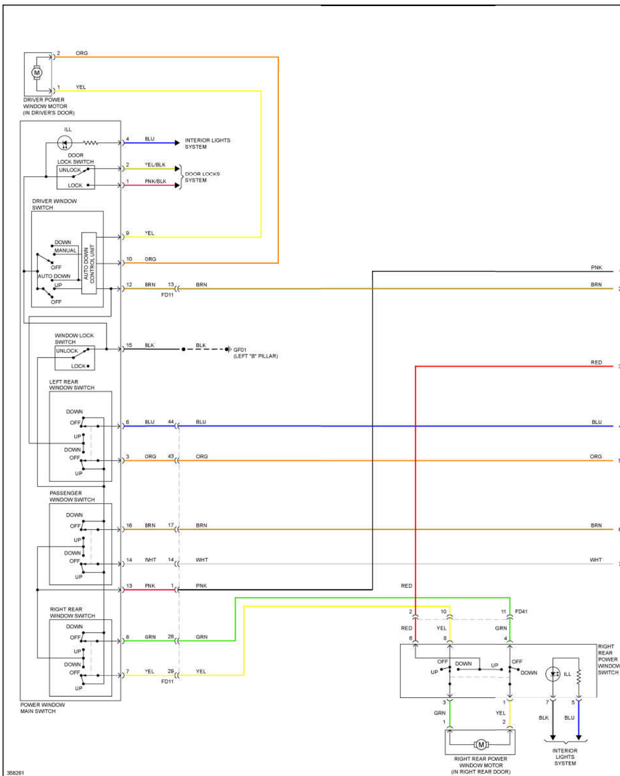
Fig. 65: Power Windows Circuit, W/O Safety Power Windows W/ Central Door Locks (1 of 2)
