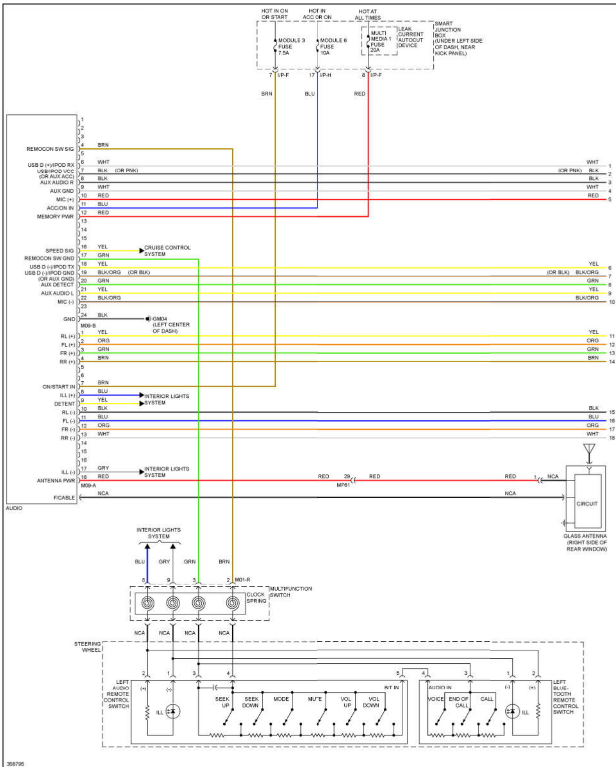
Fig. 73: Radio Circuit, W/O Amplifier (1 of 2)
