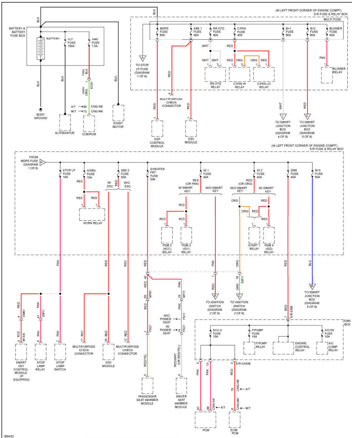
Fig. 46: Power Distribution Circuit (1 of 6)
