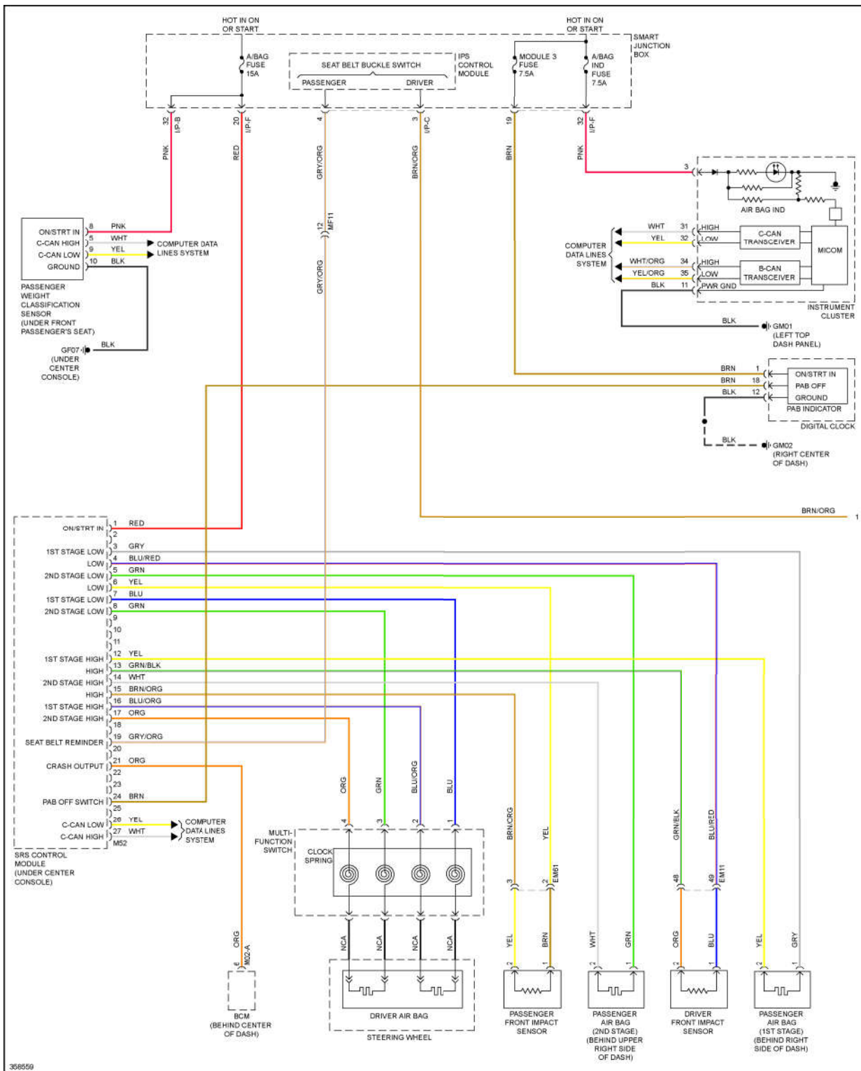
Fig. 79: Supplemental Restraints Circuit (1 of 2)
