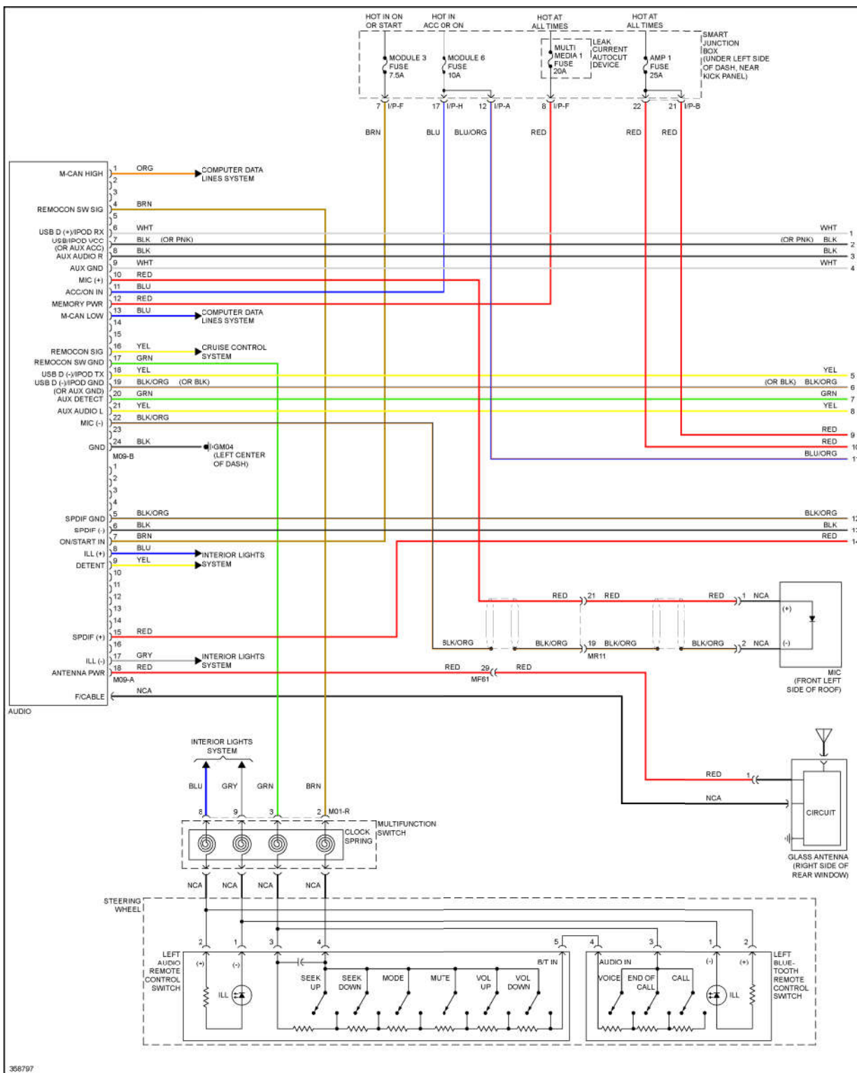
Fig. 69: Radio Circuit, W/ Amplifier (1 of 2)
