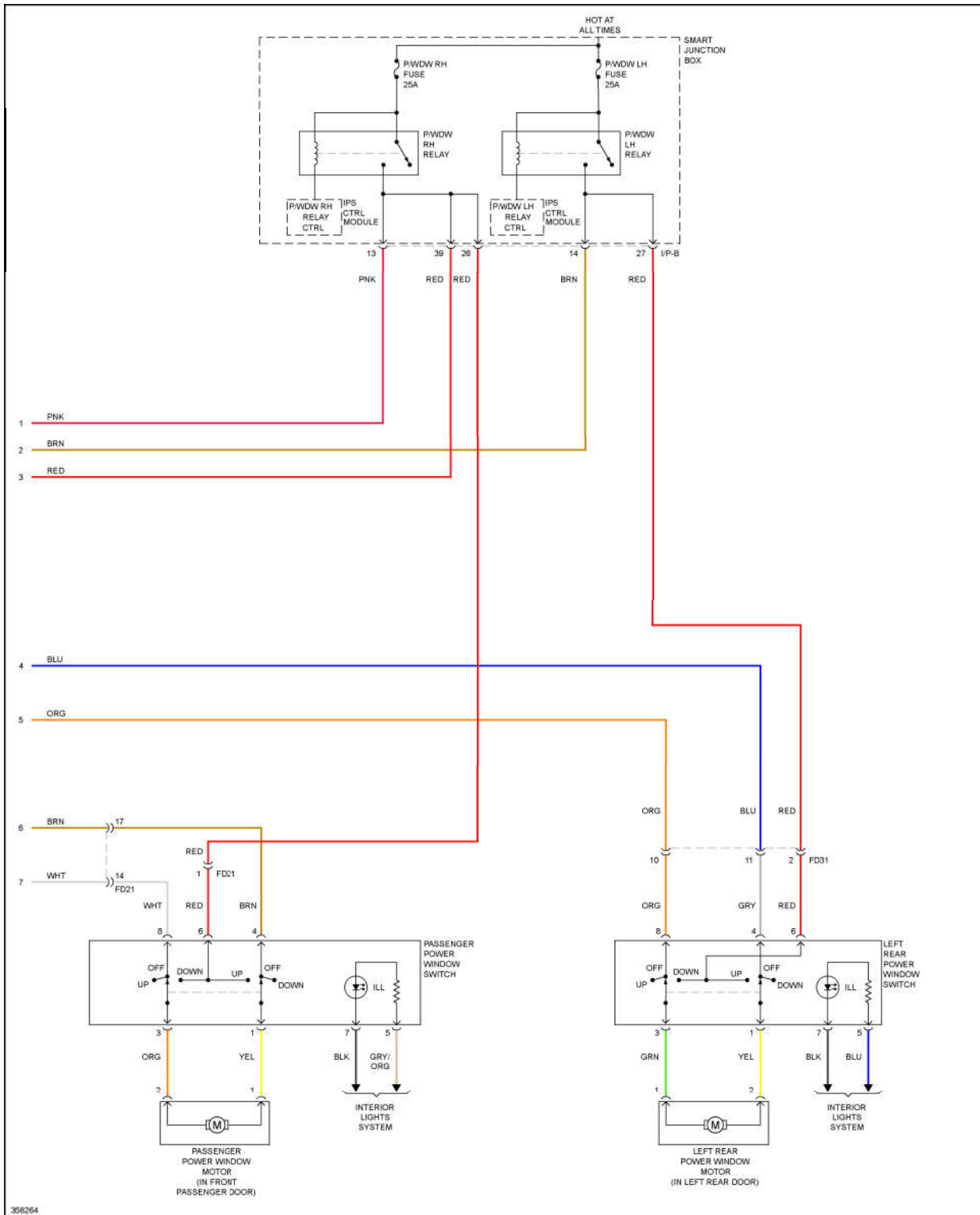
Fig. 68: Power Windows Circuit, W/O Safety Power Windows W/O Central Door Locks (2 of 2)
