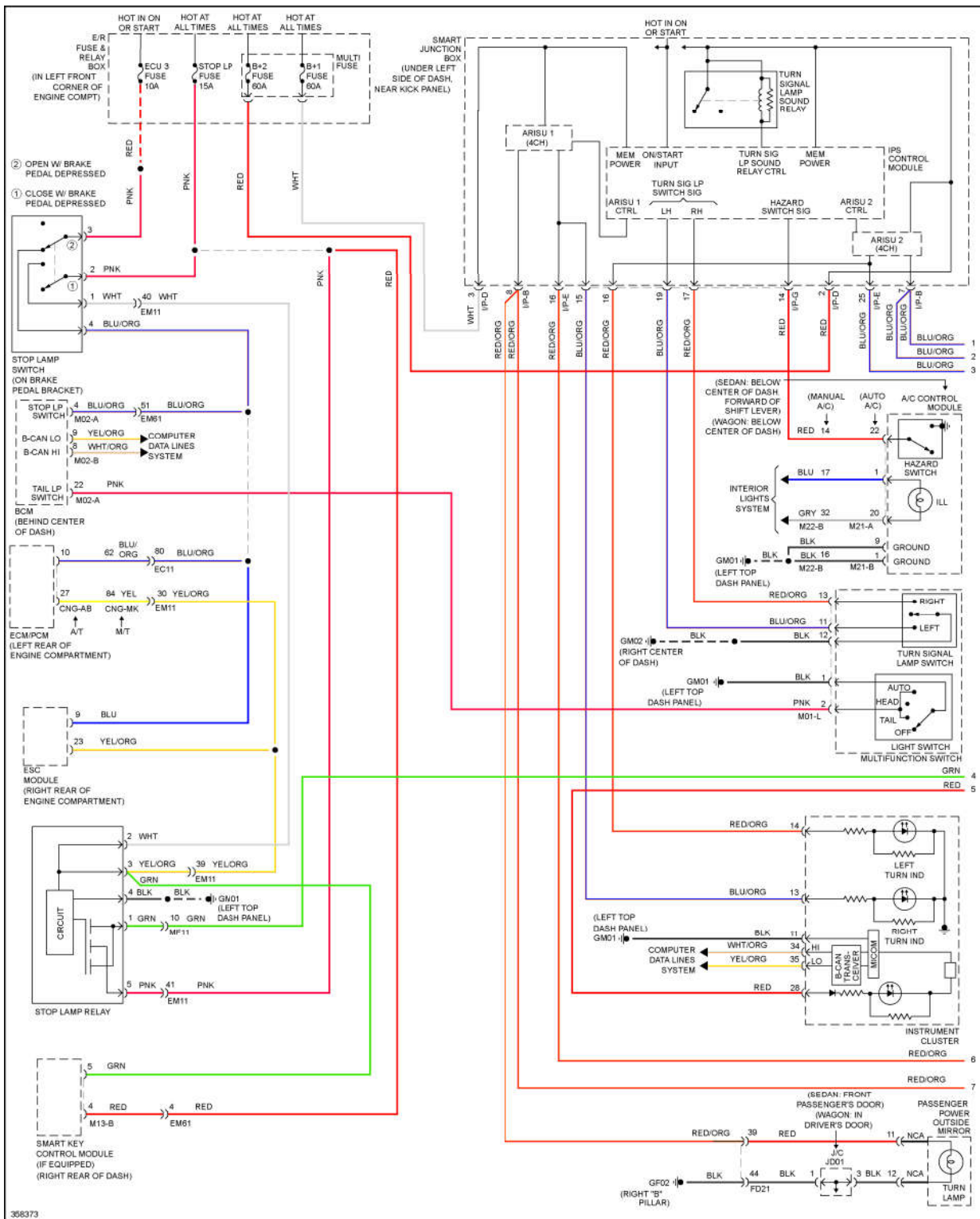
Fig. 31: Exterior Lamps Circuit (1 of 2)
