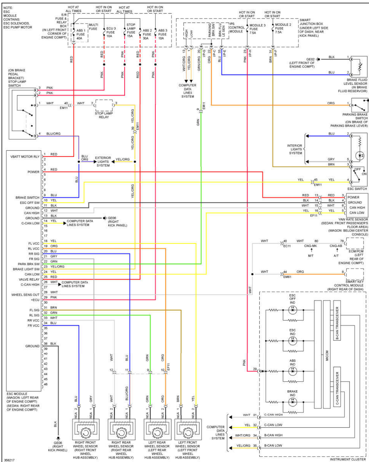
Fig. 6: Anti-lock Brakes Circuit
