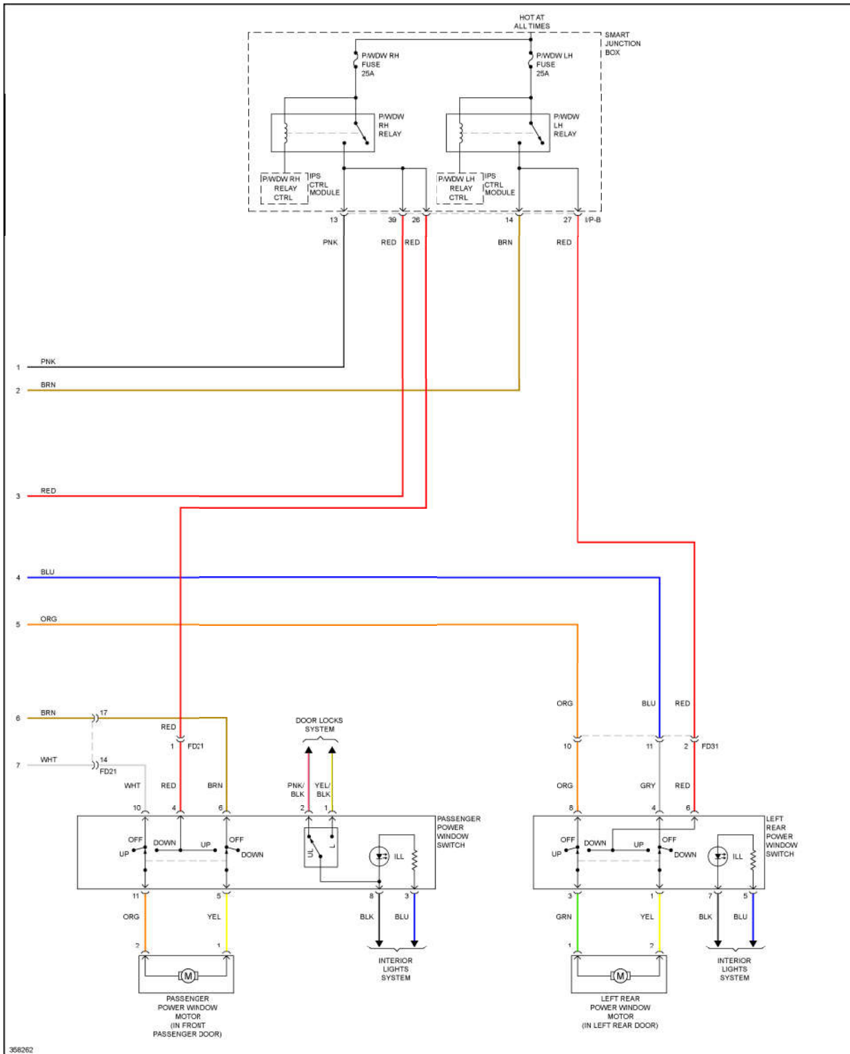
Fig. 66: Power Windows Circuit, W/O Safety Power Windows W/ Central Door Locks (2 of 2)
