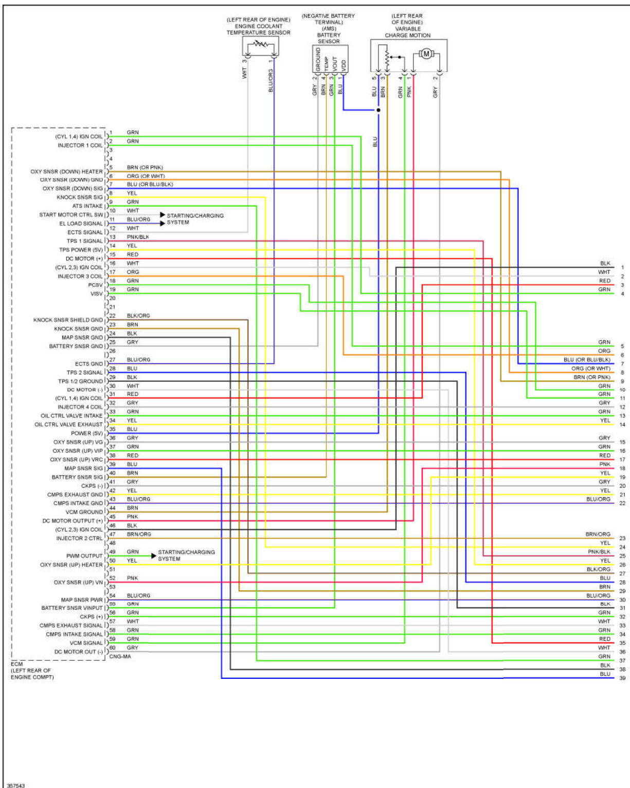
Fig. 25: 1.8L, Engine Performance Circuit, M/T (1 of 5)
