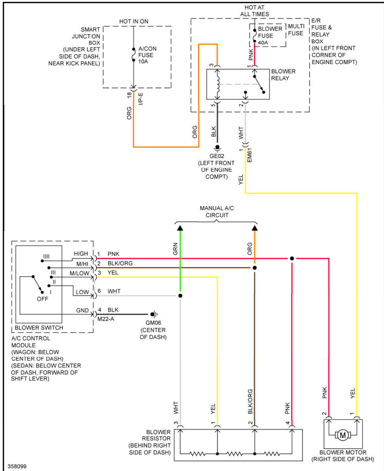
Fig. 3: Heater Circuit
