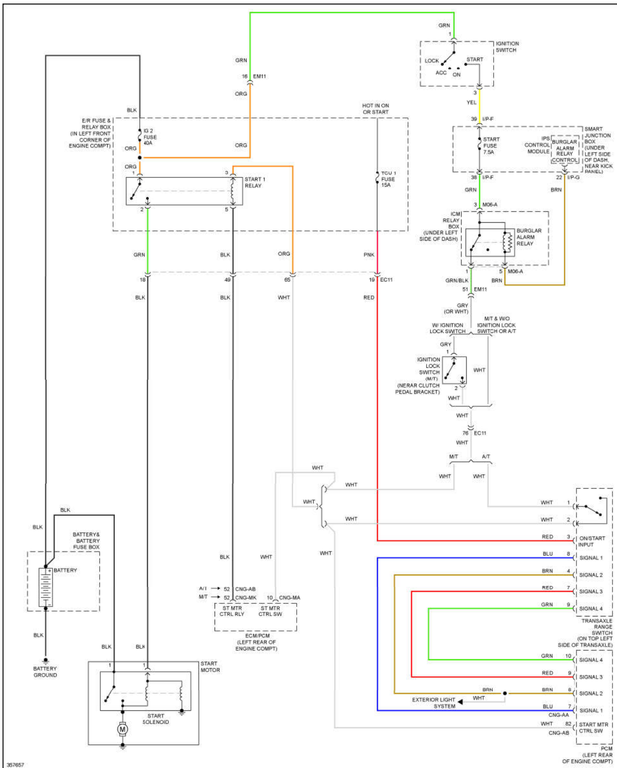
Fig. 78: Starting Circuit, W/O Smart Key & IMMO
