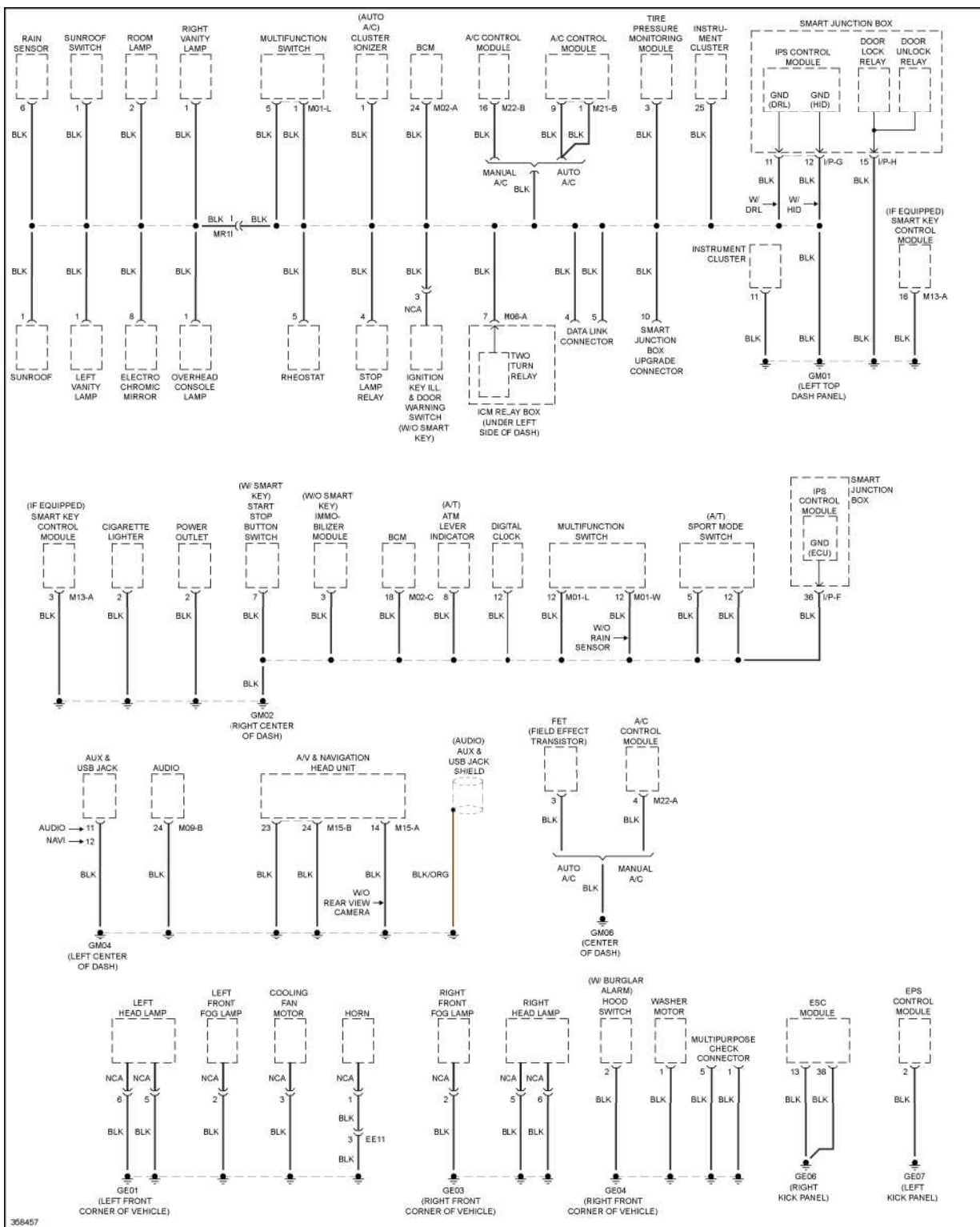
Fig. 33: Ground Distribution Circuit (1 of 3)
