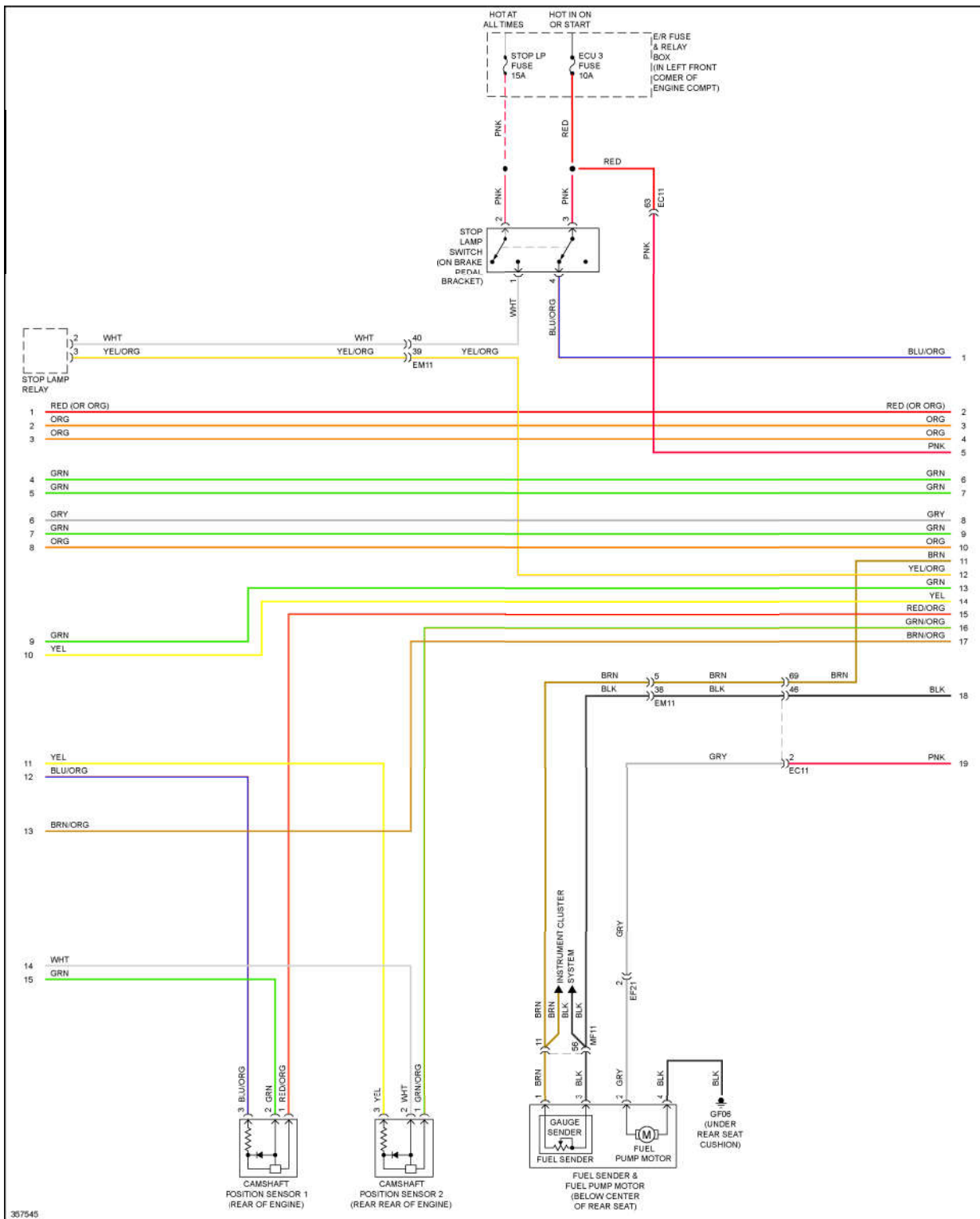
Fig. 27: 1.8L, Engine Performance Circuit, M/T (3 of 5)
