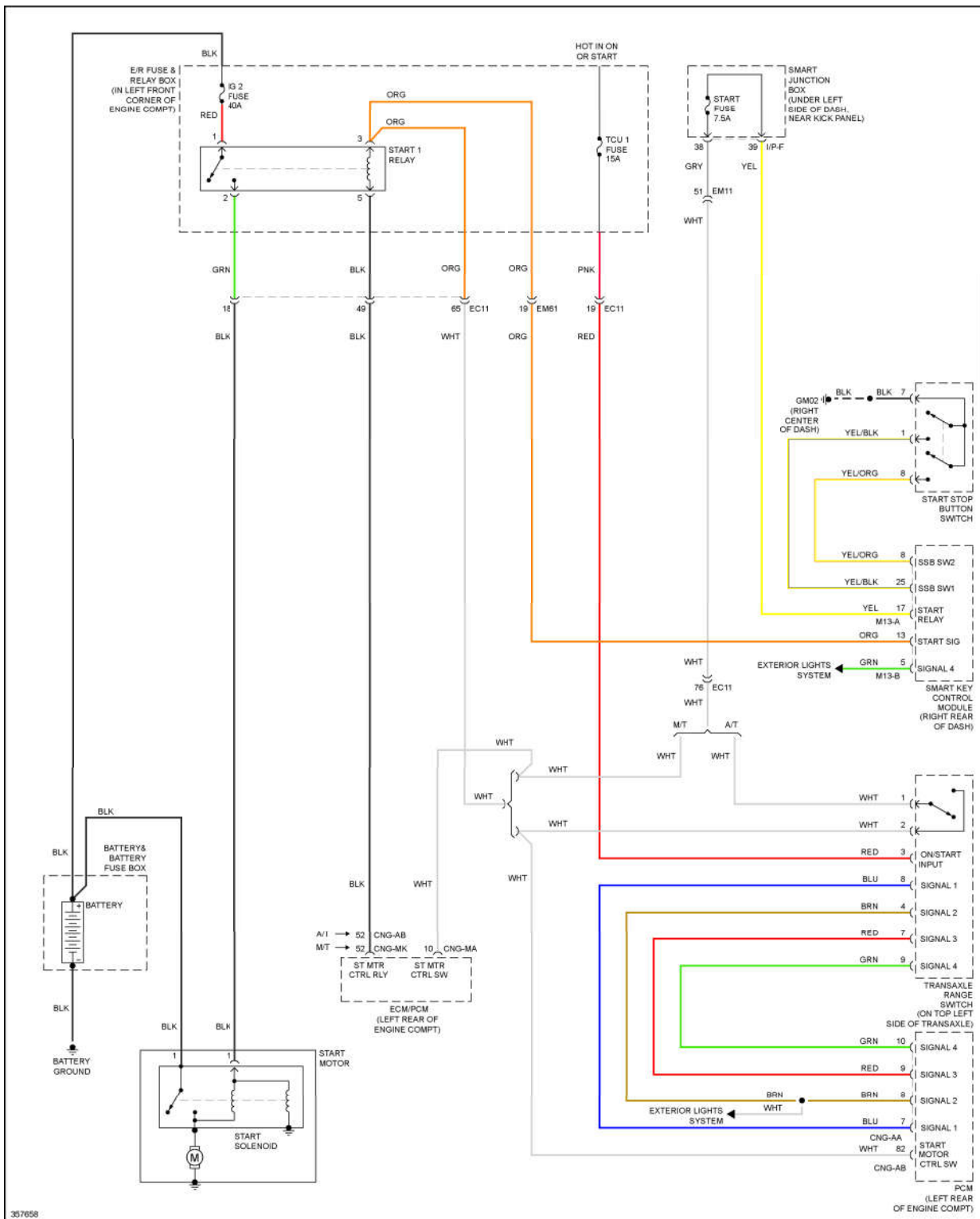
Fig. 77: Starting Circuit, W/ Smart Key & IMMO
