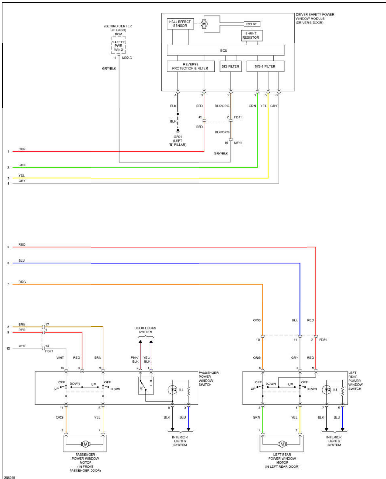
Fig. 62: Power Windows Circuit, W/ Safety Power Windows W/ Central Door Locks (2 of 2)
