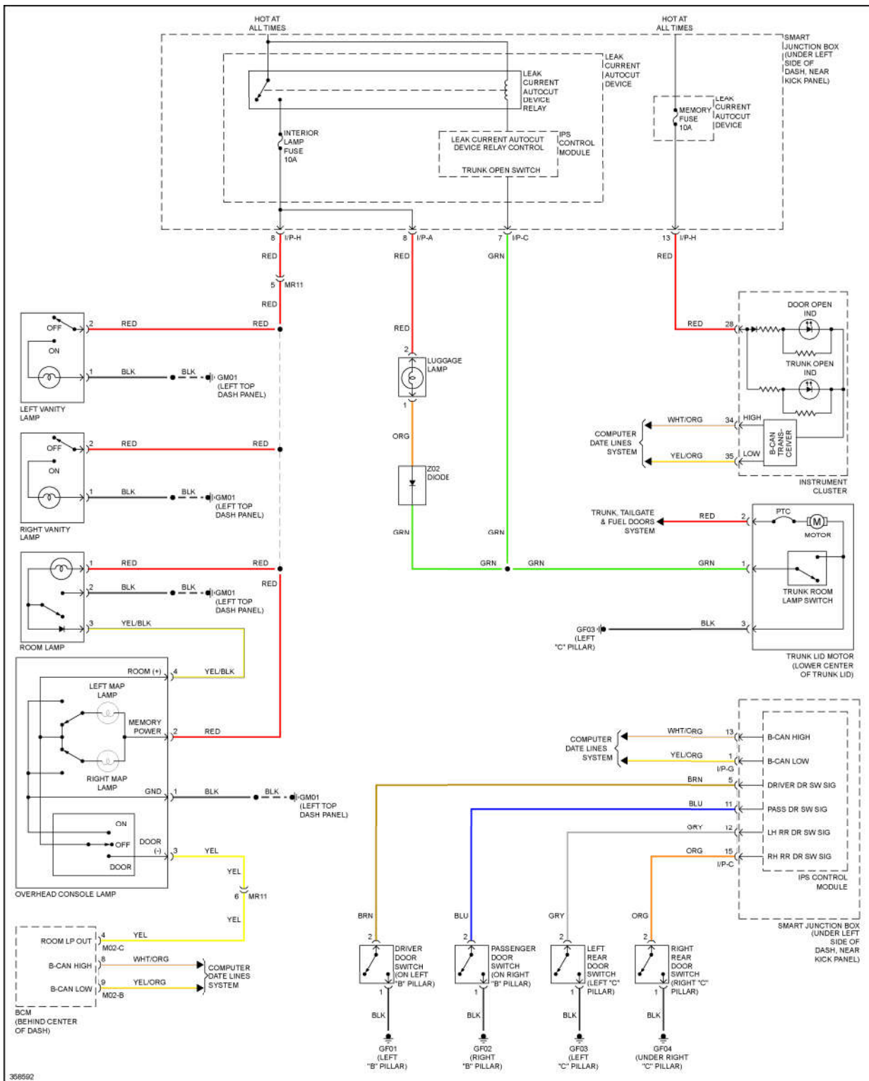
Fig. 40: Courtesy Lamps Circuit
