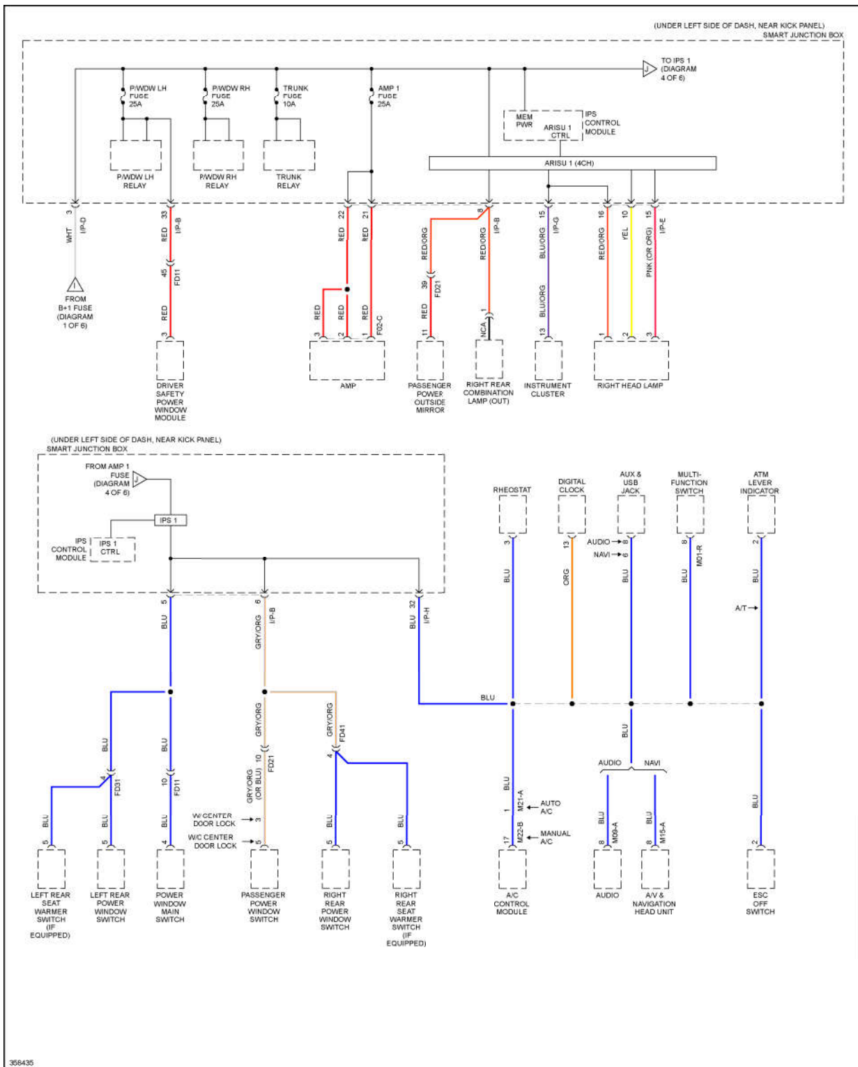
Fig. 49: Power Distribution Circuit (4 of 6)
