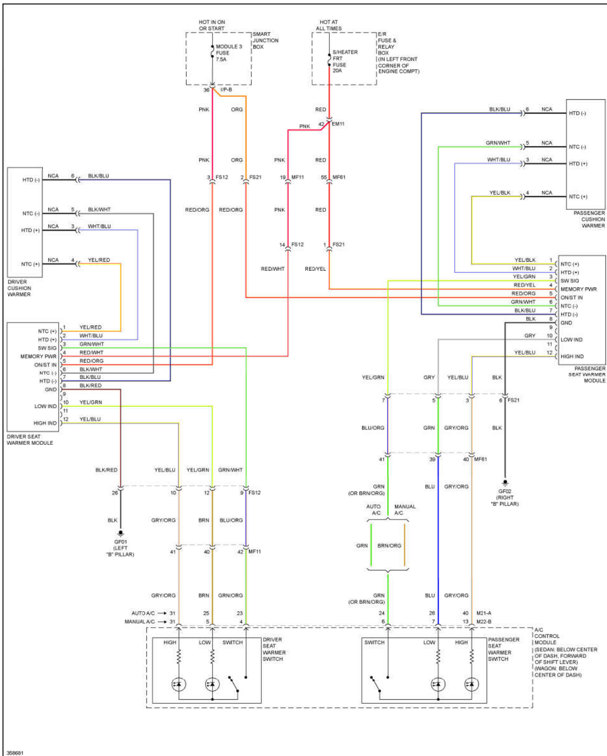
Fig. 57: Heated Seats Circuit, W/ Power Seats
