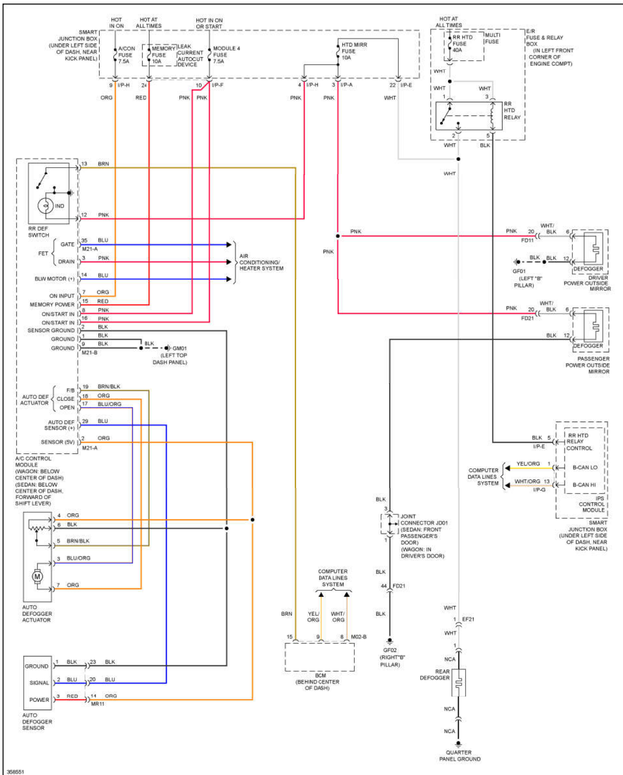
Fig. 17: Defoggers Circuit, W/ Auto Defogger
