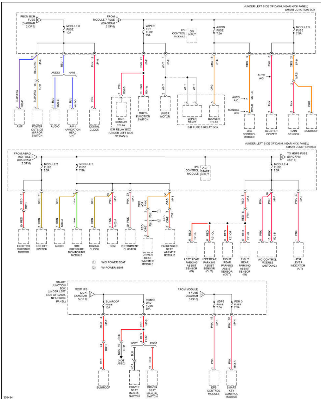
Fig. 48: Power Distribution Circuit (3 of 6)
