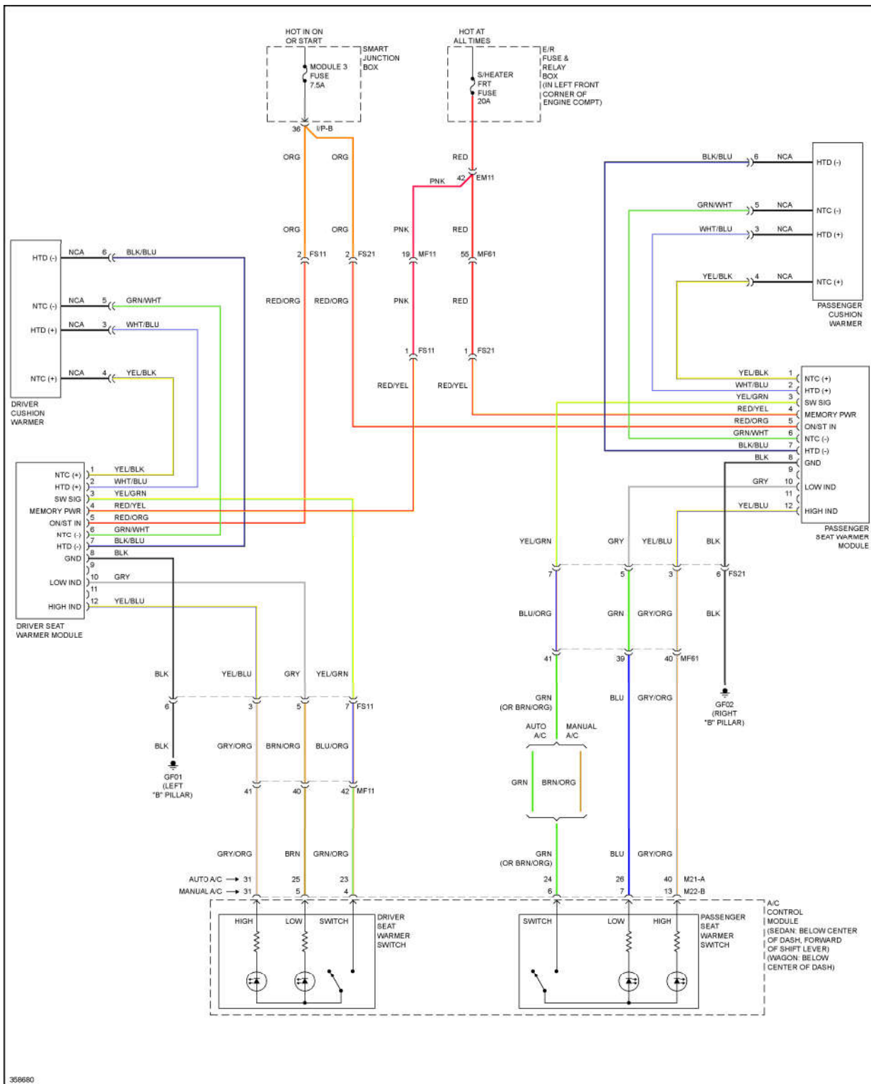
Fig. 58: Heated Seats Circuit, W/O Power Seats
