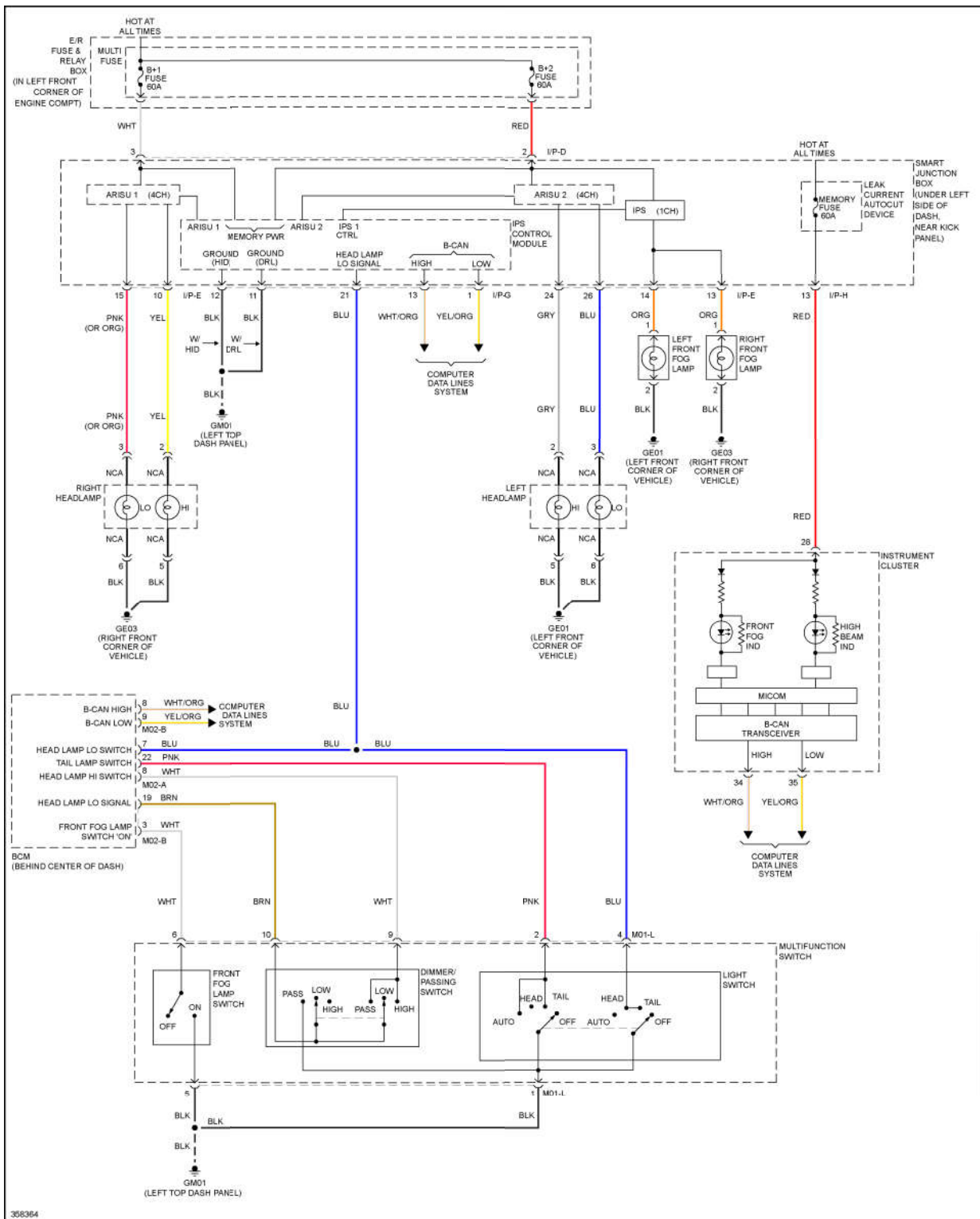
Fig. 36: Headlights Circuit
