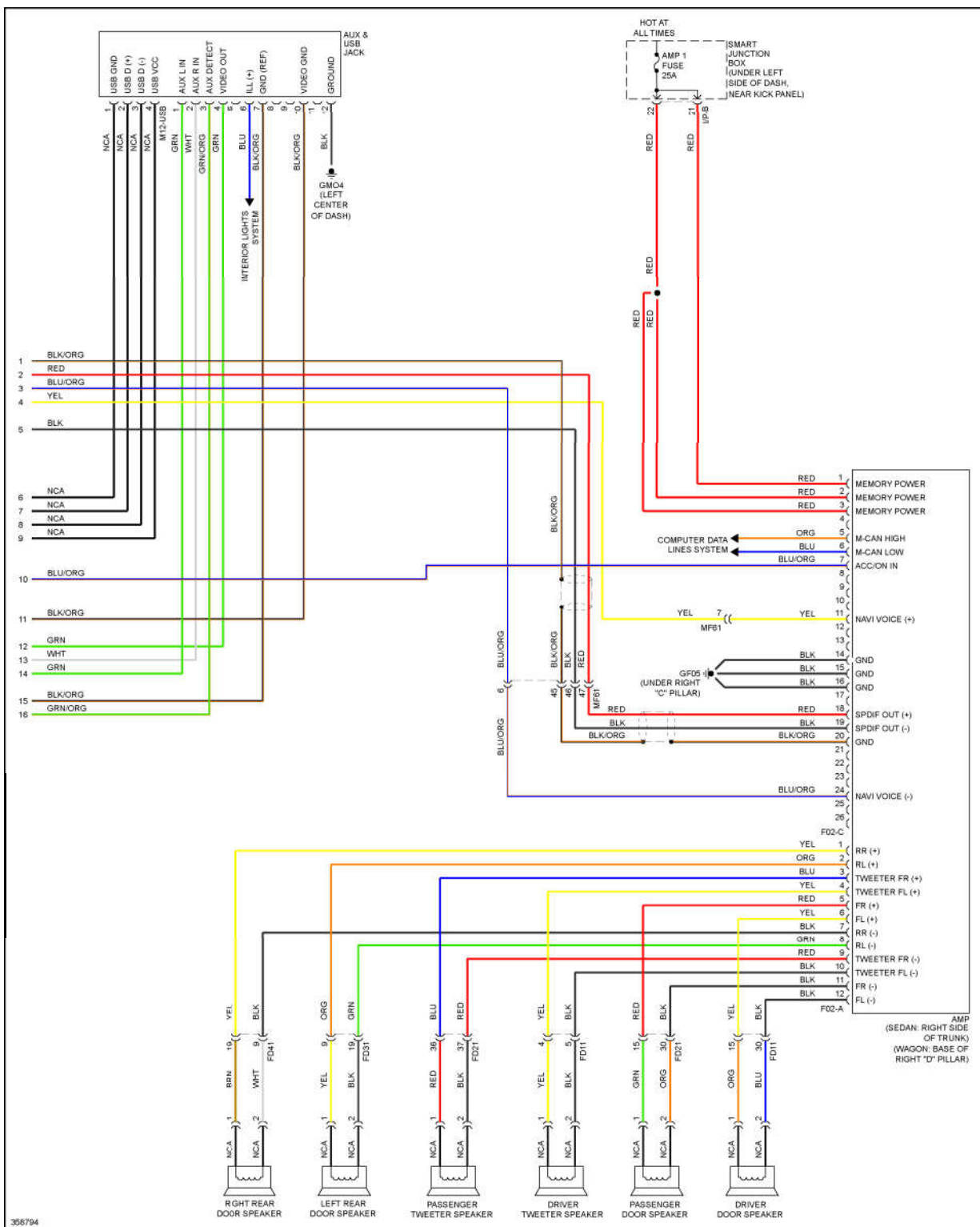
Fig. 72: Radio Circuit, W/ Navigation (2 of 2)
