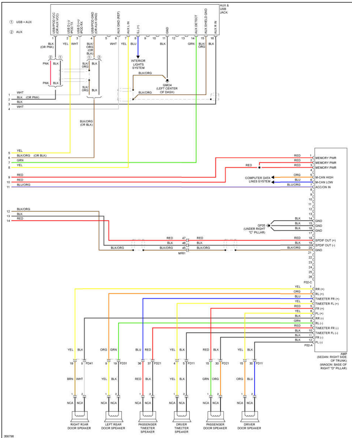
Fig. 70: Radio Circuit, W/ Amplifier (2 of 2)
