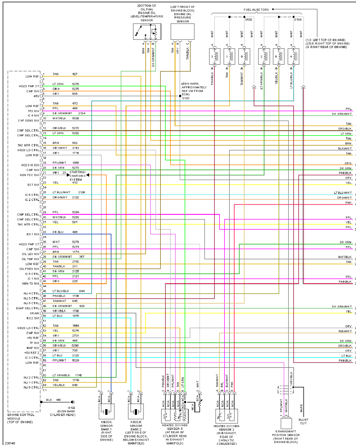
Fig. 20: 3.6L VIN 7, Engine Performance Circuit (1 of 4)
