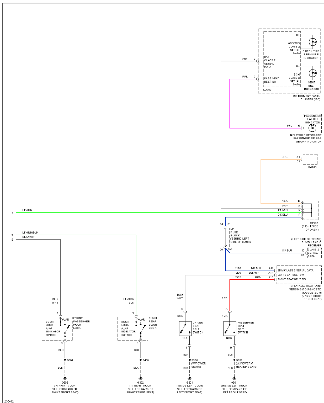
Fig. 71: Warning Systems Circuit (2 of 2)
