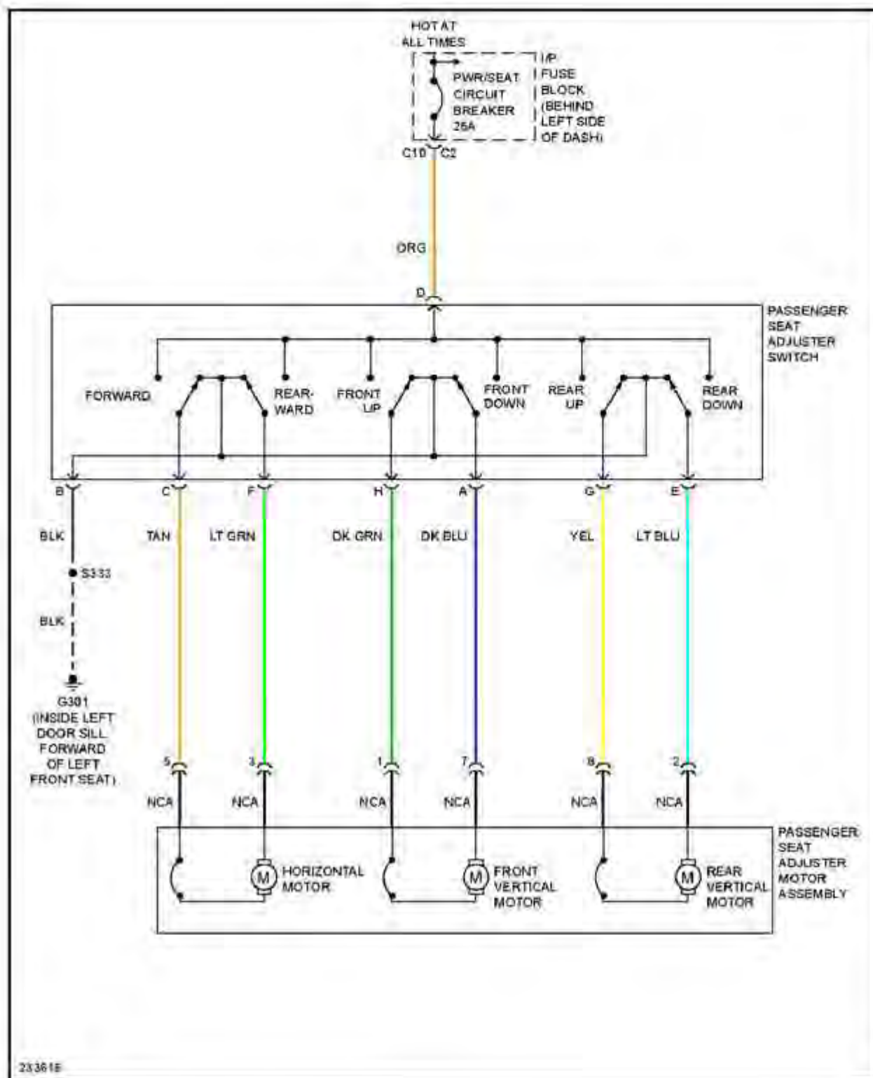
Fig. 54: Passenger's Power Seat Circuit
