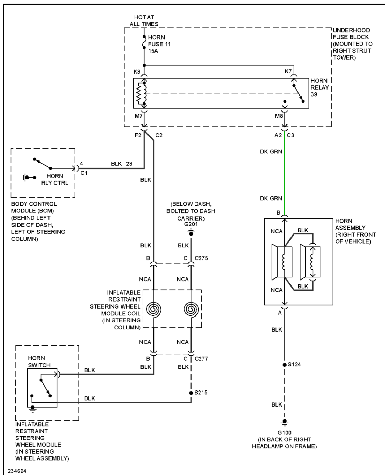
Fig. 36: Horn Circuit
