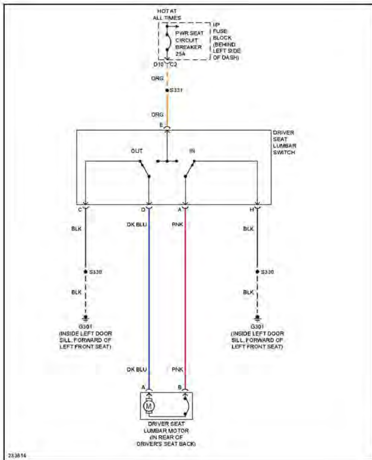
Fig. 52: Driver's Lumbar Circuit
