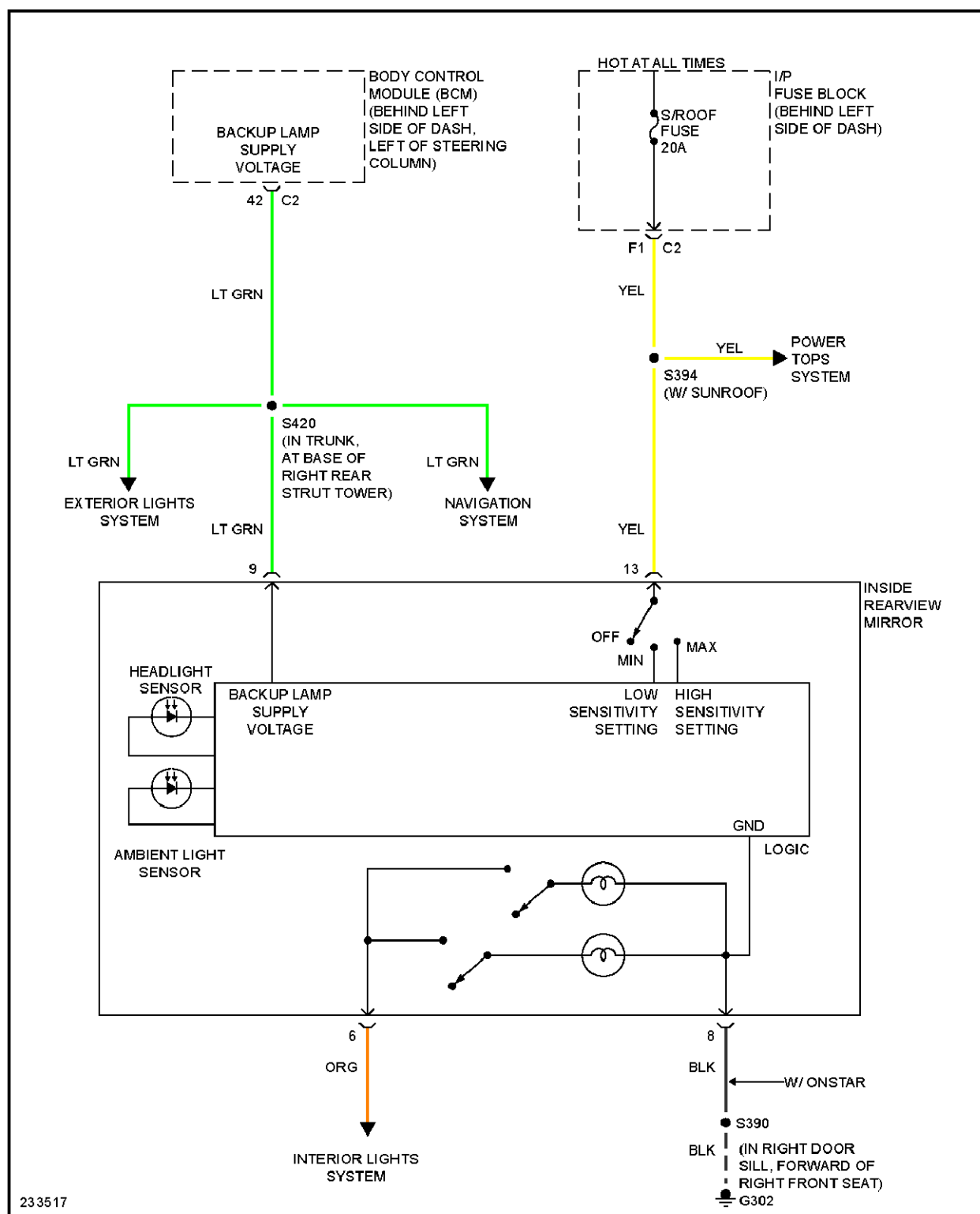
Fig. 49: Electrochromic Mirror Circuit
