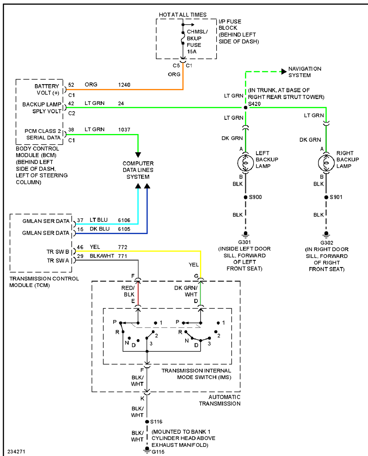
Fig. 30: 3.6L VIN 7, Backup Lamps Circuit
