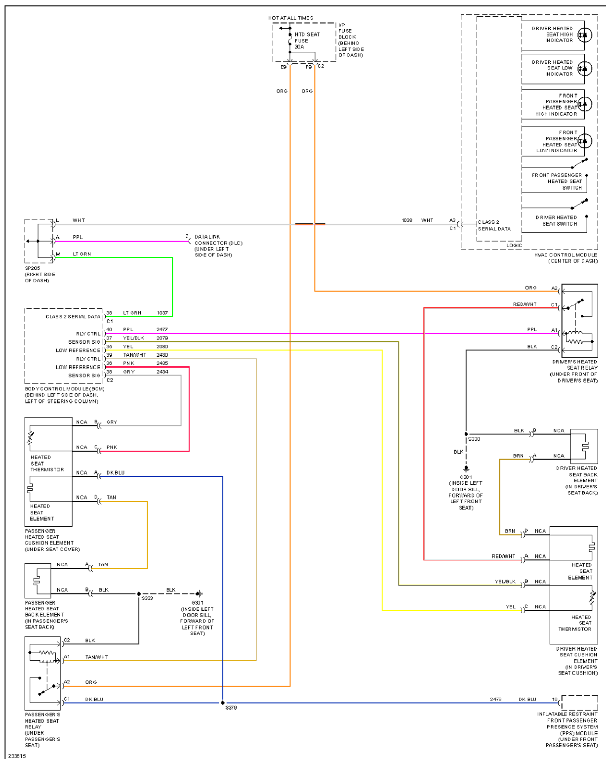
Fig. 53: Heated Seats Circuit
