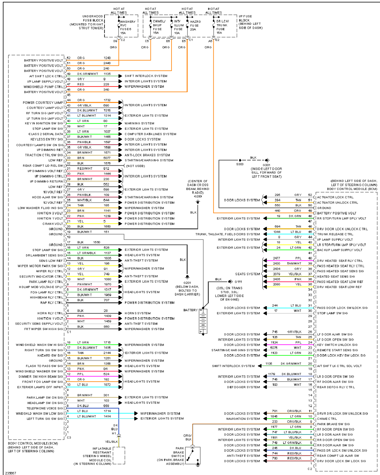
Fig. 12: Body Control Modules Circuit
