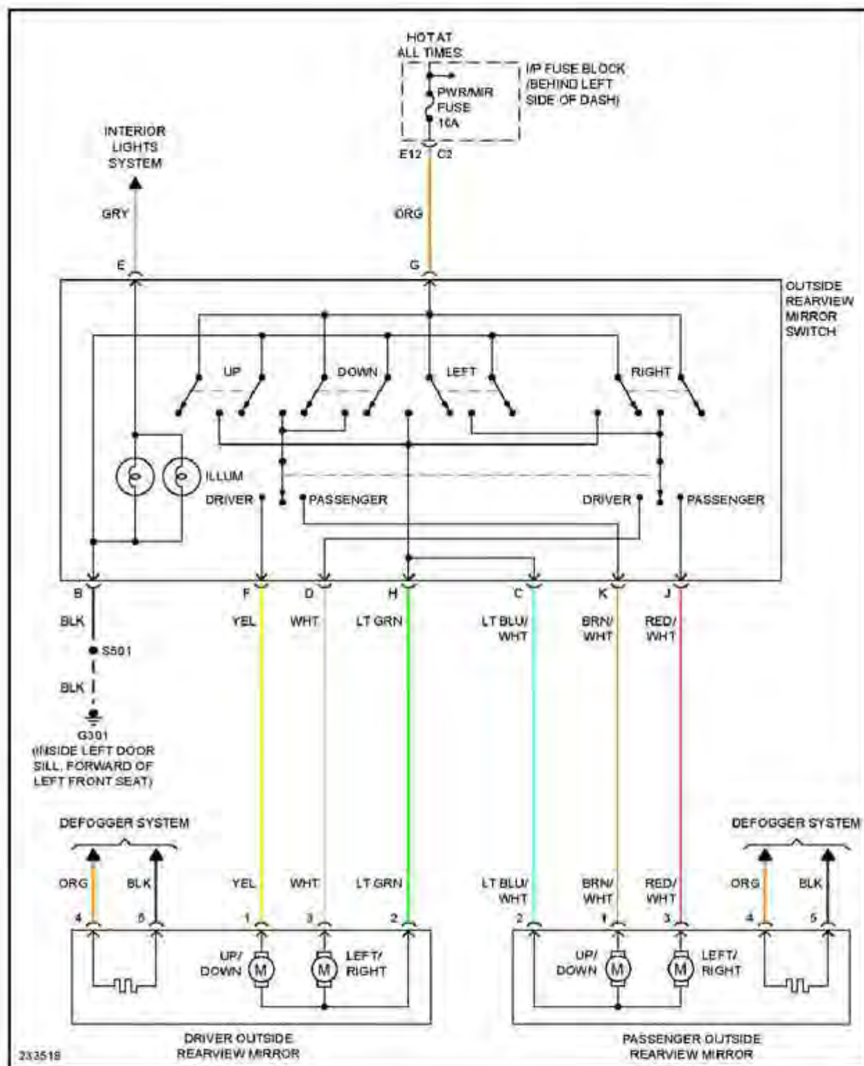
Fig. 50: Power Mirrors Circuit
