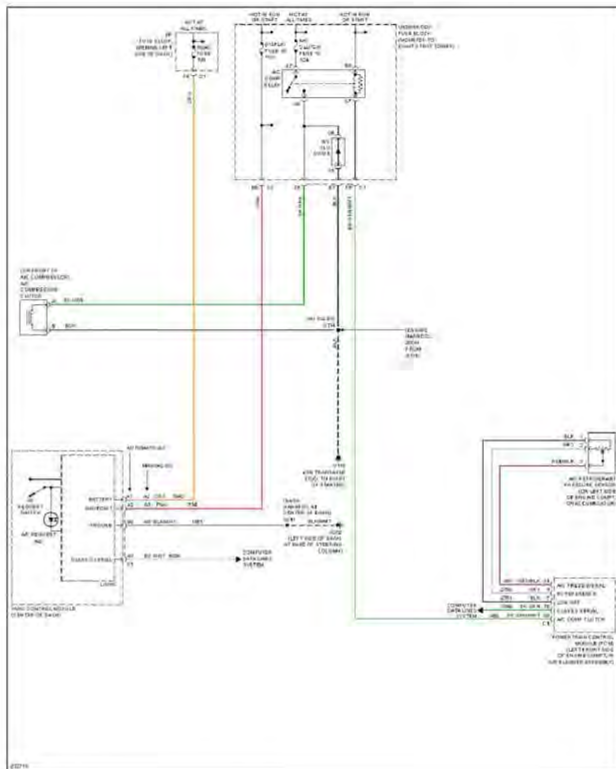
Fig. 6: 3.8L VIN 2, Compressor Circuit
