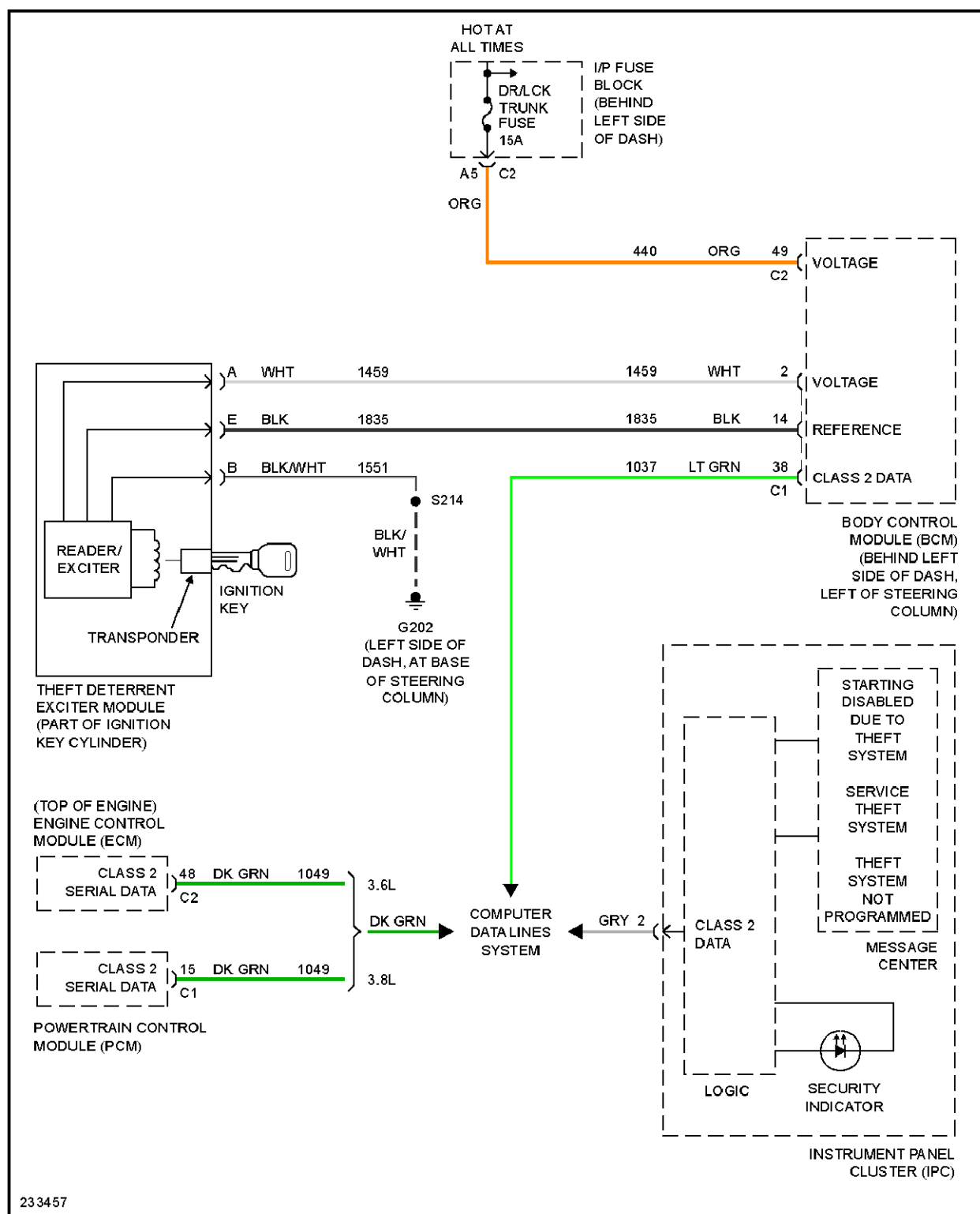
Fig. 11: Pass-Key Circuit
