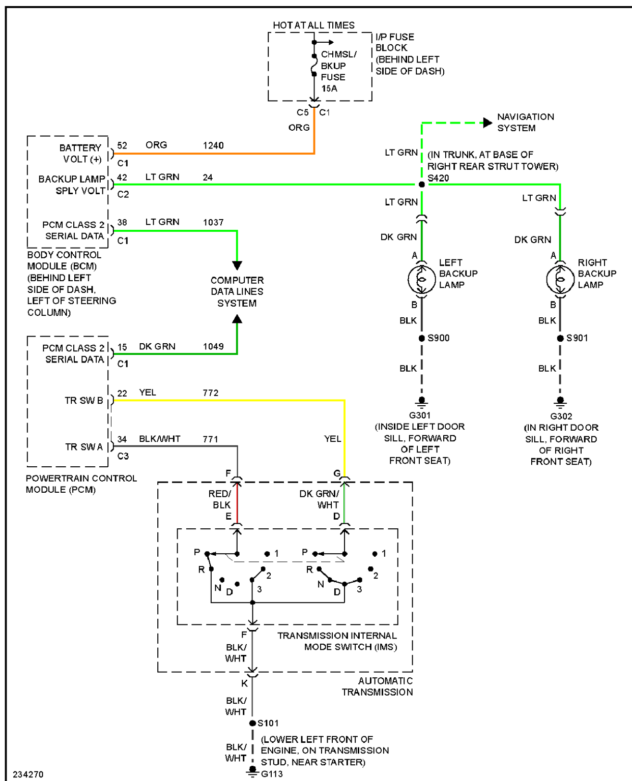
Fig. 31: 3.8L VIN 2, Backup Lamps Circuit
