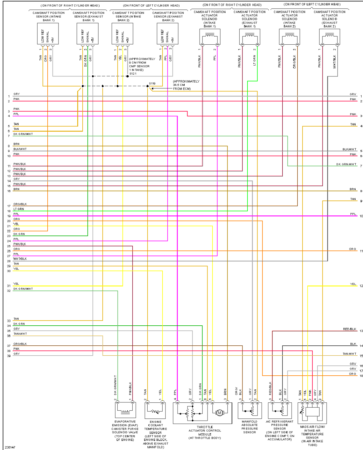
Fig. 22: 3.6L VIN 7, Engine Performance Circuit (3 of 4)
