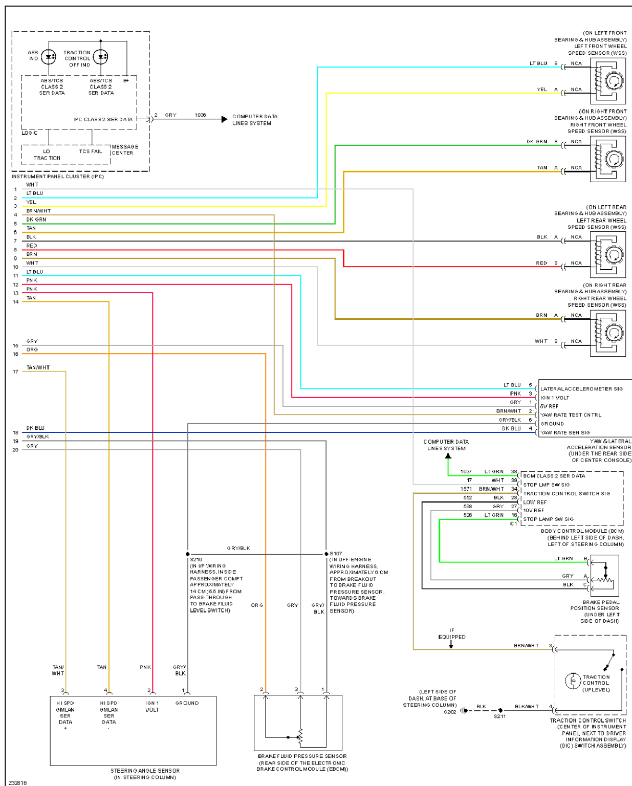
Fig. 9: Anti-lock Brakes Circuit (2 of 2)
