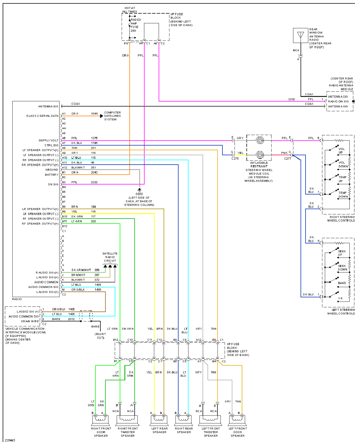
Fig. 58: Radio Circuit, W/O Amplifier
