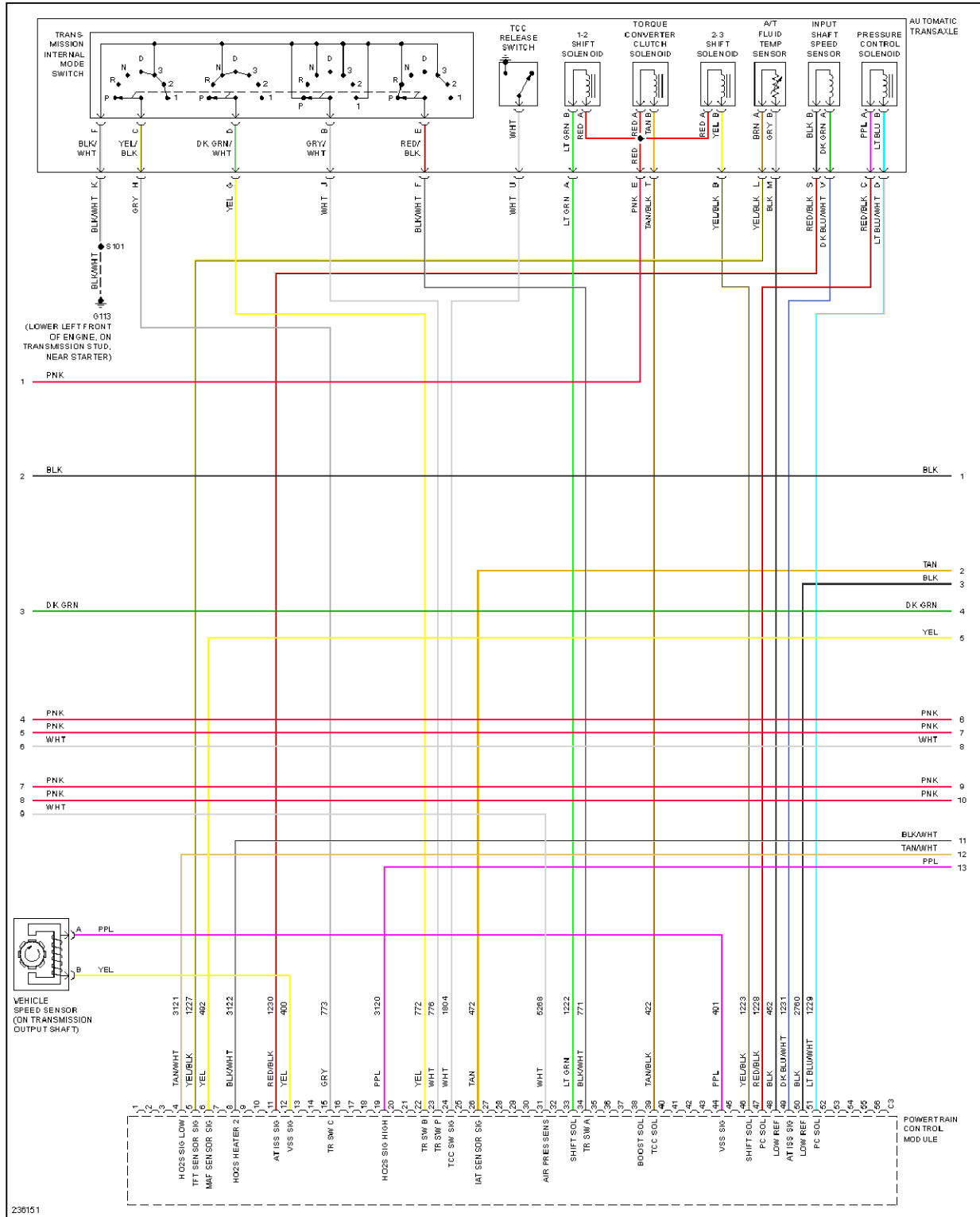
Fig. 26: 3.8L VIN 2, Engine Performance Circuit (3 of 5)
