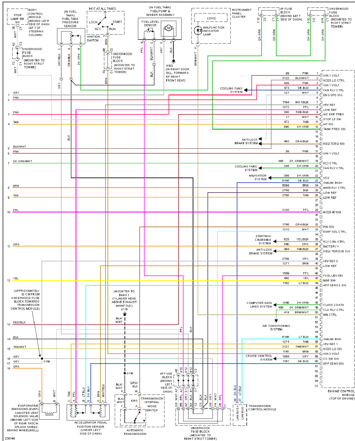
Fig. 23: 3.6L VIN 7, Engine Performance Circuit (4 of 4)
