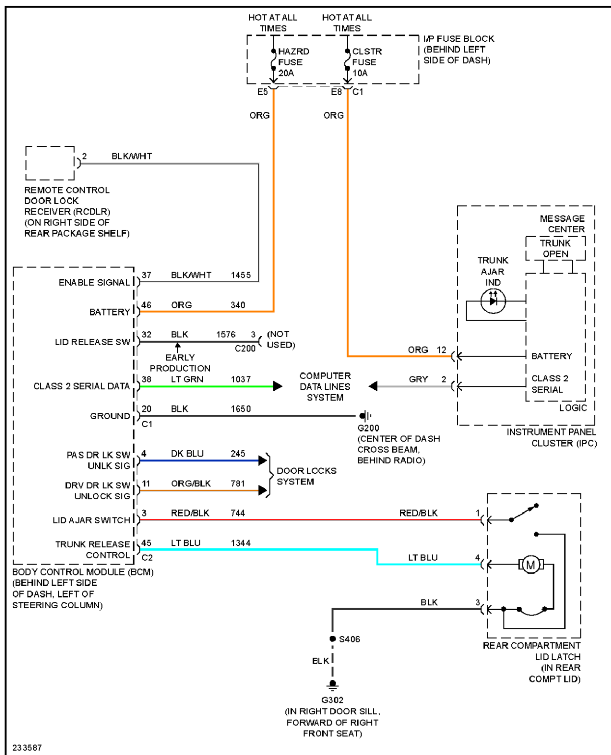
Fig. 69: Trunk Release Circuit
