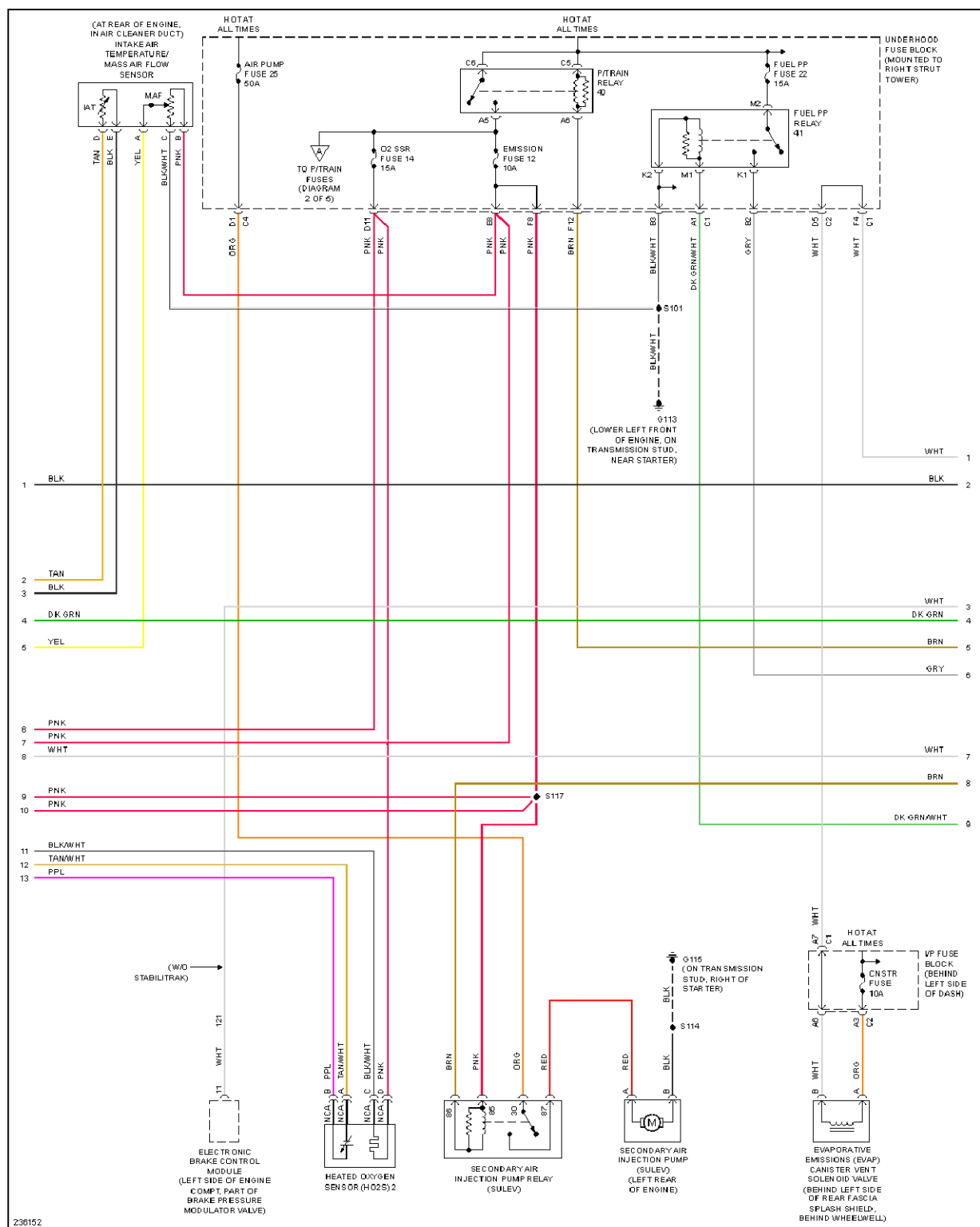
Fig. 27: 3.8L VIN 2, Engine Performance Circuit (4 of 5)
