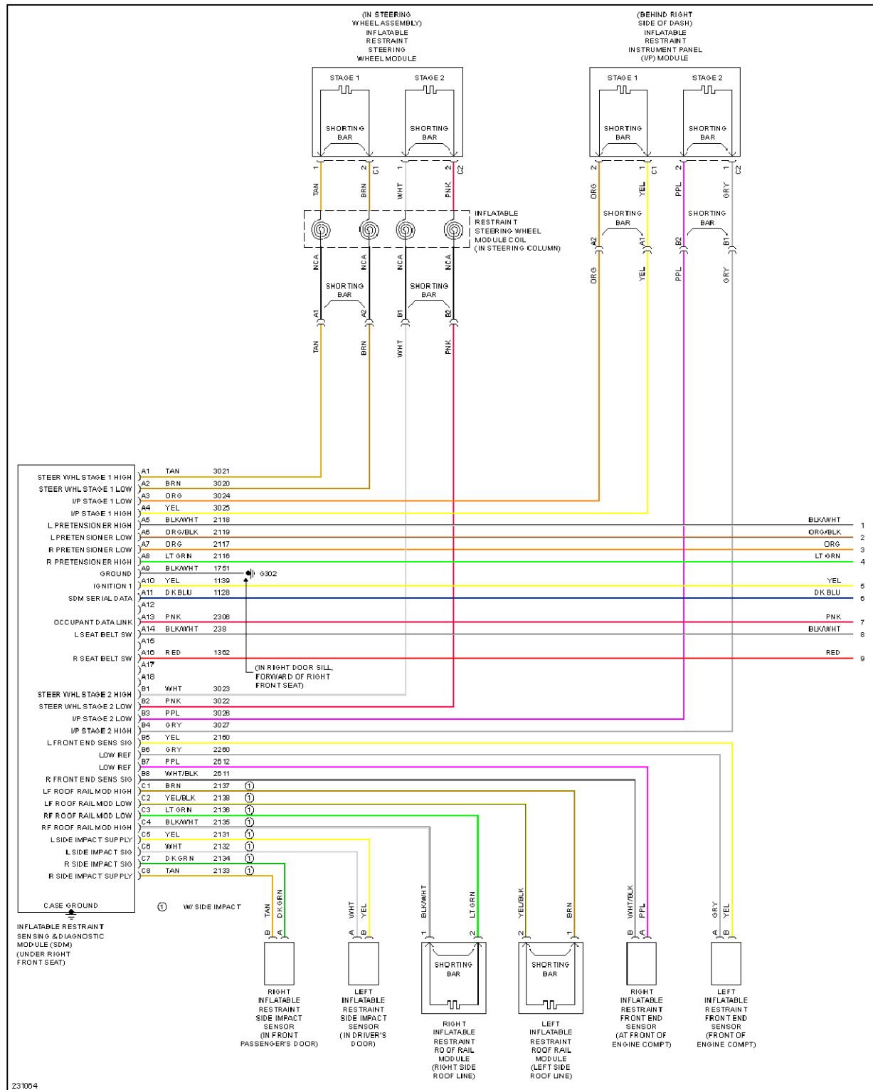
Fig. 65: Supplemental Restraints Circuit (1 of 2)
