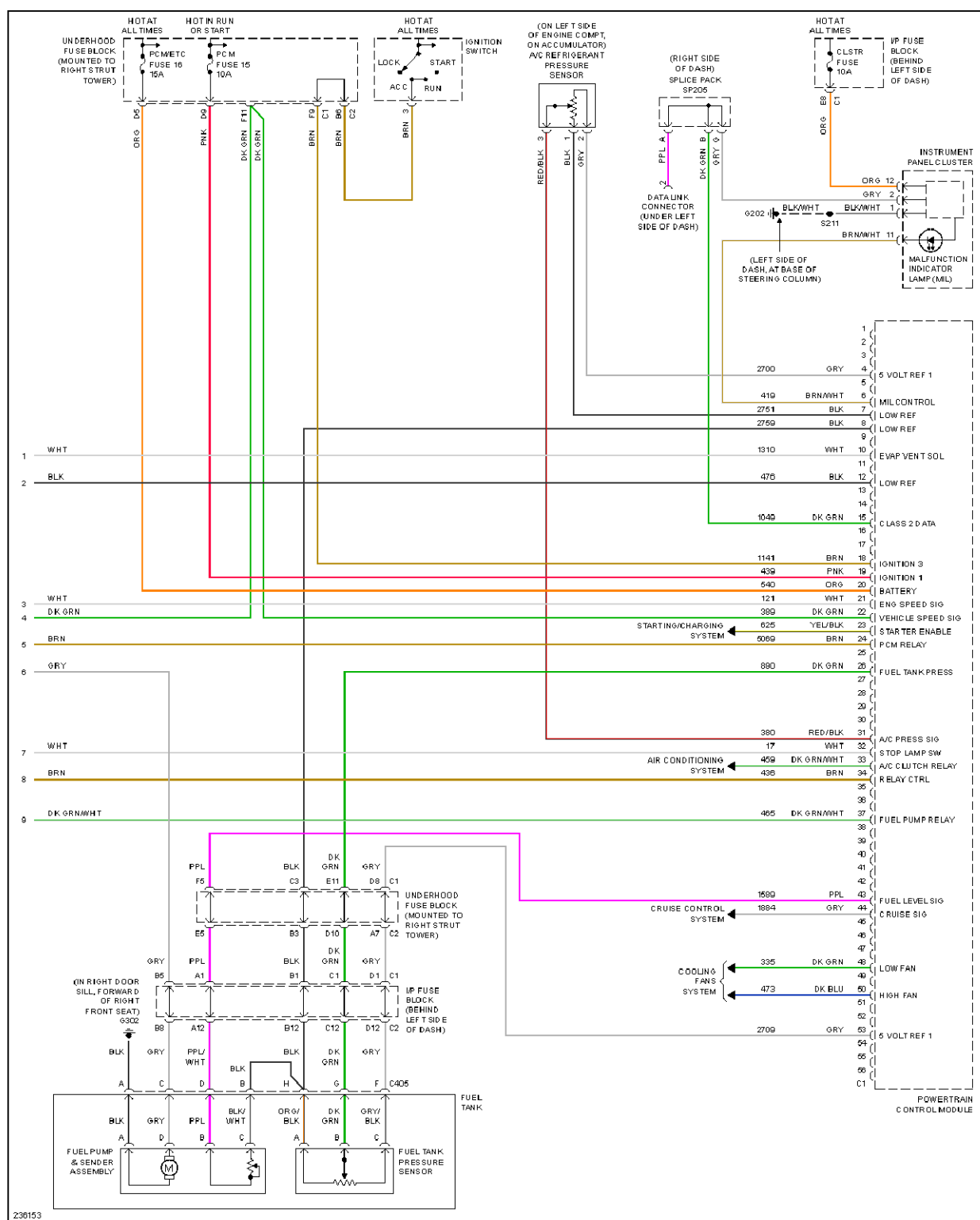
Fig. 28: 3.8L VIN 2, Engine Performance Circuit (5 of 5)
