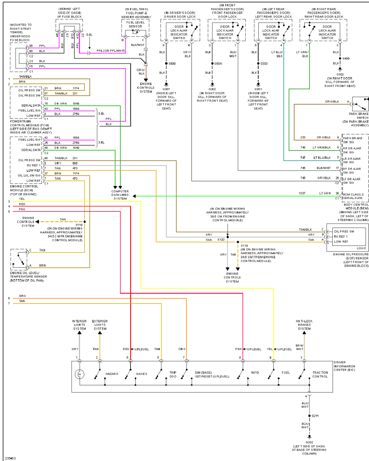
Fig. 38: Instrument Cluster Circuit, W/ Tachometer (2 of 2)
