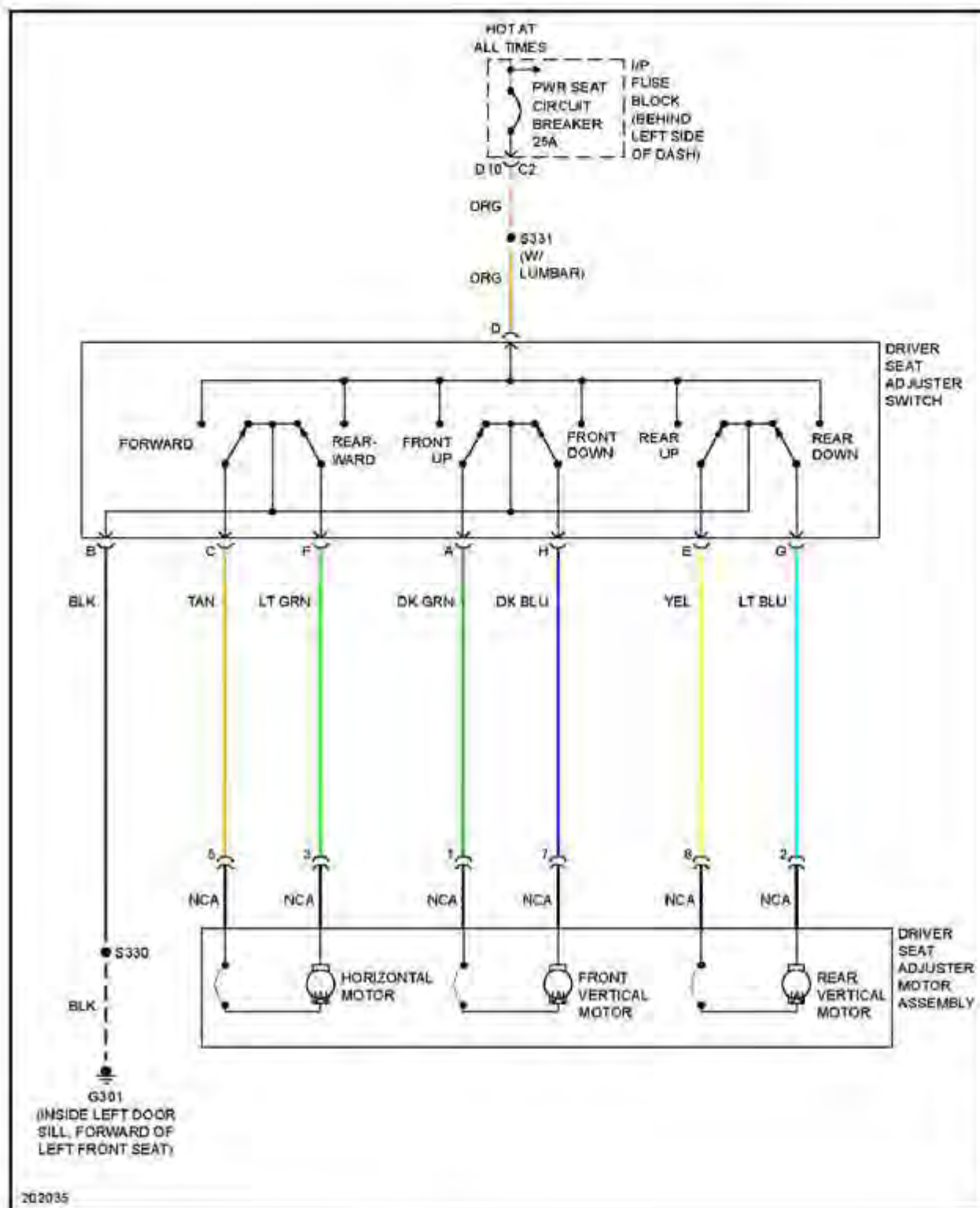
Fig. 51: Driver Power Seat Circuit
