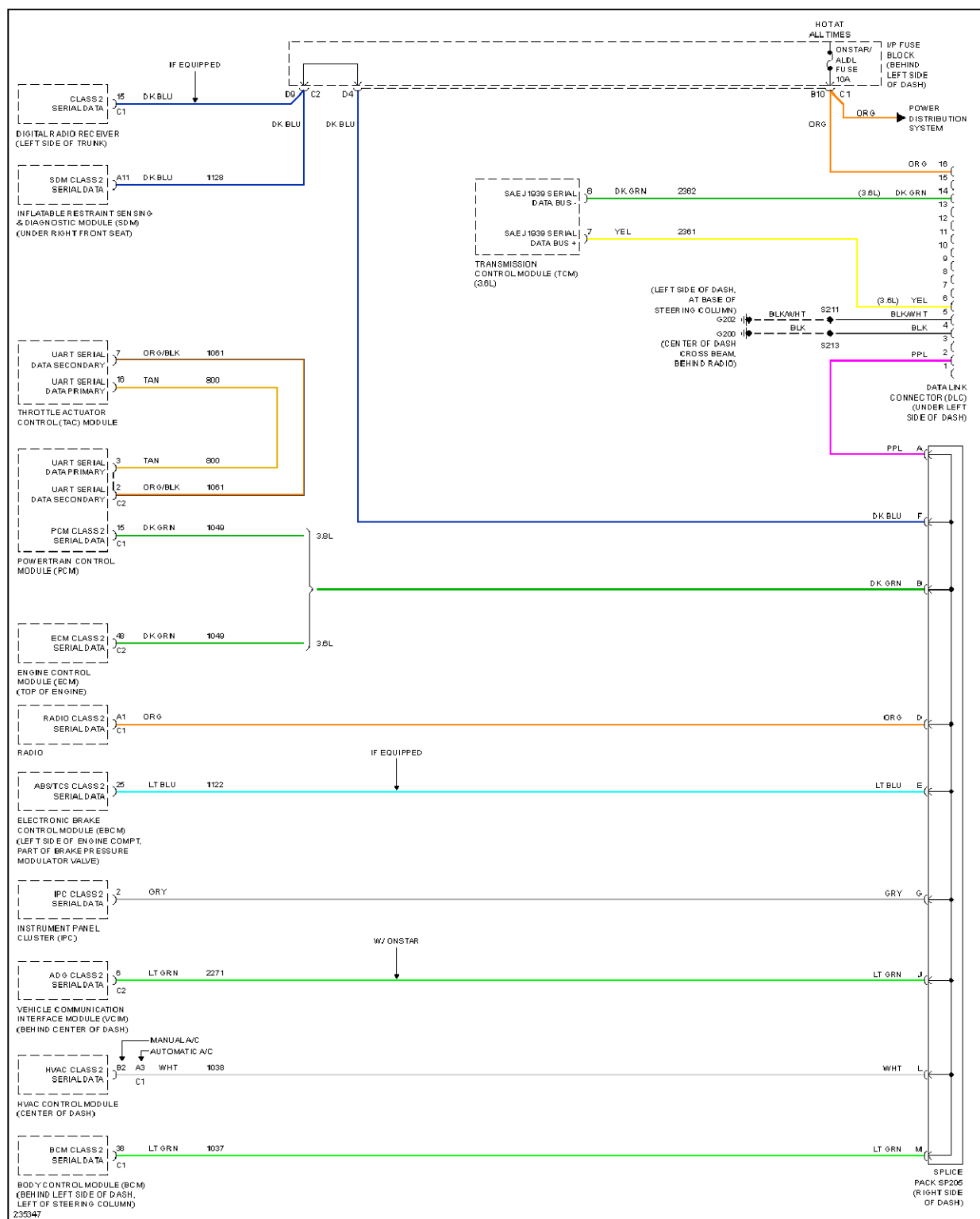
Fig. 13: Computer Data Lines Circuit
