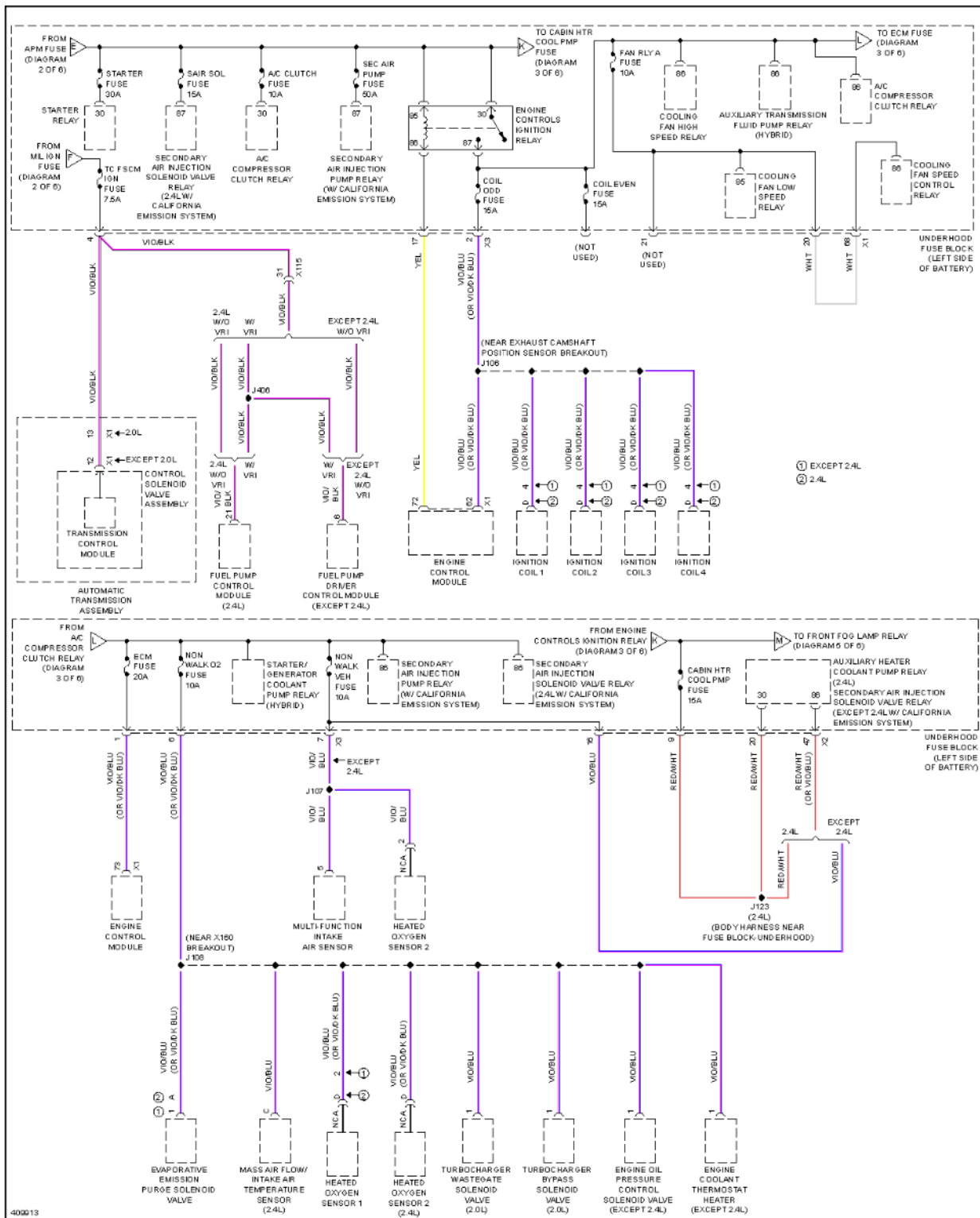
Fig. 90: Power Distribution Circuit (3 of 6)
