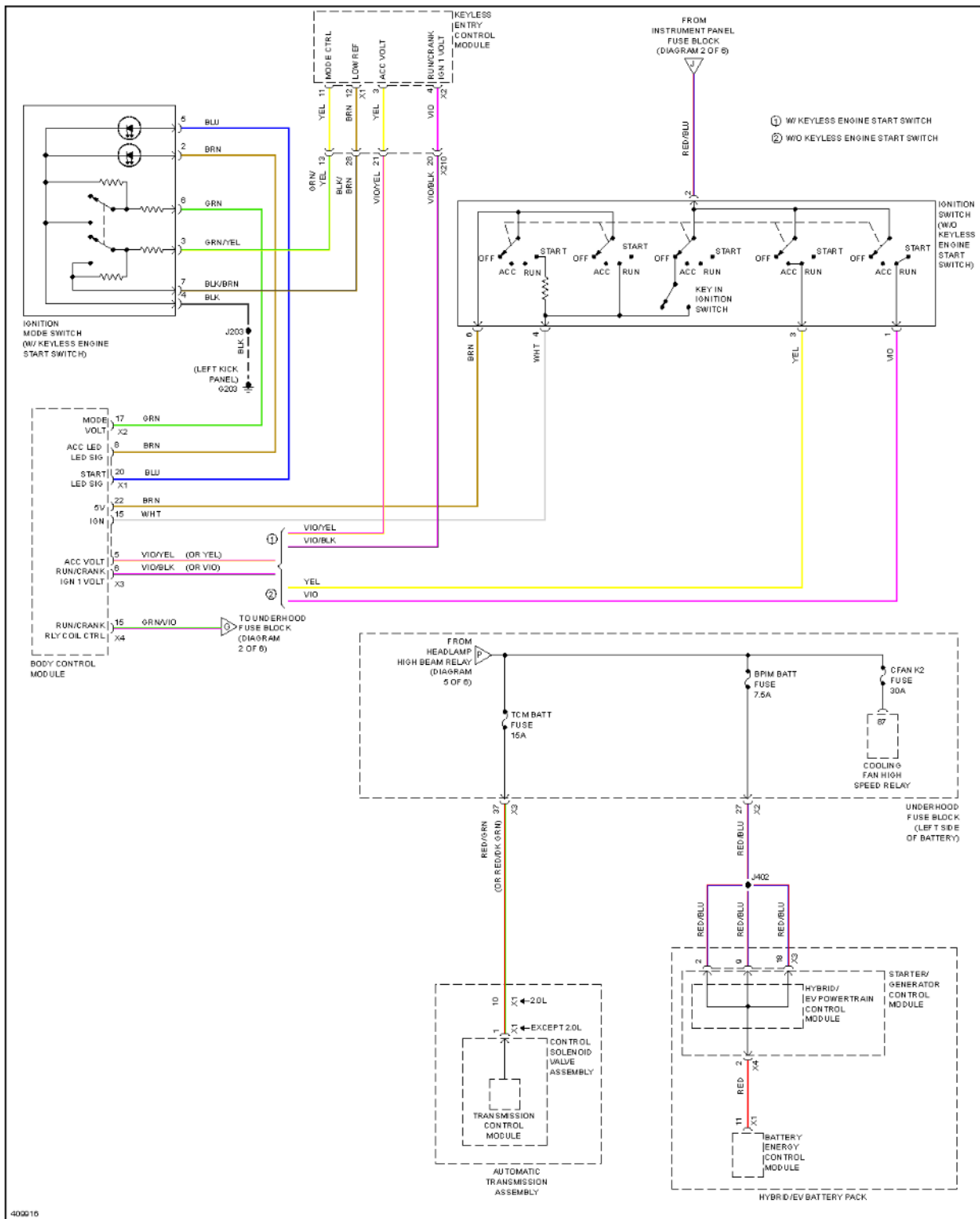
Fig. 93: Power Distribution Circuit (6 of 6)
