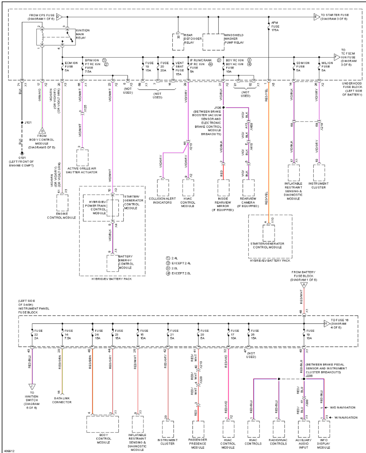
Fig. 89: Power Distribution Circuit (2 of 6)
